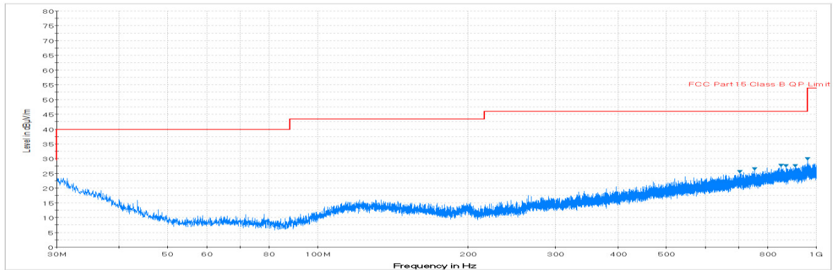
Plot 7-119. Radiated Spurious Plot below 1GHz (Pol. H)
