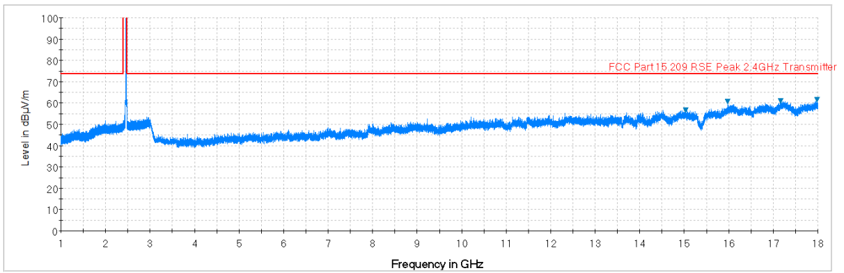
Plot 7-85. Radiated Spurious Plot above 1GHz (802.11b – Ch. 11, Ant. Pol. H)
