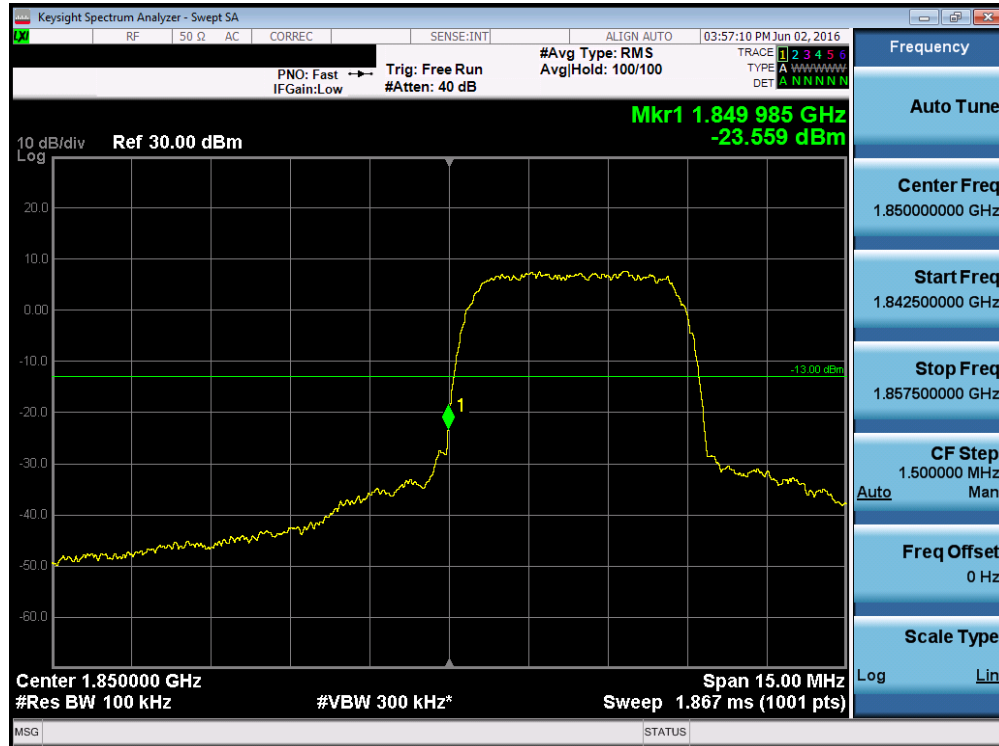
Plot 7-38. Band Edge Plot (PCS WCDMA Mode – Ch. 9262)
