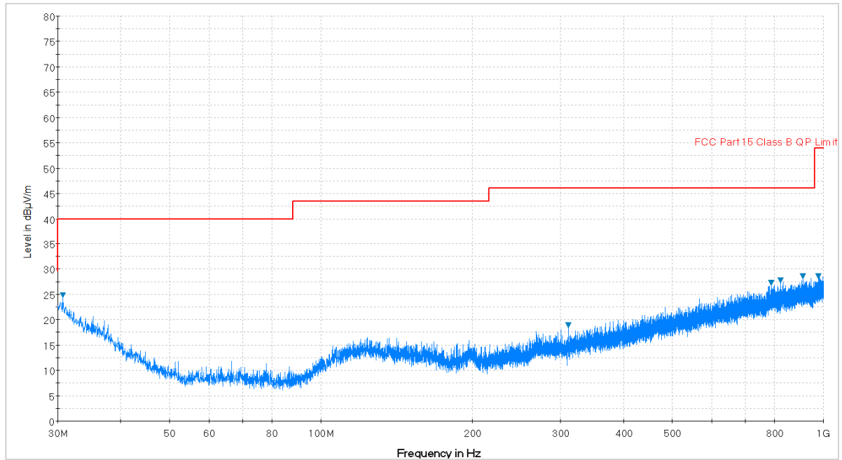
Plot 7-54. Radiated Spurious Plot below 1GHz (Pol. H)
