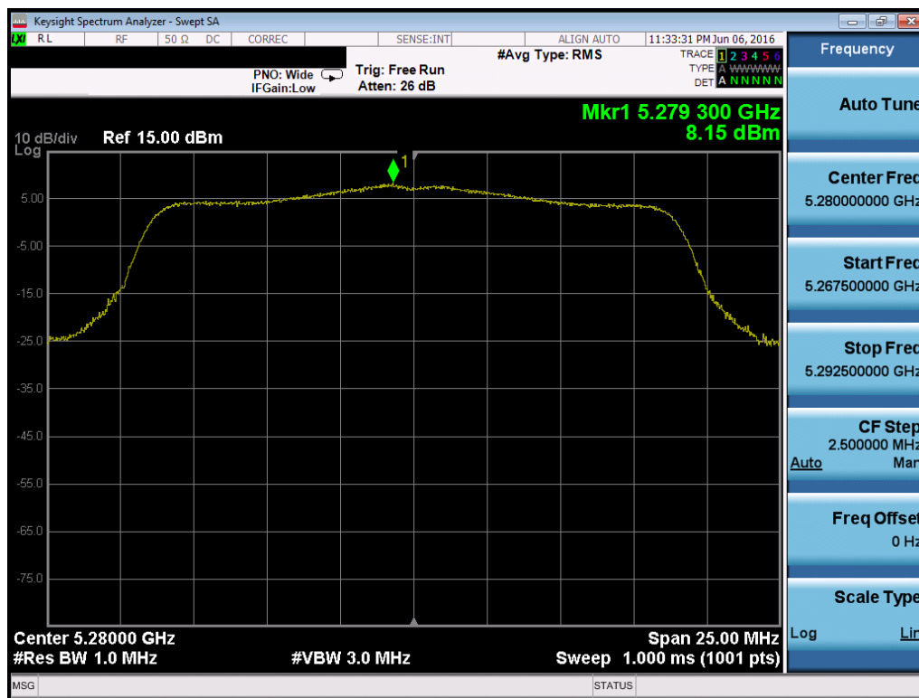
Plot 7-127. Power Spectral Density Plot (20MHz BW 802.11n (UNII Band 2A) – Ch. 56)
