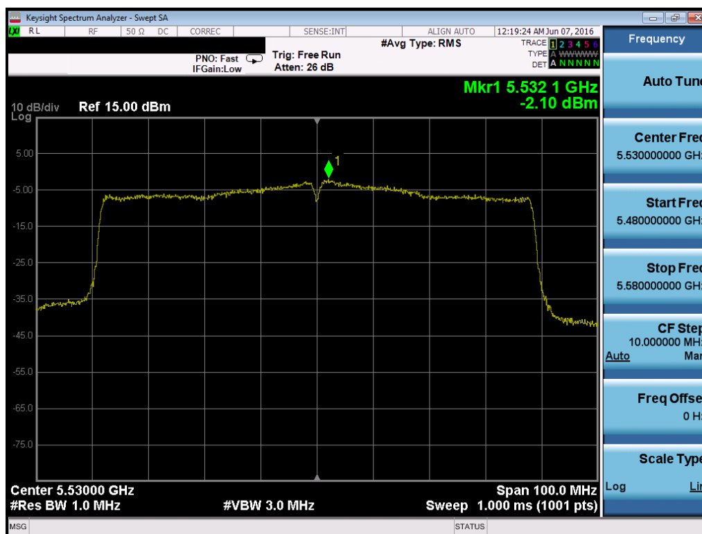
Plot 7-141. Power Spectral Density Plot (80MHz BW 802.11ac (UNII Band 2C) – Ch. 106)
