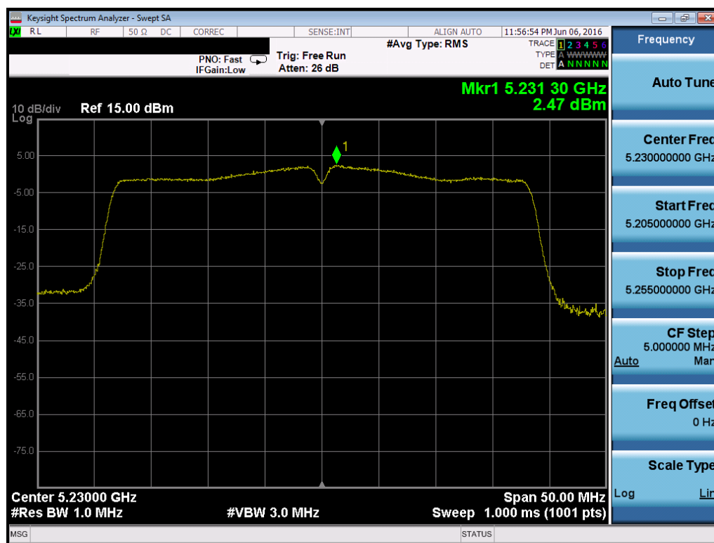
Plot 7-121. Power Spectral Density Plot (40MHz BW 802.11n (UNII Band 1) – Ch. 46)
