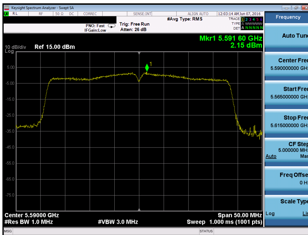
Plot 7-139. Power Spectral Density Plot (40MHz BW 802.11n (UNII Band 2C) – Ch. 118)
