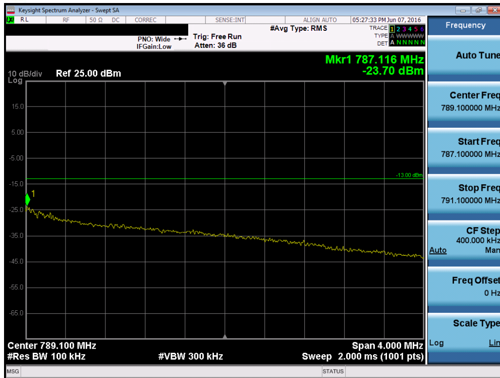
Plot 7-170. Upper Extended Band Edge Plot (Band 13 – 5.0MHz QPSK – RB Size 25)
