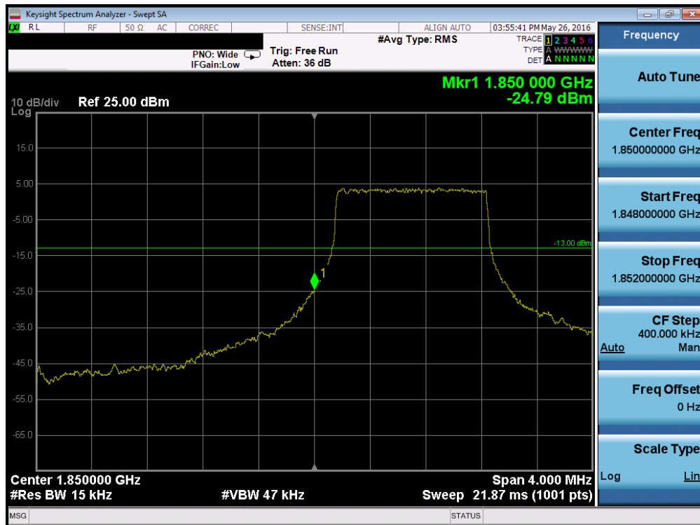
Plot 7-216. Lower Band Edge Plot (Band 2 – 1.4MHz QPSK – RB Size 6)
