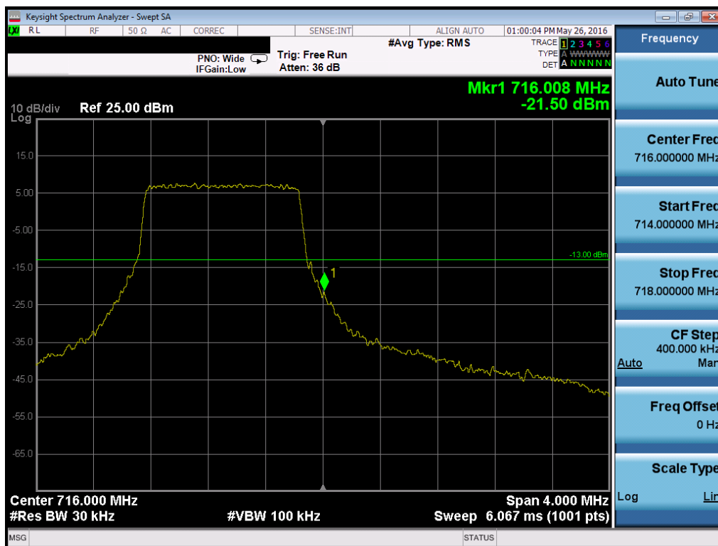
Plot 7-157. Upper Band Edge Plot (Band 12 – 1.4MHz QPSK – RB Size 6)
