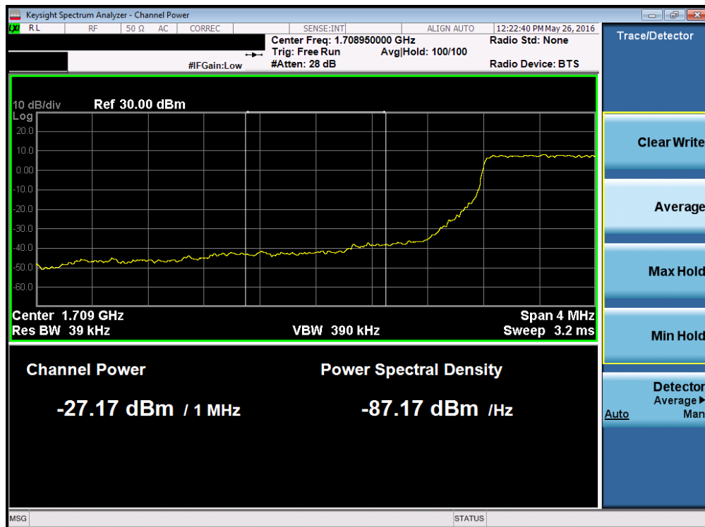
Plot 7-193. Lower Extended Band Edge Plot (Band 4 – 1.4MHz QPSK – RB Size 6)
