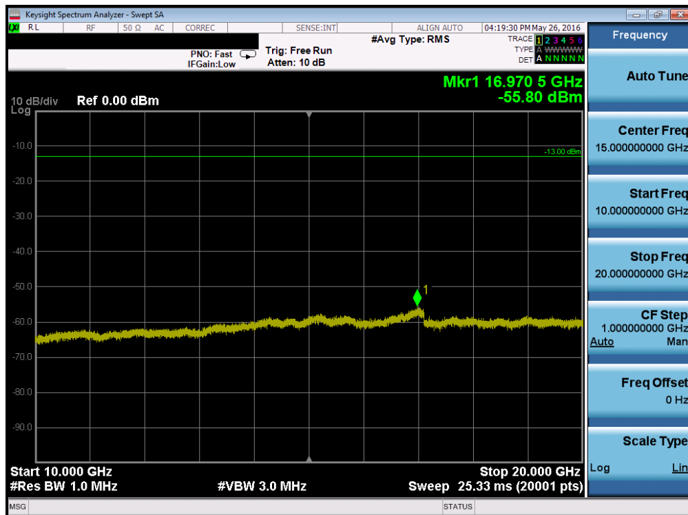
Plot 7-128. Conducted Spurious Plot (Band 2 – 3.0MHz QPSK – RB Size 1, RB Offset 0 – High Channel)
