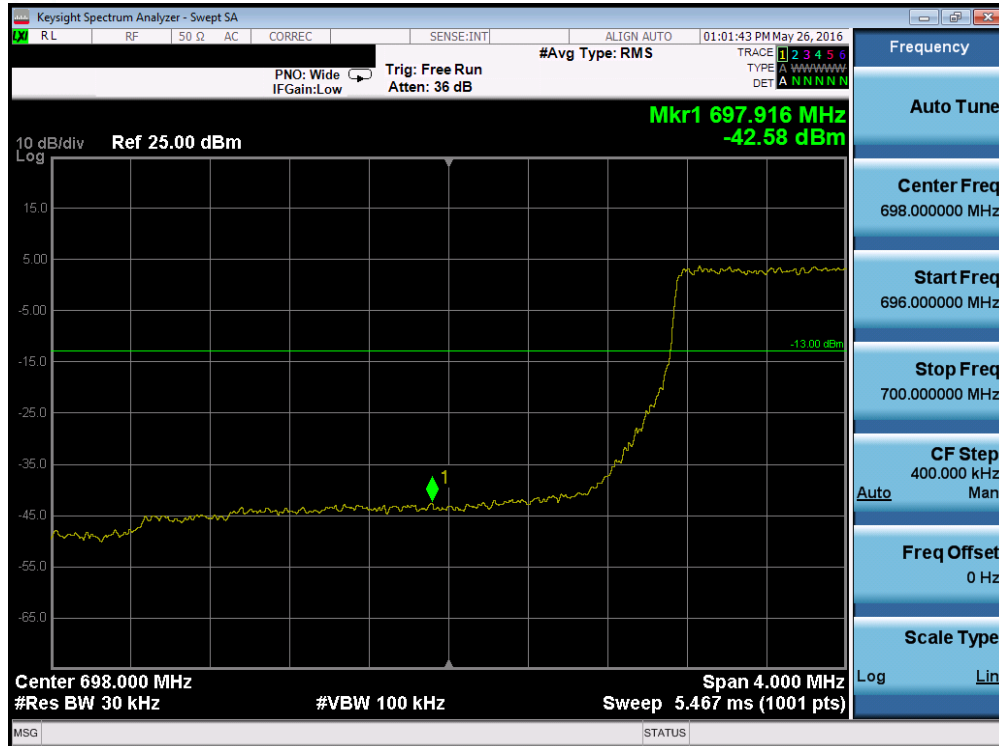
Plot 7-158. Lower Band Edge Plot (Band 12 – 3.0MHz QPSK – RB Size 15)
