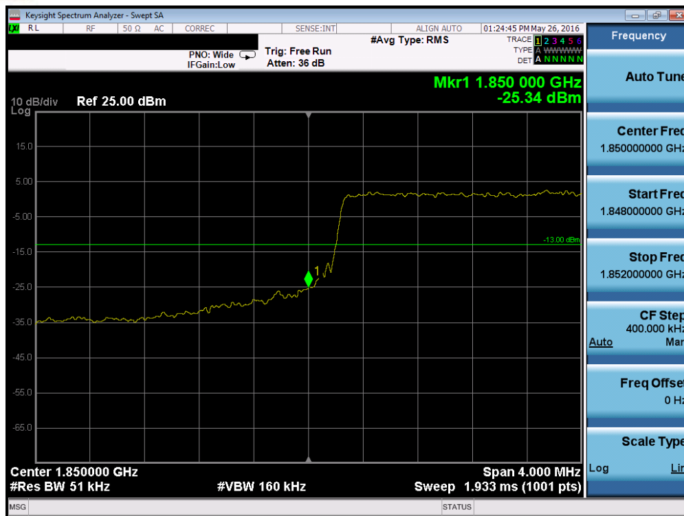
Plot 7-248. Lower Band Edge Plot (Band 25 – 5.0MHz QPSK – RB Size 25)
