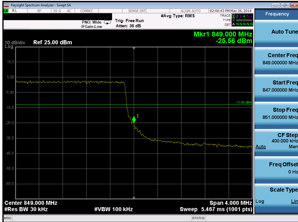
Plot 7-182. Upper Band Edge Plot (Band 26 – 3.0MHz QPSK – RB Size 15)
