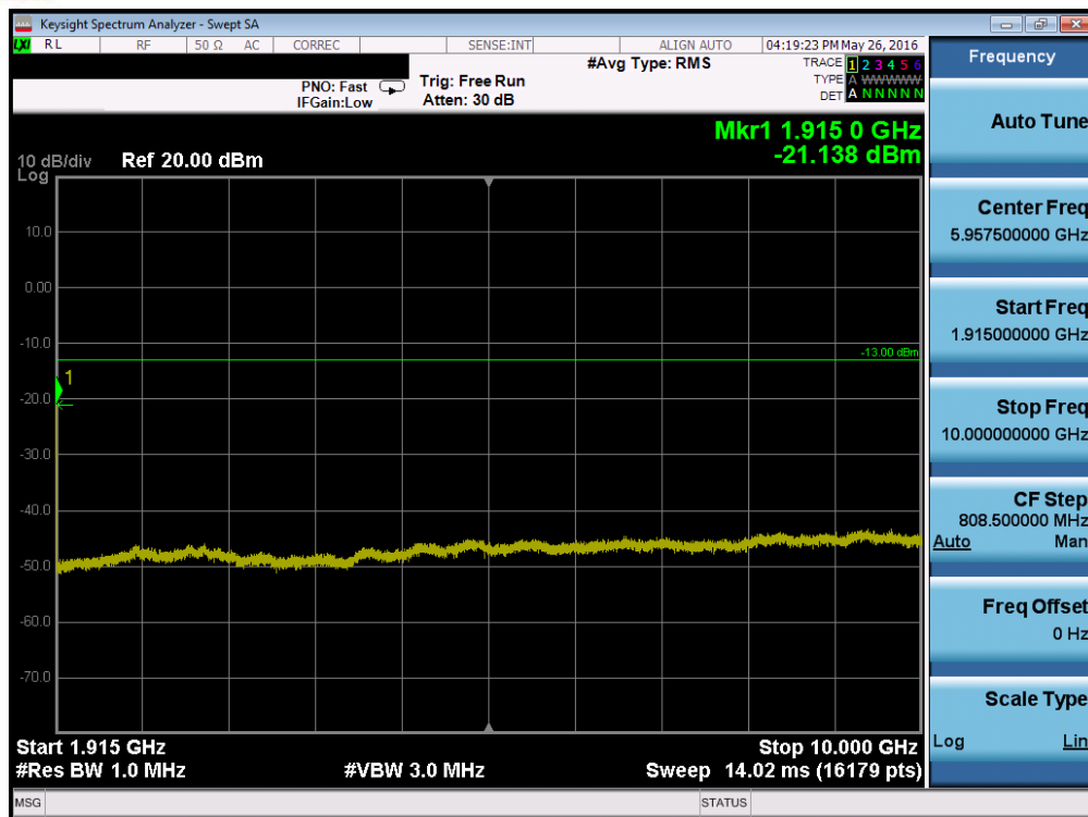
Plot 7-127. Conducted Spurious Plot (Band 2 – 3.0MHz QPSK – RB Size 1, RB Offset 0 – High Channel)
