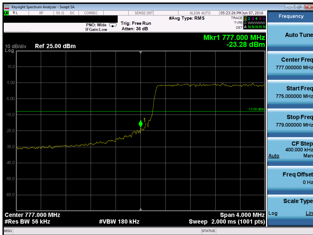
Plot 7-166. Lower Band Edge Plot (Band 13 – 5.0MHz QPSK – RB Size 25)
