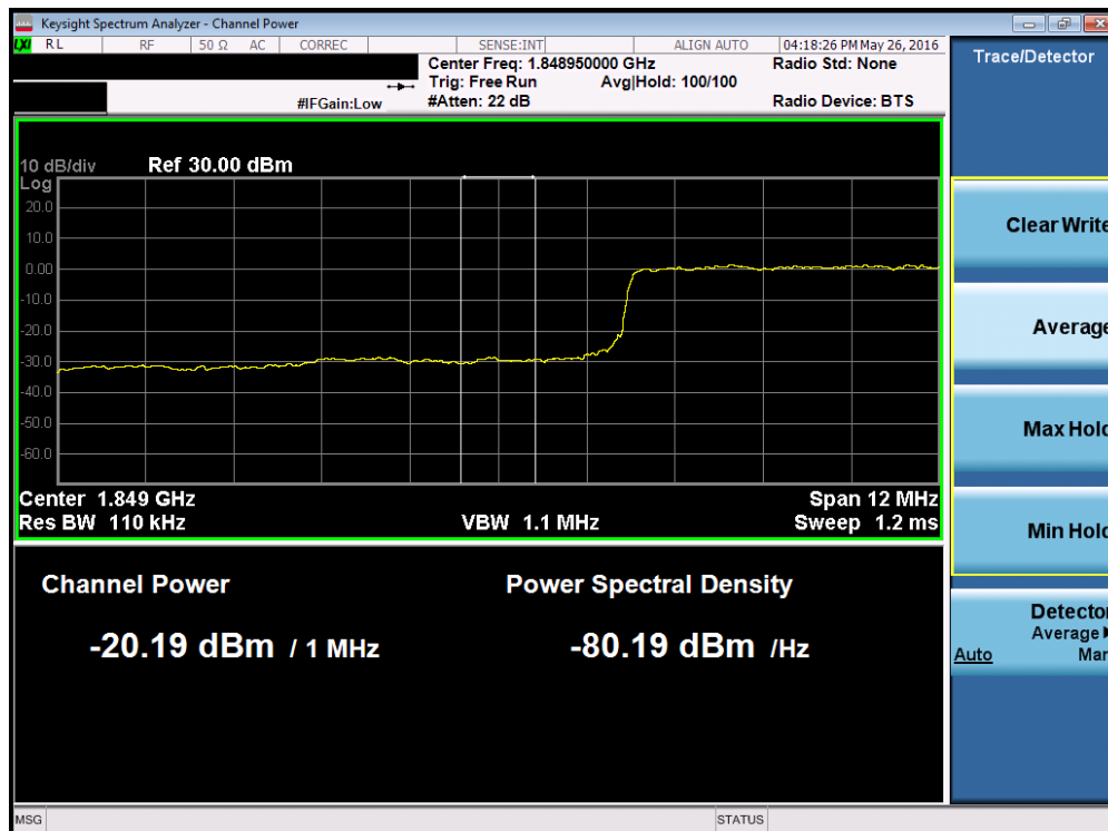
Plot 7-233. Lower Extended Band Edge Plot (Band 2 – 15.0MHz QPSK – RB Size 75)
