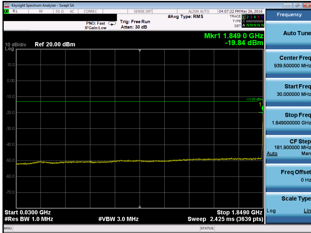
Plot 7-129. Conducted Spurious Plot (Band 2 – 10.0MHz QPSK – RB Size 1, RB Offset 0– Low Channel)
