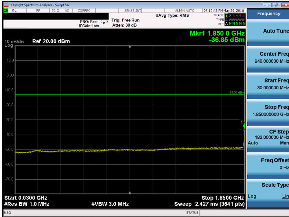
Plot 7-123. Conducted Spurious Plot (Band 2 – 3.0MHz QPSK – RB Size 1, RB Offset 0 – Mid Channel)
