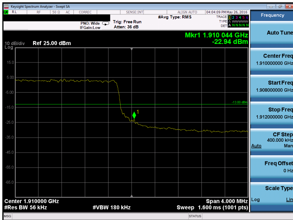
Plot 7-226. Upper Band Edge Plot (Band 2 – 5.0MHz QPSK – RB Size 25)
