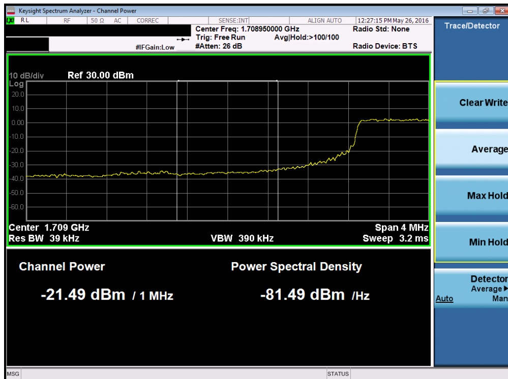
Plot 7-201. Lower Extended Band Edge Plot (Band 4 – 5.0MHz QPSK – RB Size 25)
