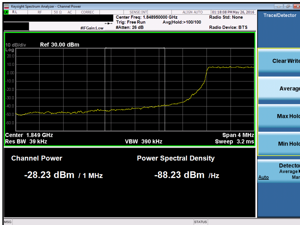
Plot 7-241. Lower Extended Band Edge Plot (Band 25 – 1.4MHz QPSK – RB Size 6)
