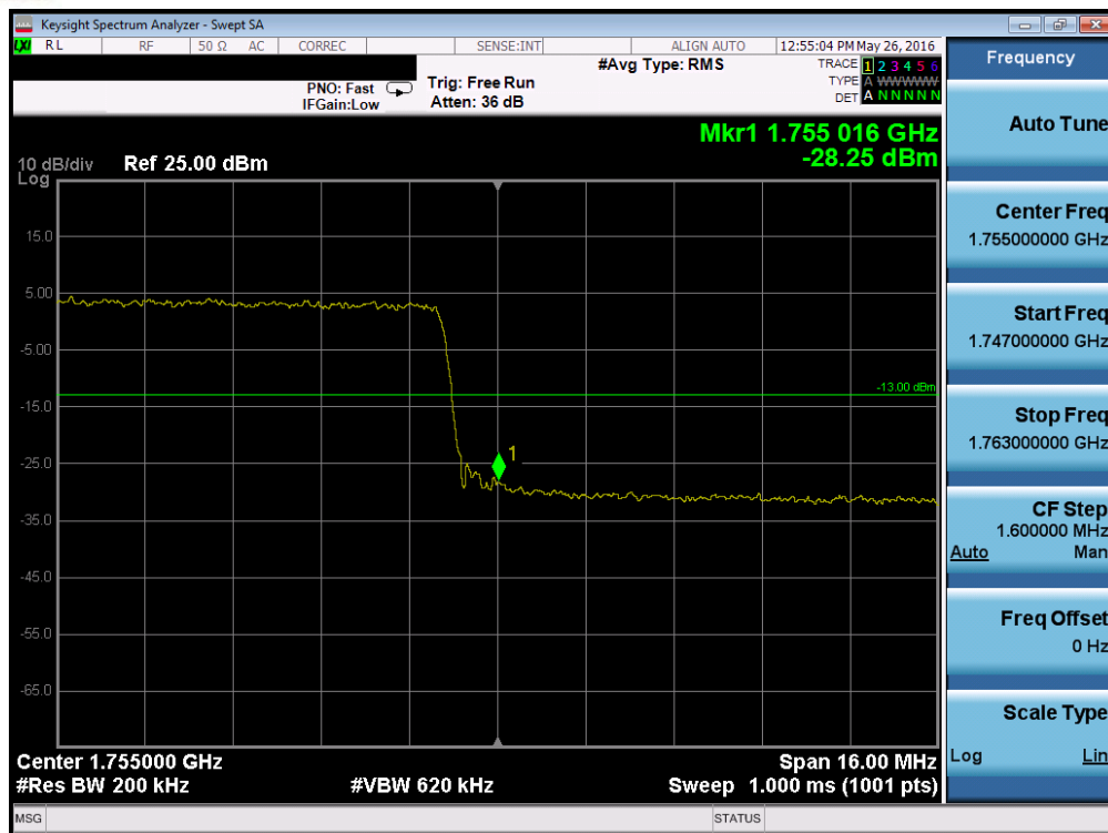
Plot 7-214. Upper Band Edge Plot (Band 4 – 20.0MHz QPSK – RB Size 100)
