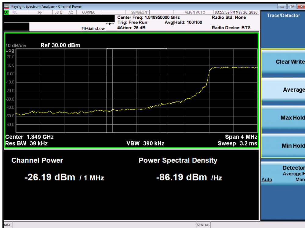
Plot 7-217. Lower Extended Band Edge Plot (Band 2 – 1.4MHz QPSK – RB Size 6)
