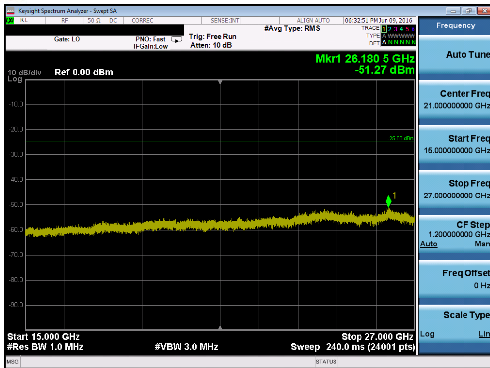
Plot 7-155. Conducted Spurious Plot (Band 41 – 5.0MHz QPSK – RB Size 1, RB Offset 0 – High Channel)
