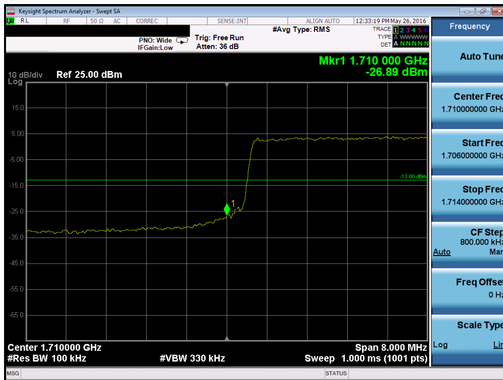
Plot 7-204. Lower Band Edge Plot (Band 4 – 10.0MHz QPSK – RB Size 50)
