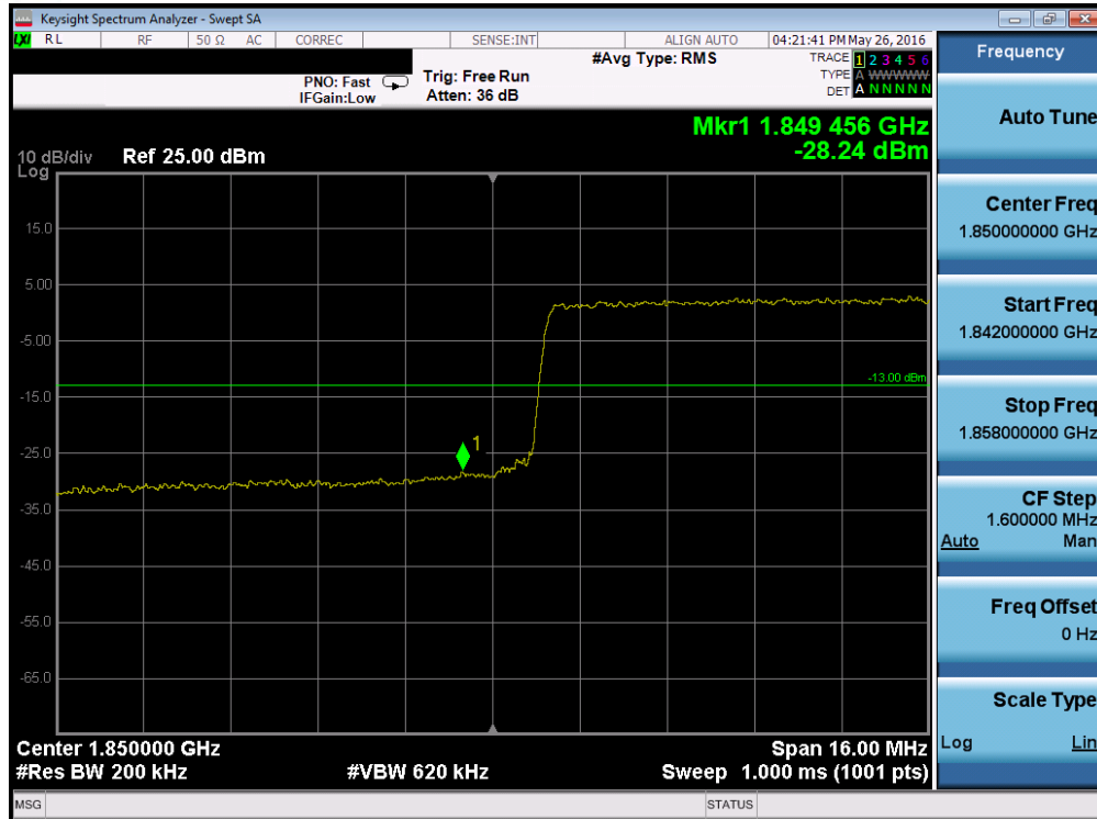
Plot 7-236. Lower Band Edge Plot (Band 2 - 20.0MHz QPSK - RB Size 100)
