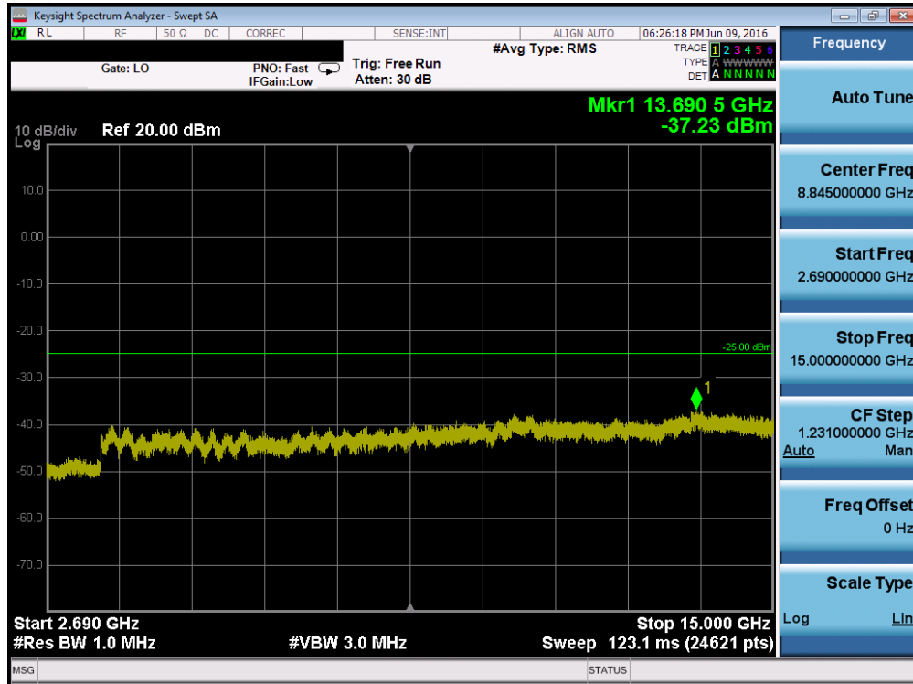
Plot 7-151. Conducted Spurious Plot (Band 41 – 5.0MHz QPSK – RB Size 1, RB Offset 0 – Mid Channel)
