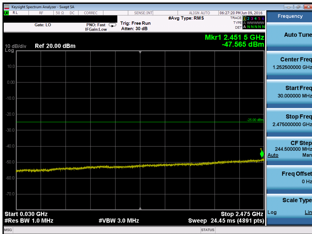
Plot 7-147. Conducted Spurious Plot (Band 41 – 5.0MHz QPSK – RB Size 1, RB Offset 0 – Low Channel)
