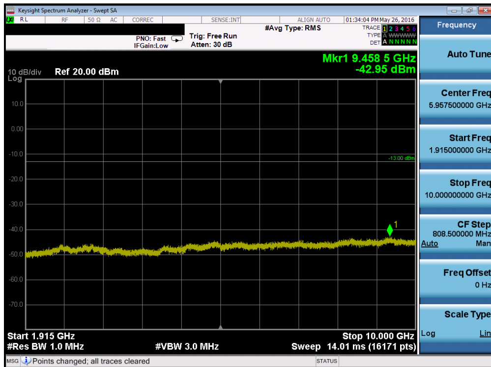
Plot 7-142. Conducted Spurious Plot (Band 25 – 3.0MHz QPSK – RB Size 1, RB Offset 0 – Mid Channel)
