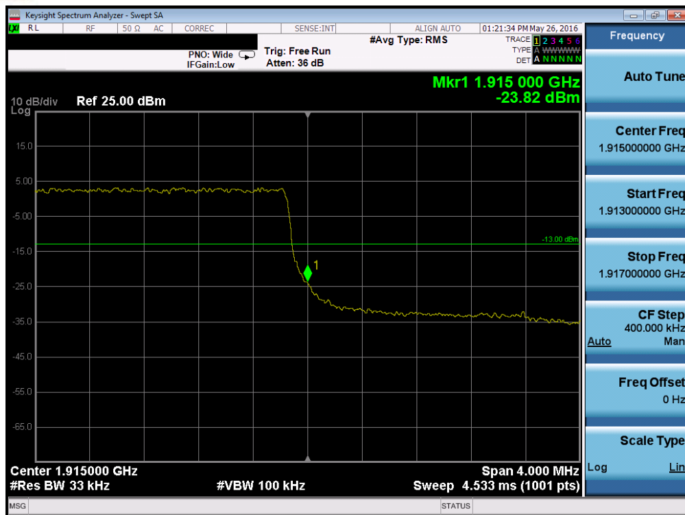
Plot 7-246. Upper Band Edge Plot (Band 25 – 3.0MHz QPSK – RB Size 15)
