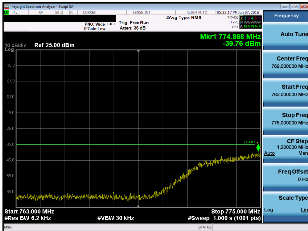
Plot 7-173. Lower Emission Mask Edge Plot (Band 13 – 10.0MHz QPSK – RB Size 50)
