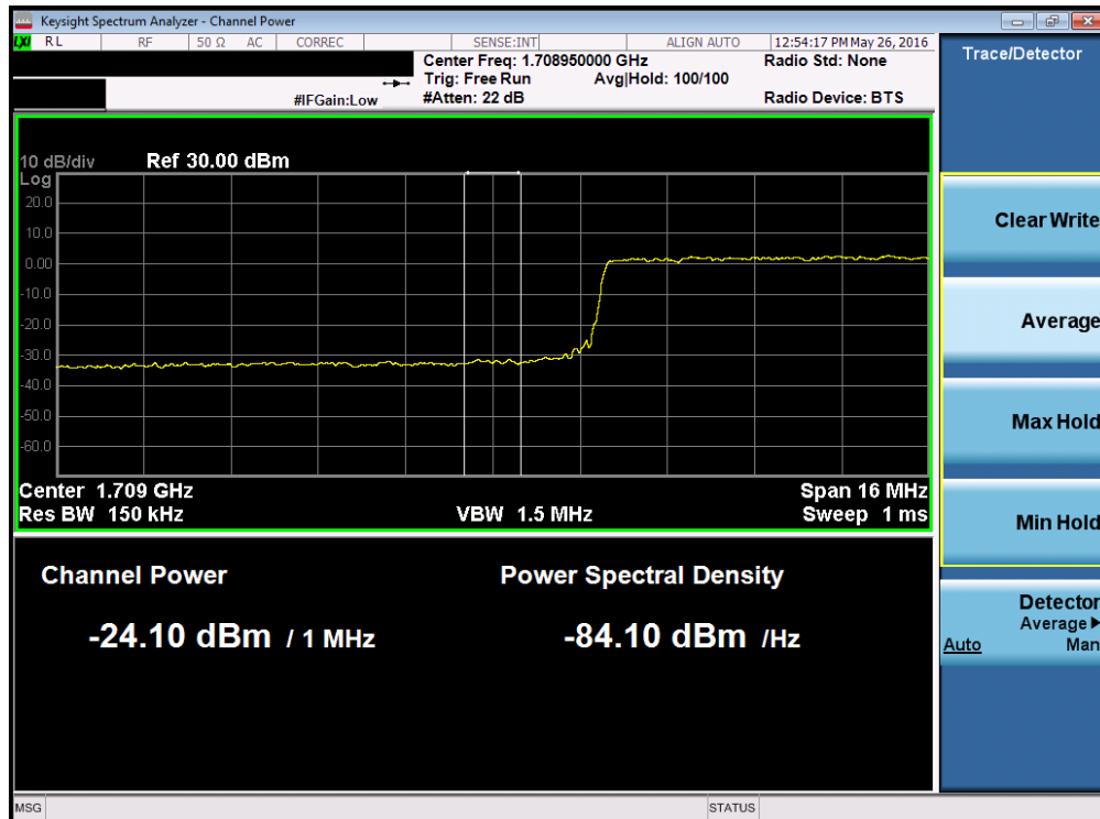
Plot 7-213. Lower Extended Band Edge Plot (Band 4 – 20.0MHz QPSK – RB Size 100)
