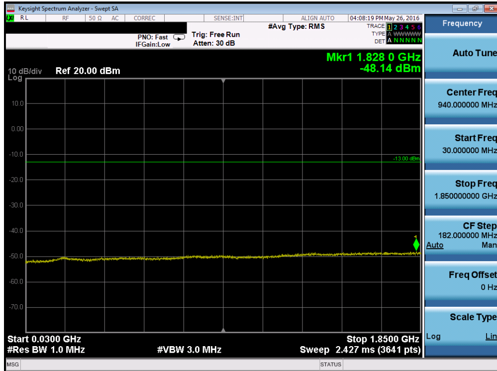
Plot 7-135. Conducted Spurious Plot (Band 2 – 10.0MHz QPSK – RB Size 1, RB Offset 0 – High Channel)
