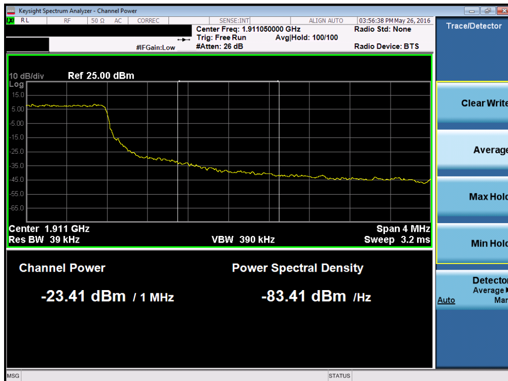
Plot 7-219. Upper Extended Band Edge Plot (Band 2 – 1.4MHz QPSK – RB Size 6)
