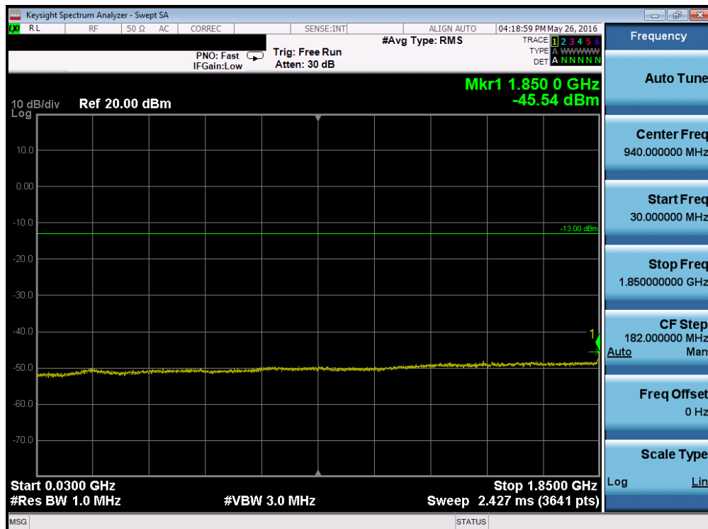
Plot 7-126. Conducted Spurious Plot (Band 2 – 3.0MHz QPSK – RB Size 1, RB Offset 0 – High Channel)
