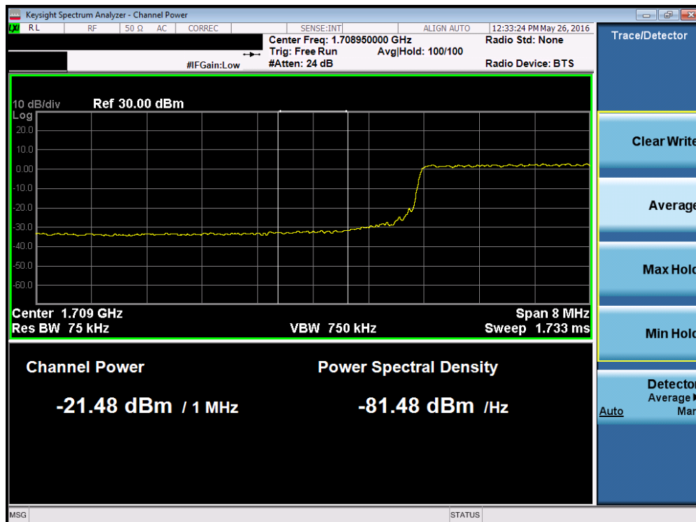
Plot 7-205. Lower Extended Band Edge Plot (Band 4 – 10.0MHz QPSK – RB Size 50)
