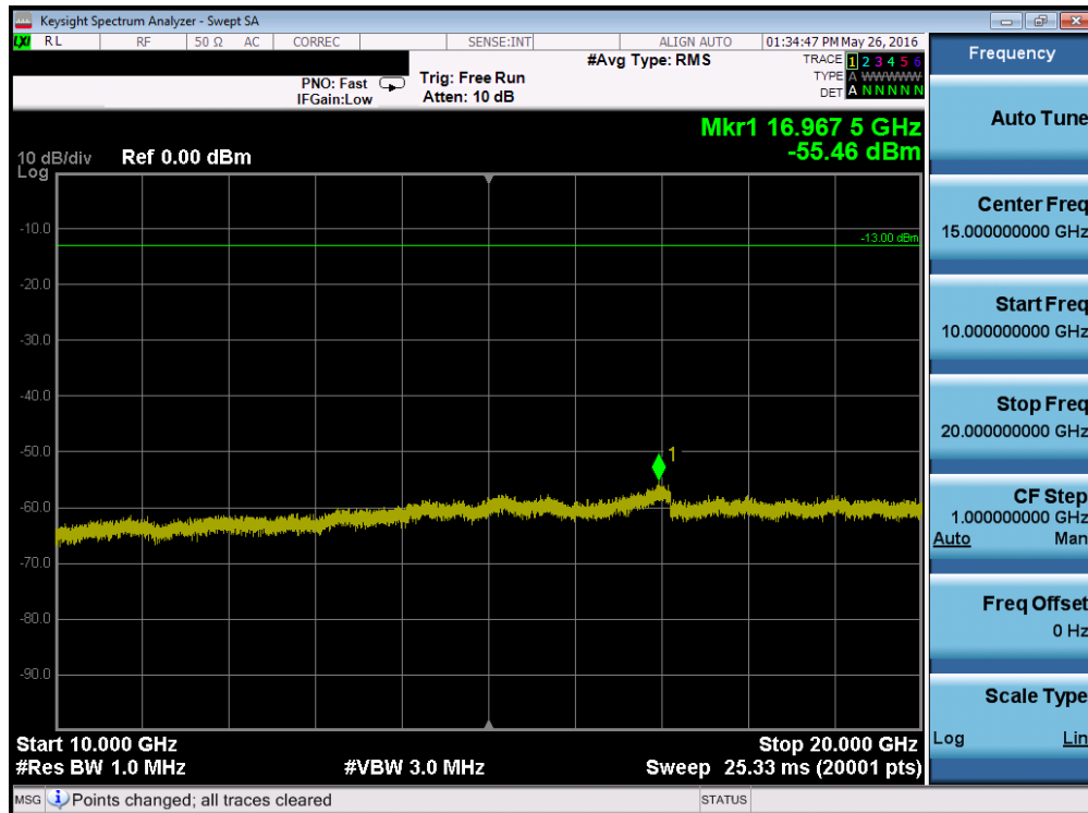
Plot 7-140. Conducted Spurious Plot (Band 25 – 3.0MHz QPSK – RB Size 1, RB Offset 0 – Low Channel)
