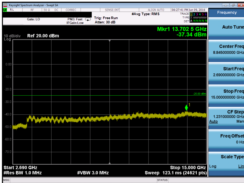
Plot 7-148. Conducted Spurious Plot (Band 41 – 5.0MHz QPSK – RB Size 1, RB Offset 0 – Low Channel)
