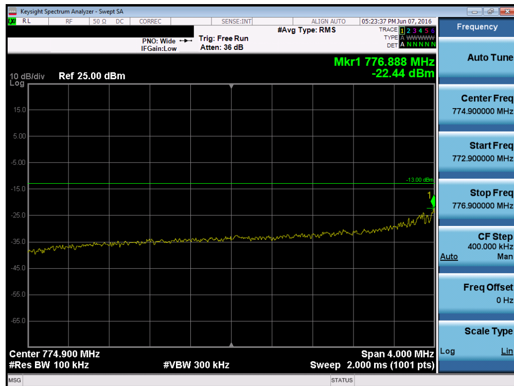
Plot 7-167. Lower Extended Band Edge Plot (Band 13 – 5.0MHz QPSK – RB Size 25)
