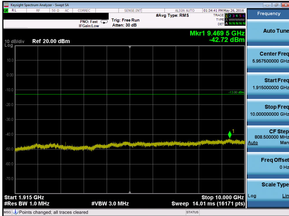
Plot 7-139. Conducted Spurious Plot (Band 25 – 3.0MHz QPSK – RB Size 1, RB Offset 0 – Low Channel)
