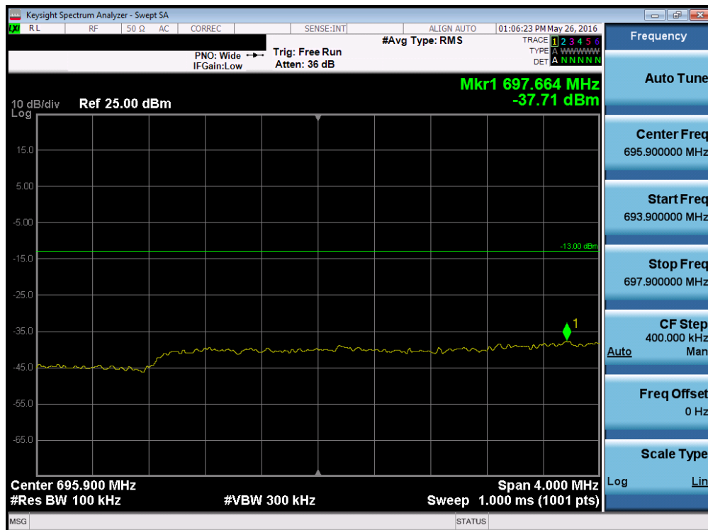
Plot 7-161. Lower Extended Band Edge Plot (Band 12/17 – 5.0MHz QPSK – RB Size 25)
