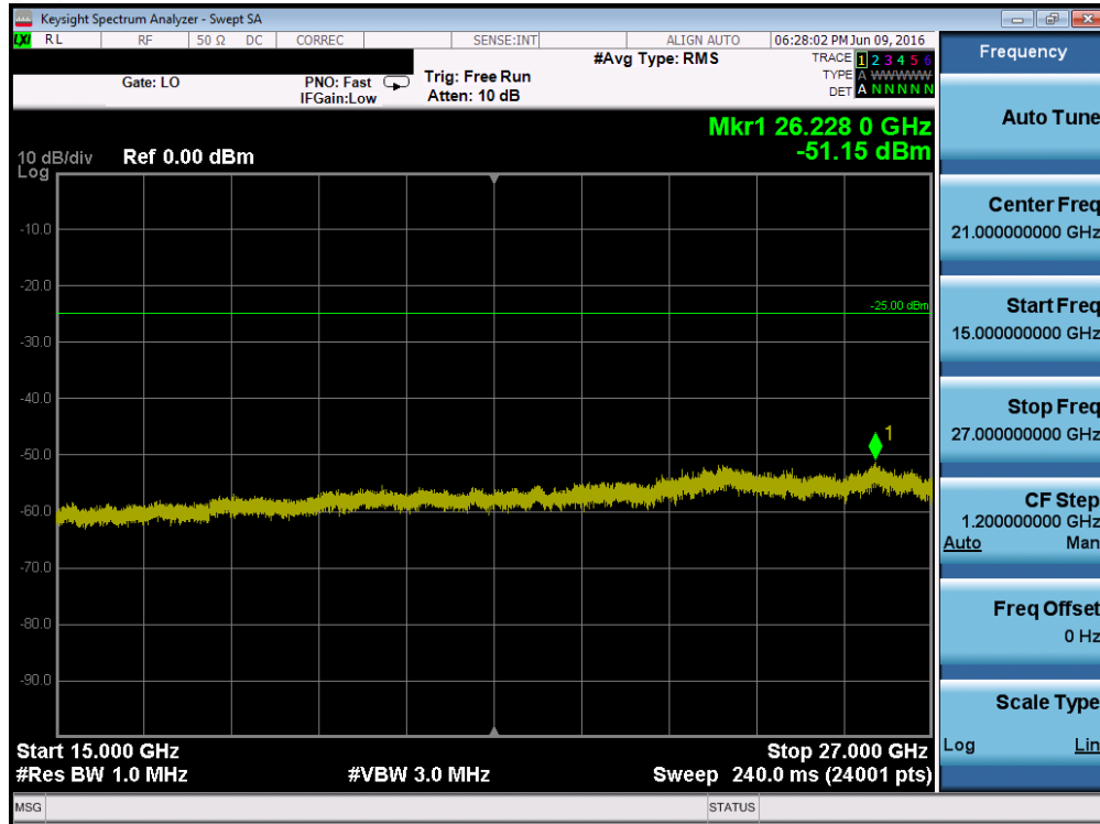
Plot 7-149. Conducted Spurious Plot (Band 41 – 5.0MHz QPSK – RB Size 1, RB Offset 0 – Low Channel)
