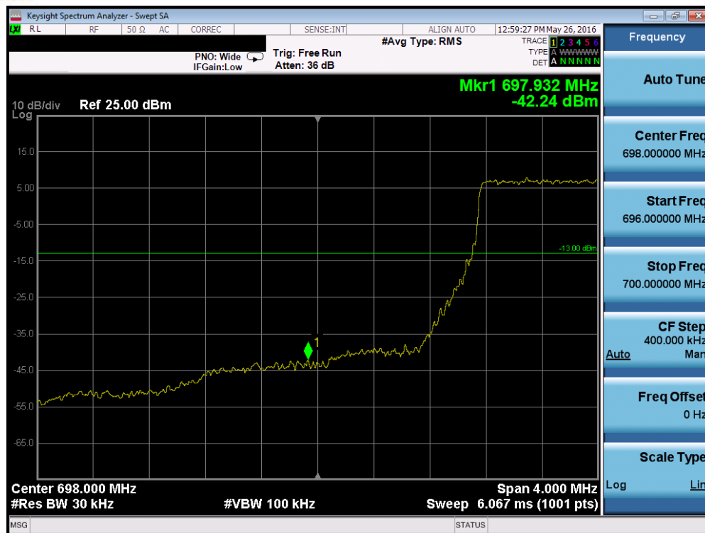
Plot 7-156. Lower Band Edge Plot (Band 12 – 1.4MHz QPSK – RB Size 6)
