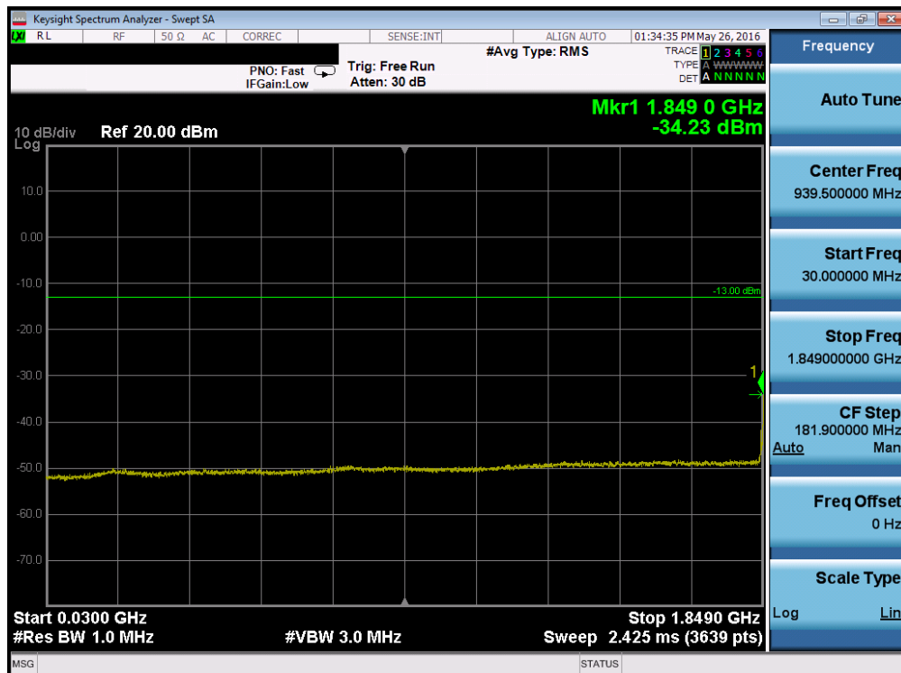
Plot 7-138. Conducted Spurious Plot (Band 25 – 3.0MHz QPSK – RB Size 1, RB Offset 0 – Low Channel)
