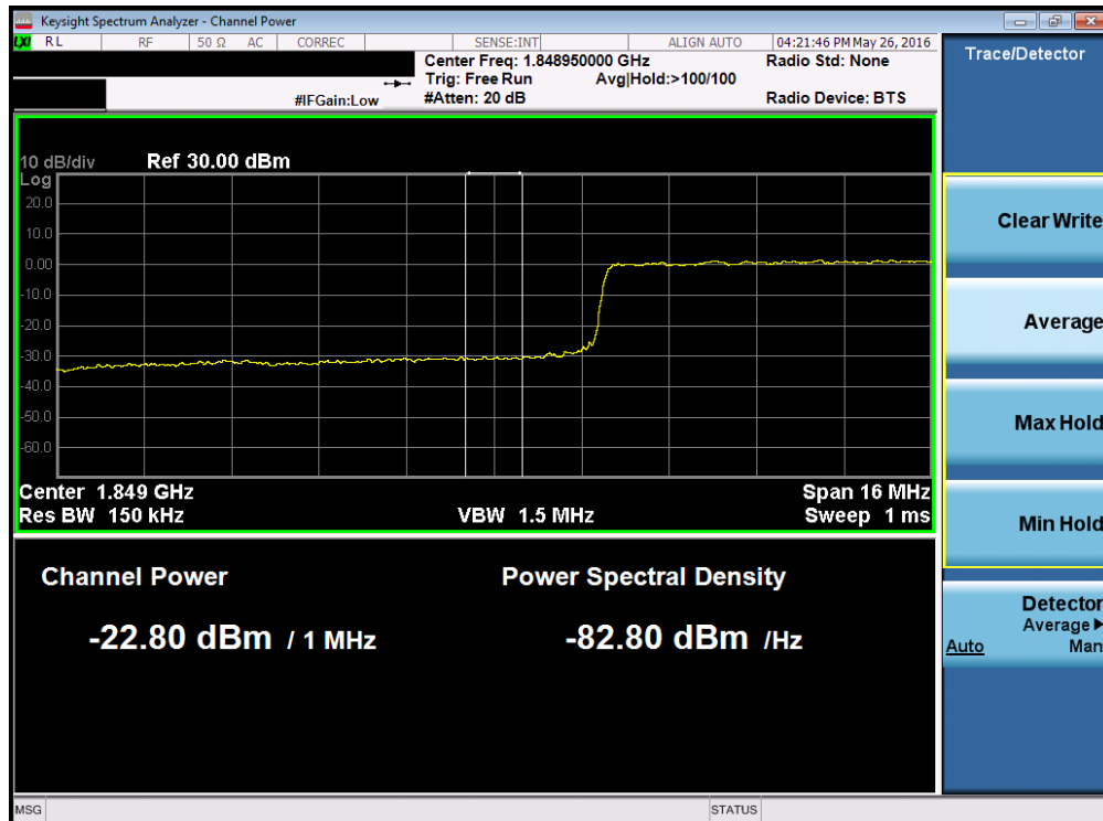
Plot 7-237. Lower Extended Band Edge Plot (Band 2 - 20.0MHz QPSK - RB Size 100)
