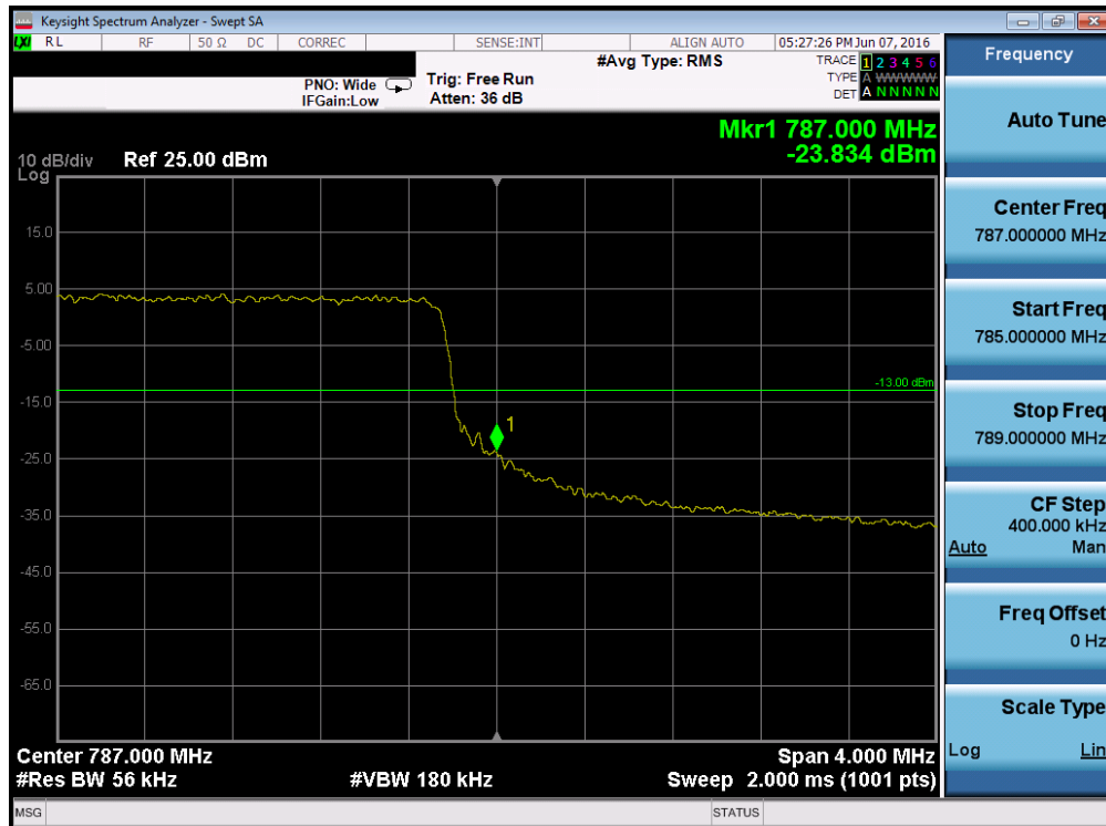
Plot 7-169. Upper Band Edge Plot (Band 13 - 5.0MHz QPSK - RB Size 25)
