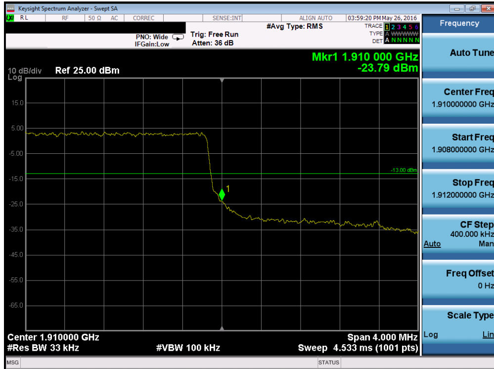
Plot 7-222. Upper Band Edge Plot (Band 2 – 3.0MHz QPSK – RB Size 15)
