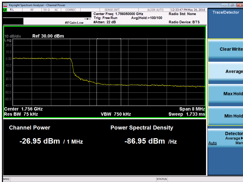
Plot 7-207. Upper Extended Band Edge Plot (Band 4 – 10.0MHz QPSK – RB Size 50)
