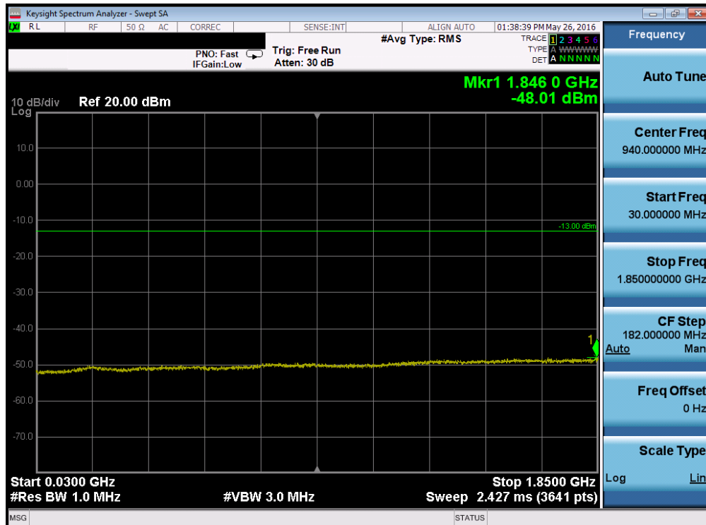
Plot 7-144. Conducted Spurious Plot (Band 25 – 3.0MHz QPSK – RB Size 1, RB Offset 0 – High Channel)
