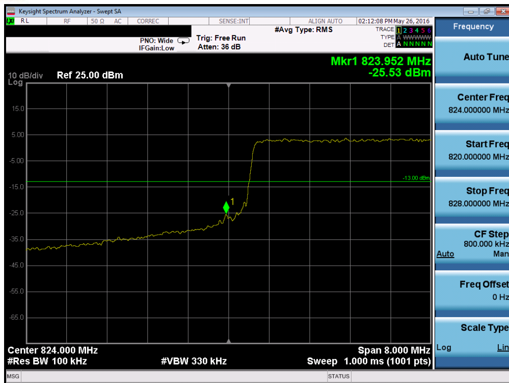
Plot 7-188. Lower Band Edge Plot (Band 26 – 10.0MHz QPSK – RB Size 50)
