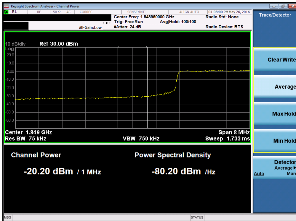
Plot 7-229. Lower Extended Band Edge Plot (Band 2 – 10.0MHz QPSK – RB Size 50)
