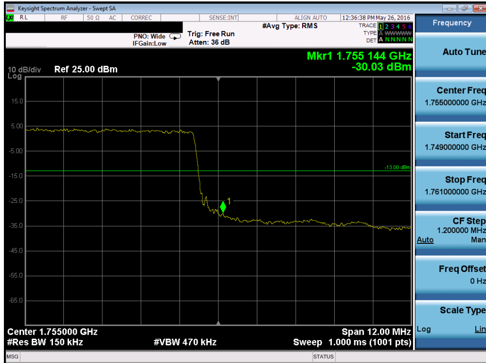
Plot 7-210. Upper Band Edge Plot (Band 4 – 15.0MHz QPSK – RB Size 75)
