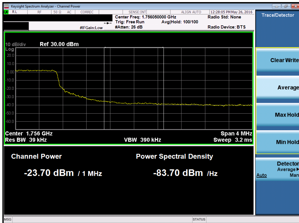
Plot 7-203. Upper Extended Band Edge Plot (Band 4 – 5.0MHz QPSK – RB Size 25)
