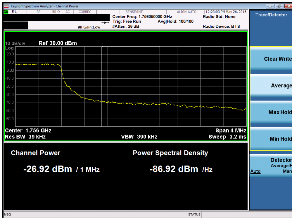
Plot 7-195. Upper Extended Band Edge Plot (Band 4 – 1.4MHz QPSK – RB Size 6)
