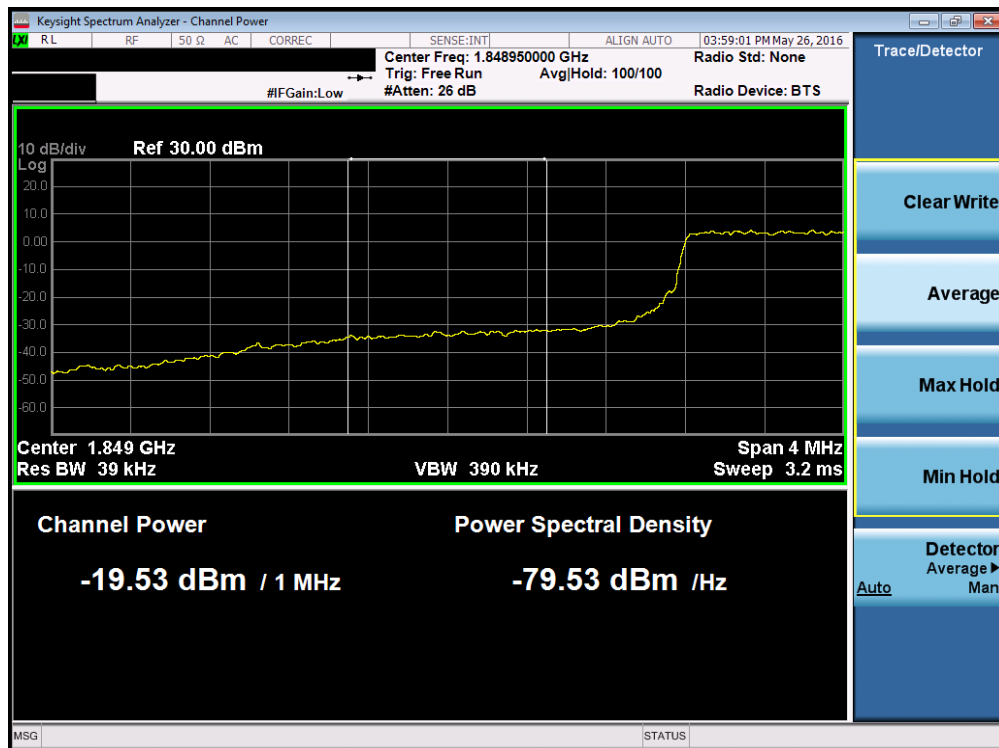
Plot 7-221. Lower Extended Band Edge Plot (Band 2 – 3.0MHz QPSK – RB Size 15)
