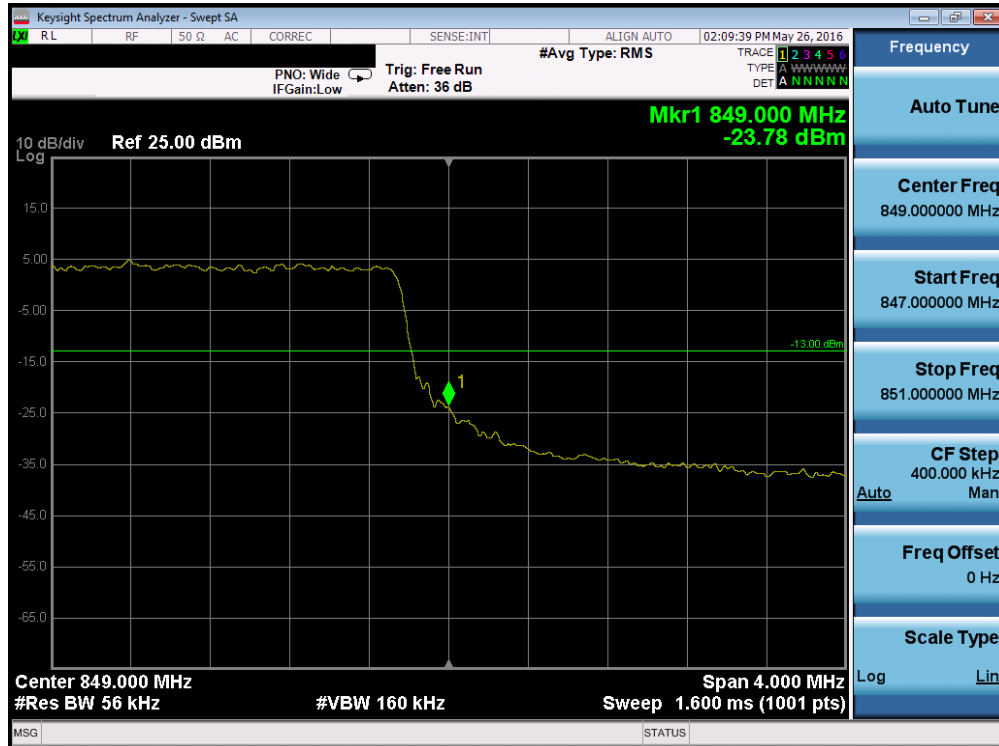
Plot 7-186. Upper Band Edge Plot (Band 26 – 5.0MHz QPSK – RB Size 25)
