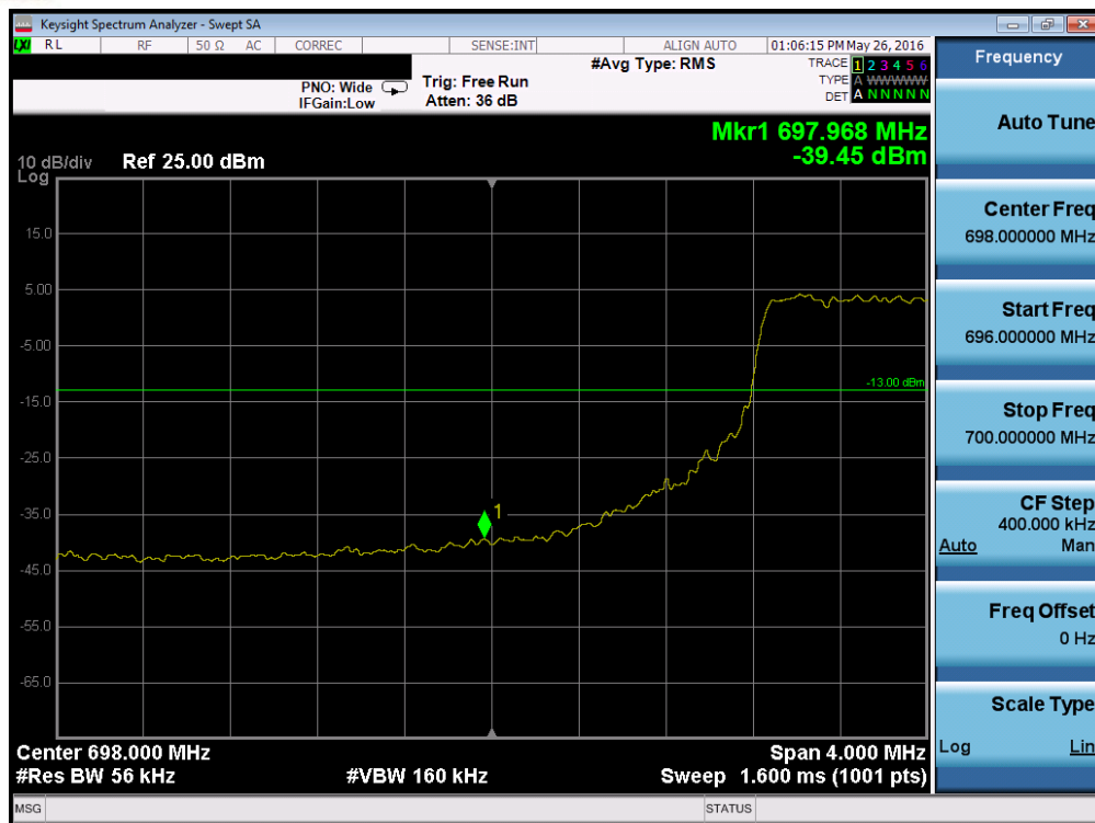
Plot 7-160. Lower Band Edge Plot (Band 12/17 – 5.0MHz QPSK – RB Size 25)
