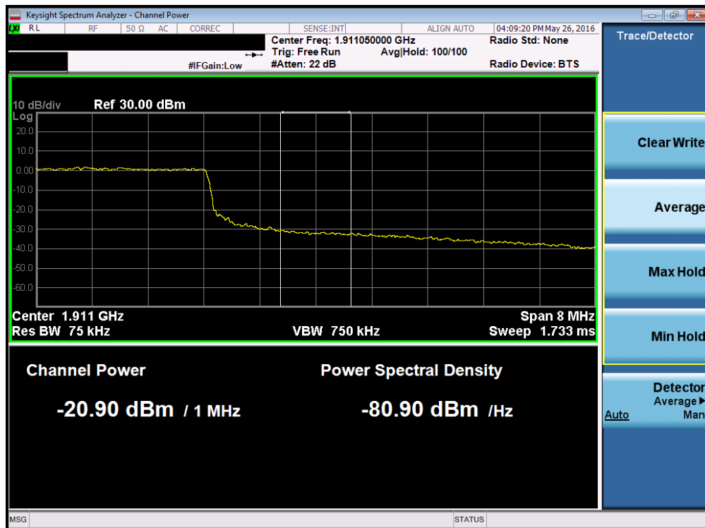
Plot 7-231. Upper Extended Band Edge Plot (Band 2 – 10.0MHz QPSK – RB Size 50)
