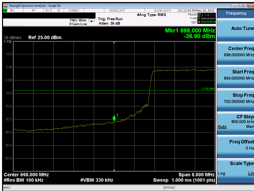
Plot 7-164. Lower Band Edge Plot (Band 12/17 - 10.0MHz QPSK - RB Size 50)
