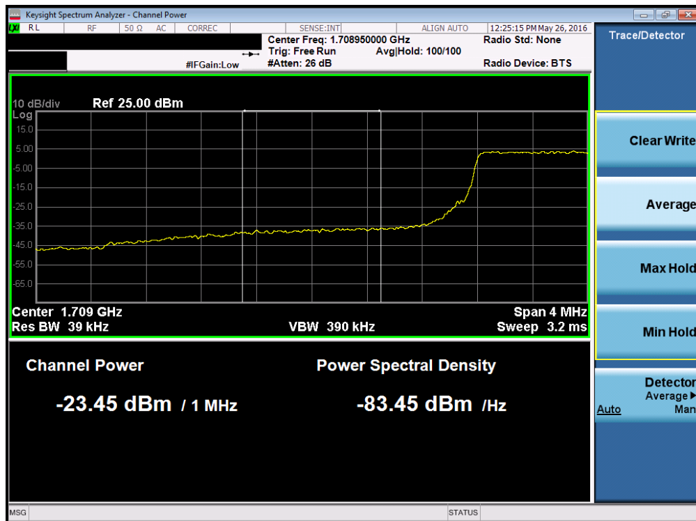
Plot 7-197. Lower Extended Band Edge Plot (Band 4 – 3.0MHz QPSK – RB Size 15)
