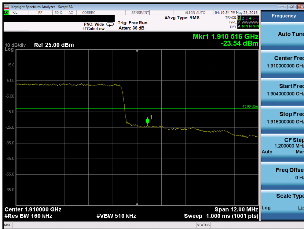
Plot 7-234. Upper Band Edge Plot (Band 2 – 15.0MHz QPSK – RB Size 75)
