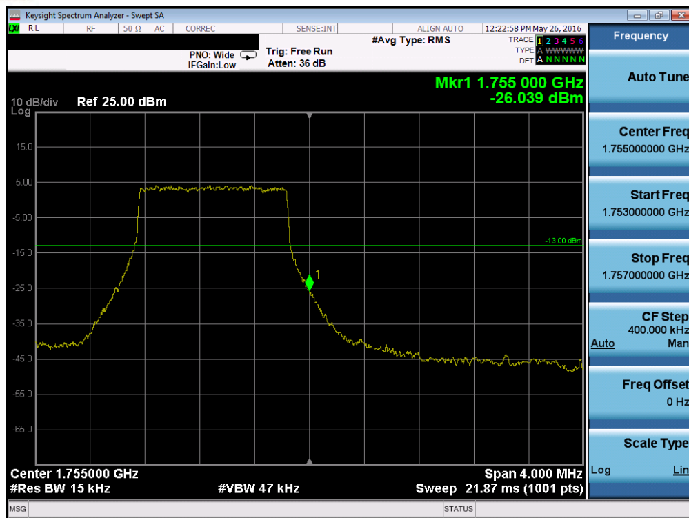
Plot 7-194. Upper Band Edge Plot (Band 4 – 1.4MHz QPSK – RB Size 6)
