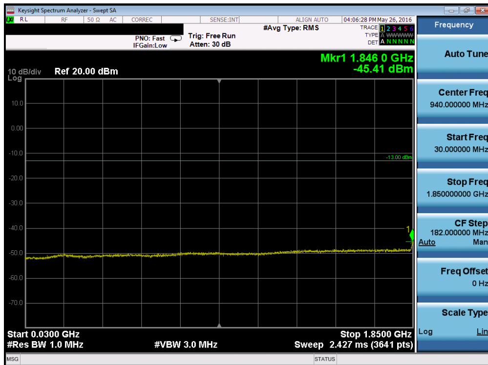
Plot 7-132. Conducted Spurious Plot (Band 2 – 10.0MHz QPSK – RB Size 1, RB Offset 0 – Mid Channel)
