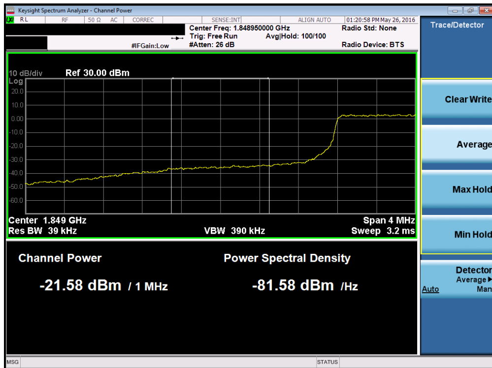
Plot 7-245. Lower Extended Band Edge Plot (Band 25 – 3.0MHz QPSK – RB Size 15)
