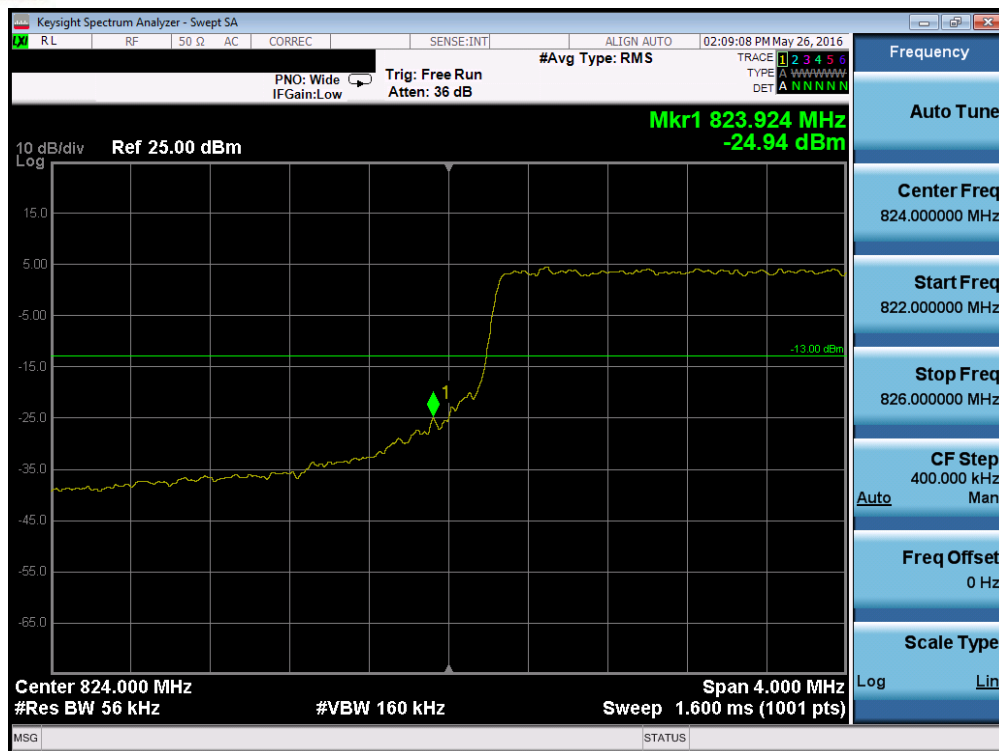
Plot 7-184. Lower Band Edge Plot (Band 26 - 5.0MHz QPSK - RB Size 25)
