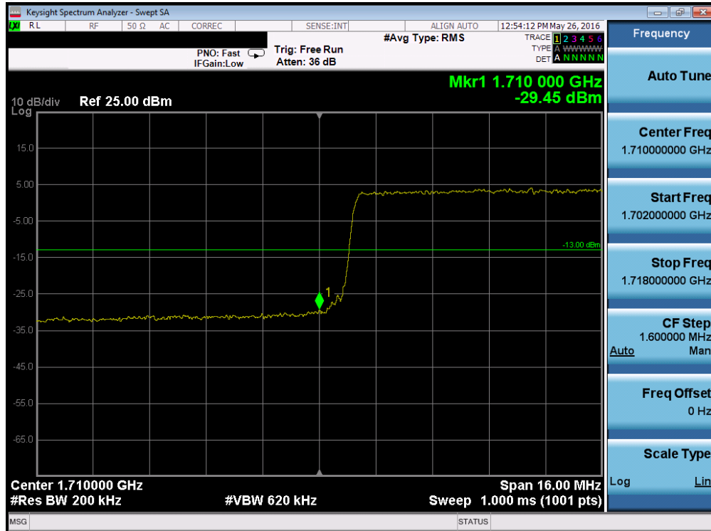
Plot 7-212. Lower Band Edge Plot (Band 4 – 20.0MHz QPSK – RB Size 100)
