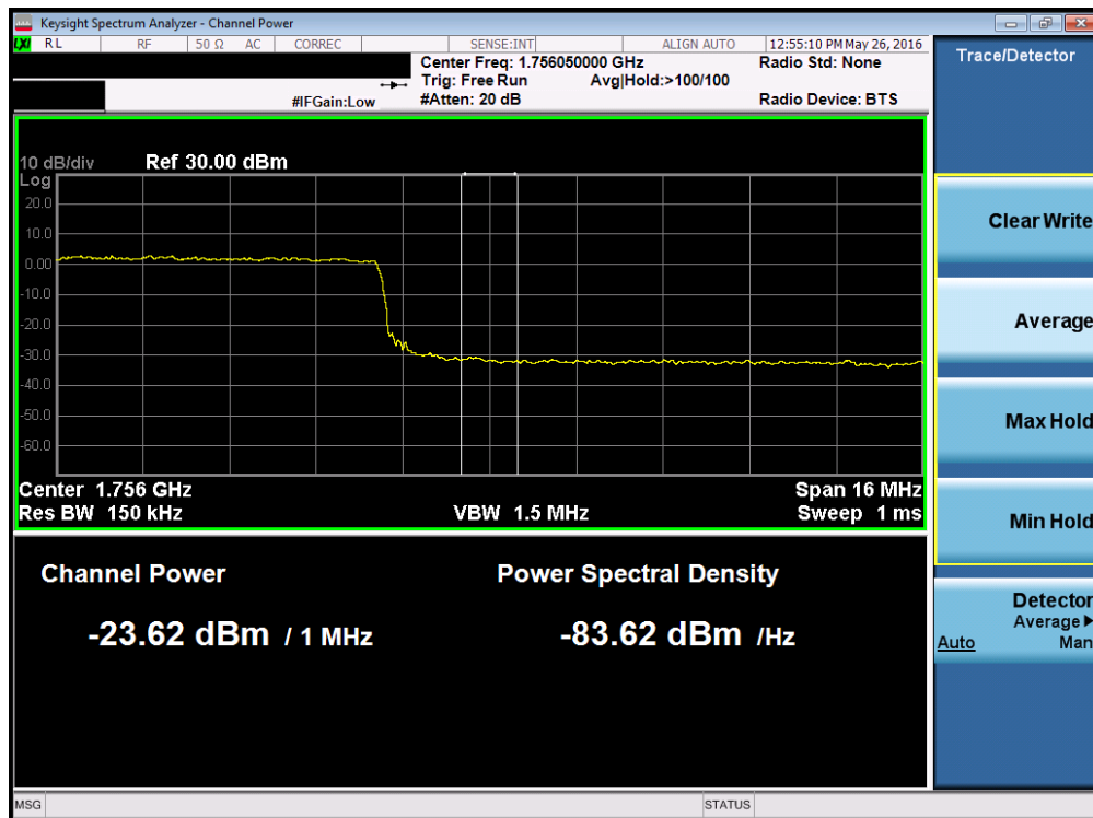
Plot 7-215. Upper Extended Band Edge Plot (Band 4 – 20.0MHz QPSK – RB Size 100)
