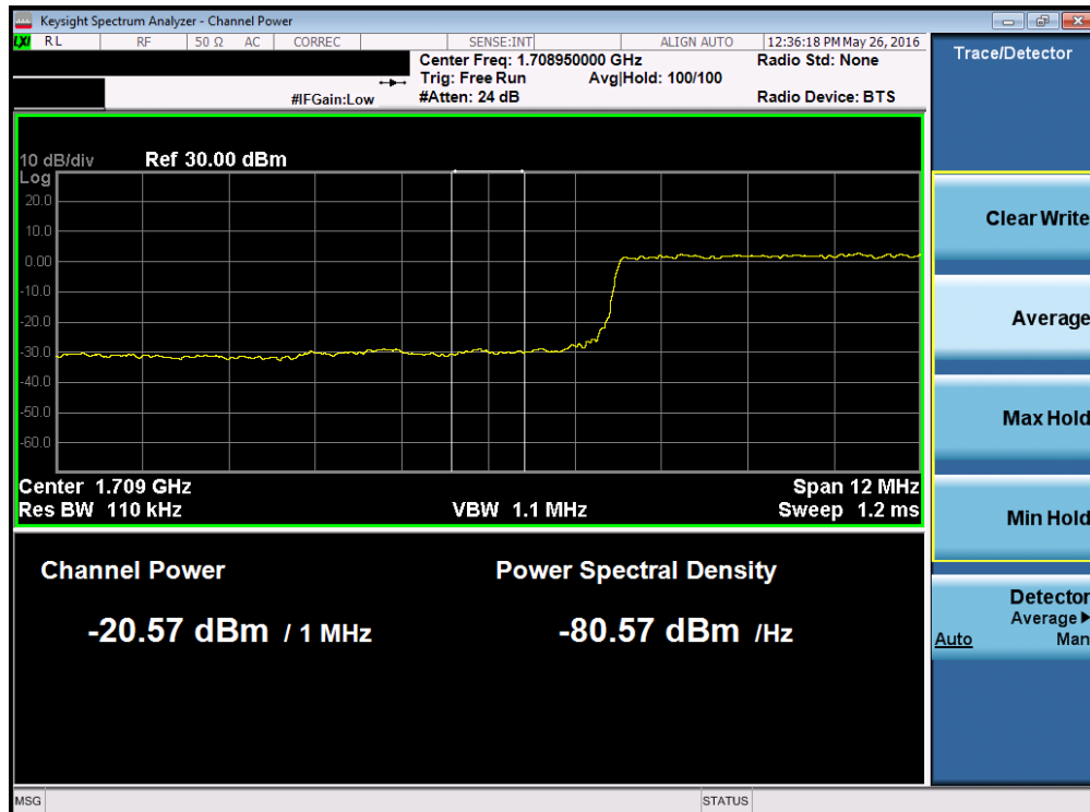
Plot 7-209. Lower Extended Band Edge Plot (Band 4 – 15.0MHz QPSK – RB Size 75)
