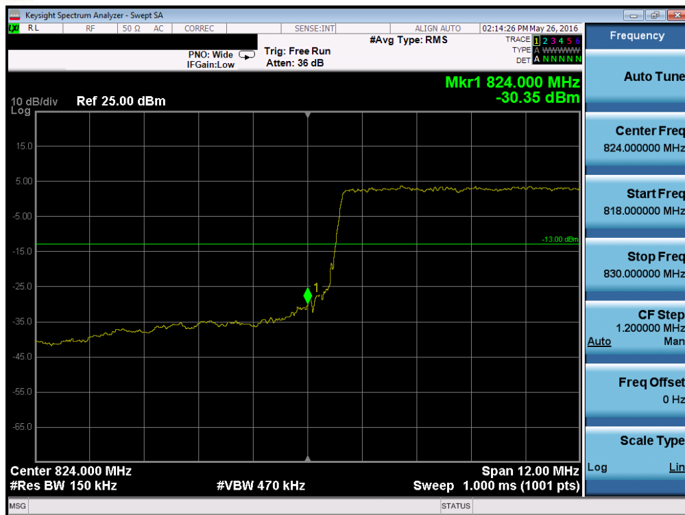
Plot 7-190. Lower Band Edge Plot (Band 26 – 15.0MHz QPSK – RB Size 75)
