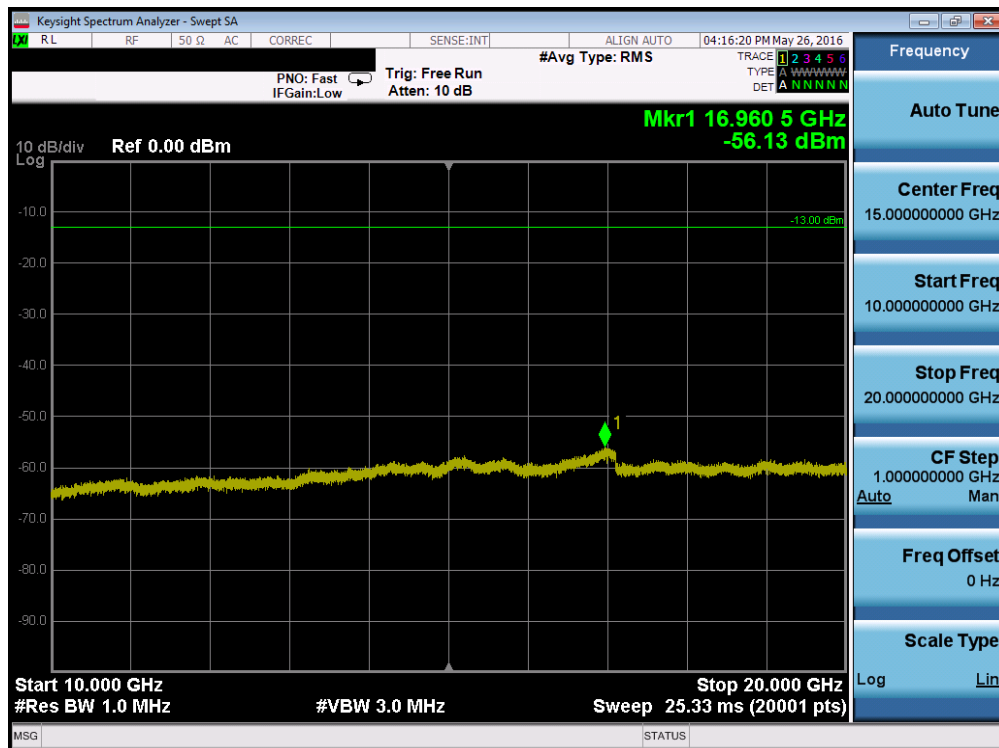
Plot 7-122. Conducted Spurious Plot (Band 2 – 3.0MHz QPSK – RB Size 1, RB Offset 0 – Low Channel)
