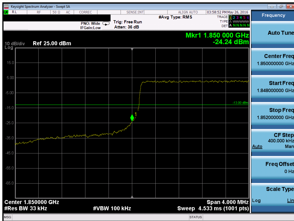
Plot 7-220. Lower Band Edge Plot (Band 2 – 3.0MHz QPSK – RB Size 15)
