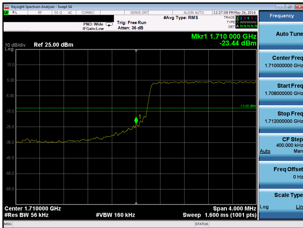
Plot 7-200. Lower Band Edge Plot (Band 4 – 5.0MHz QPSK – RB Size 25)
