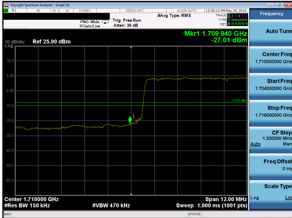
Plot 7-208. Lower Band Edge Plot (Band 4 – 15.0MHz QPSK – RB Size 75)
