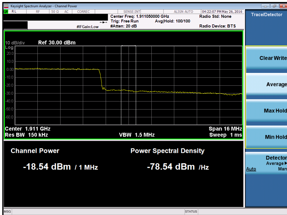
Plot 7-239. Upper Extended Band Edge Plot (Band 2 – 20.0MHz QPSK – RB Size 100)
