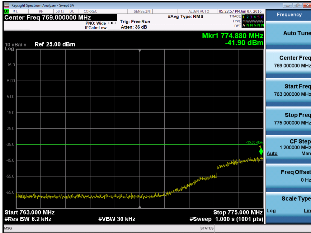
Plot 7-168. Lower Emission Mask Edge Plot (Band 13 - 5.0MHz QPSK - RB Size 25)
