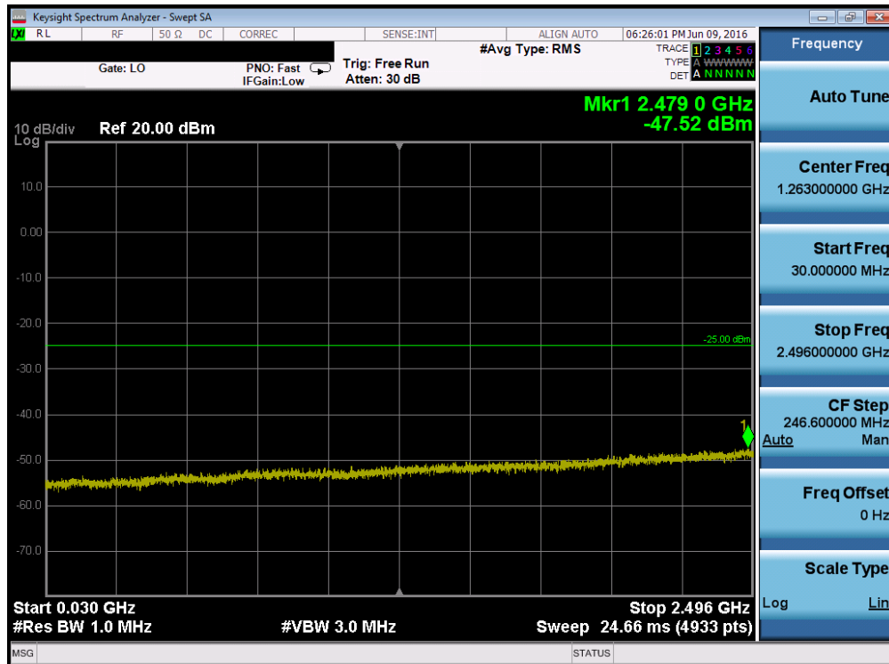
Plot 7-150. Conducted Spurious Plot (Band 41 – 5.0MHz QPSK – RB Size 1, RB Offset 0 – Mid Channel)
