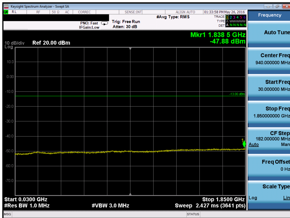
Plot 7-141. Conducted Spurious Plot (Band 25 – 3.0MHz QPSK – RB Size 1, RB Offset 0 – Mid Channel)
