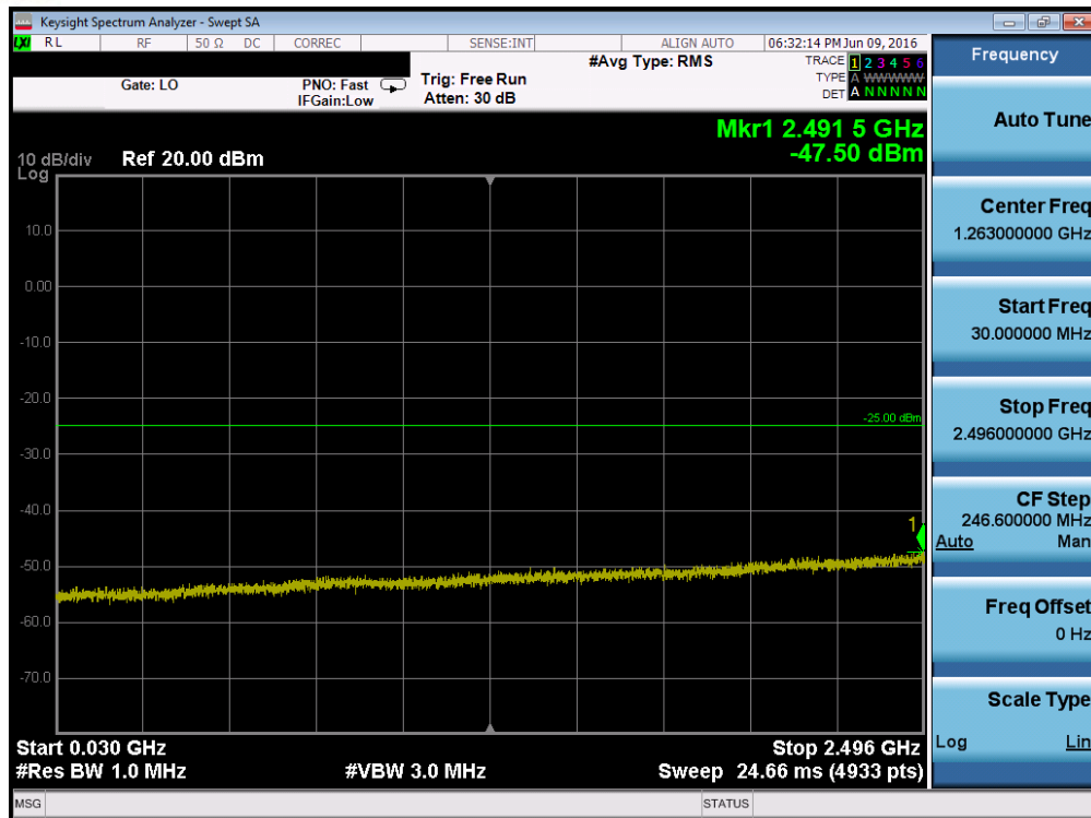
Plot 7-153. Conducted Spurious Plot (Band 41 – 5.0MHz QPSK – RB Size 1, RB Offset 0 – High Channel)
