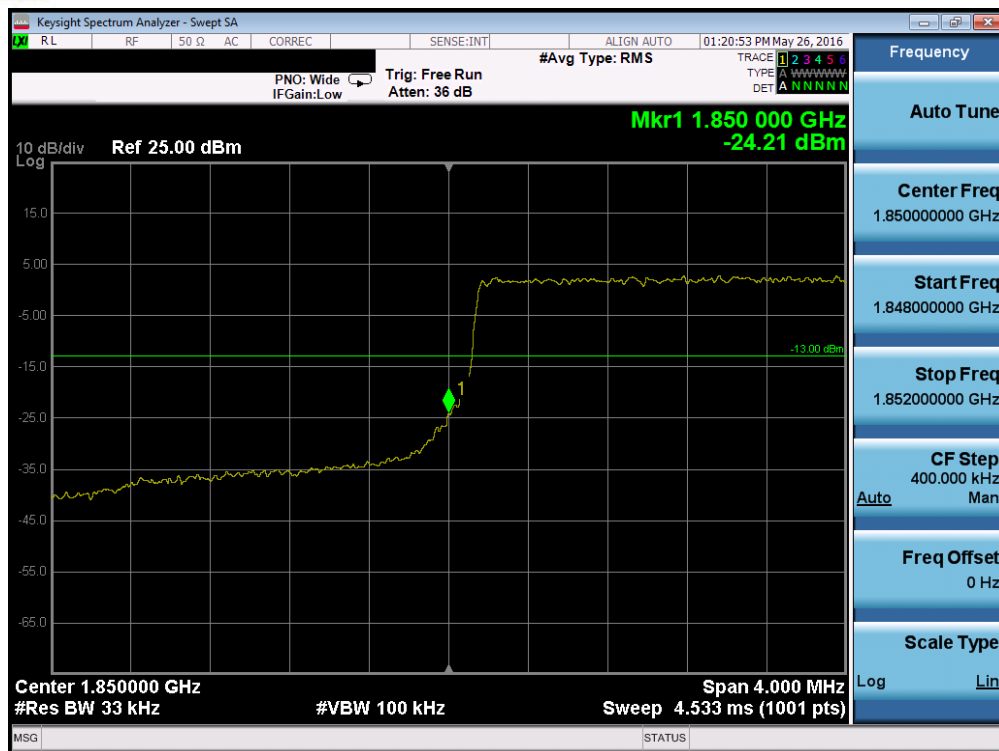
Plot 7-244. Lower Band Edge Plot (Band 25 – 3.0MHz QPSK – RB Size 15)
