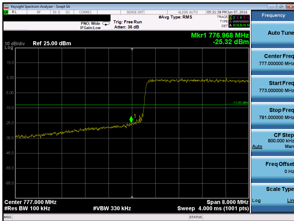
Plot 7-172. Lower Band Edge Plot (Band 13 – 10.0MHz QPSK – RB Size 50)
