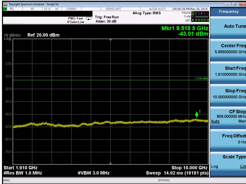
Plot 7-133. Conducted Spurious Plot (Band 2 – 10.0MHz QPSK – RB Size 1, RB Offset 0 – Mid Channel)
