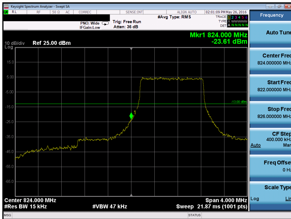
Plot 7-176. Lower Band Edge Plot (Band 26 – 1.4MHz QPSK – RB Size 6)
