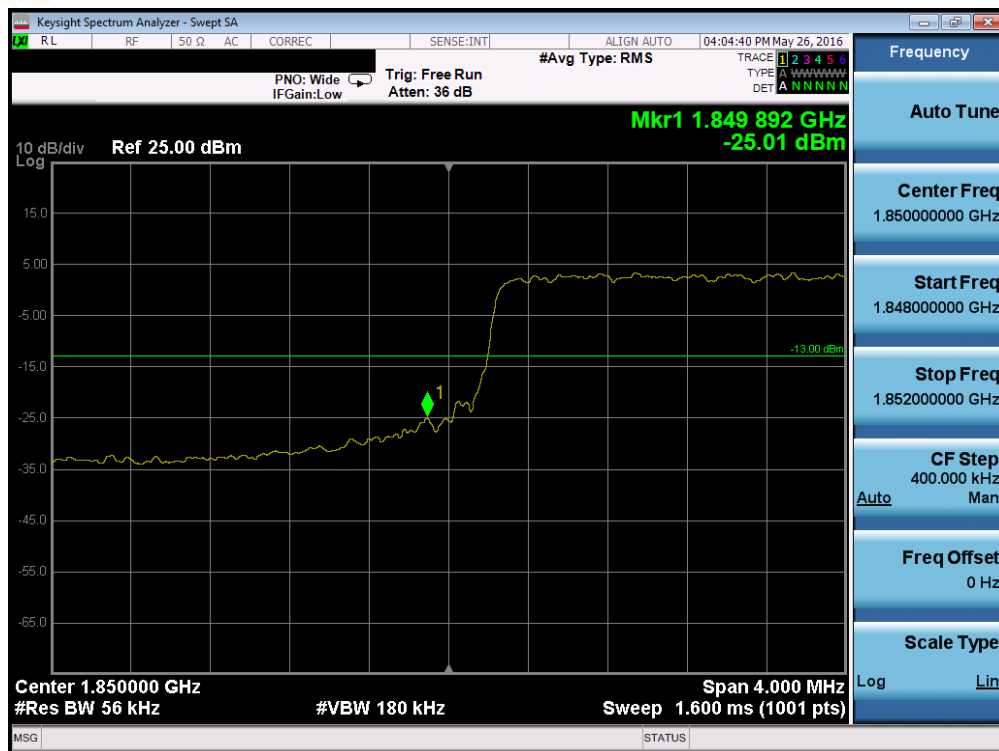
Plot 7-224. Lower Band Edge Plot (Band 2 – 5.0MHz QPSK – RB Size 25)
