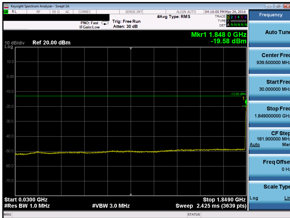
Plot 7-120. Conducted Spurious Plot (Band 2 – 3.0MHz QPSK – RB Size 1, RB Offset 0 – Low Channel)
