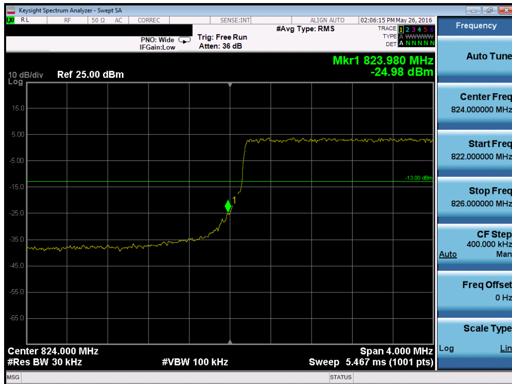
Plot 7-180. Lower Band Edge Plot (Band 26 – 3.0MHz QPSK – RB Size 15)
