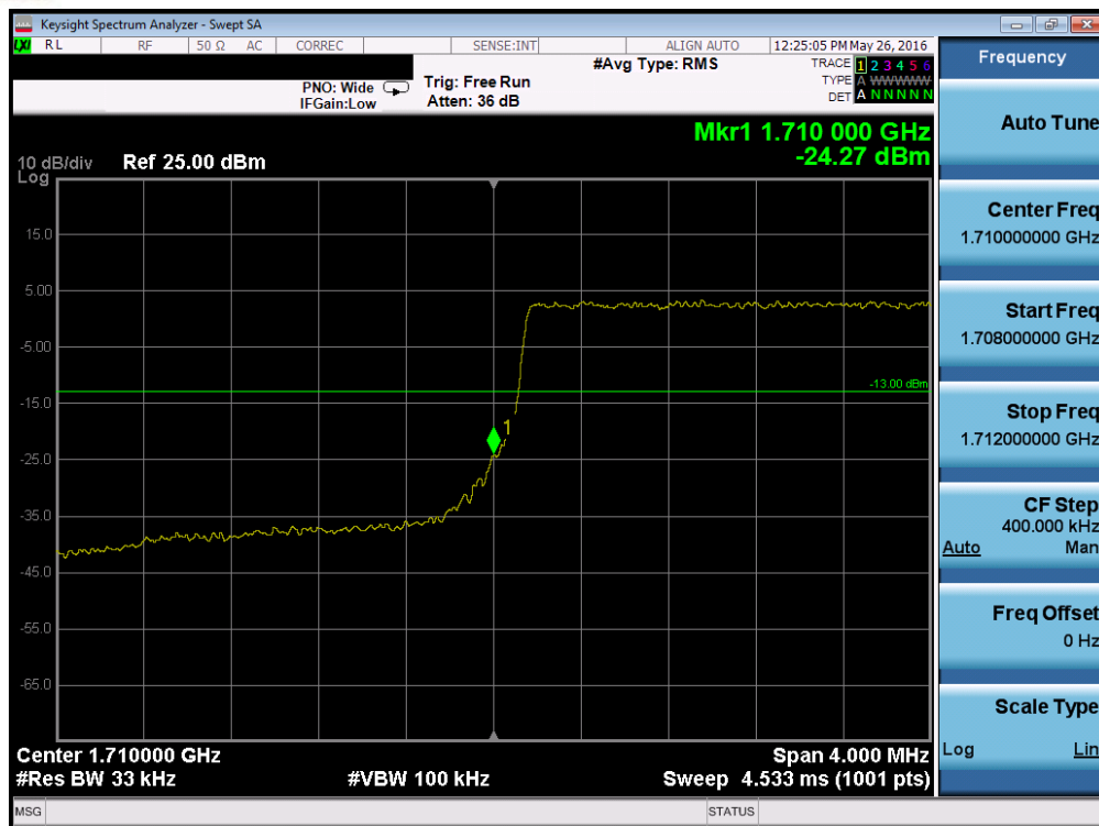
Plot 7-196. Lower Band Edge Plot (Band 4 – 3.0MHz QPSK – RB Size 15)
