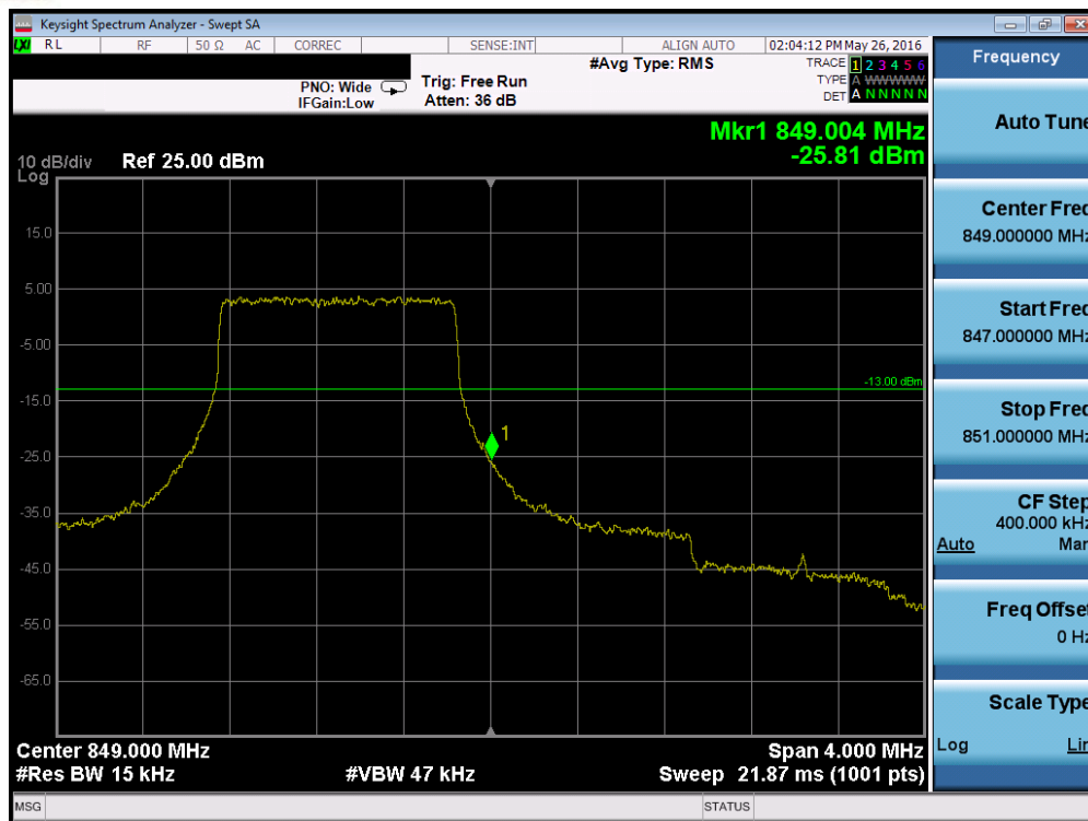
Plot 7-178. Upper Band Edge Plot (Band 26 – 1.4MHz QPSK – RB Size 6)
