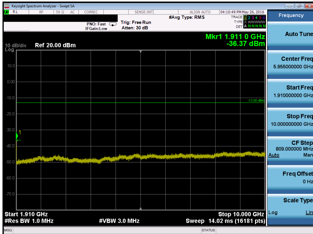
Plot 7-124. Conducted Spurious Plot (Band 2 – 3.0MHz QPSK – RB Size 1, RB Offset 0 – Mid Channel)
