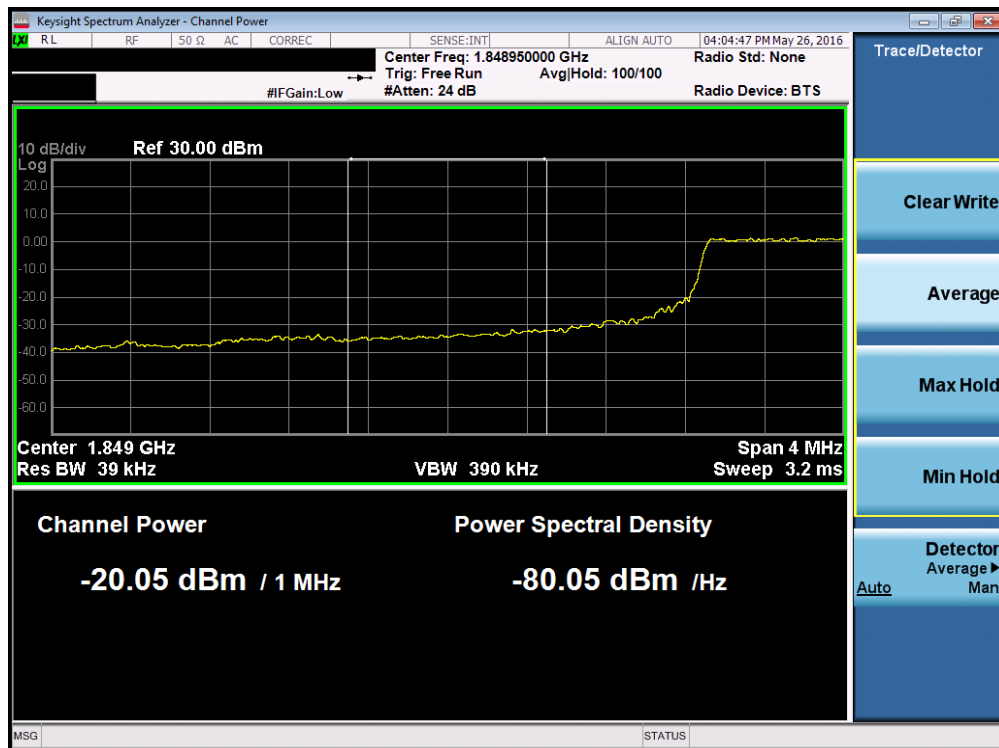
Plot 7-225. Lower Extended Band Edge Plot (Band 2 – 5.0MHz QPSK – RB Size 25)
