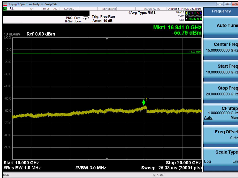
Plot 7-125. Conducted Spurious Plot (Band 2 – 3.0MHz QPSK – RB Size 1, RB Offset 0 – Mid Channel)
