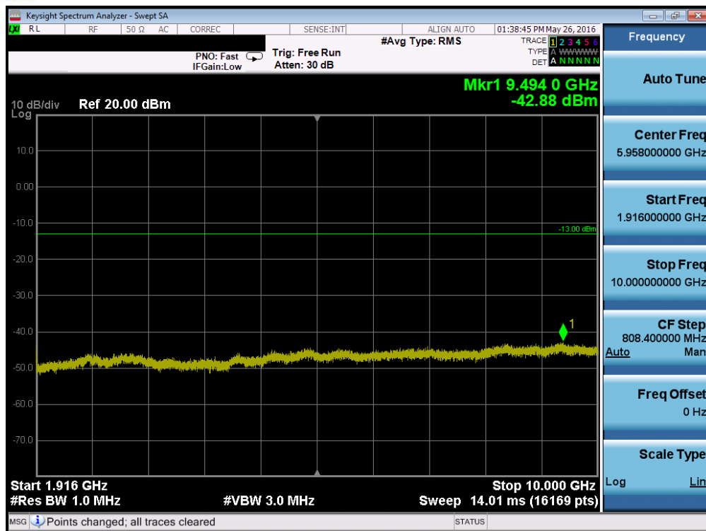
Plot 7-145. Conducted Spurious Plot (Band 25 – 3.0MHz QPSK – RB Size 1, RB Offset 0 – High Channel)
