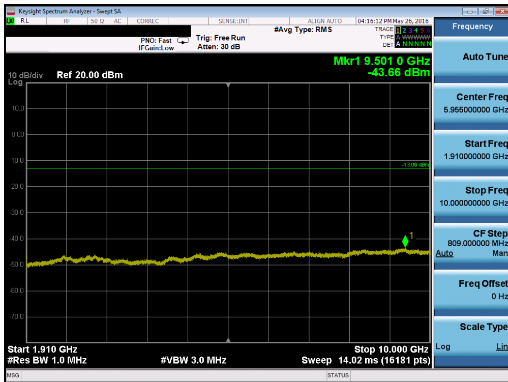
Plot 7-121. Conducted Spurious Plot (Band 2 – 3.0MHz QPSK – RB Size 1, RB Offset 0 – Low Channel)
