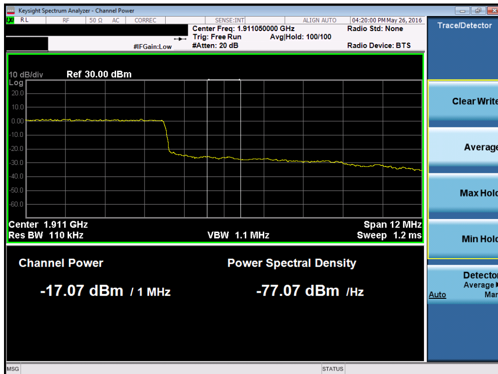
Plot 7-235. Upper Extended Band Edge Plot (Band 2 – 15.0MHz QPSK – RB Size 75)
