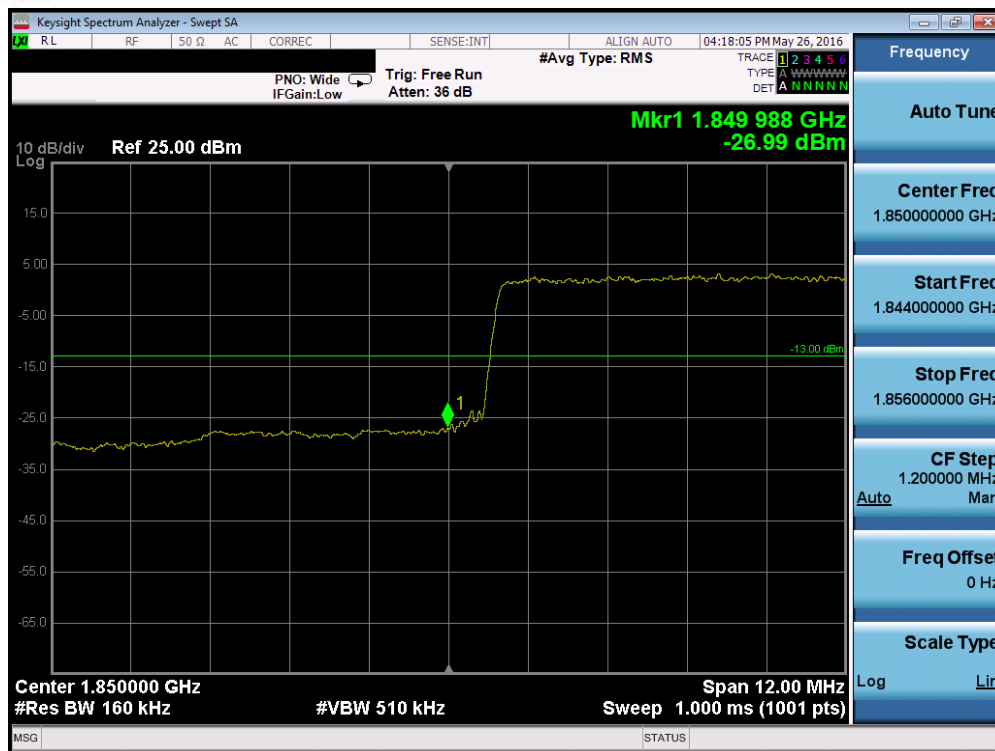
Plot 7-232. Lower Band Edge Plot (Band 2 – 15.0MHz QPSK – RB Size 75)
