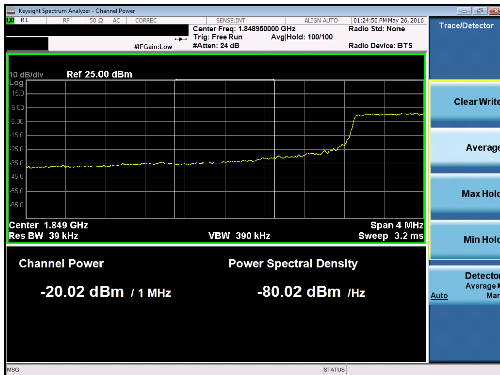
Plot 7-249. Lower Extended Band Edge Plot (Band 25 – 5.0MHz QPSK – RB Size 25)
