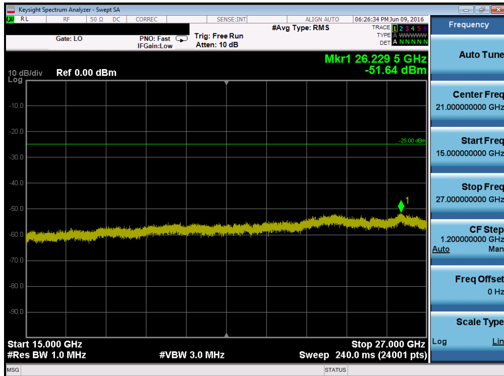
Plot 7-152. Conducted Spurious Plot (Band 41 – 5.0MHz QPSK – RB Size 1, RB Offset 0 – Mid Channel)
