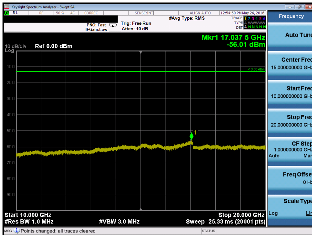
Plot 7-119. Conducted Spurious Plot (Band 4 – 3.0MHz QPSK – RB Size 1, RB Offset 0 – High Channel)
