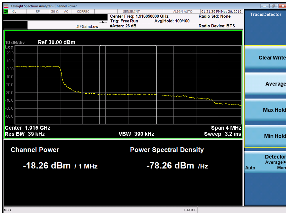
Plot 7-247. Upper Extended Band Edge Plot (Band 25 – 3.0MHz QPSK – RB Size 15)
