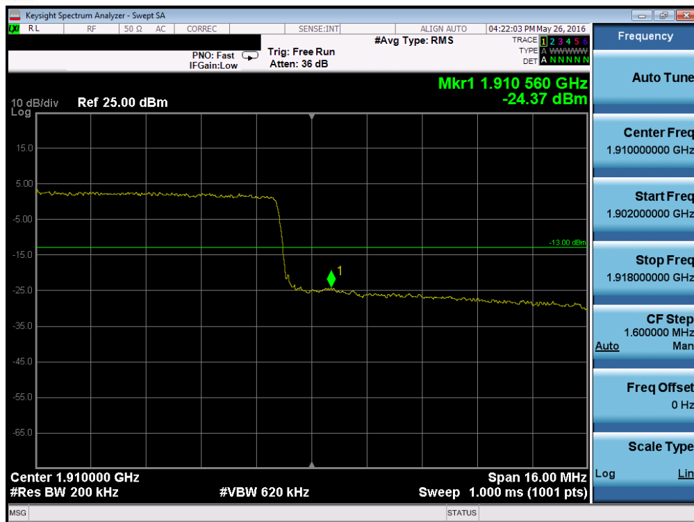
Plot 7-238. Upper Band Edge Plot (Band 2 – 20.0MHz QPSK – RB Size 100)
