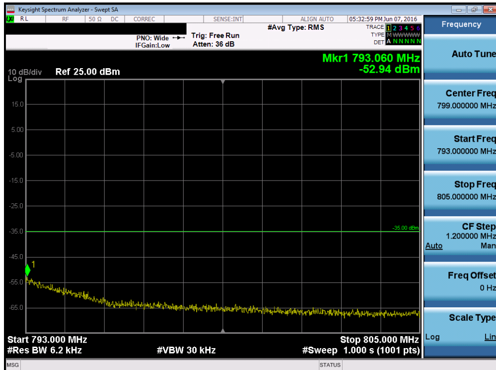
Plot 7-175. Upper Emission Mask Edge Plot (Band 13 – 10.0MHz QPSK – RB Size 50)
