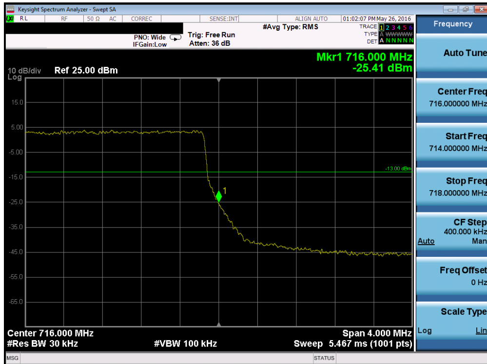
Plot 7-159. Upper Band Edge Plot (Band 12 – 3.0MHz QPSK – RB Size 15)
