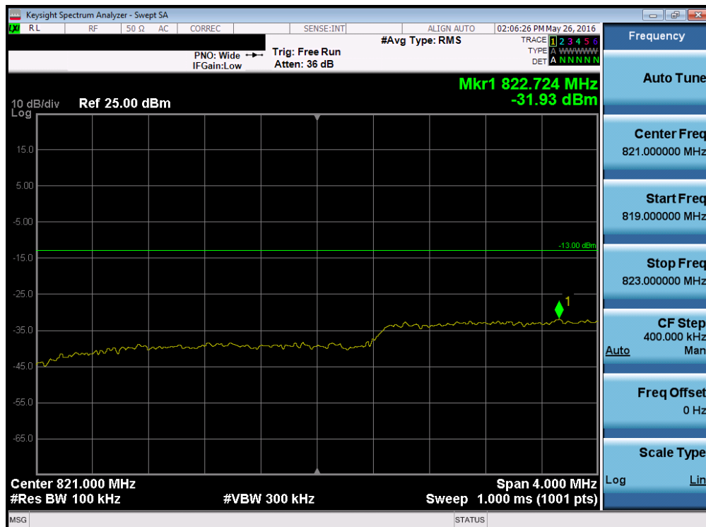
Plot 7-181. Lower Extended Band Edge Plot (Band 26 – 3.0MHz QPSK – RB Size 15)
