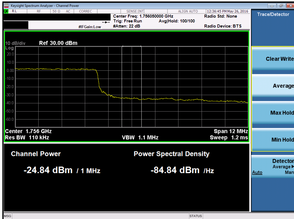
Plot 7-211. Upper Extended Band Edge Plot (Band 4 – 15.0MHz QPSK – RB Size 75)
