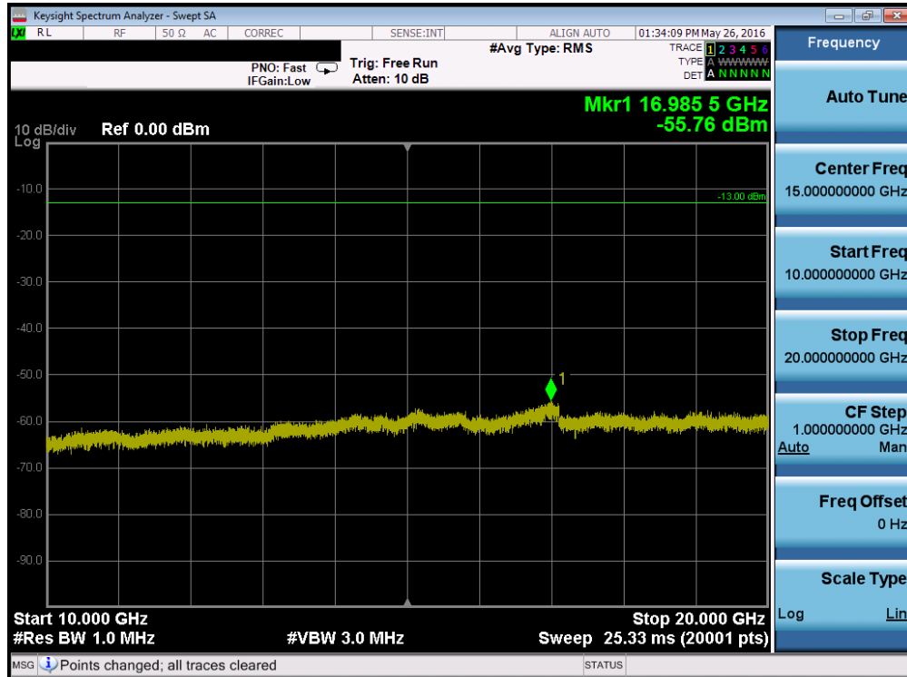
Plot 7-143. Conducted Spurious Plot (Band 25 – 3.0MHz QPSK – RB Size 1, RB Offset 0 – Mid Channel)
