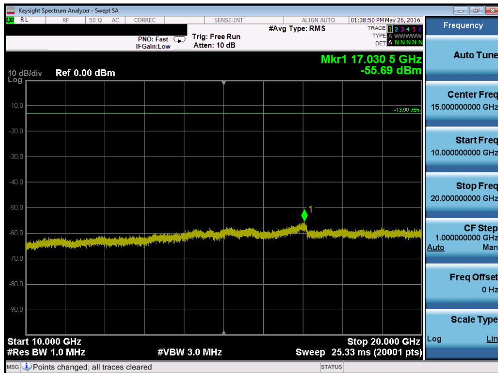
Plot 7-146. Conducted Spurious Plot (Band 25 – 3.0MHz QPSK – RB Size 1, RB Offset 0 – High Channel)
