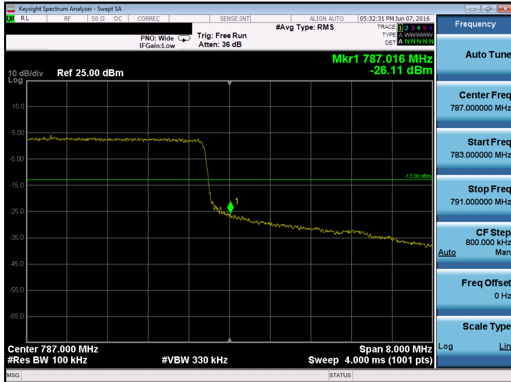
Plot 7-174. Upper Band Edge Plot (Band 13 – 10.0MHz QPSK – RB Size 50)
