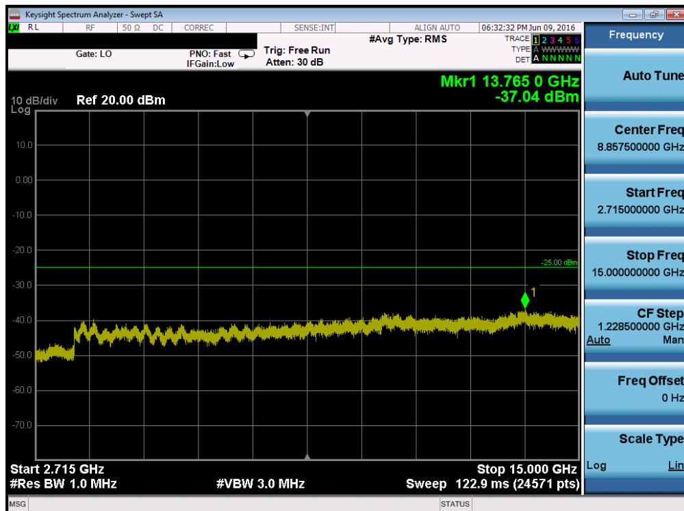
Plot 7-154. Conducted Spurious Plot (Band 41 – 5.0MHz QPSK – RB Size 1, RB Offset 0 – High Channel)
