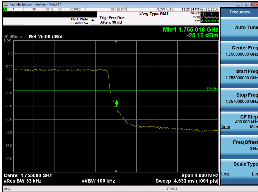
Plot 7-198. Upper Band Edge Plot (Band 4 – 3.0MHz QPSK – RB Size 15)
