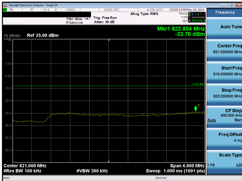
Plot 7-185. Lower Extended Band Edge Plot (Band 26 - 5.0MHz QPSK - RB Size 25)
