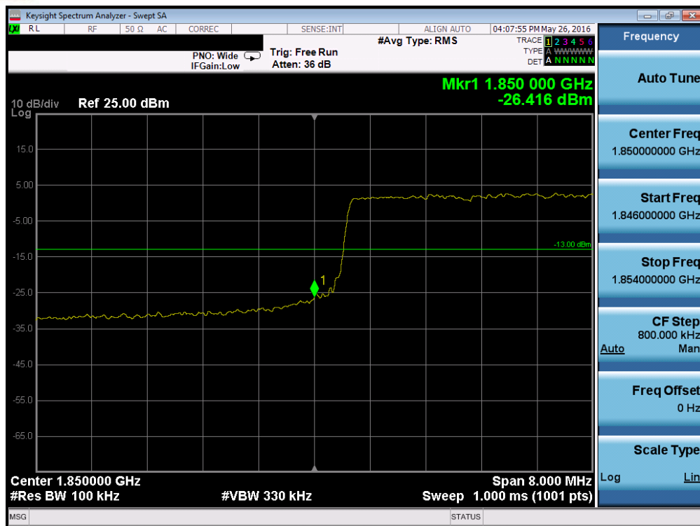
Plot 7-228. Lower Band Edge Plot (Band 2 – 10.0MHz QPSK – RB Size 50)
