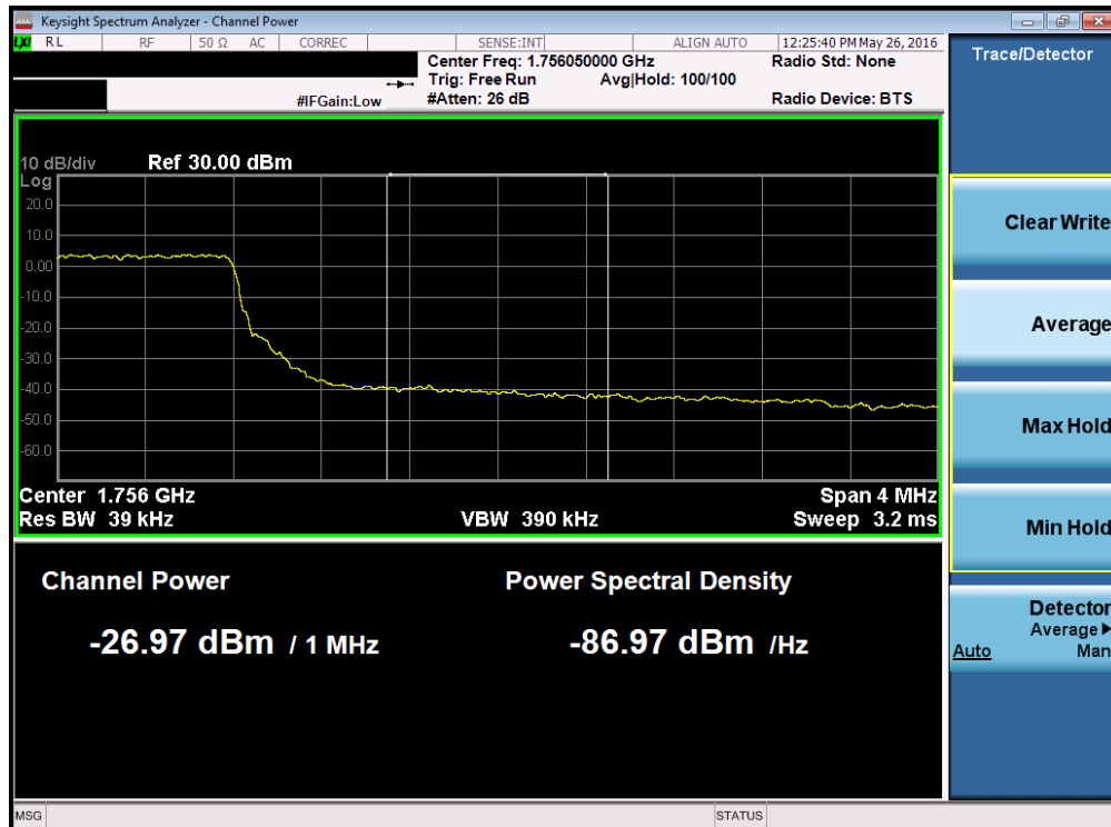
Plot 7-199. Upper Extended Band Edge Plot (Band 4 – 3.0MHz QPSK – RB Size 15)
