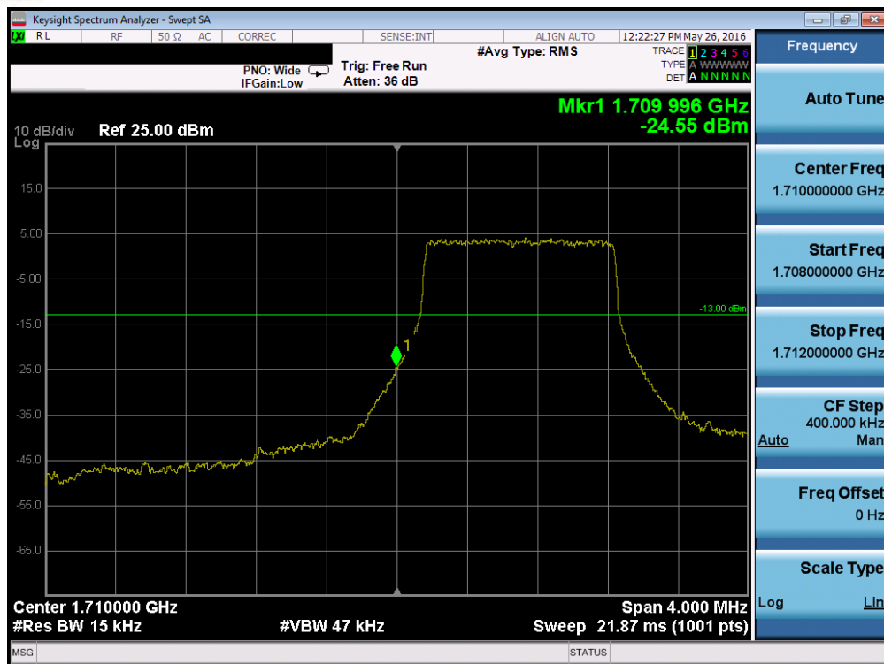
Plot 7-192. Lower Band Edge Plot (Band 4 – 1.4MHz QPSK – RB Size 6)
