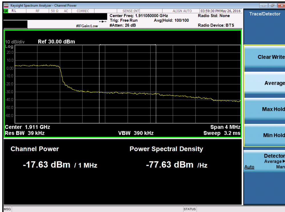
Plot 7-223. Upper Extended Band Edge Plot (Band 2 – 3.0MHz QPSK – RB Size 15)
