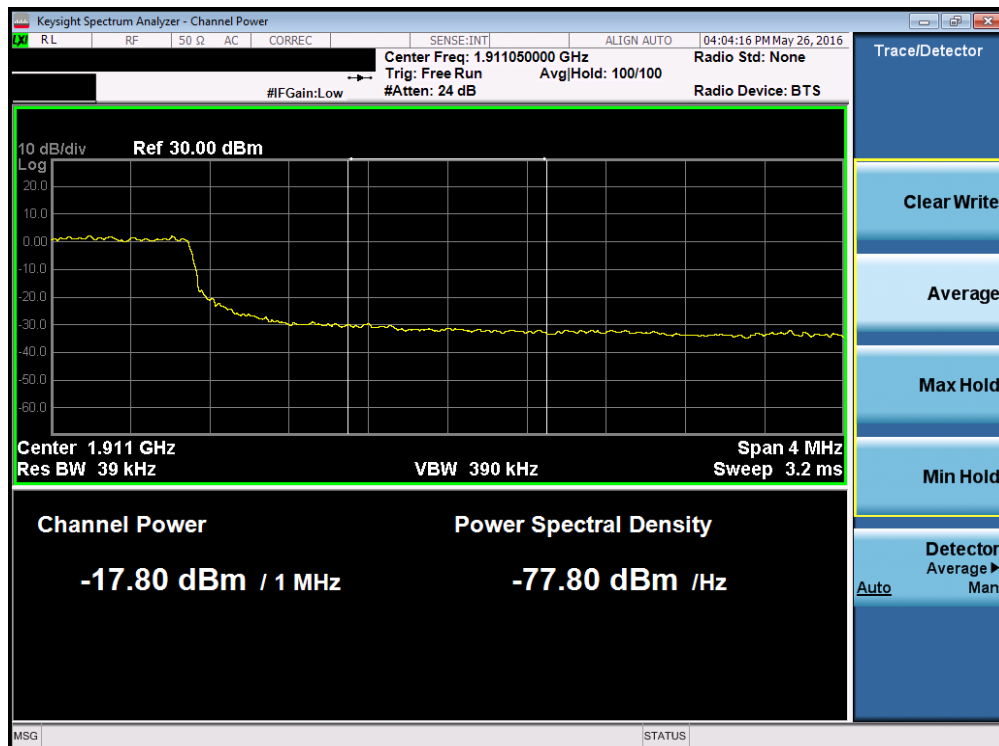
Plot 7-227. Upper Extended Band Edge Plot (Band 2 – 5.0MHz QPSK – RB Size 25)
