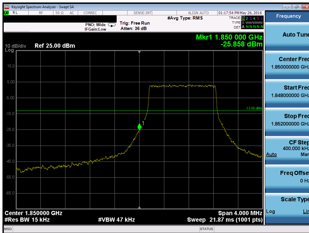
Plot 7-240. Lower Band Edge Plot (Band 25 – 1.4MHz QPSK – RB Size 6)
