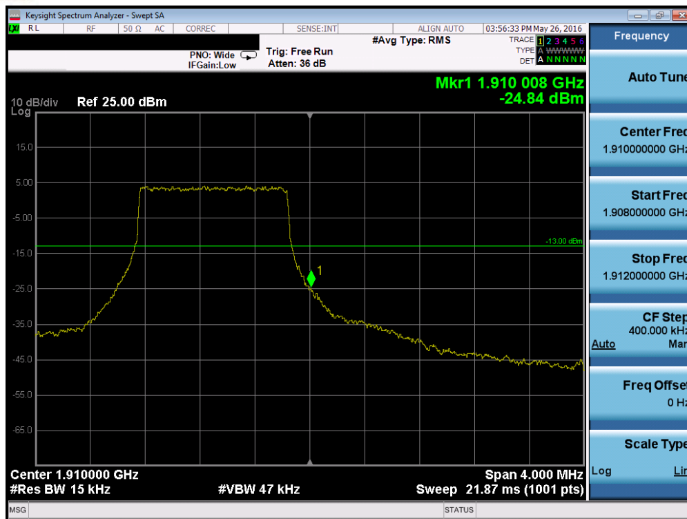
Plot 7-218. Upper Band Edge Plot (Band 2 – 1.4MHz QPSK – RB Size 6)
