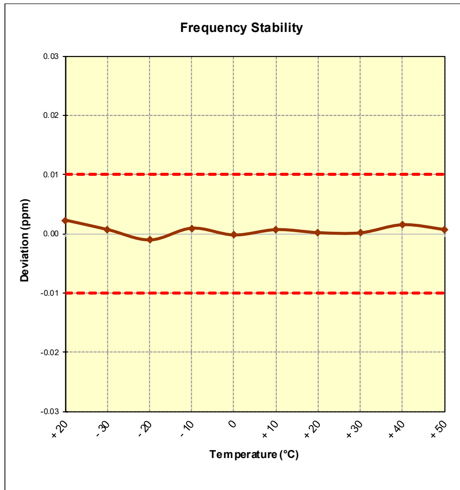
Figure 8-4. Frequency Stability Plot
