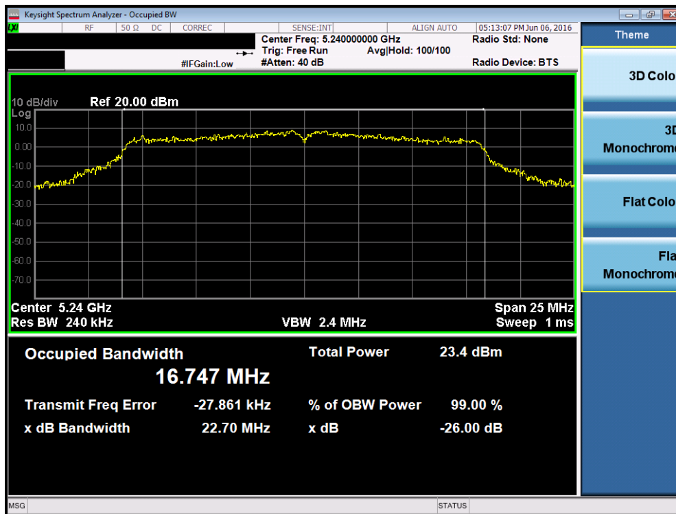
Plot 7-33. 26dB Bandwidth Plot (802.11a (UNII Band 1) – Ch. 48)
