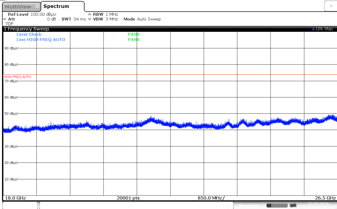
Plot 7-87. Radiated Spurious Plot above 18GHz (Pol. H)
