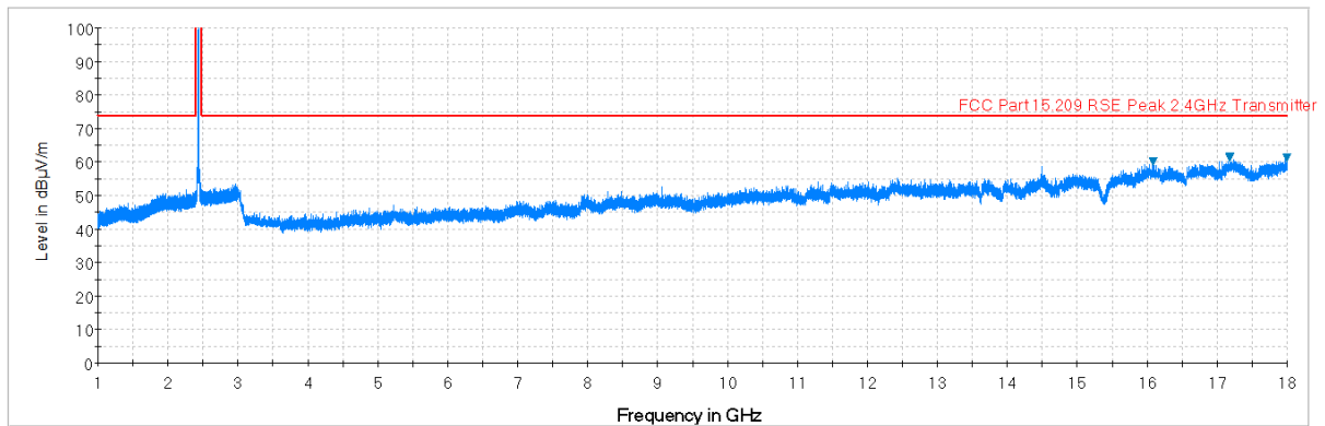
Plot 7-75. Radiated Spurious Plot above 1GHz (802.11b – Ch. 6, Ant. Pol. H)
