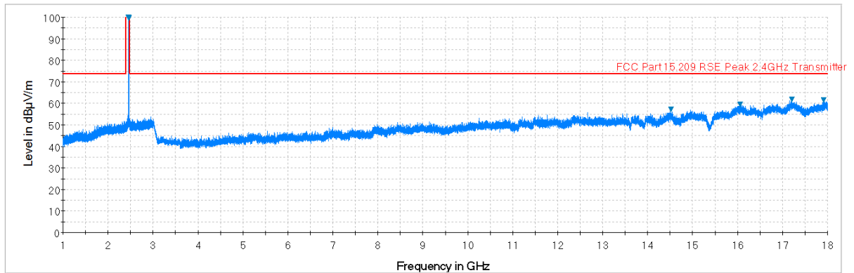
Plot 7-78. Radiated Spurious Plot above 1GHz (802.11b – Ch. 11, Ant. Pol. V)
