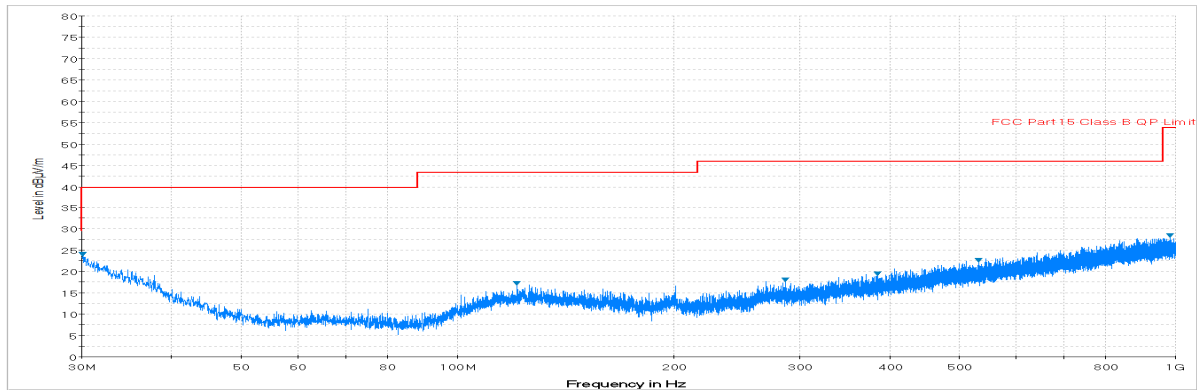
Plot 7-121. Radiated Spurious Plot below 1GHz (Pol. H)
