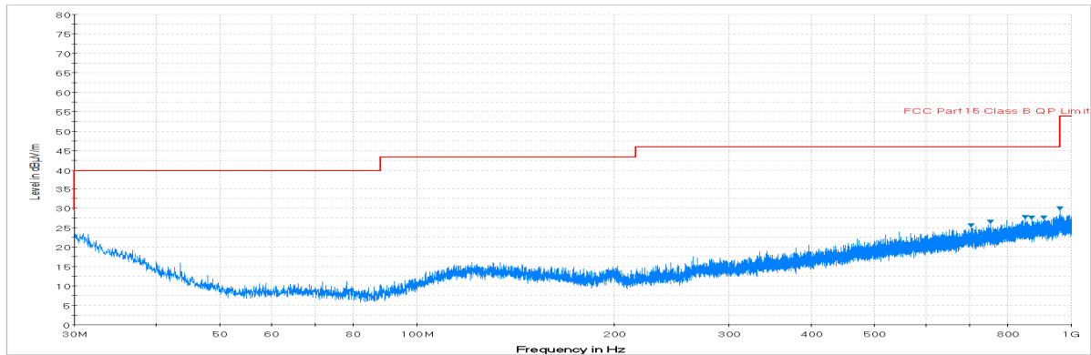
Plot 7-119. Radiated Spurious Plot below 1GHz (Pol. H)
