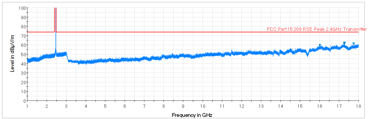
Plot 7-77. Radiated Spurious Plot above 1GHz (802.11b – Ch. 11, Ant. Pol. H)
