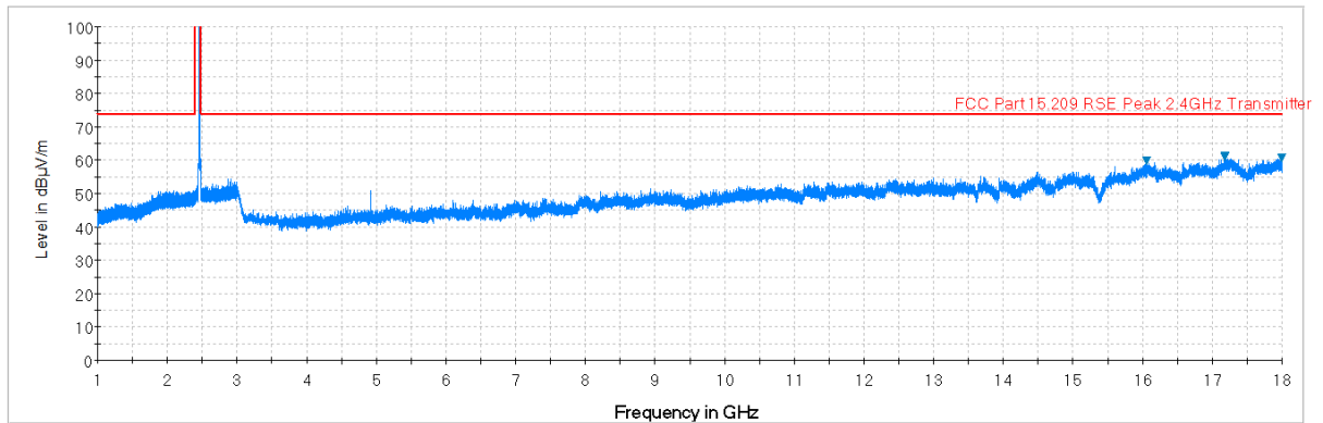
Plot 7-86. Radiated Spurious Plot above 1GHz (802.11b – Ch. 11, Ant. Pol. V)
