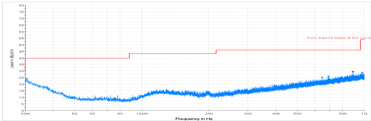
Plot 7-120. Radiated Spurious Plot below 1GHz (Pol. V)
