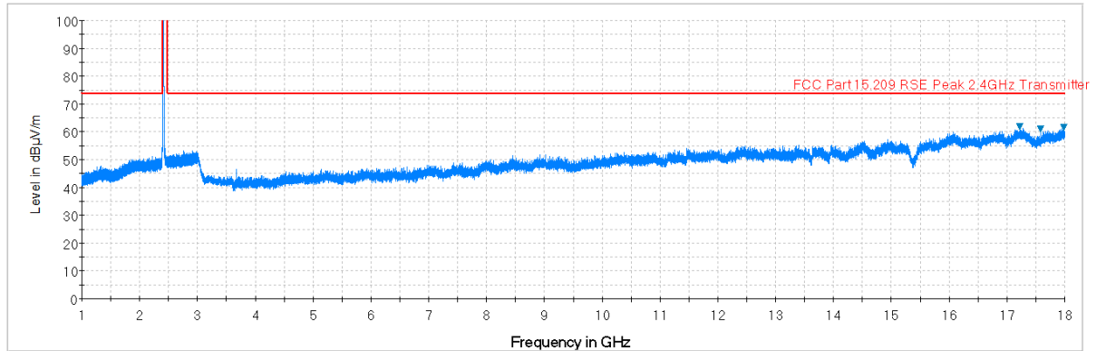
Plot 7-81. Radiated Spurious Plot above 1GHz (802.11b – Ch. 1, Ant. Pol. H)
