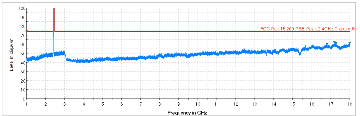
Plot 7-74. Radiated Spurious Plot above 1GHz (802.11b – Ch. 1, Ant. Pol. V)
