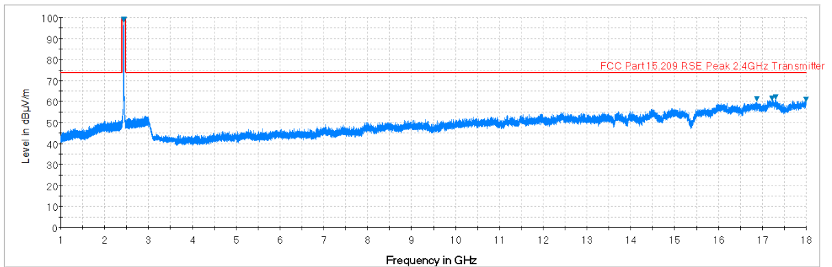
Plot 7-83. Radiated Spurious Plot above 1GHz (802.11b – Ch. 6, Ant. Pol. H)
