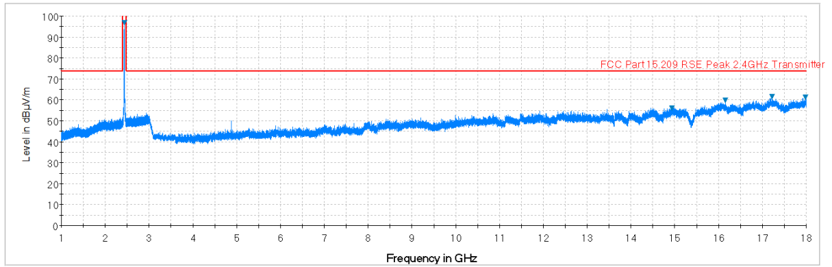
Plot 7-84. Radiated Spurious Plot above 1GHz (802.11b – Ch. 6, Ant. Pol. V)
