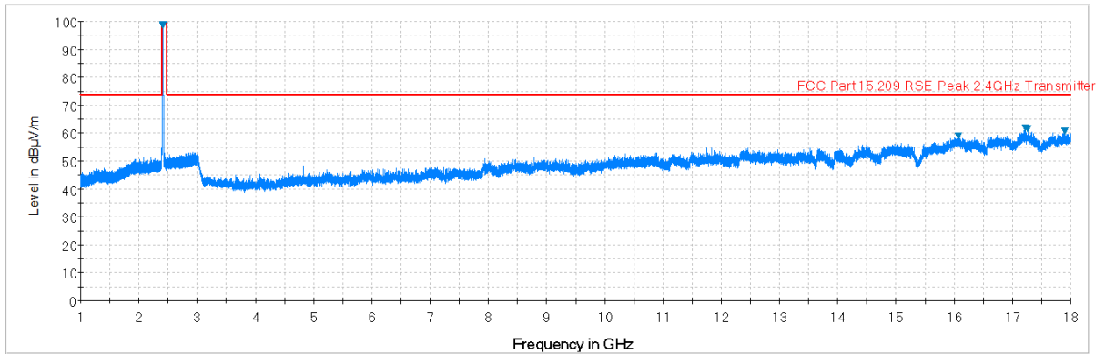
Plot 7-82. Radiated Spurious Plot above 1GHz (802.11b – Ch. 1, Ant. Pol. V)
