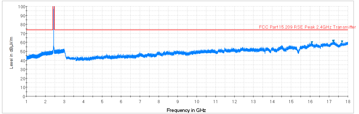
Plot 7-76. Radiated Spurious Plot above 1GHz (802.11b – Ch. 6, Ant. Pol. V)
