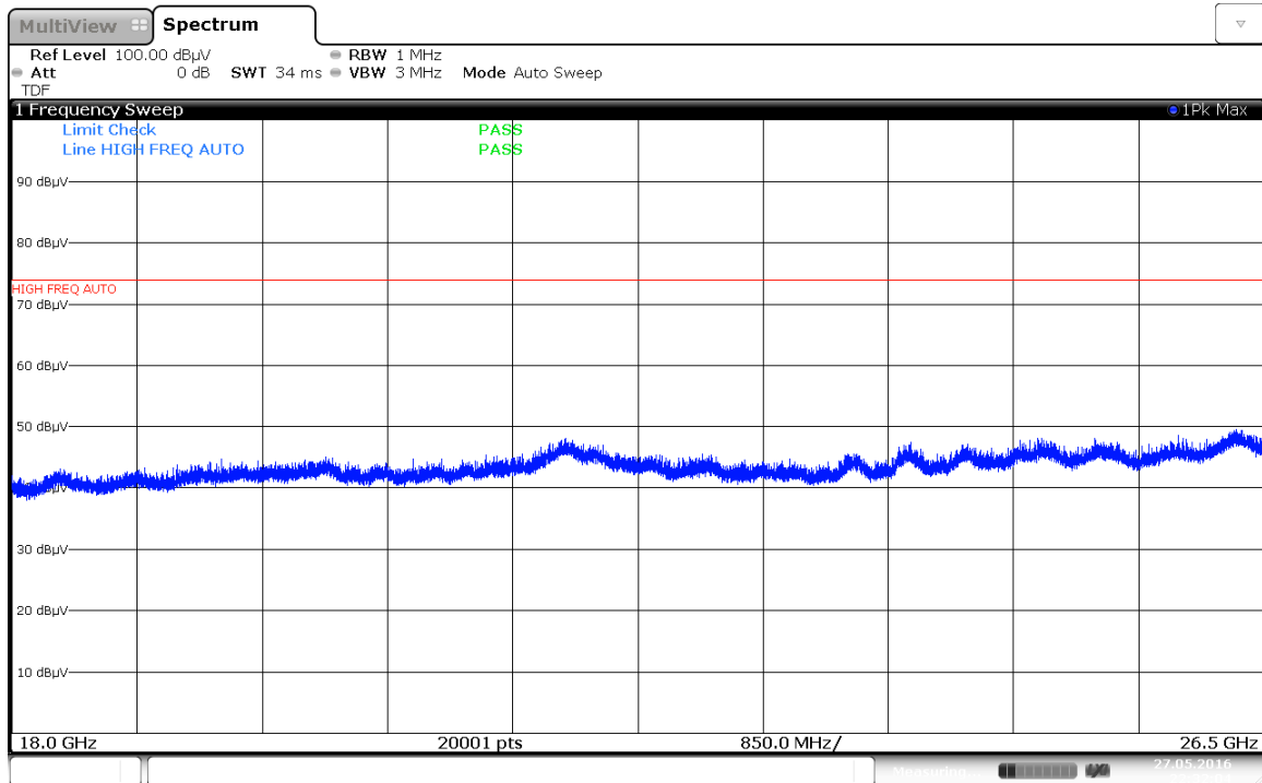
Plot 7-88. Radiated Spurious Plot above 18GHz (Pol. V)
