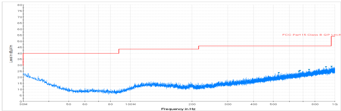
Plot 7-122. Radiated Spurious Plot below 1GHz (Pol. V)
