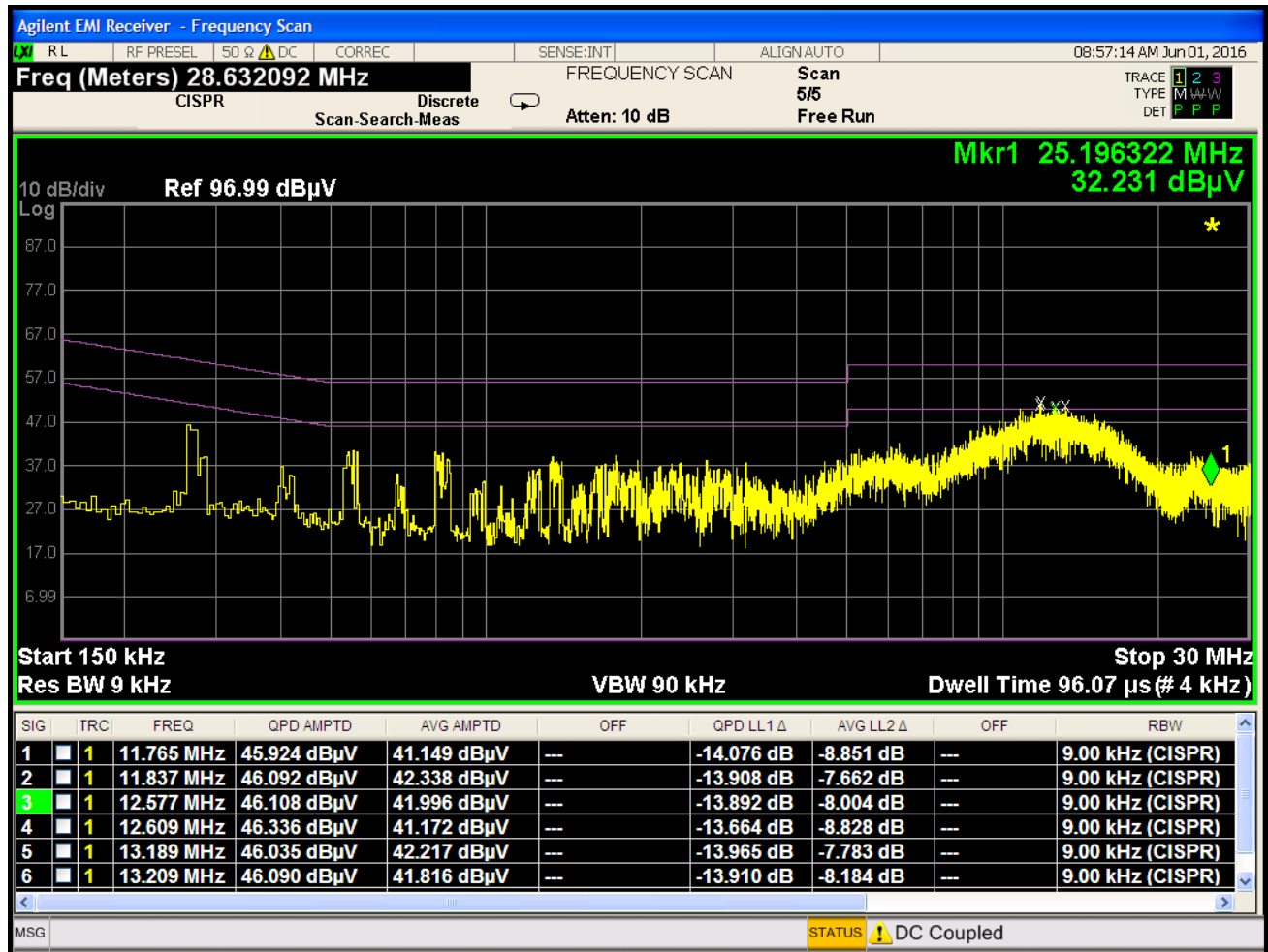
Plot 7-123. Line Conducted Plot with 802.11b (L1)
