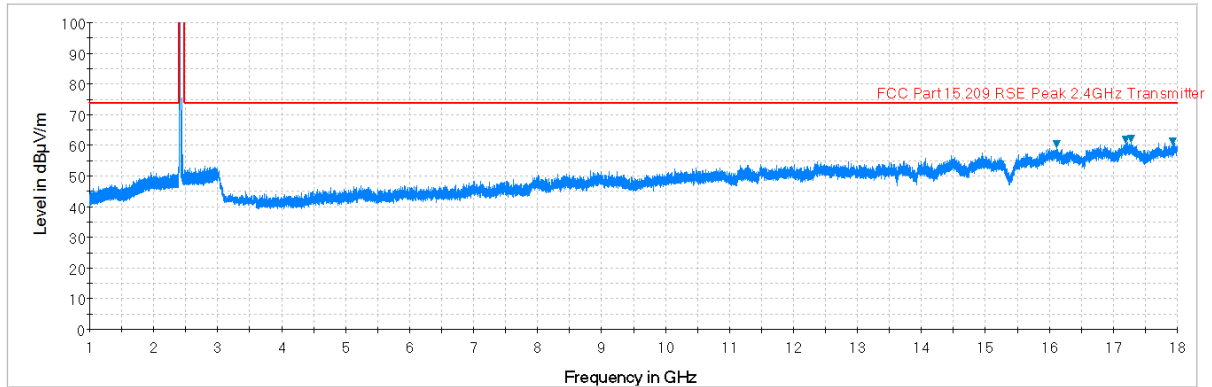
Plot 7-73. Radiated Spurious Plot above 1GHz (802.11b – Ch. 1, Ant. Pol. H)
