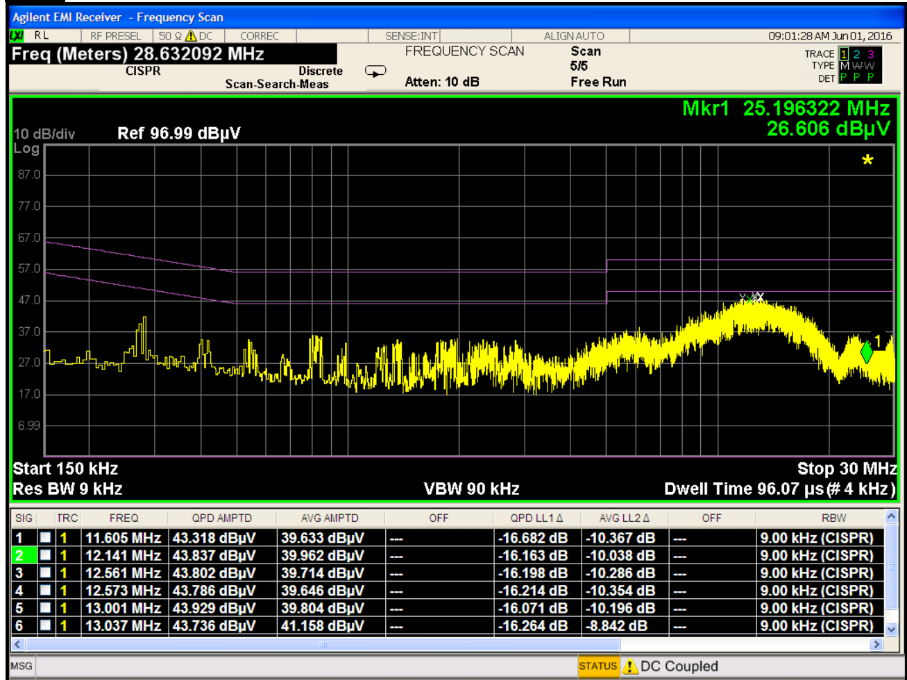
Plot 7-124. Line Conducted Plot with 802.11b (N)
