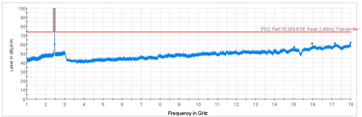
Plot 7-85. Radiated Spurious Plot above 1GHz (802.11b – Ch. 11, Ant. Pol. H)
