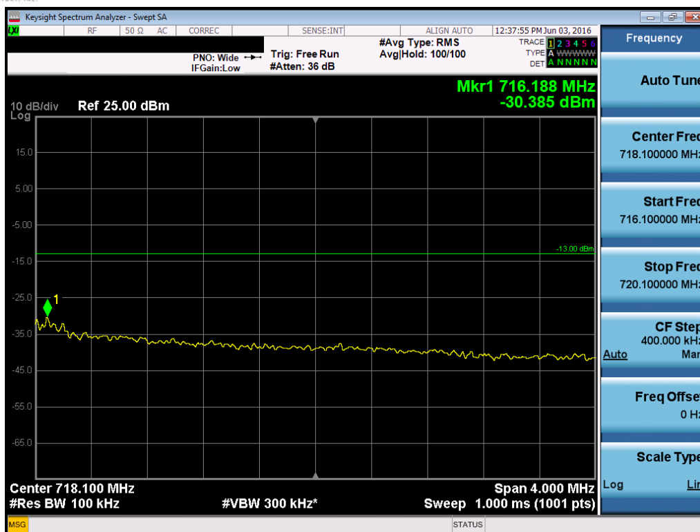
Plot 7-111. Upper Extended Band Edge Plot (Band 12/17 - 10.0MHz QPSK - RB Size 50)
