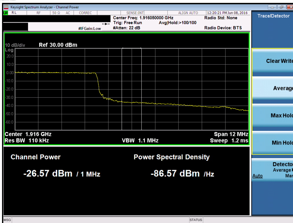
Plot 7-165. Upper Extended Band Edge Plot (Band 25 – 15.0MHz QPSK – RB Size 75)
