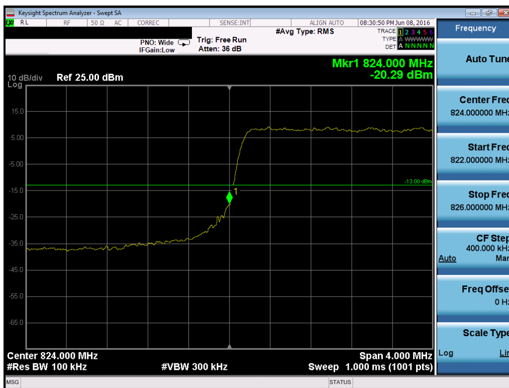
Plot 7-114. Lower Band Edge Plot (Band 5/26 – 3.0MHz QPSK – RB Size 15)
