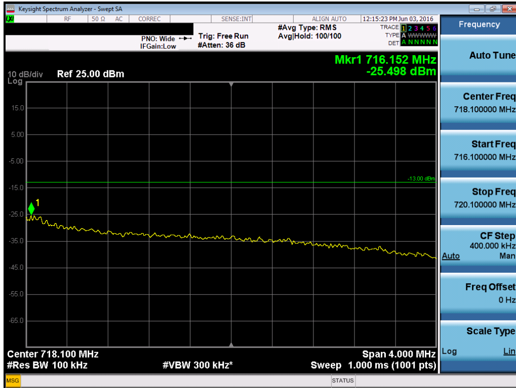
Plot 7-107. Upper Extended Band Edge Plot (Band 12/17 – 5.0MHz QPSK – RB Size 25)
