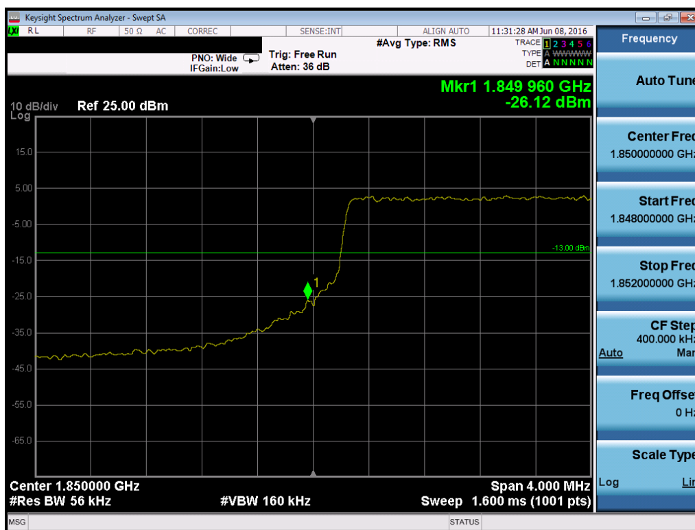
Plot 7-154. Lower Band Edge Plot (Band 25 – 5.0MHz QPSK – RB Size 25)
