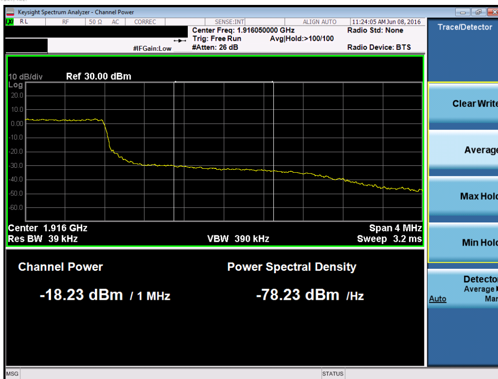
Plot 7-153. Upper Extended Band Edge Plot (Band 25 – 3.0MHz QPSK – RB Size 15)
