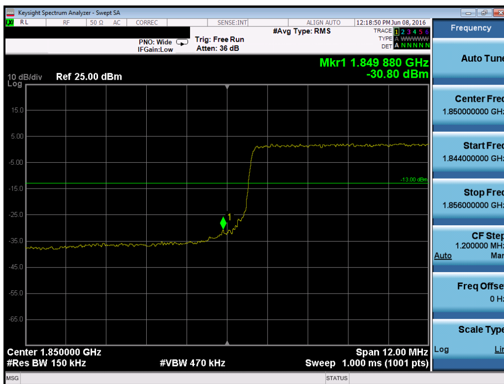
Plot 7-162. Lower Band Edge Plot (Band 25 – 15.0MHz QPSK – RB Size 75)
