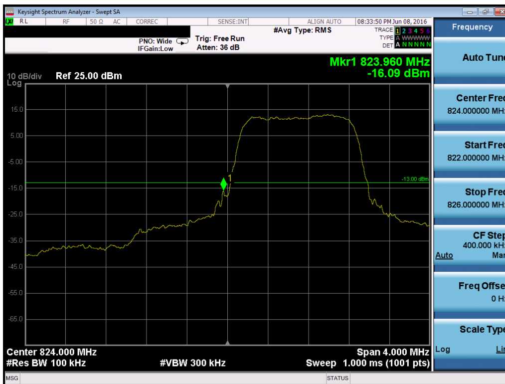
Plot 7-112. Lower Band Edge Plot (Band 5/26 - 1.4MHz QPSK - RB Size 6)
