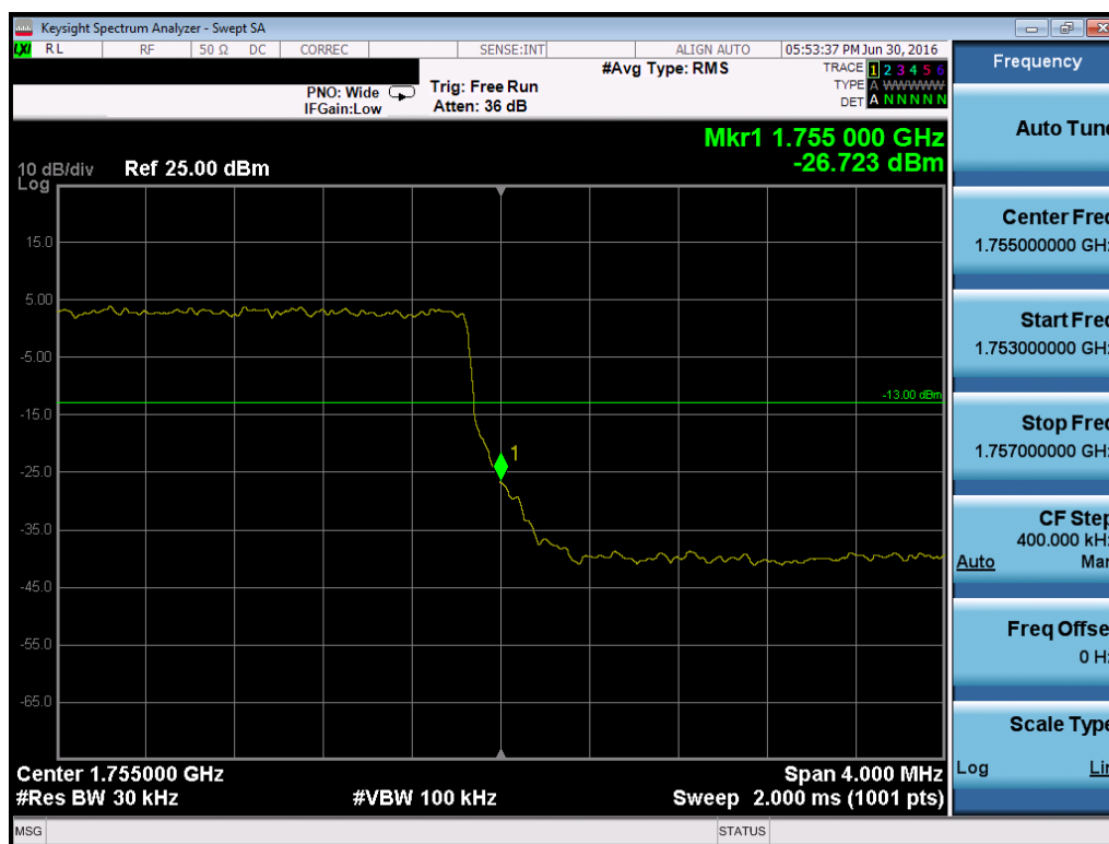
Plot 7-128. Upper Band Edge Plot (Band 4 – 3.0MHz QPSK – RB Size 15)
