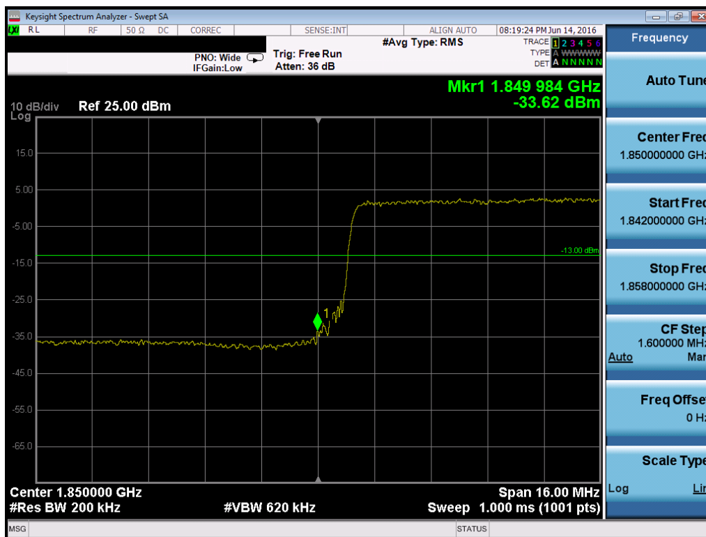
Plot 7-166. Lower Band Edge Plot (Band 25 – 20.0MHz QPSK – RB Size 100)
