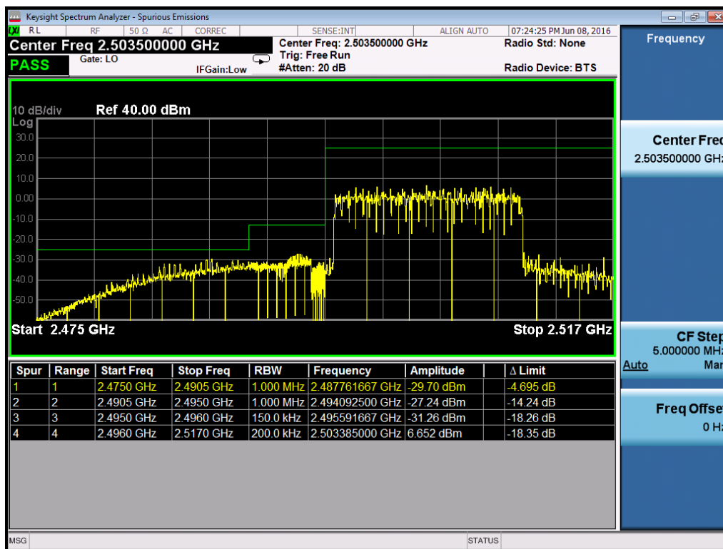
Plot 7-174. Lower ACP Plot (Band 41 – 15.0MHz QPSK – RB Size 75)
