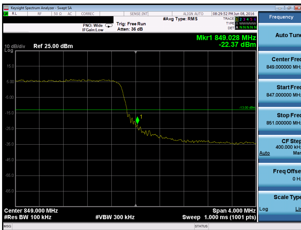
Plot 7-117. Upper Band Edge Plot (Band 5/26 – 5.0MHz QPSK – RB Size 25)
