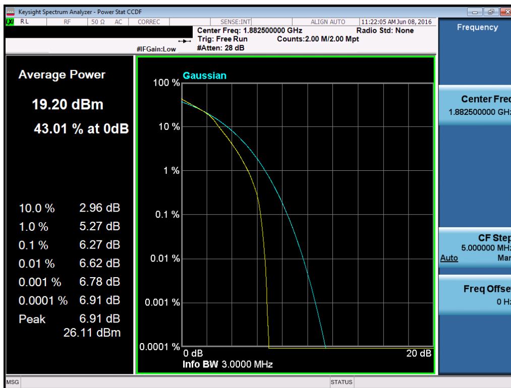
Plot 7-181. PAR Plot (Band 2/25 – 3.0MHz 16-QAM – RB Size 15)
