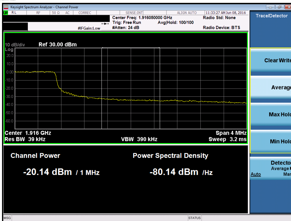
Plot 7-157. Upper Extended Band Edge Plot (Band 25 – 5.0MHz QPSK – RB Size 25)
