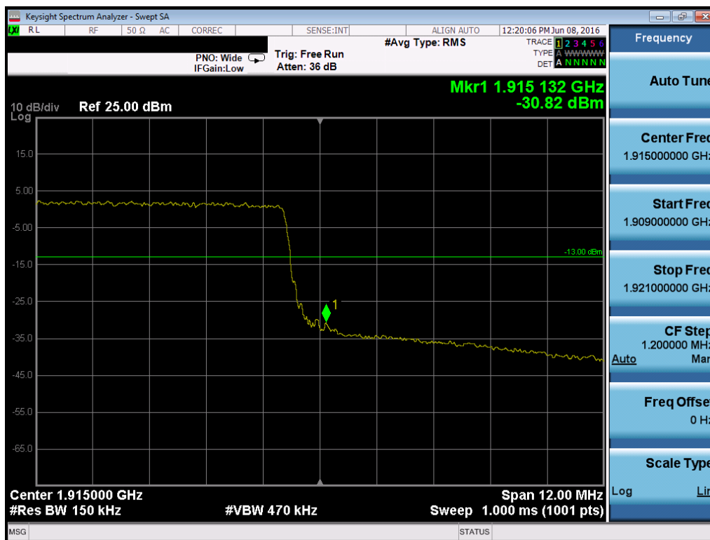
Plot 7-164. Upper Band Edge Plot (Band 25 – 15.0MHz QPSK – RB Size 75)
