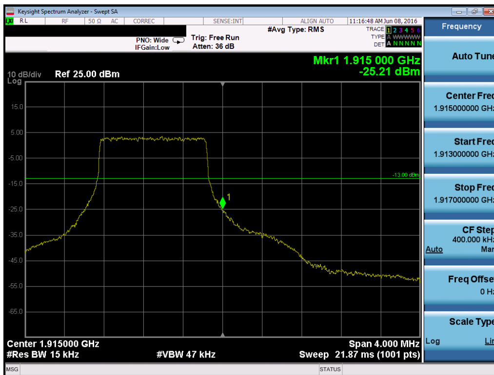
Plot 7-148. Upper Band Edge Plot (Band 25 – 1.4MHz QPSK – RB Size 6)
