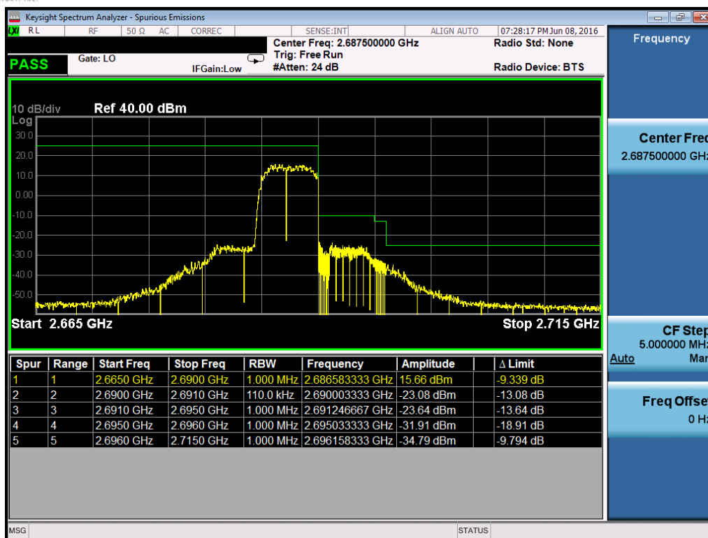
Plot 7-171. Upper ACP Plot (Band 41 – 5.0MHz QPSK – RB Size 25)
