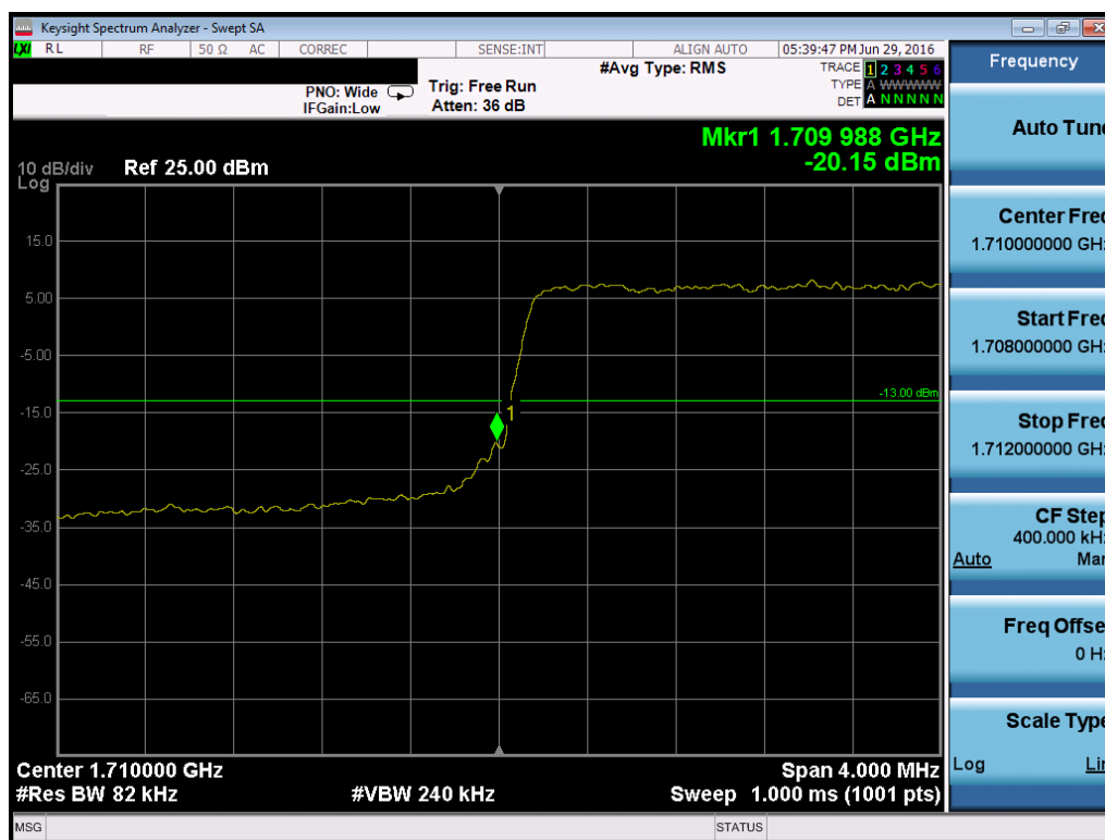
Plot 7-126. Lower Band Edge Plot (Band 4 – 3.0MHz QPSK – RB Size 15)
