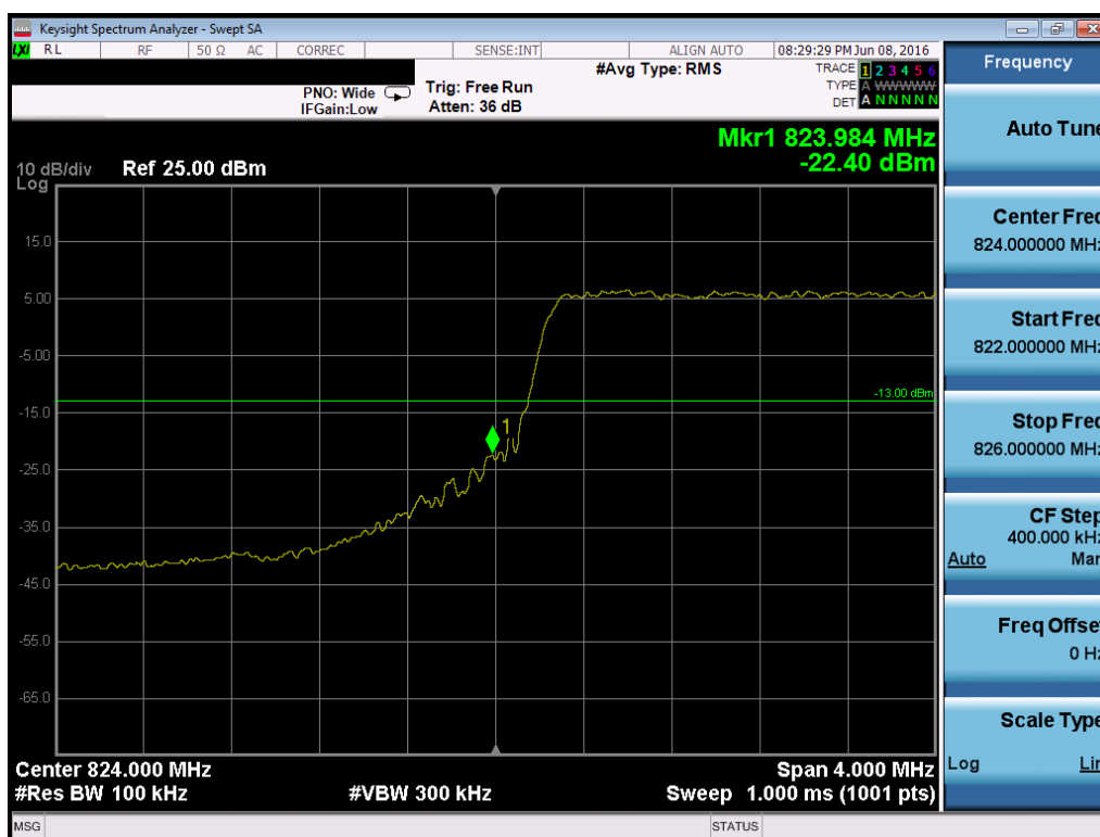
Plot 7-116. Lower Band Edge Plot (Band 5/26 – 5.0MHz QPSK – RB Size 25)
