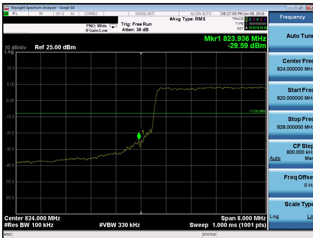
Plot 7-118. Lower Band Edge Plot (Band 5/26 – 10.0MHz QPSK – RB Size 50)
