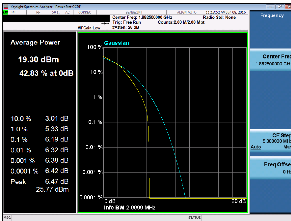
Plot 7-179. PAR Plot (Band 2/25 – 1.4MHz 16-QAM – RB Size 6)
