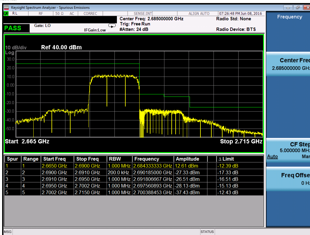
Plot 7-173. Upper ACP Plot (Band 41 – 10.0MHz QPSK – RB Size 50)
