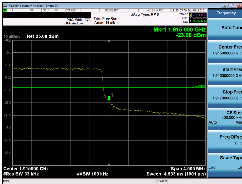
Plot 7-152. Upper Band Edge Plot (Band 25 – 3.0MHz QPSK – RB Size 15)
