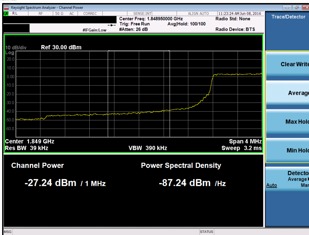
Plot 7-151. Lower Extended Band Edge Plot (Band 25 – 3.0MHz QPSK – RB Size 15)
