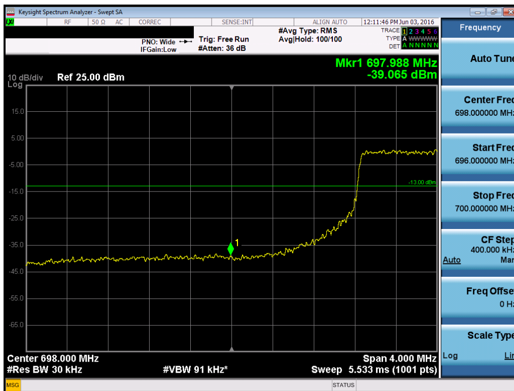
Plot 7-104. Lower Band Edge Plot (Band 12/17 – 5.0MHz QPSK – RB Size 25)
