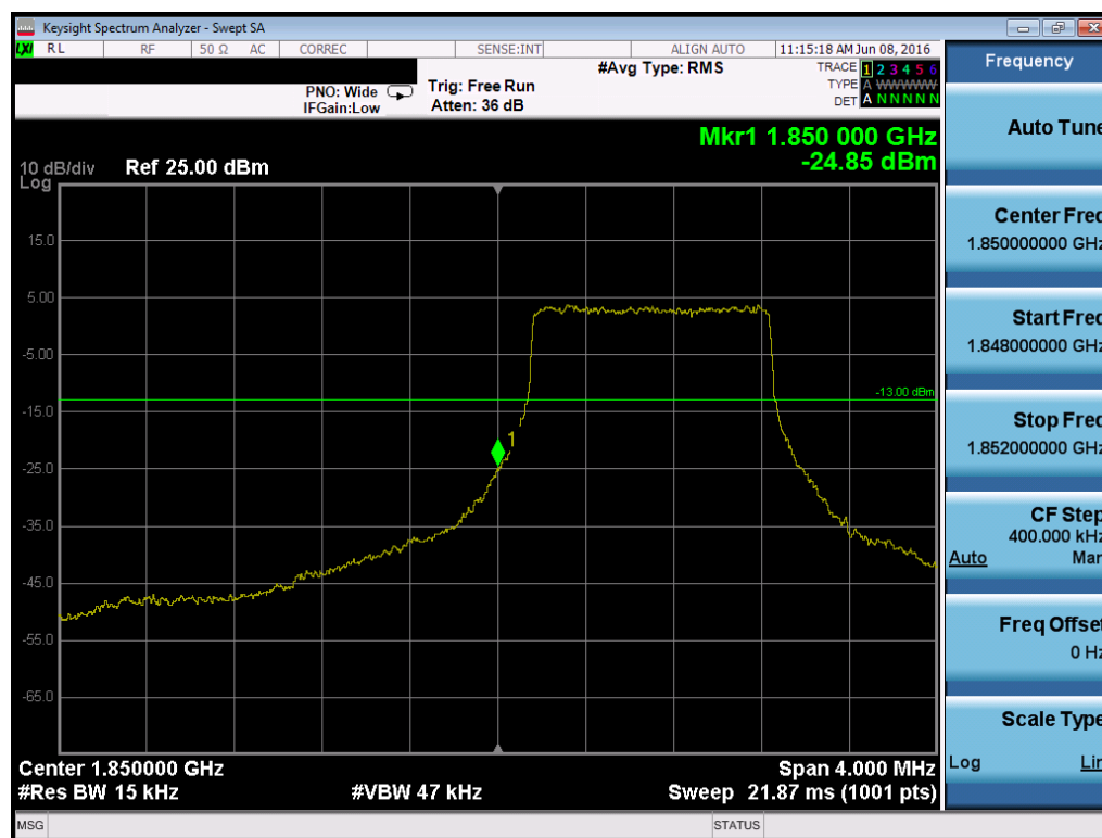
Plot 7-146. Lower Band Edge Plot (Band 25 – 1.4MHz QPSK – RB Size 6)
