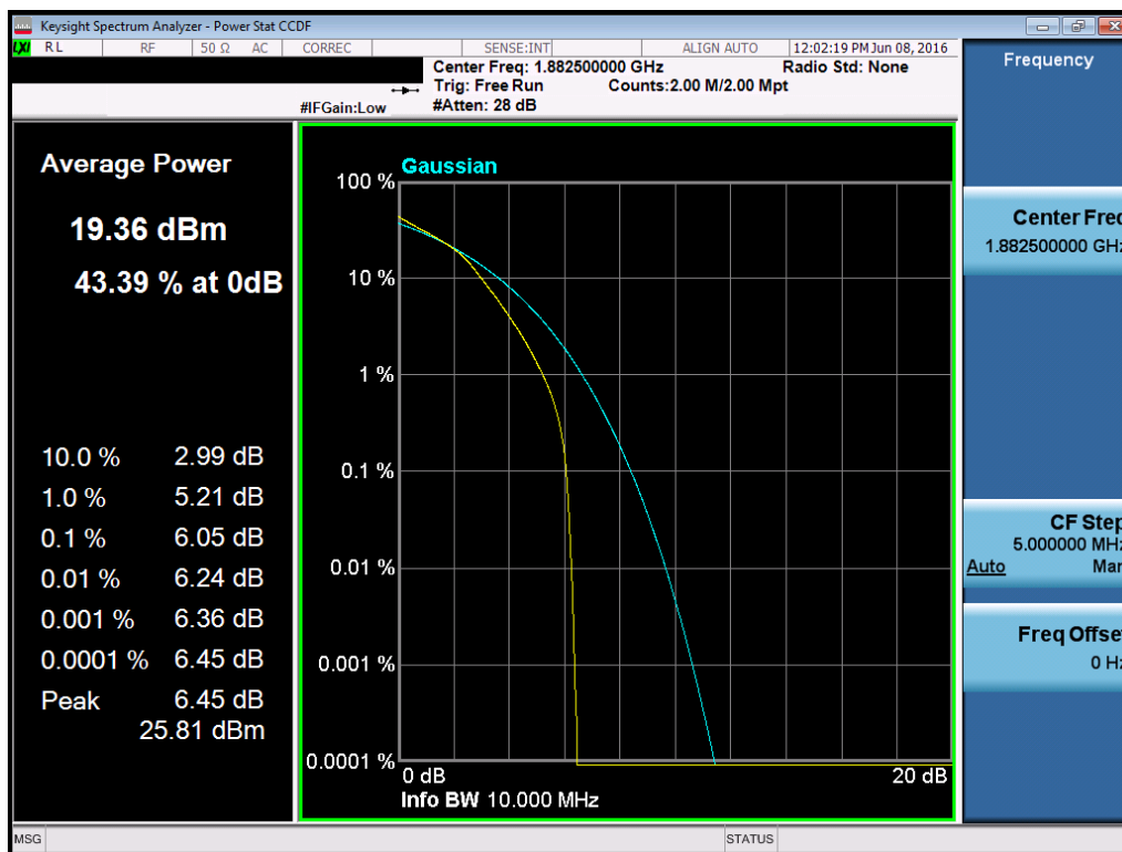
Plot 7-185. PAR Plot (Band 2/25 – 10.0MHz 16-QAM – RB Size 50)
