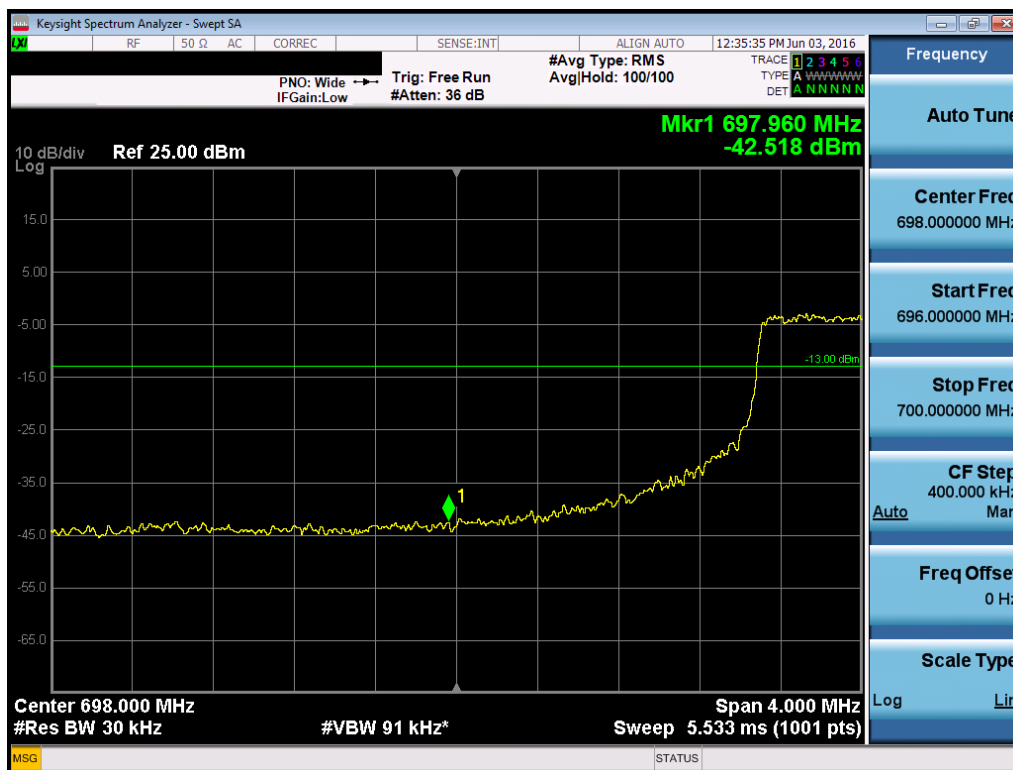
Plot 7-108. Lower Band Edge Plot (Band 12/17 – 10.0MHz QPSK – RB Size 50)
