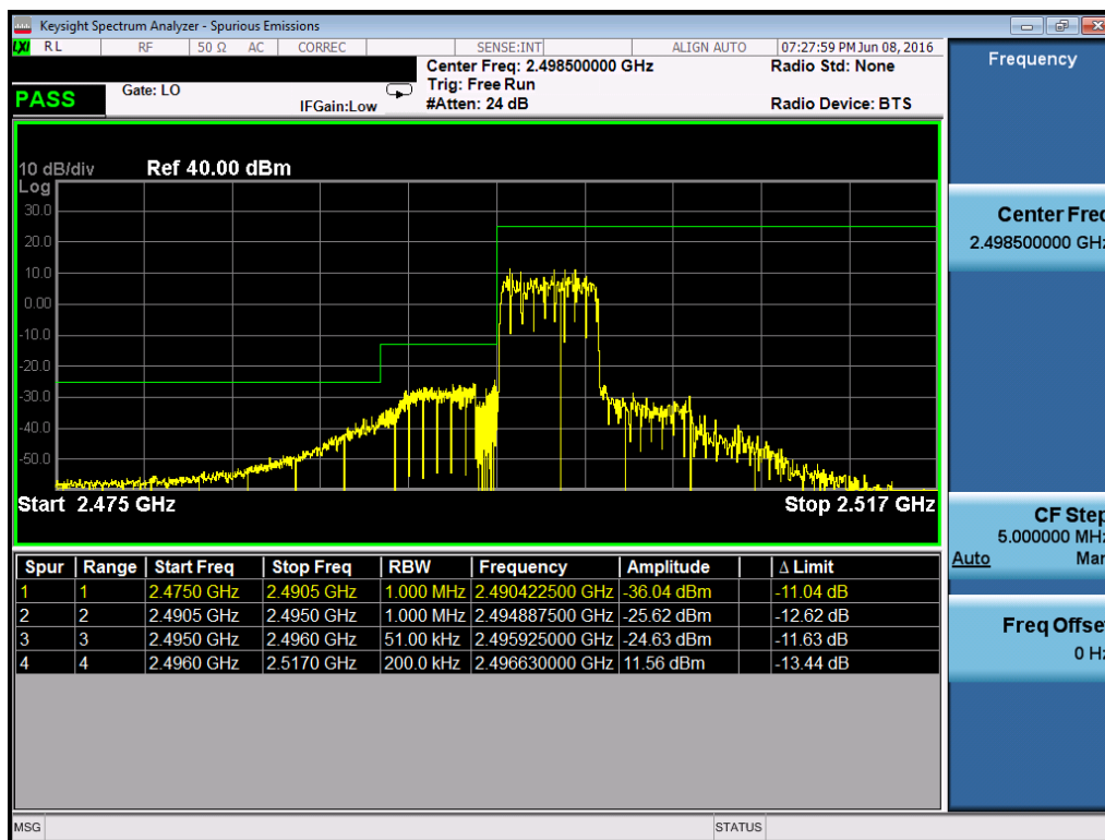
Plot 7-170. Lower ACP Plot (Band 41 – 5.0MHz QPSK – RB Size 25)
