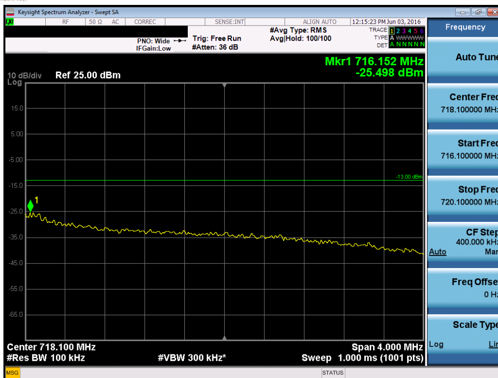
Plot 7-107. Upper Extended Band Edge Plot (Band 12/17 – 5.0MHz QPSK – RB Size 25)
