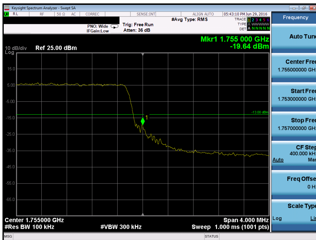
Plot 7-132. Upper Band Edge Plot (Band 4 – 5.0MHz QPSK – RB Size 25)
