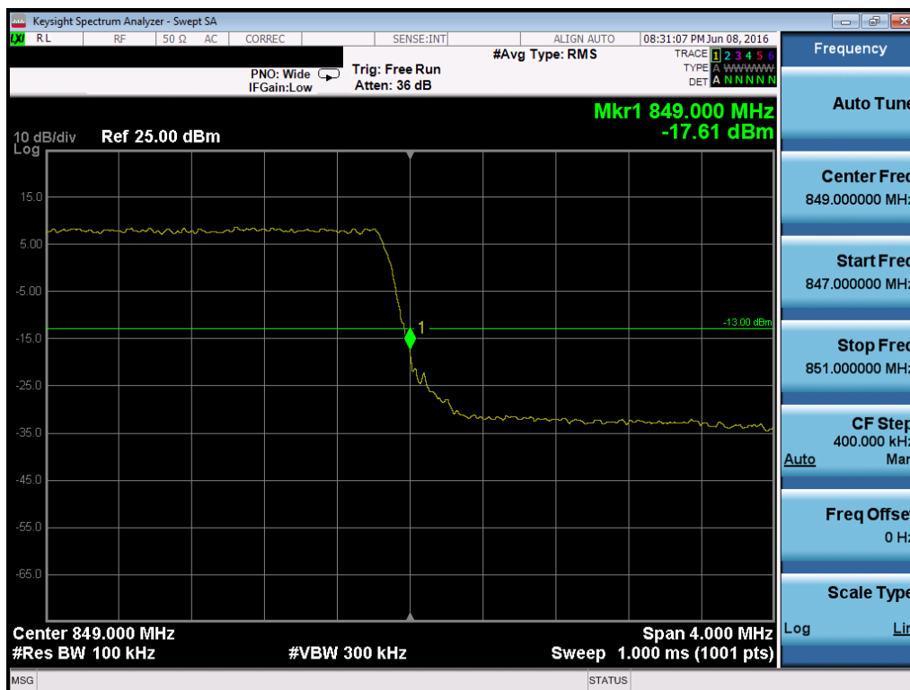
Plot 7-115. Upper Band Edge Plot (Band 5/26 – 3.0MHz QPSK – RB Size 15)
