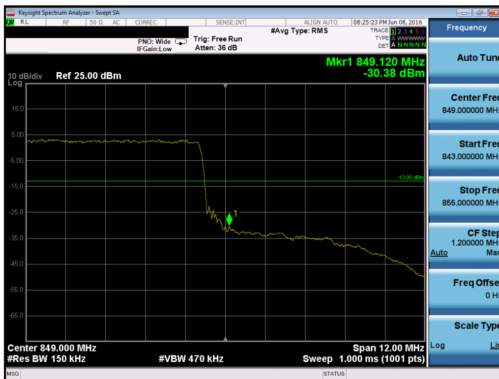
Plot 7-121. Upper Band Edge Plot (Band 26 – 15.0MHz QPSK – RB Size 50)
