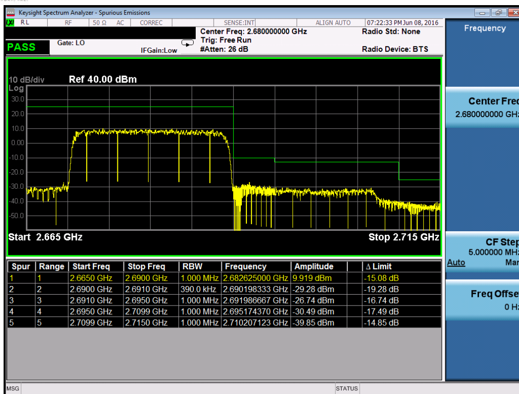
Plot 7-177. Upper ACP Plot (Band 41 – 20.0MHz QPSK – RB Size 100)
