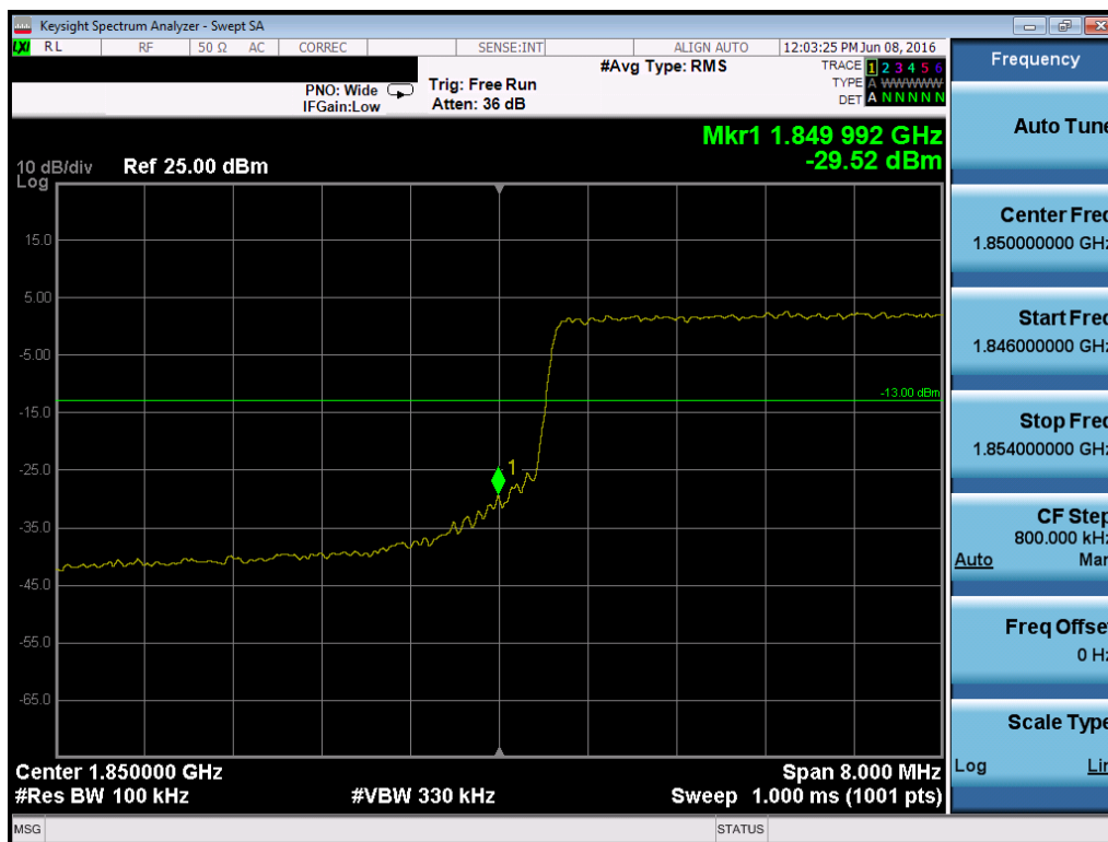
Plot 7-158. Lower Band Edge Plot (Band 25 – 10.0MHz QPSK – RB Size 50)
