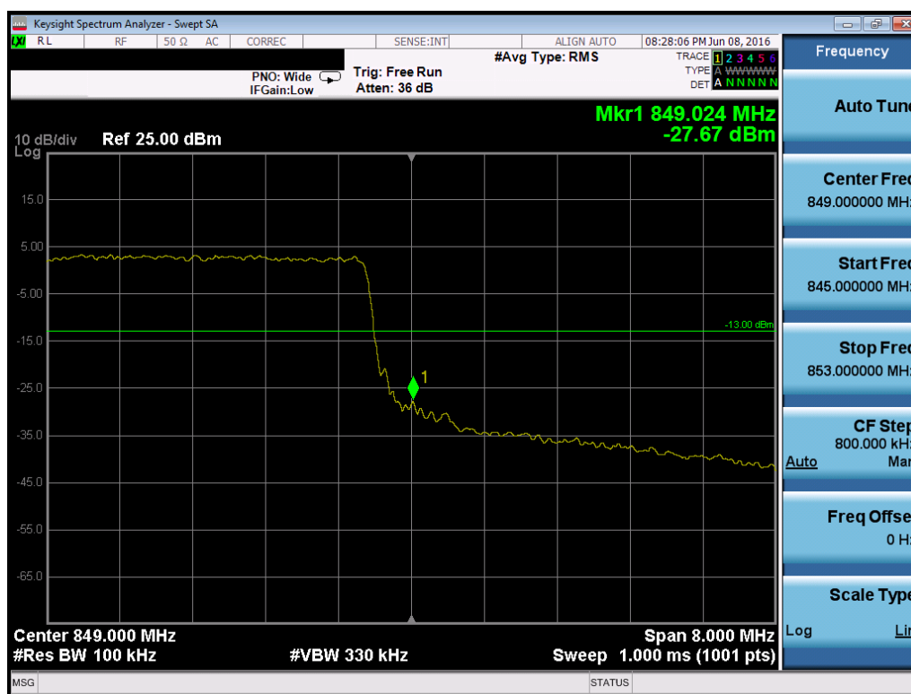
Plot 7-119. Upper Band Edge Plot (Band 5/26 – 10.0MHz QPSK – RB Size 50)
