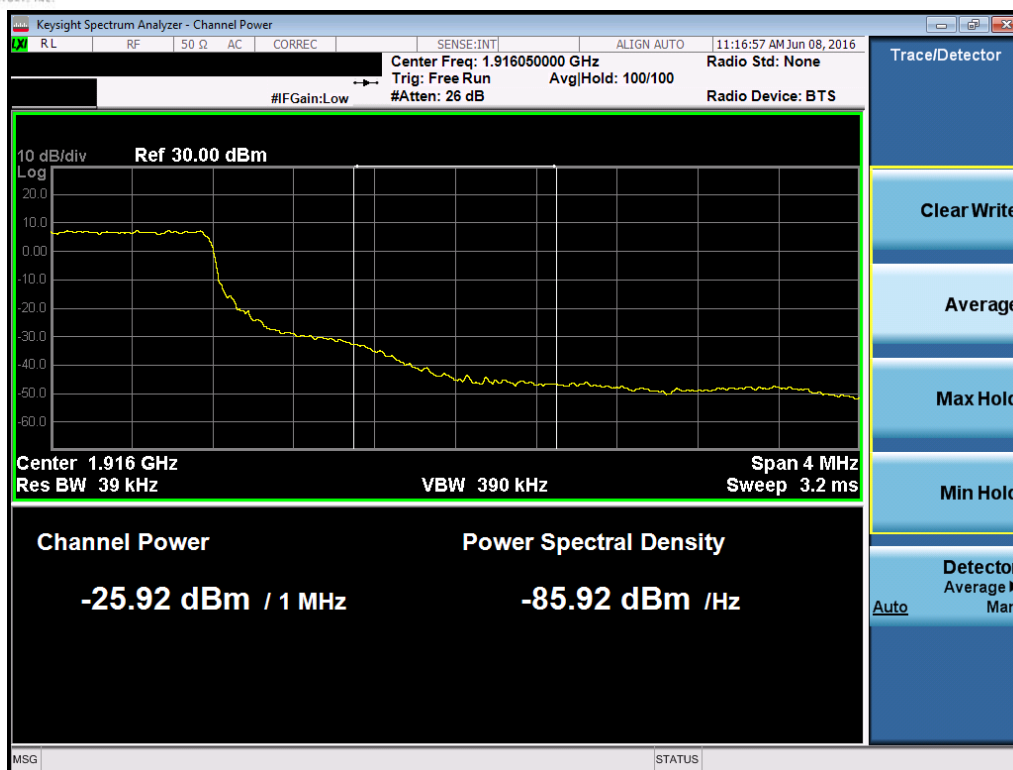
Plot 7-149. Upper Extended Band Edge Plot (Band 25 – 1.4MHz QPSK – RB Size 6)
