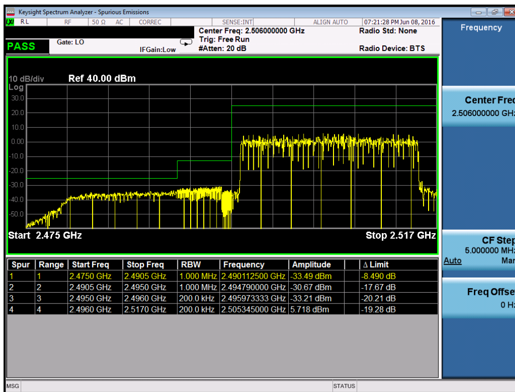
Plot 7-176. Lower ACP Plot (Band 41 – 20.0MHz QPSK – RB Size 100)
