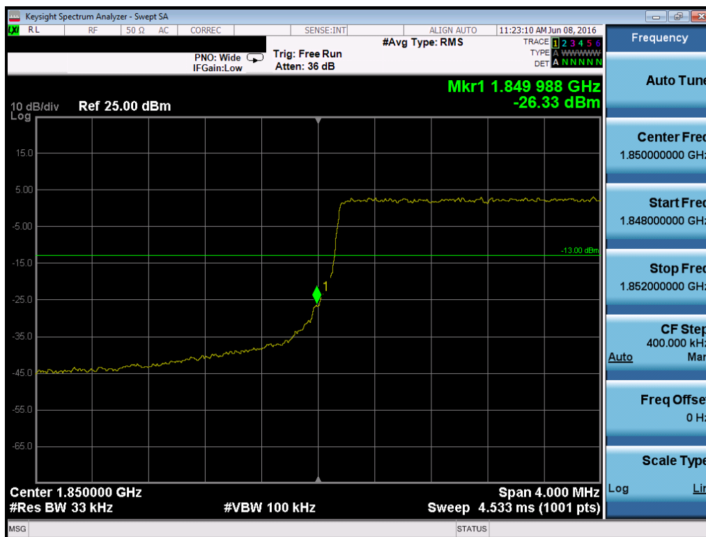
Plot 7-150. Lower Band Edge Plot (Band 25 – 3.0MHz QPSK – RB Size 15)
