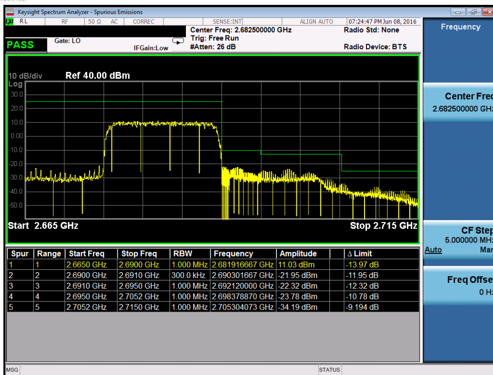
Plot 7-175. Upper ACP Plot (Band 41 – 15.0MHz QPSK – RB Size 75)
