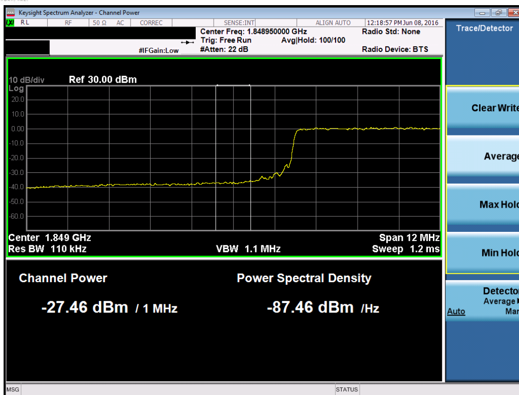
Plot 7-163. Lower Extended Band Edge Plot (Band 25 – 15.0MHz QPSK – RB Size 75)
