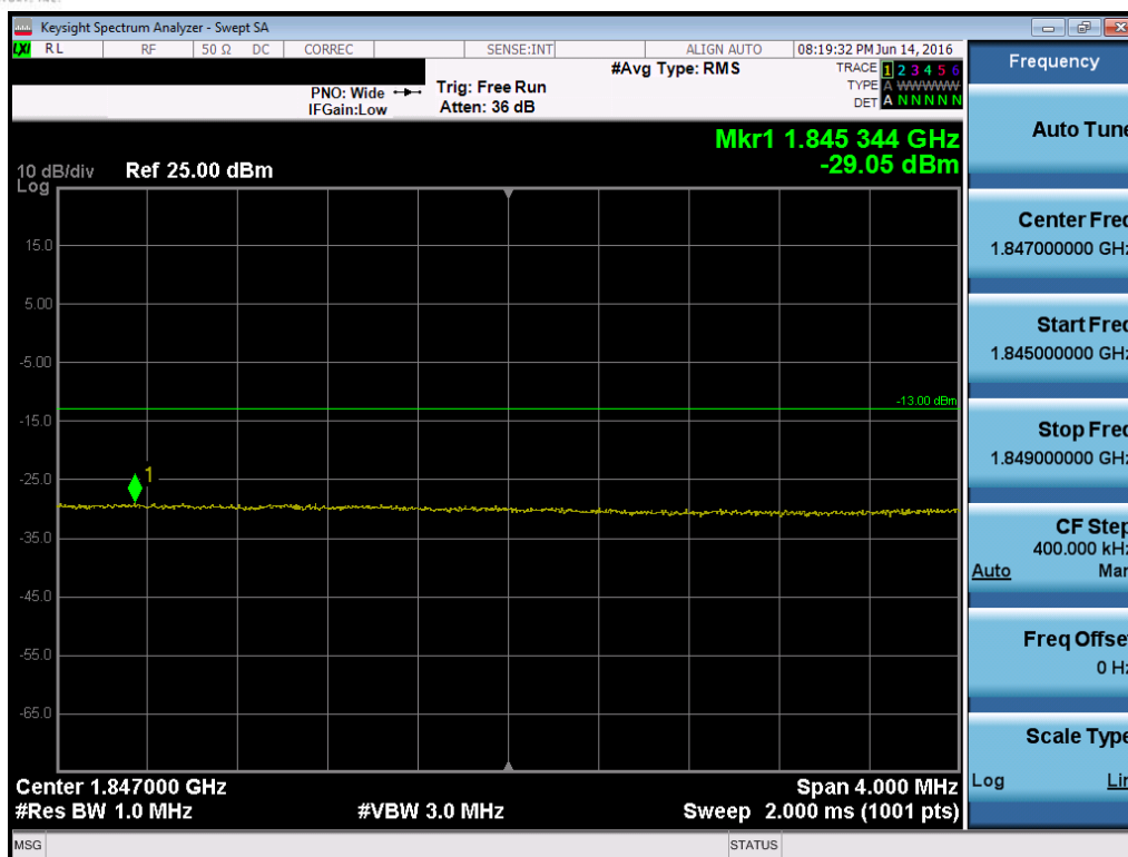
Plot 7-167. Lower Extended Band Edge Plot (Band 25 – 20.0MHz QPSK – RB Size 100)
