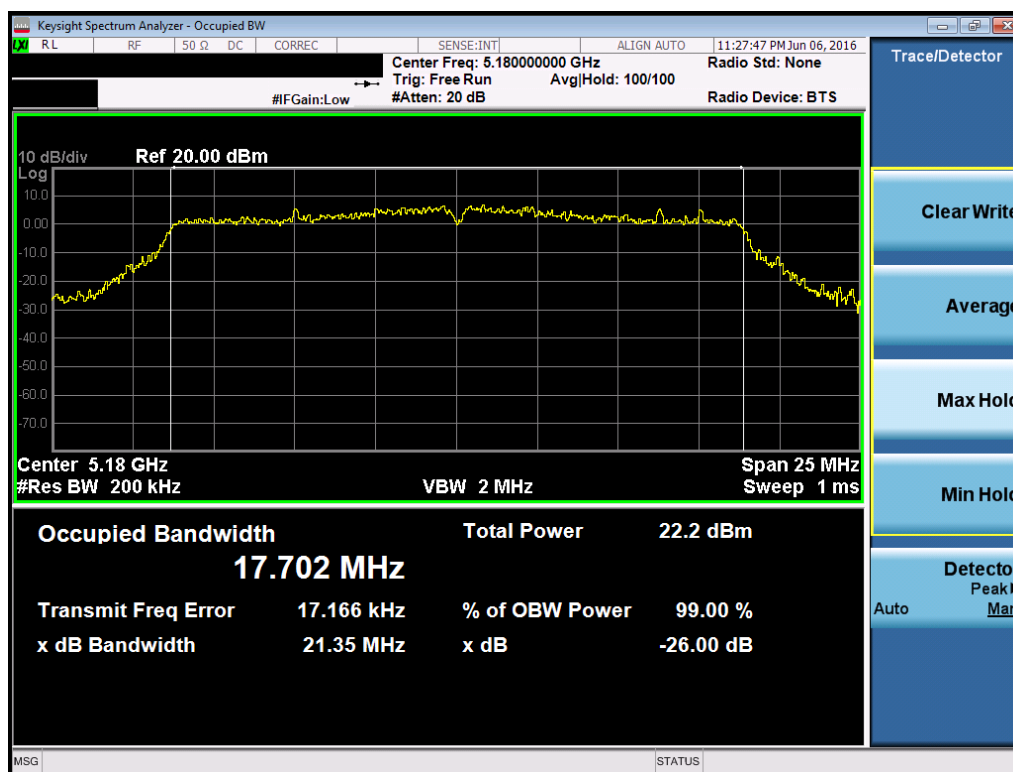
Plot 7-32. 26dB Bandwidth Plot (20MHz BW 802.11n (UNII Band 1) – Ch. 36)
