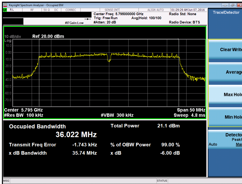
Plot 7-64. 6dB Bandwidth Plot (40MHz BW 802.11n (UNII Band 3) – Ch. 159)
