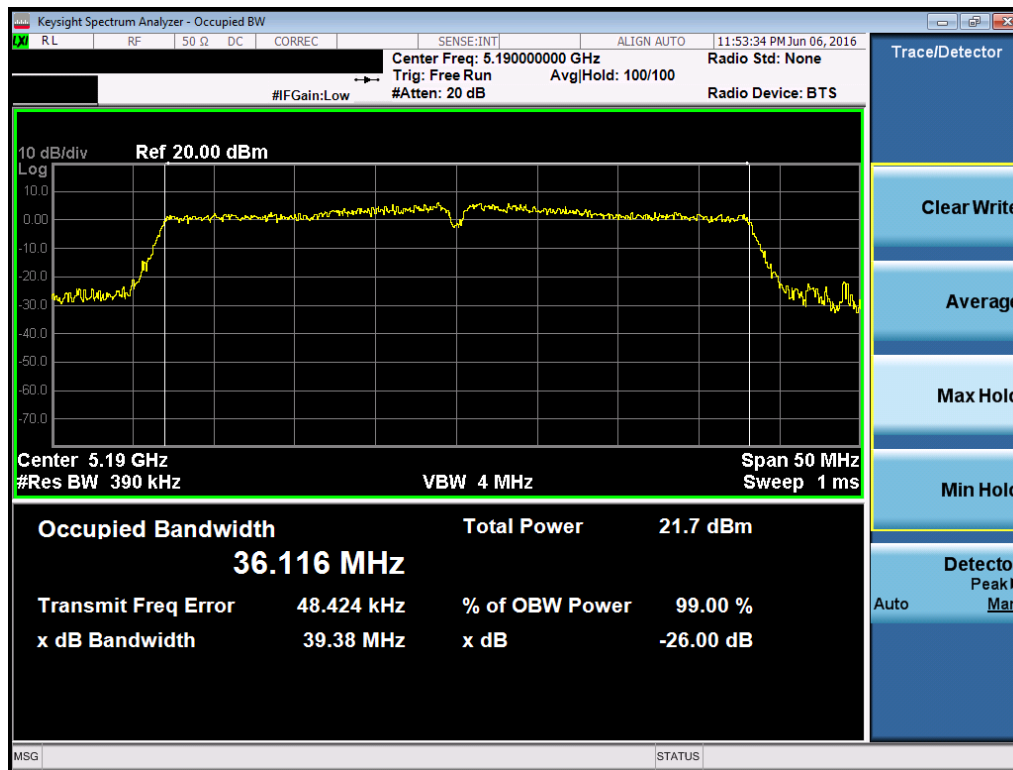
Plot 7-35. 26dB Bandwidth Plot (40MHz BW 802.11n (UNII Band 1) – Ch. 38)
