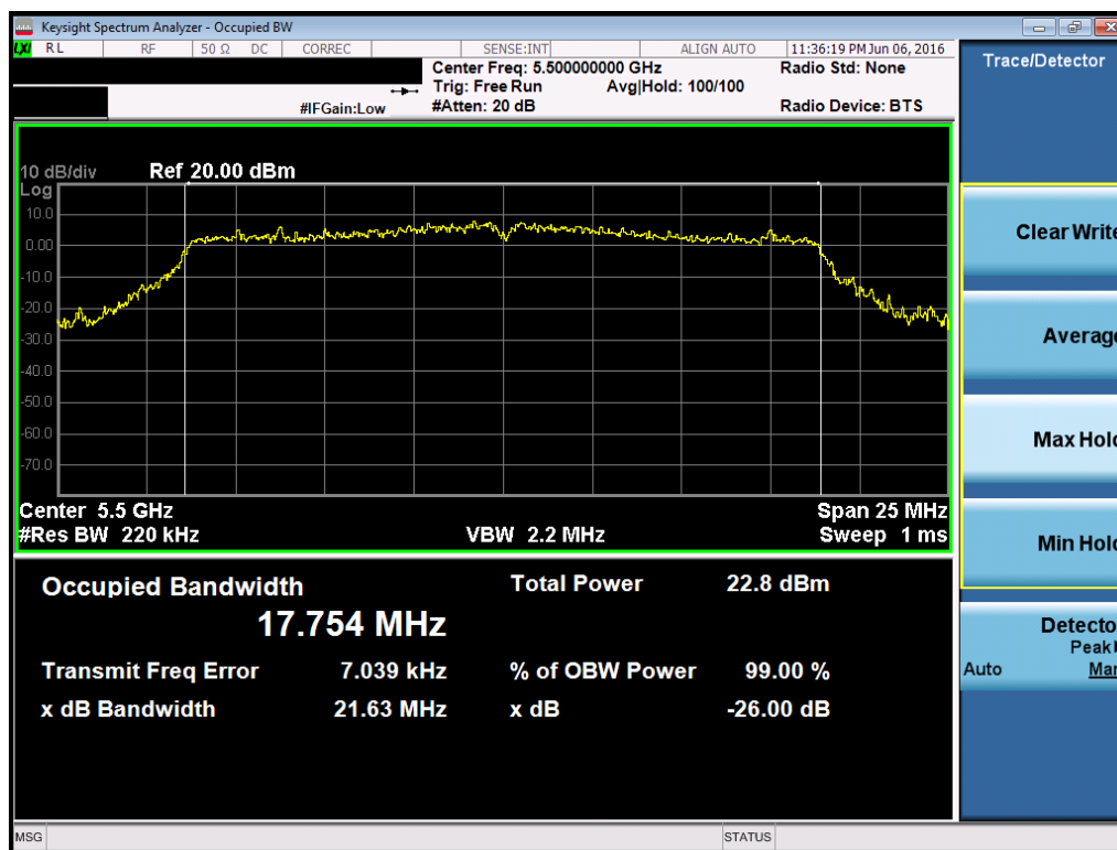
Plot 7-50. 26dB Bandwidth Plot (20MHz BW 802.11n (UNII Band 2C) – Ch. 100)
