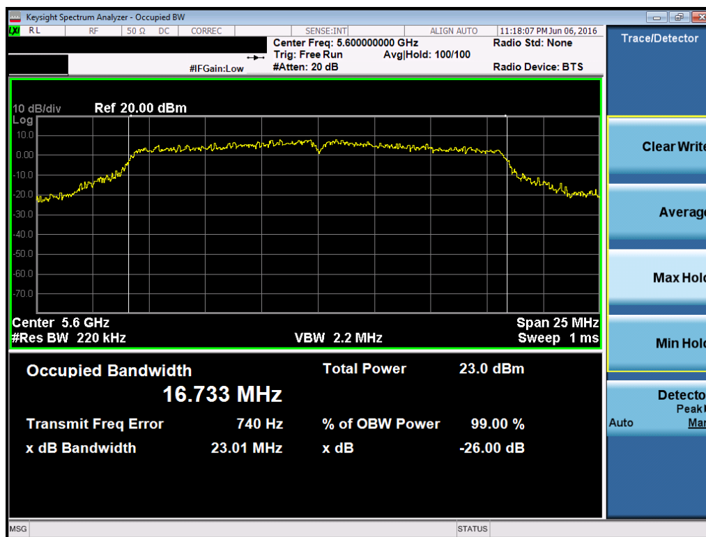
Plot 7-48. 26dB Bandwidth Plot (802.11a (UNII Band 2C) – Ch. 120)
