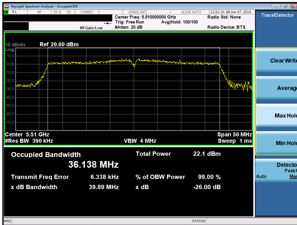
Plot 7-53. 26dB Bandwidth Plot (40MHz BW 802.11n (UNII Band 2C) – Ch. 102)
