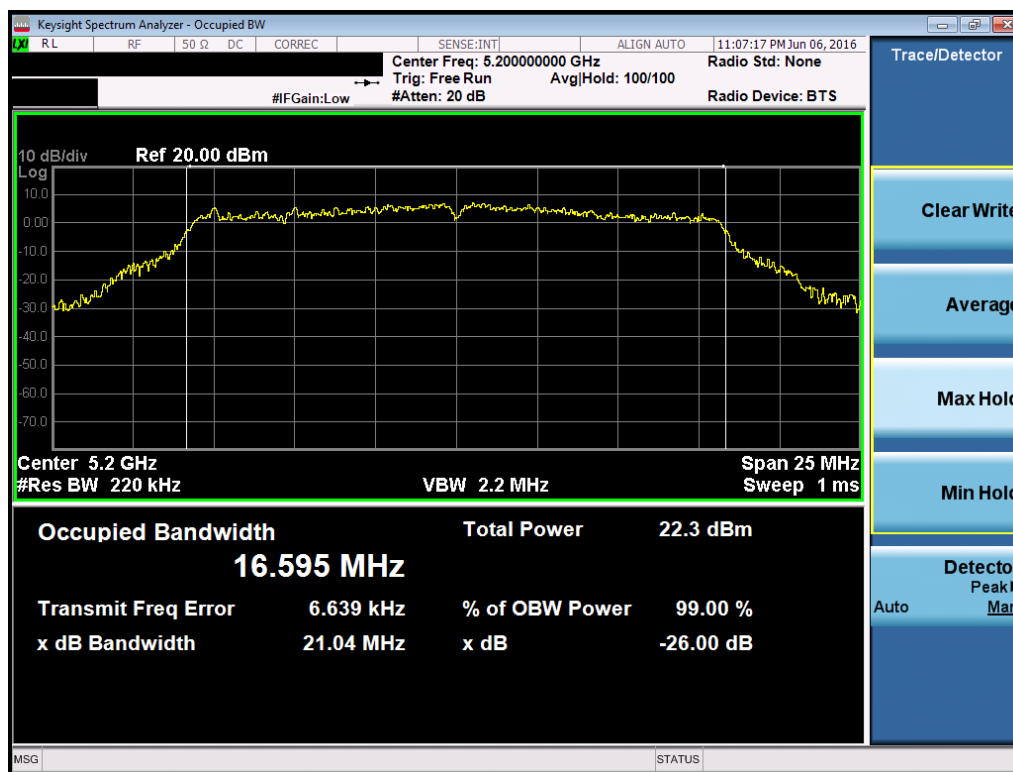
Plot 7-30. 26dB Bandwidth Plot (802.11a (UNII Band 1) – Ch. 40)
