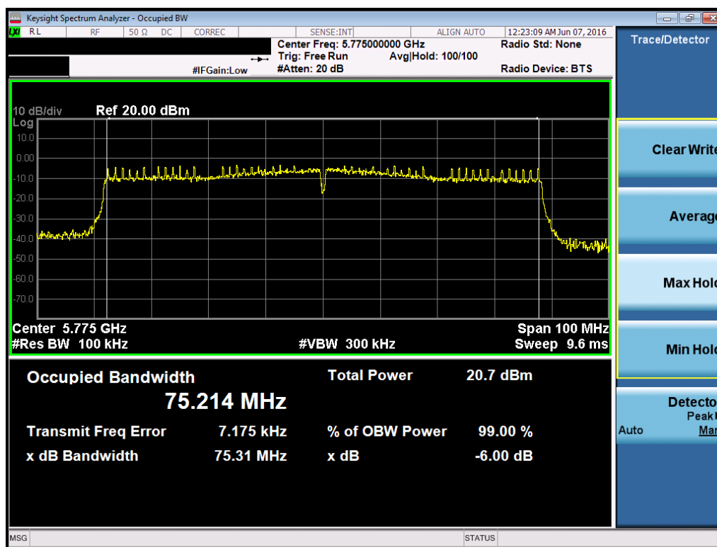
Plot 7-74. 6dB Bandwidth Plot (80MHz BW 802.11ac (UNII Band 3) – Ch. 155)
