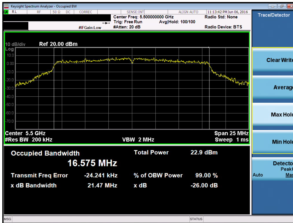
Plot 7-47. 26dB Bandwidth Plot (802.11a (UNII Band 2C) – Ch. 100)
