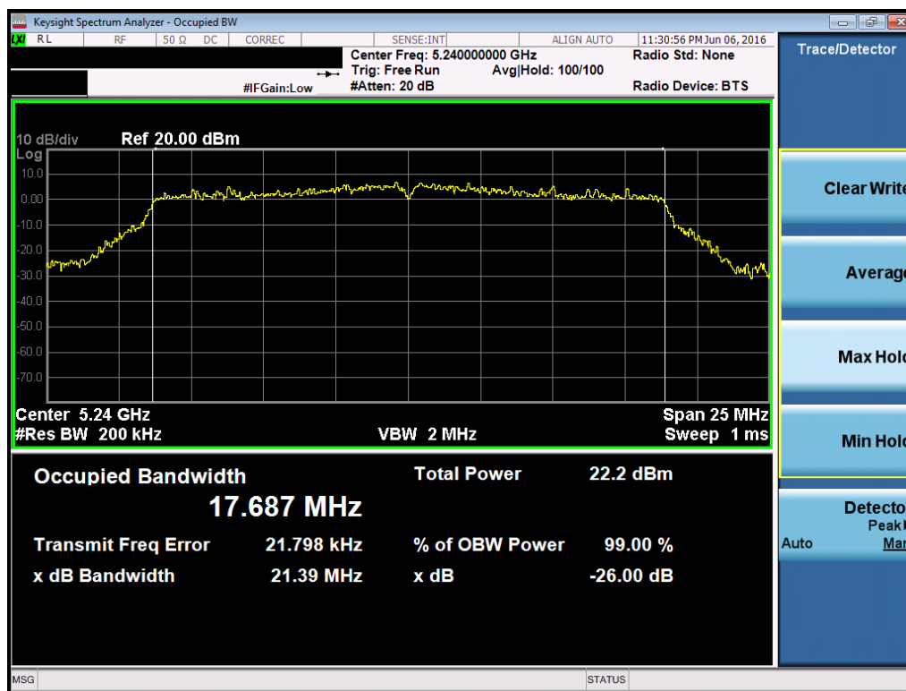
Plot 7-34. 26dB Bandwidth Plot (20MHz BW 802.11n (UNII Band 1) – Ch. 48)
