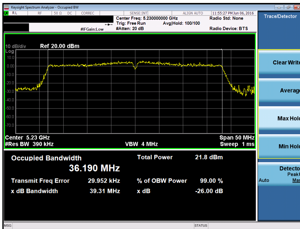
Plot 7-36. 26dB Bandwidth Plot (40MHz BW 802.11n (UNII Band 1) – Ch. 46)
