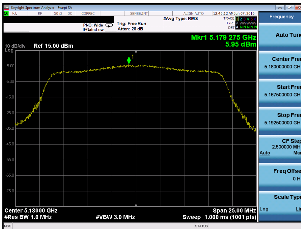
Plot 7-78. Power Spectral Density Plot (20MHz BW 802.11n (UNII Band 1) – Ch. 36)
