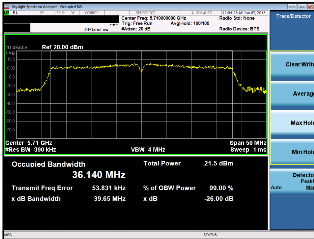
Plot 7-55. 26dB Bandwidth Plot (40MHz BW 802.11n (UNII Band 2C) – Ch. 142)
