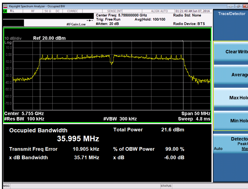
Plot 7-63. 6dB Bandwidth Plot (40MHz BW 802.11n (UNII Band 3) – Ch. 151)
