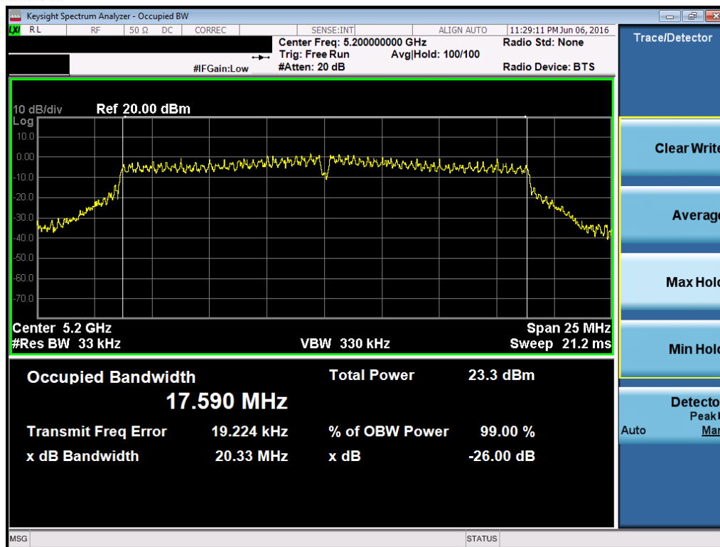
Plot 7-33. 26dB Bandwidth Plot (20MHz BW 802.11n (UNII Band 1) – Ch. 40)
