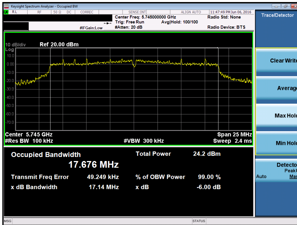
Plot 7-69. 6dB Bandwidth Plot (20MHz BW 802.11n (UNII Band 3) – Ch. 149)
