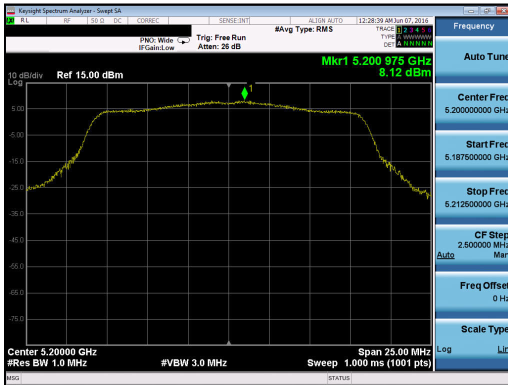
Plot 7-76. Power Spectral Density Plot (802.11a (UNII Band 1) – Ch. 40)
