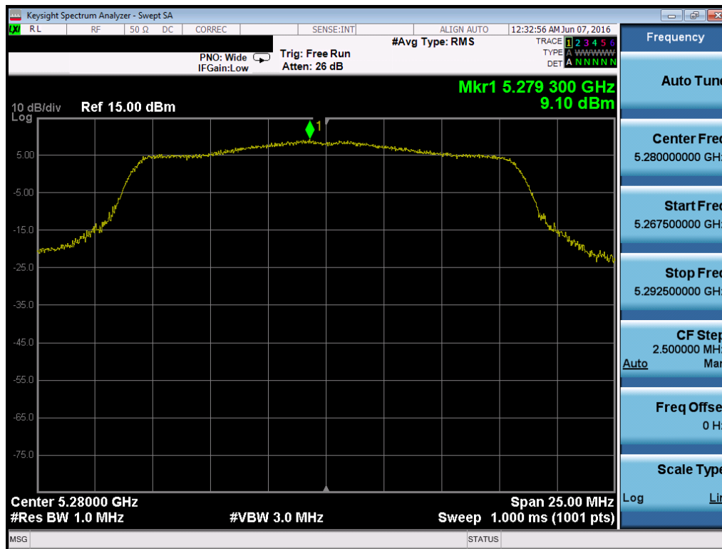
Plot 7-85. Power Spectral Density Plot (802.11a (UNII Band 2A) – Ch. 56)
