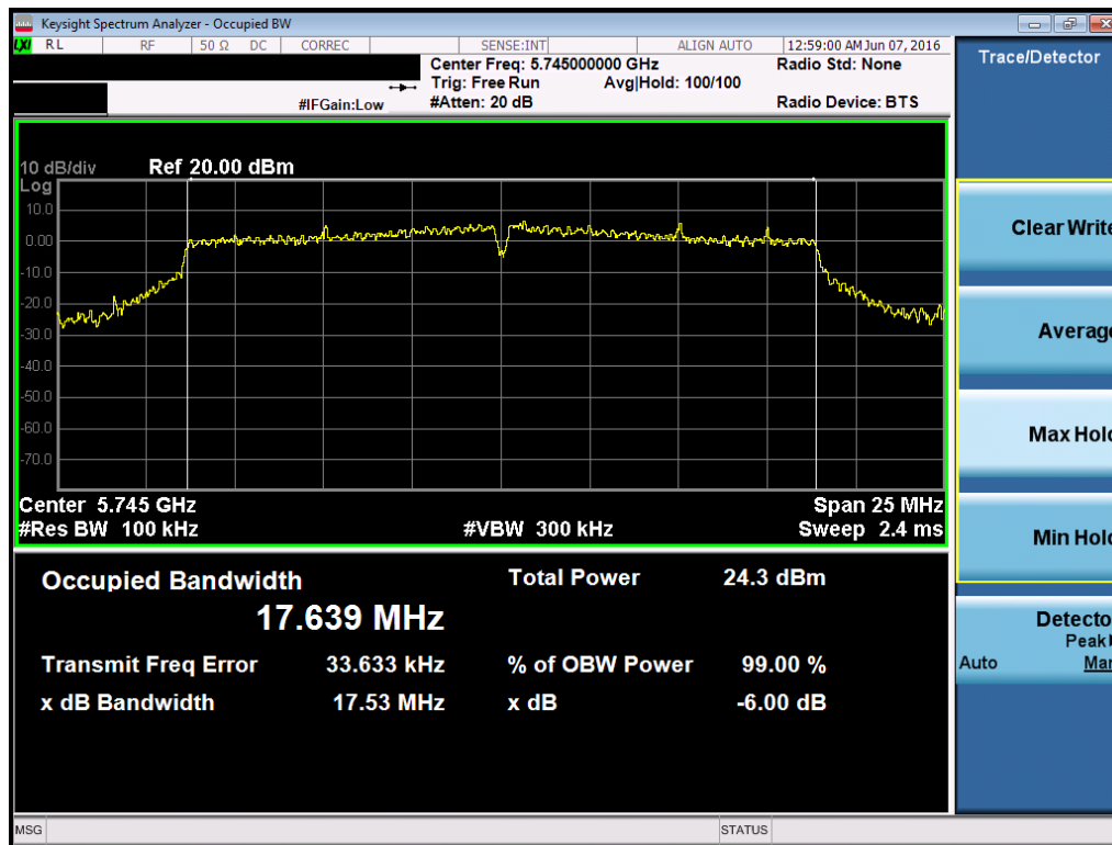
Plot 7-60. 6dB Bandwidth Plot (20MHz BW 802.11n (UNII Band 3) – Ch. 149)
