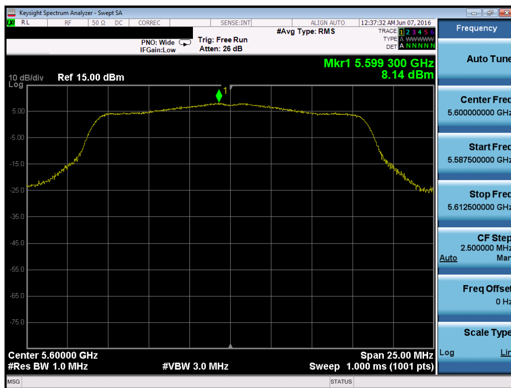
Plot 7-94. Power Spectral Density Plot (802.11a (UNII Band 2C) – Ch. 120)
