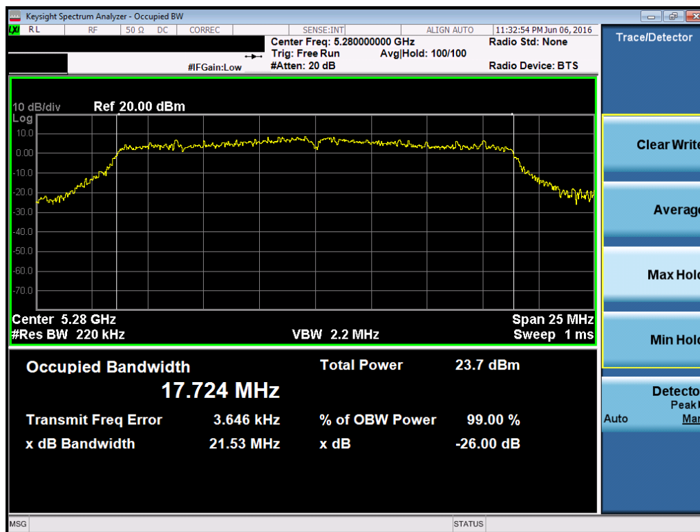
Plot 7-42. 26dB Bandwidth Plot (20MHz BW 802.11n (UNII Band 2A) – Ch. 56)
