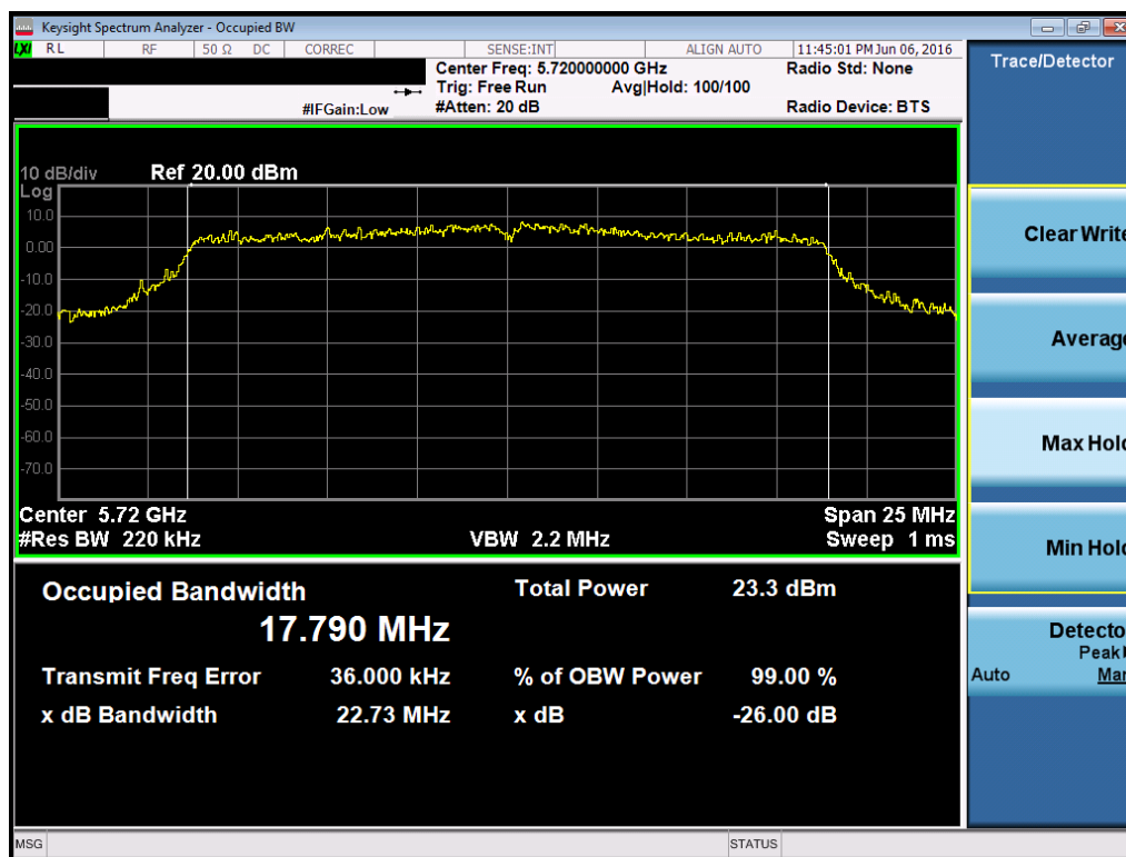
Plot 7-52. 26dB Bandwidth Plot (20MHz BW 802.11n (UNII Band 2C) – Ch. 144)
