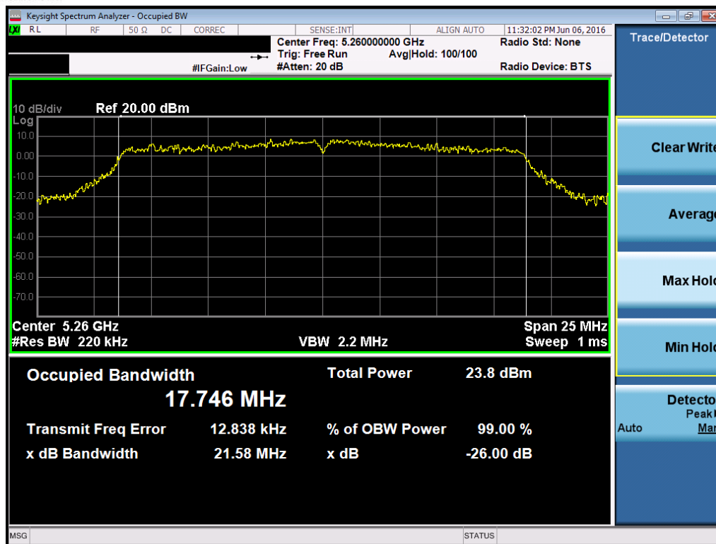
Plot 7-41. 26dB Bandwidth Plot (20MHz BW 802.11n (UNII Band 2A) – Ch. 52)
