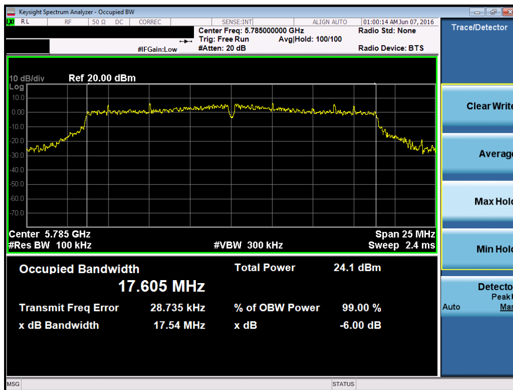
Plot 7-61. 6dB Bandwidth Plot (20MHz BW 802.11n (UNII Band 3) – Ch. 157)
