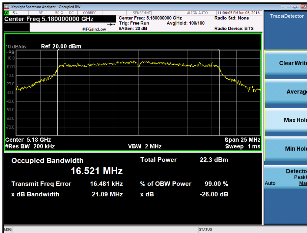
Plot 7-29. 26dB Bandwidth Plot (802.11a (UNII Band 1) – Ch. 36)
