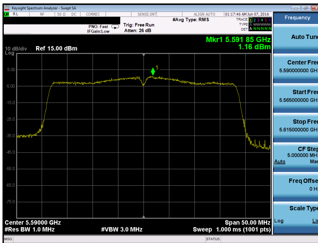
Plot 7-100. Power Spectral Density Plot (40MHz BW 802.11n (UNII Band 2C) – Ch. 118)
