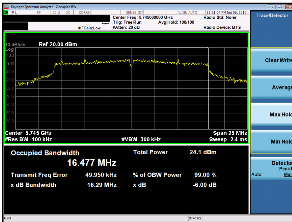
Plot 7-66. 6dB Bandwidth Plot (802.11a (UNII Band 3) – Ch. 149)
