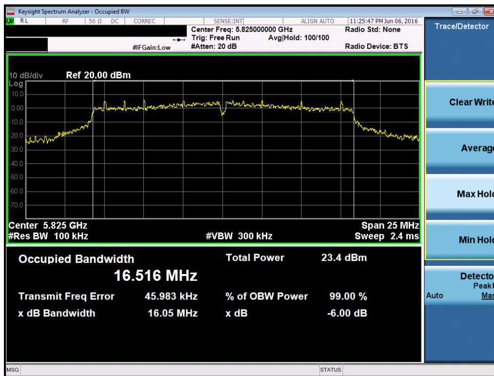
Plot 7-68. 6dB Bandwidth Plot (802.11a (UNII Band 3) – Ch. 165)
