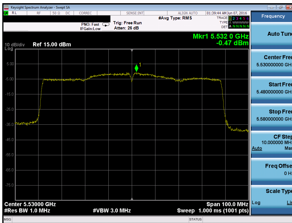
Plot 7-102. Power Spectral Density Plot (80MHz BW 802.11ac (UNII Band 2C) – Ch. 106)
