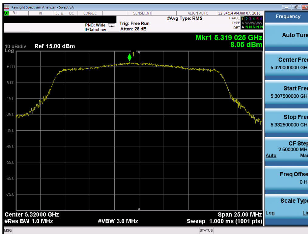
Plot 7-86. Power Spectral Density Plot (802.11a (UNII Band 2A) – Ch. 64)
