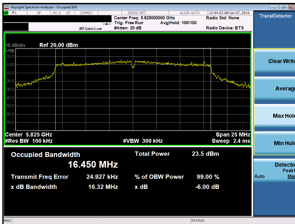
Plot 7-59. 6dB Bandwidth Plot (802.11a (UNII Band 3) – Ch. 165)
