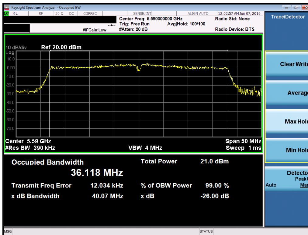
Plot 7-54. 26dB Bandwidth Plot (40MHz BW 802.11n (UNII Band 2C) – Ch. 118)
