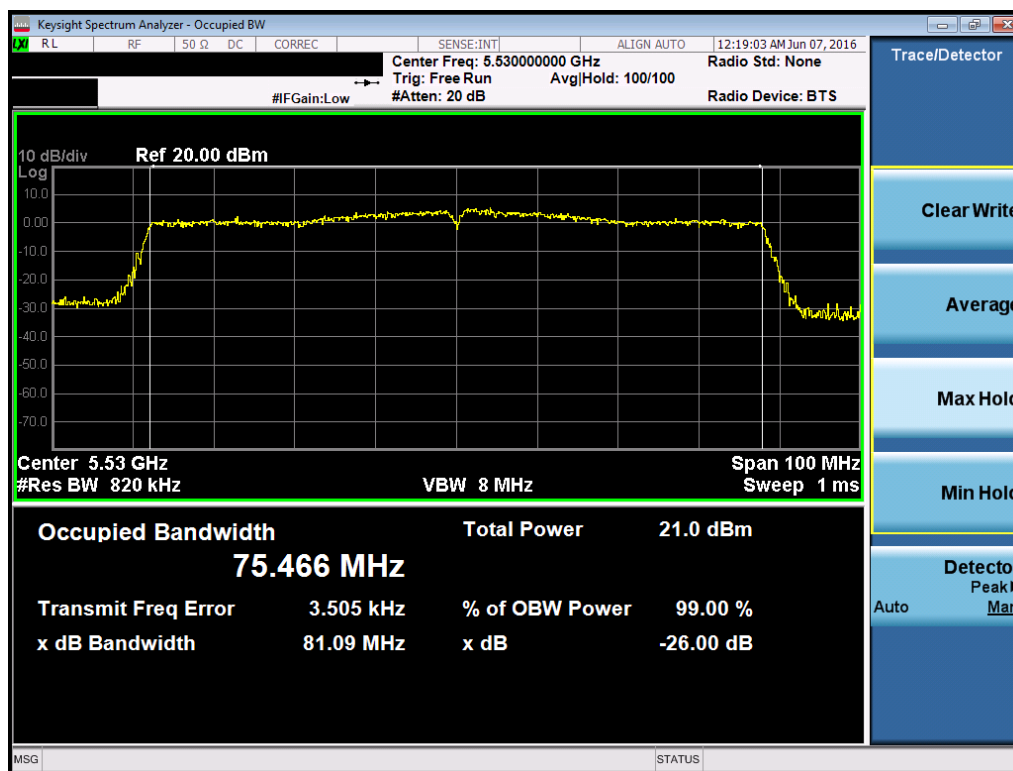
Plot 7-56. 26dB Bandwidth Plot (80MHz BW 802.11ac (UNII Band 2C) – Ch. 106)
