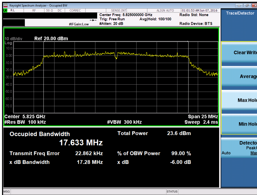
Plot 7-62. 6dB Bandwidth Plot (20MHz BW 802.11n (UNII Band 3) – Ch. 165)
