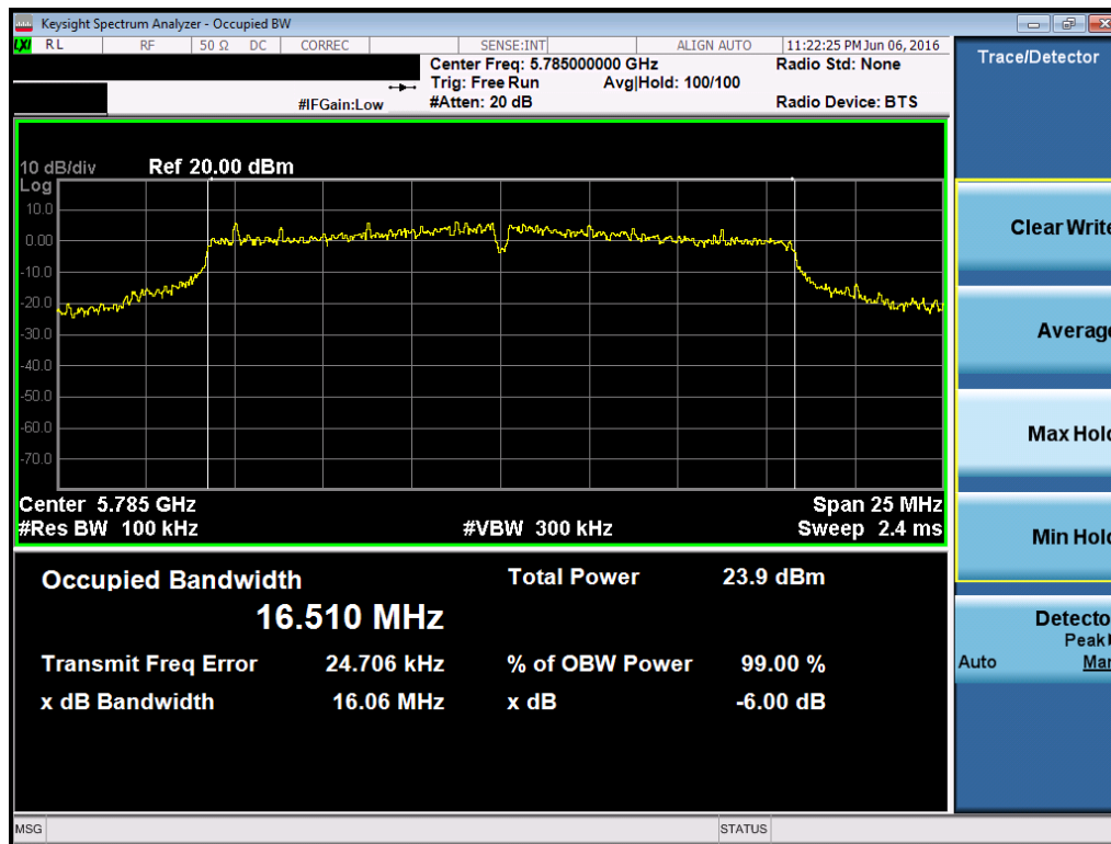
Plot 7-67. 6dB Bandwidth Plot (802.11a (UNII Band 3) – Ch. 157)
