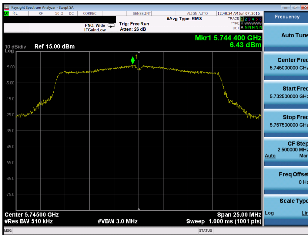
Plot 7-105. Power Spectral Density Plot (802.11a (UNII Band 3) – Ch. 149)
