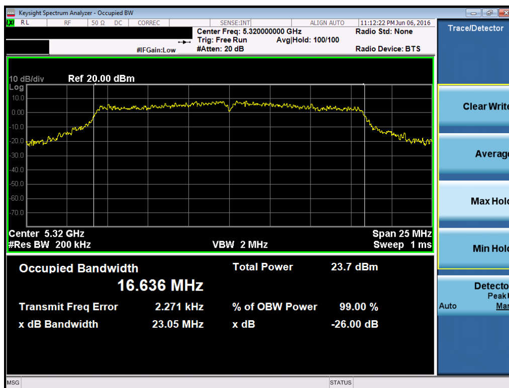
Plot 7-40. 26dB Bandwidth Plot (802.11a (UNII Band 2A) – Ch. 64)
