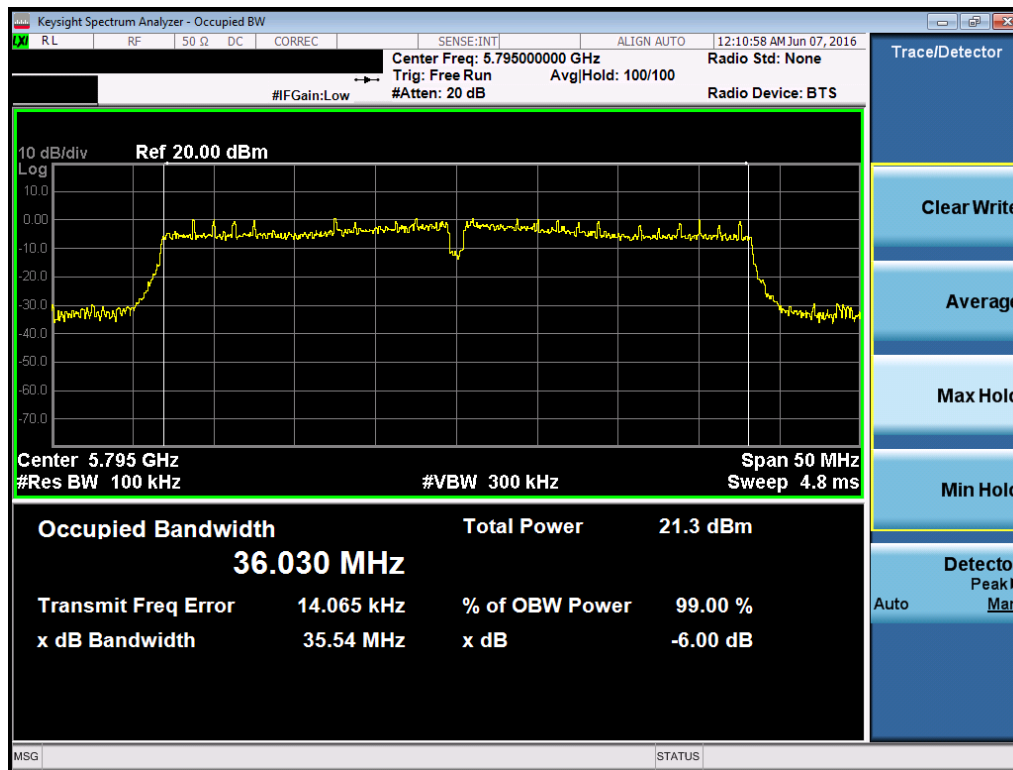
Plot 7-73. 6dB Bandwidth Plot (40MHz BW 802.11n (UNII Band 3) – Ch. 159)
