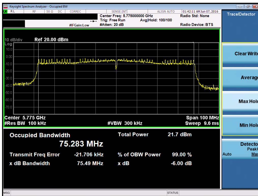
Plot 7-65. 6dB Bandwidth Plot (80MHz BW 802.11ac (UNII Band 3) – Ch. 155)
