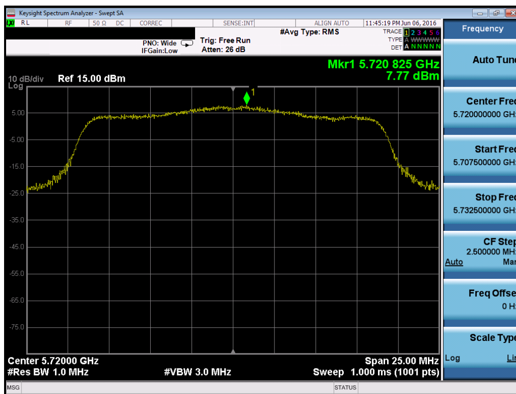
Plot 7-137. Power Spectral Density Plot (20MHz BW 802.11n (UNII Band 2C) – Ch. 144)
