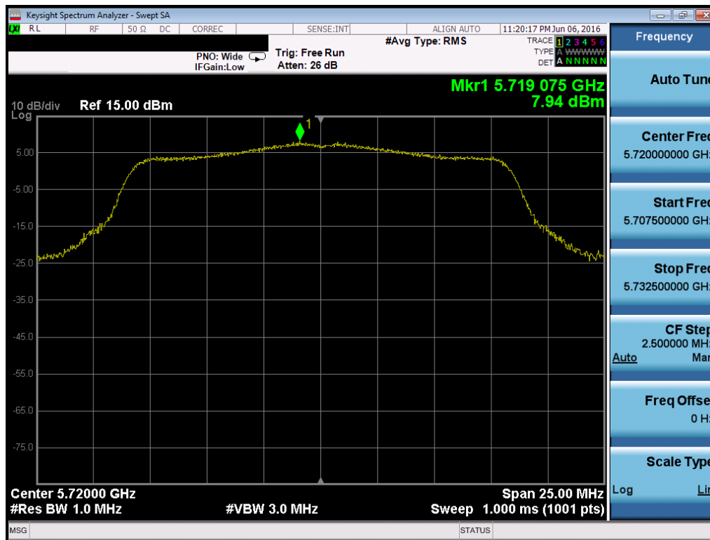
Plot 7-134. Power Spectral Density Plot (802.11a (UNII Band 2C) – Ch. 144)
