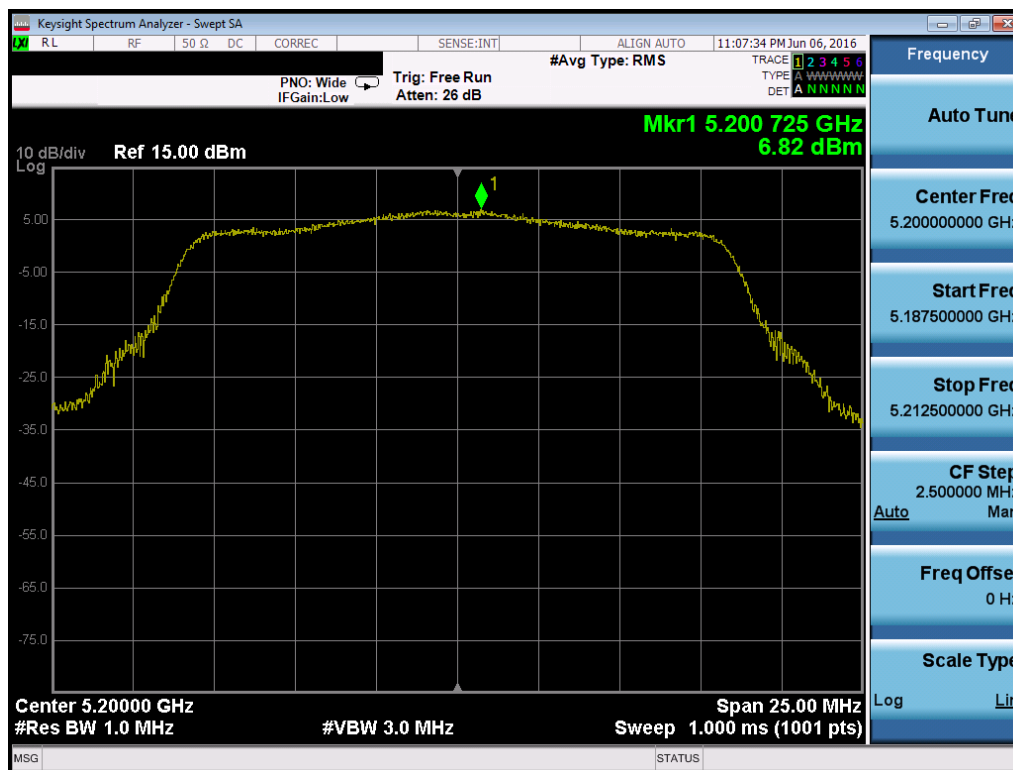
Plot 7-115. Power Spectral Density Plot (802.11a (UNII Band 1) – Ch. 40)
