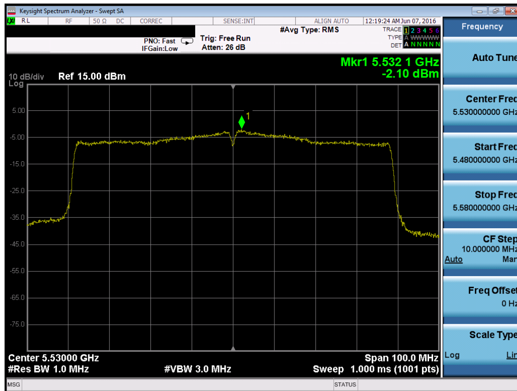
Plot 7-141. Power Spectral Density Plot (80MHz BW 802.11ac (UNII Band 2C) – Ch. 106)
