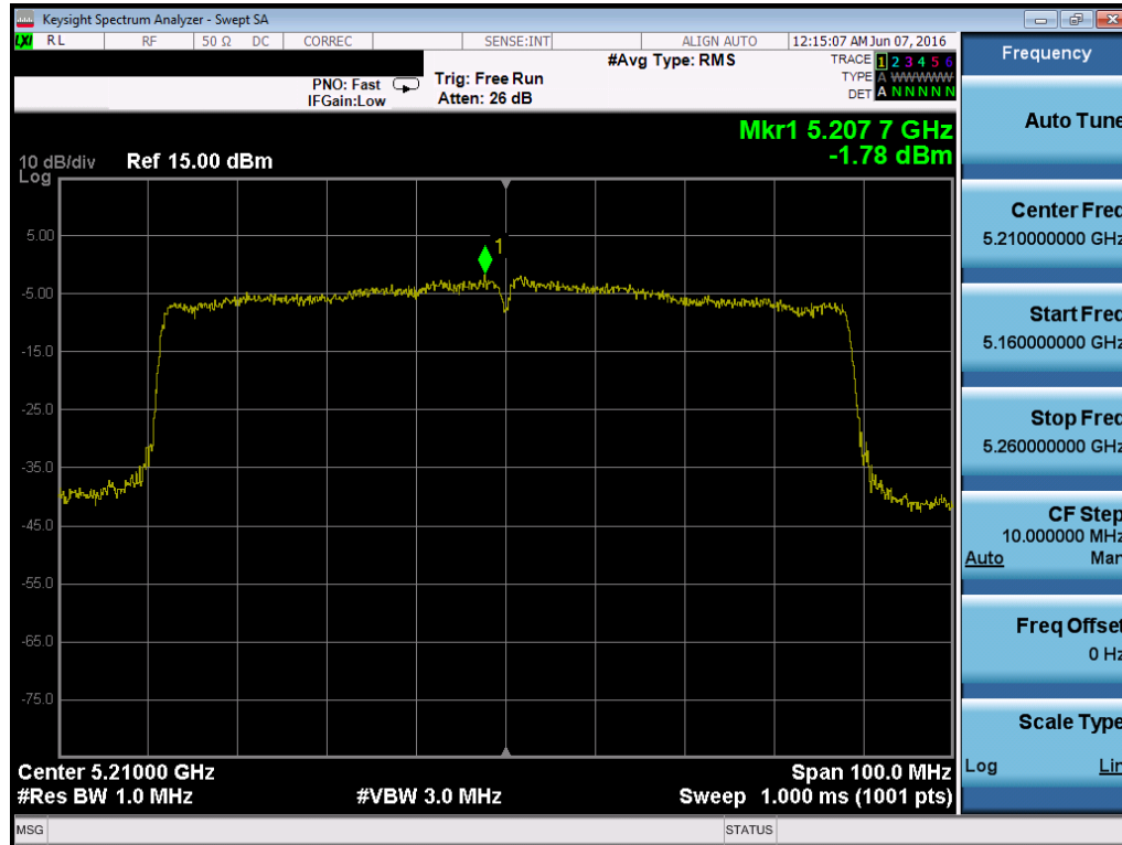
Plot 7-122. Power Spectral Density Plot (80MHz BW 802.11ac (UNII Band 1) – Ch. 42)
