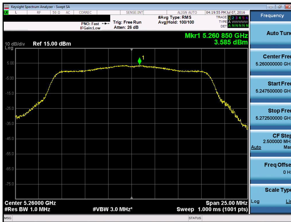
Plot 0 A3-13. Power Spectral Density Plot (802.11a (UNII Band 2A) – Ch. 52)
