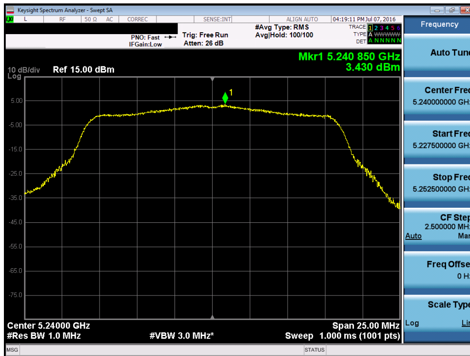
Plot A3-12. Power Spectral Density Plot (802.11a (UNII Band 1) – Ch. 48)
