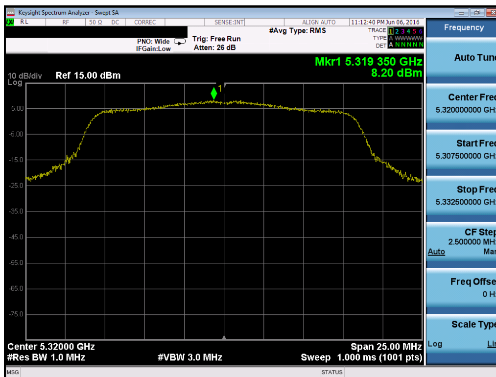
Plot 7-125. Power Spectral Density Plot (802.11a (UNII Band 2A) – Ch. 64)
