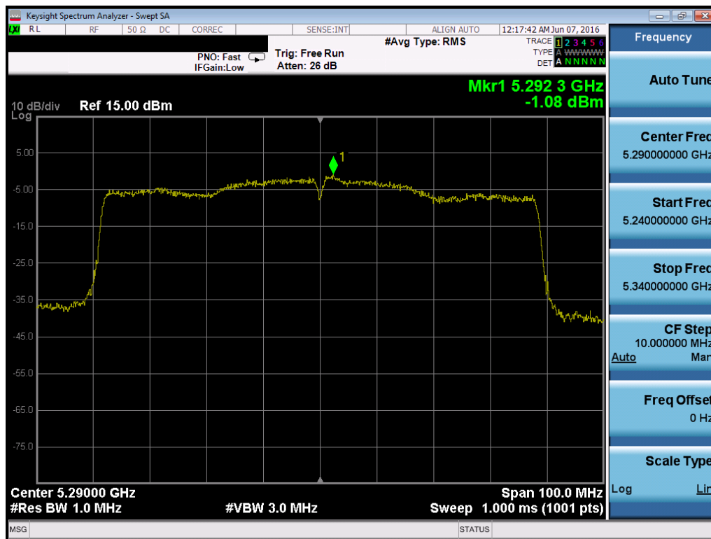
Plot 7-131. Power Spectral Density Plot (80MHz BW 802.11ac (UNII Band 2A) – Ch. 58)
