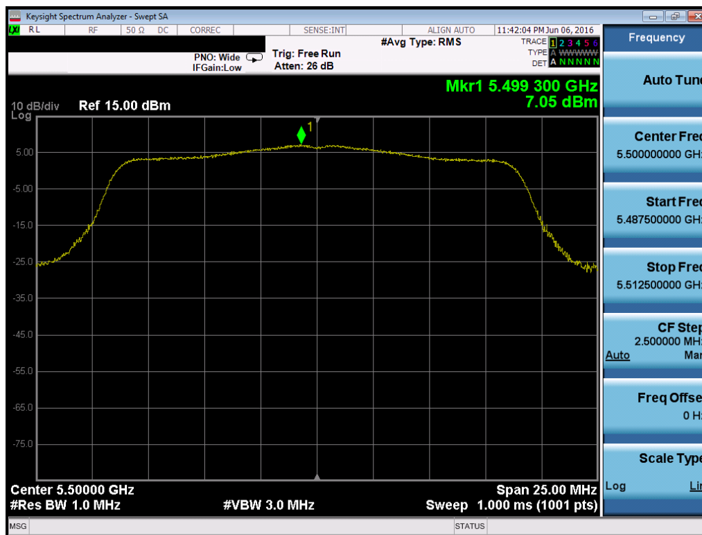
Plot 7-135. Power Spectral Density Plot (20MHz BW 802.11n (UNII Band 2C) – Ch. 100)
