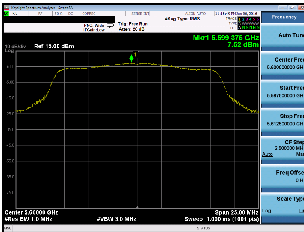
Plot 7-133. Power Spectral Density Plot (802.11a (UNII Band 2C) – Ch. 120)
