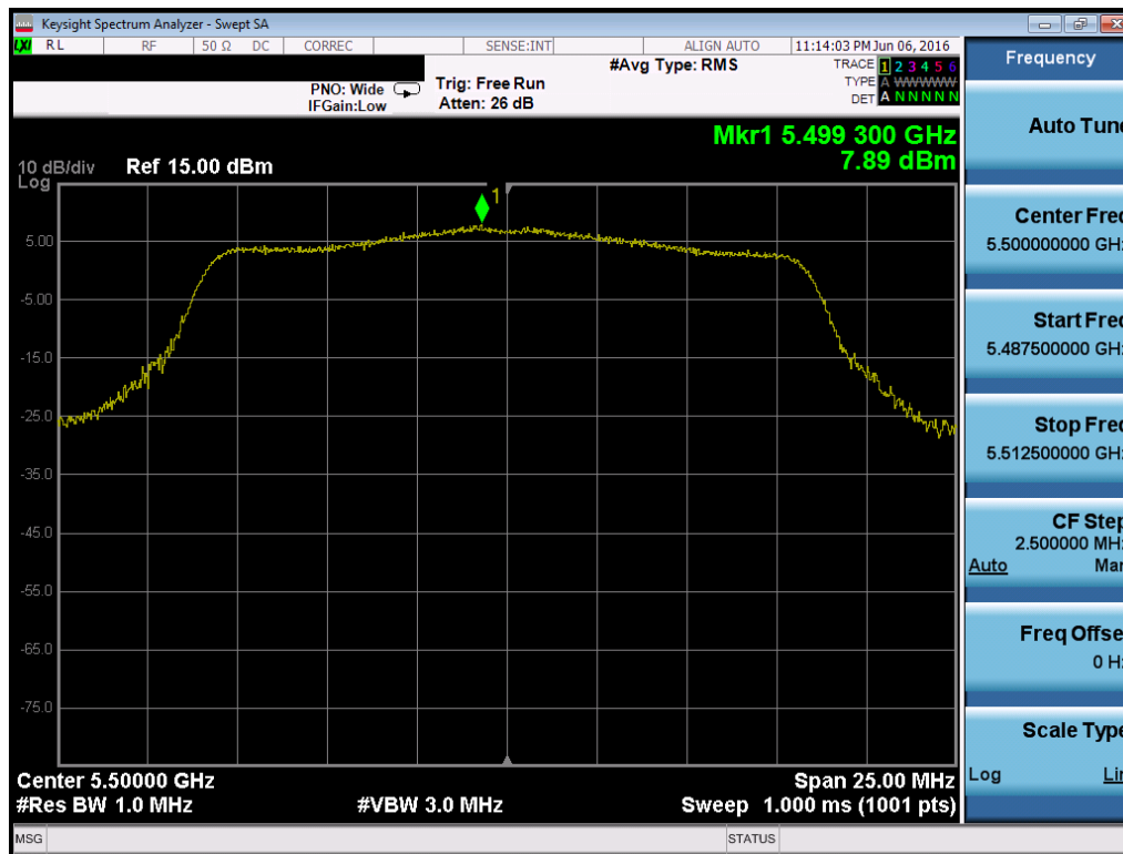
Plot 7-132. Power Spectral Density Plot (802.11a (UNII Band 2C) – Ch. 100)
