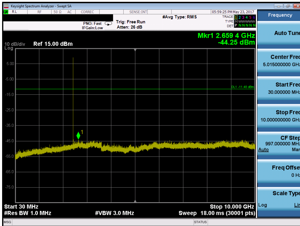
Plot 7-29. Conducted Spurious Plot (Bluetooth (LE), 2Mbps – Ch. 19)
