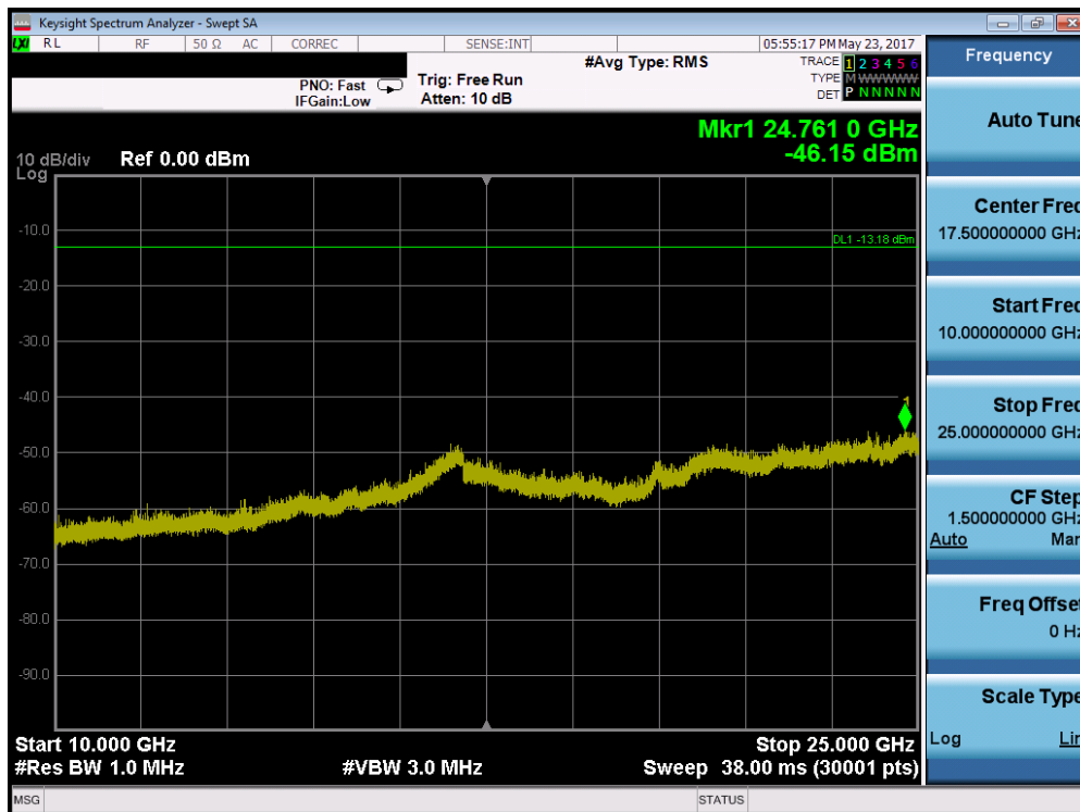
Plot 7-28. Conducted Spurious Plot (Bluetooth (LE), 2Mbps – Ch. 0)
