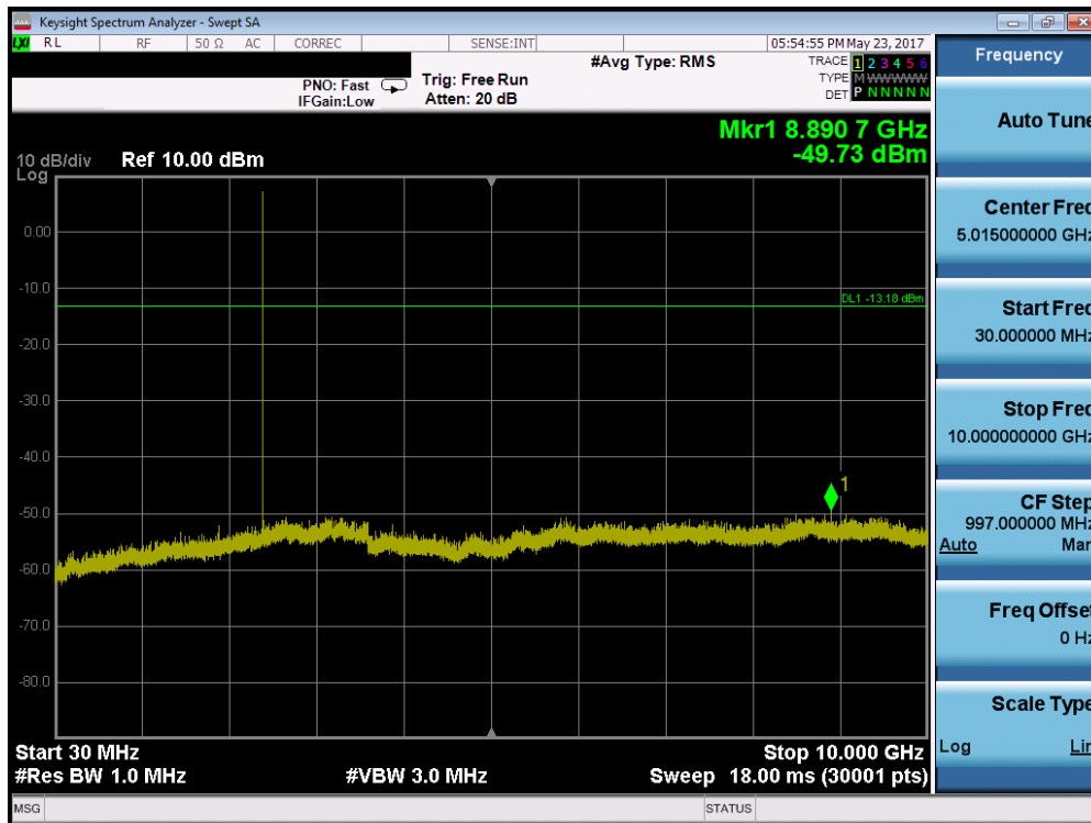
Plot 7-27. Conducted Spurious Plot (Bluetooth (LE), 2Mbps – Ch. 0)
