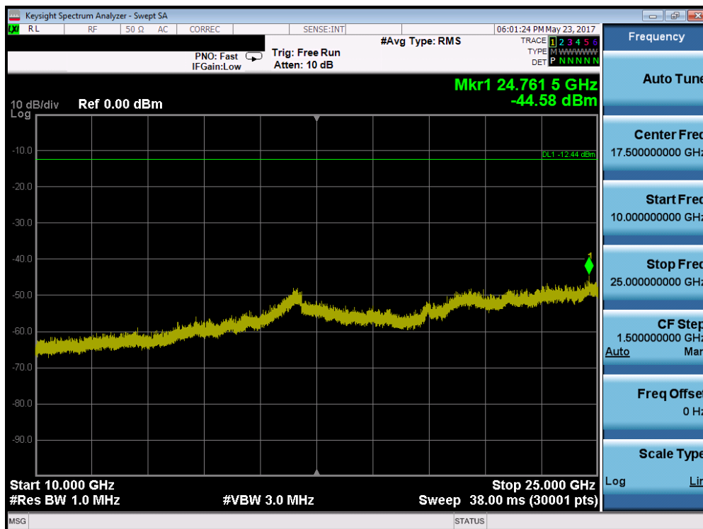
Plot 7-32. Conducted Spurious Plot (Bluetooth (LE), 2Mbps – Ch. 39)
