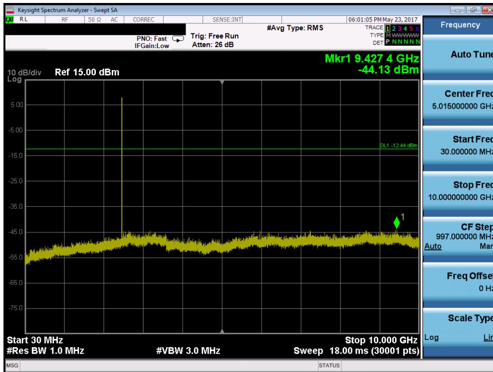
Plot 7-31. Conducted Spurious Plot (Bluetooth (LE), 2Mbps – Ch. 39)
