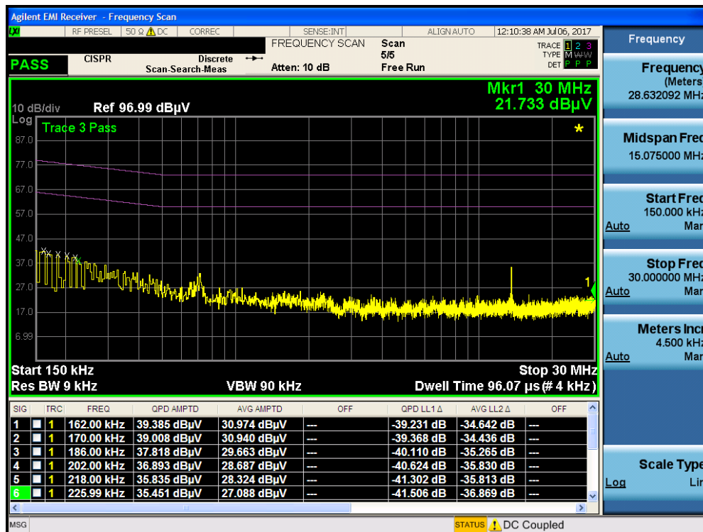
Plot 7-4. Line-Conducted Test Plot, RFID Antenna Terminated in 50Ω (N)
