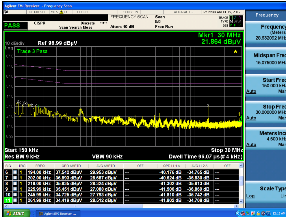
Plot 7-3. Line-Conducted Test Plot, RFID Antenna Terminated in 50Ω (L1)
