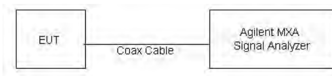
Figure 9-5 Power Measurement Setup for Bandwidths > 50 MHz
