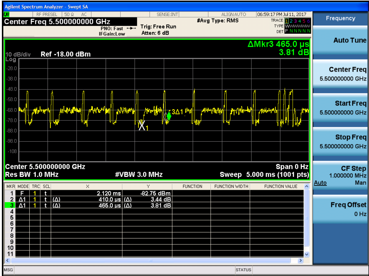
Figure 5-2. Band 2C Channel Loading
