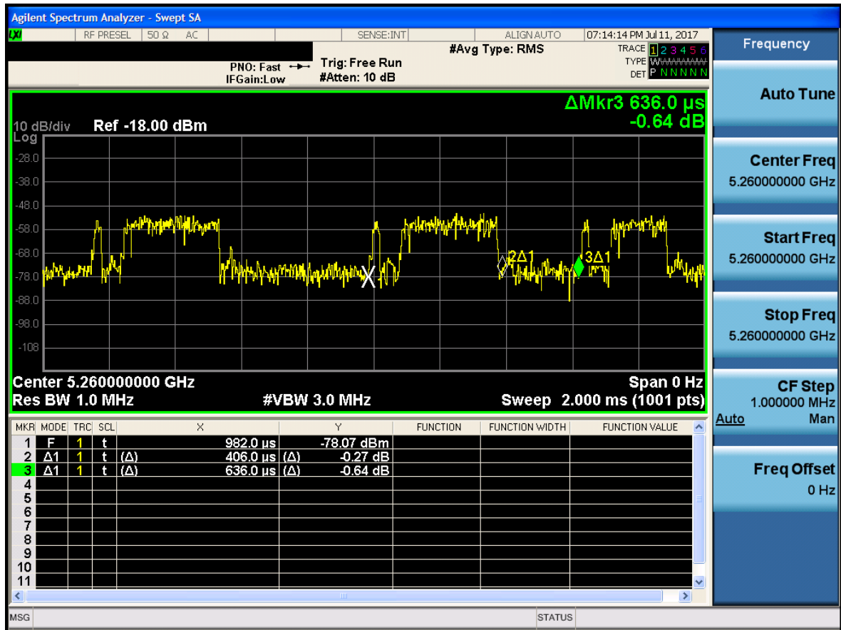
Figure 5-1. Band 2A Channel Loading
