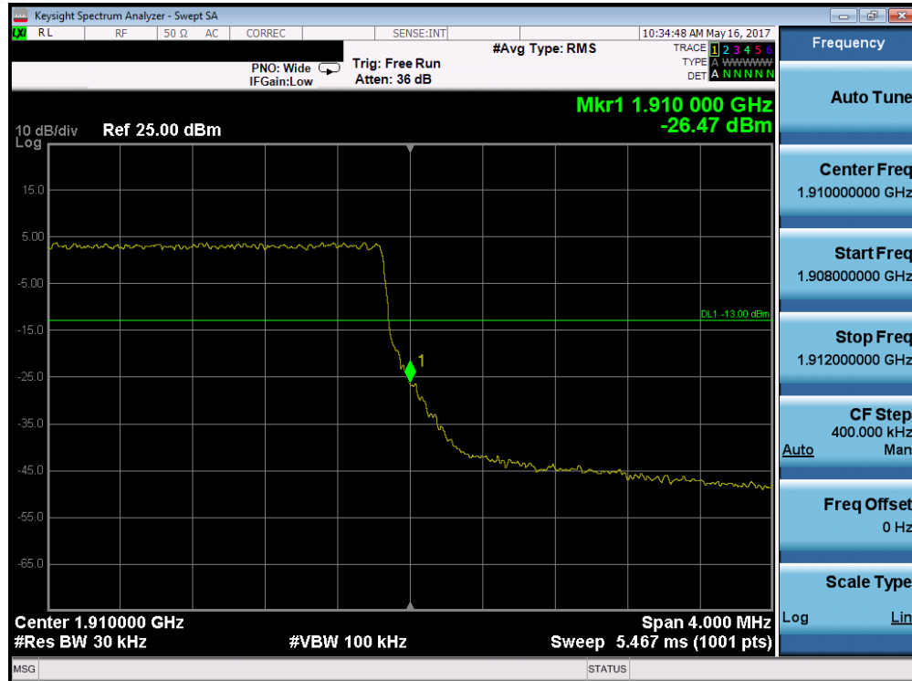
Plot 7-219. Upper Band Edge Plot (Band 2 – 3.0MHz QPSK – RB Size 15)
