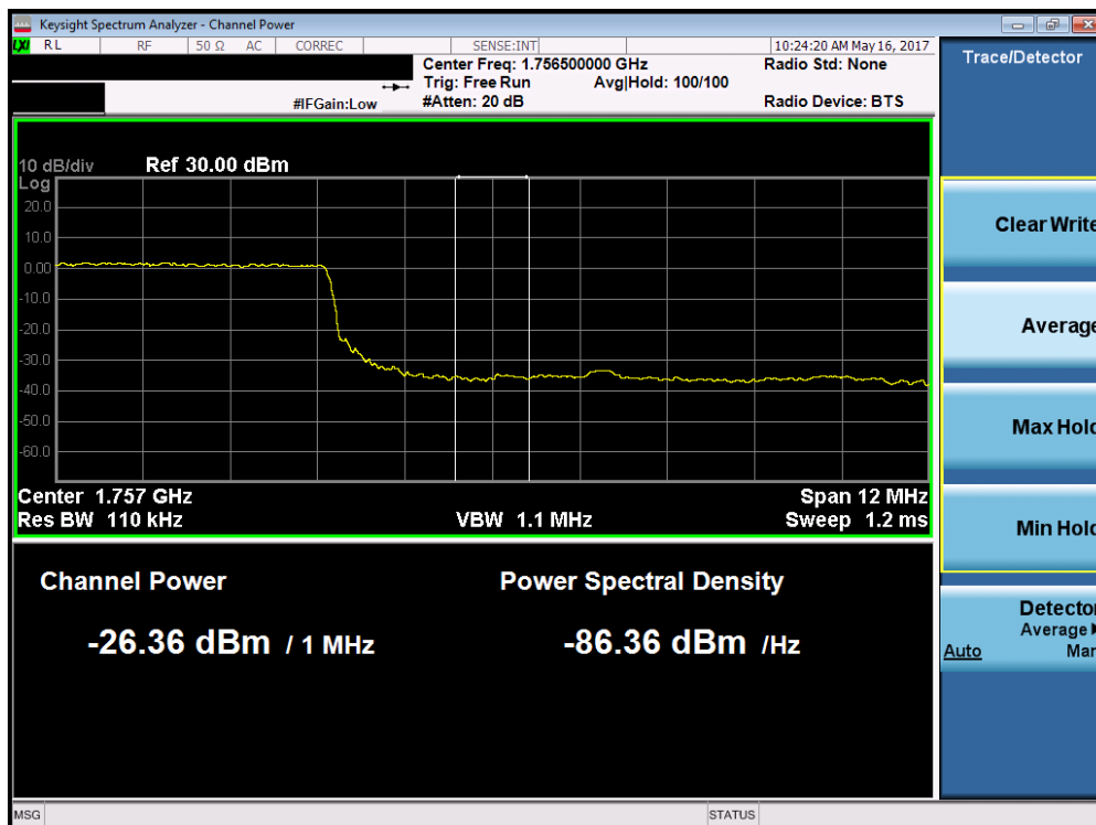
Plot 7-196. Upper Extended Band Edge Plot (Band 4 – 15.0MHz QPSK – RB Size 75)
