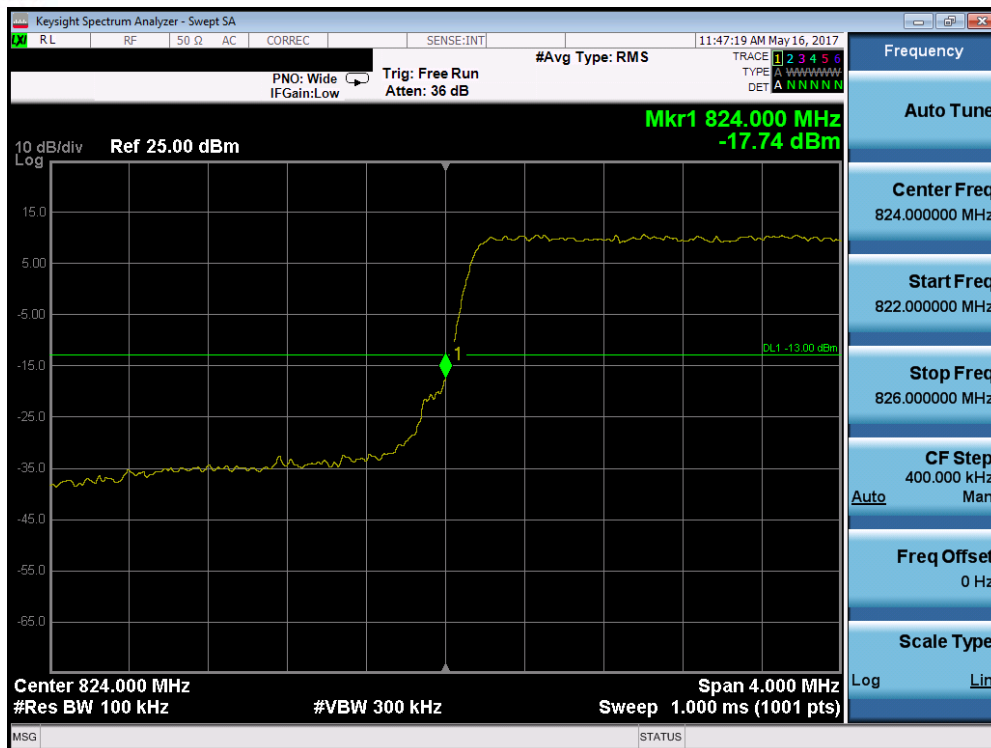
Plot 7-169. Lower Band Edge Plot (Band 5/26 - 3.0MHz QPSK - RB Size 15)
