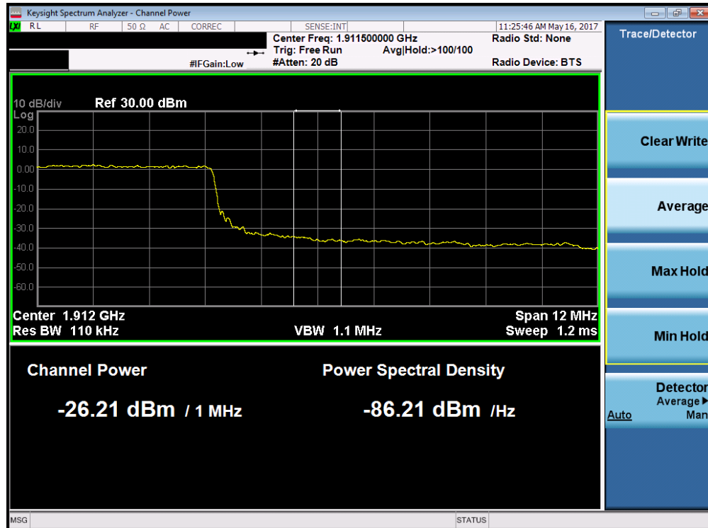
Plot 7-232. Upper Extended Band Edge Plot (Band 2 – 15.0MHz QPSK – RB Size 75)
