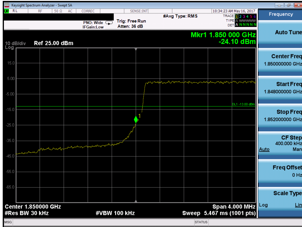
Plot 7-217. Lower Band Edge Plot (Band 2/25 – 3.0MHz QPSK – RB Size 15)
