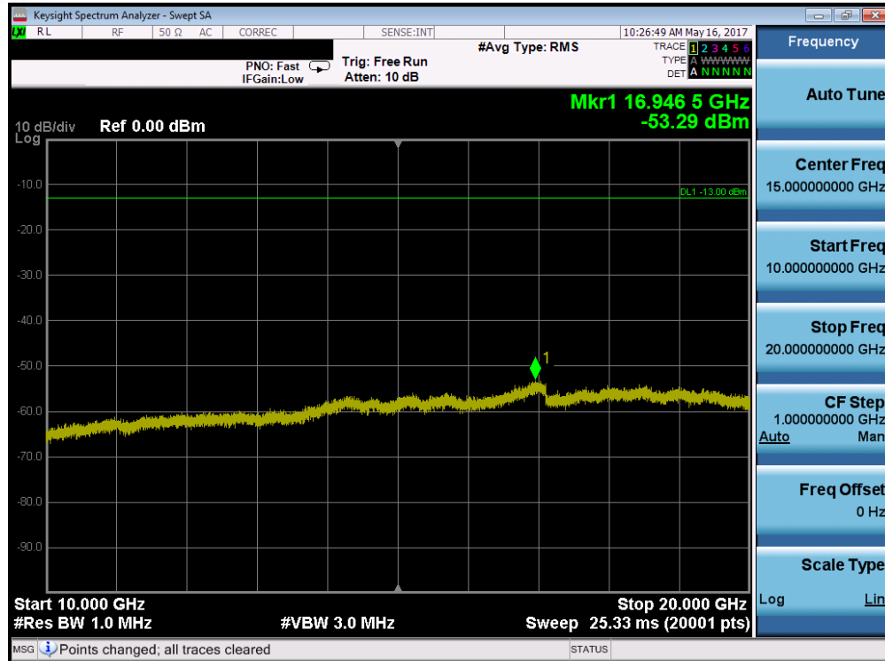
Plot 7-126. Conducted Spurious Plot (Band 2/25 – 20.0MHz QPSK – RB Size 1, RB Offset 0 – Low Channel)
