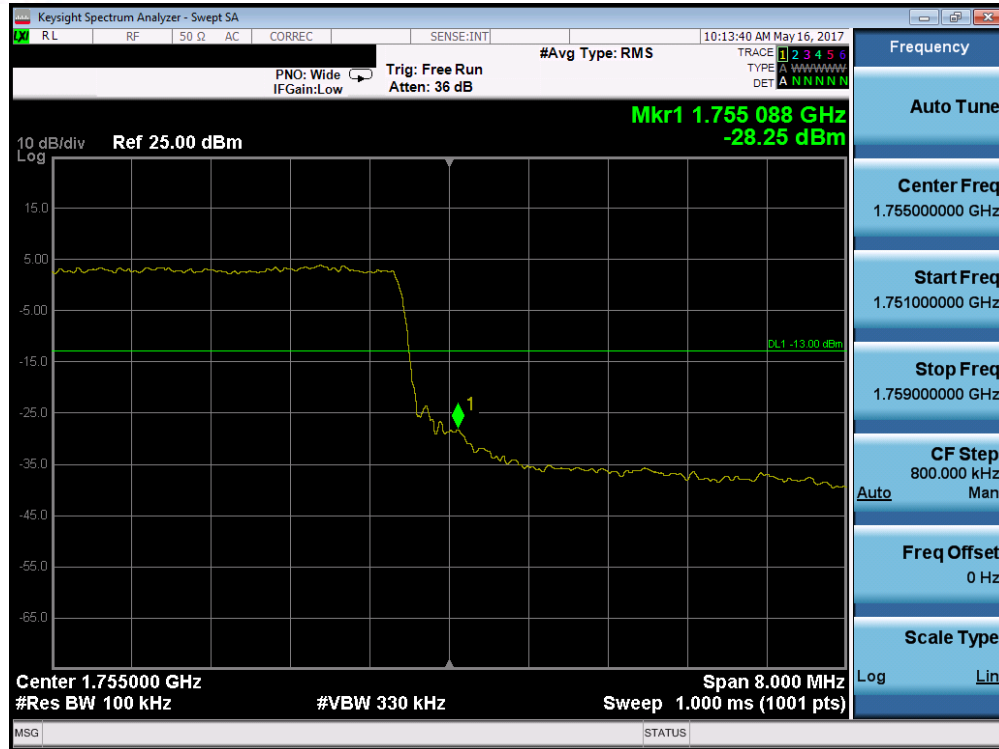
Plot 7-191. Upper Band Edge Plot (Band 4 – 10.0MHz QPSK – RB Size 50)
