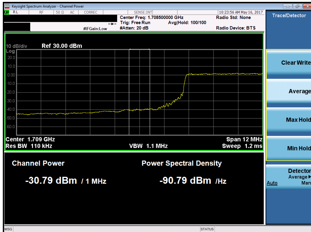
Plot 7-194. Lower Extended Band Edge Plot (Band 4/66 – 15.0MHz QPSK – RB Size 75)
