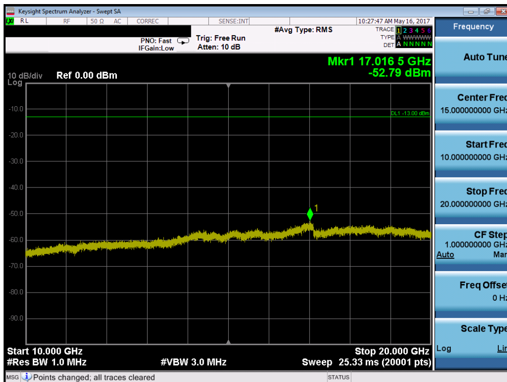
Plot 7-123. Conducted Spurious Plot (Band 4 – 20.0MHz QPSK – RB Size 1, RB Offset 0 – High Channel)
