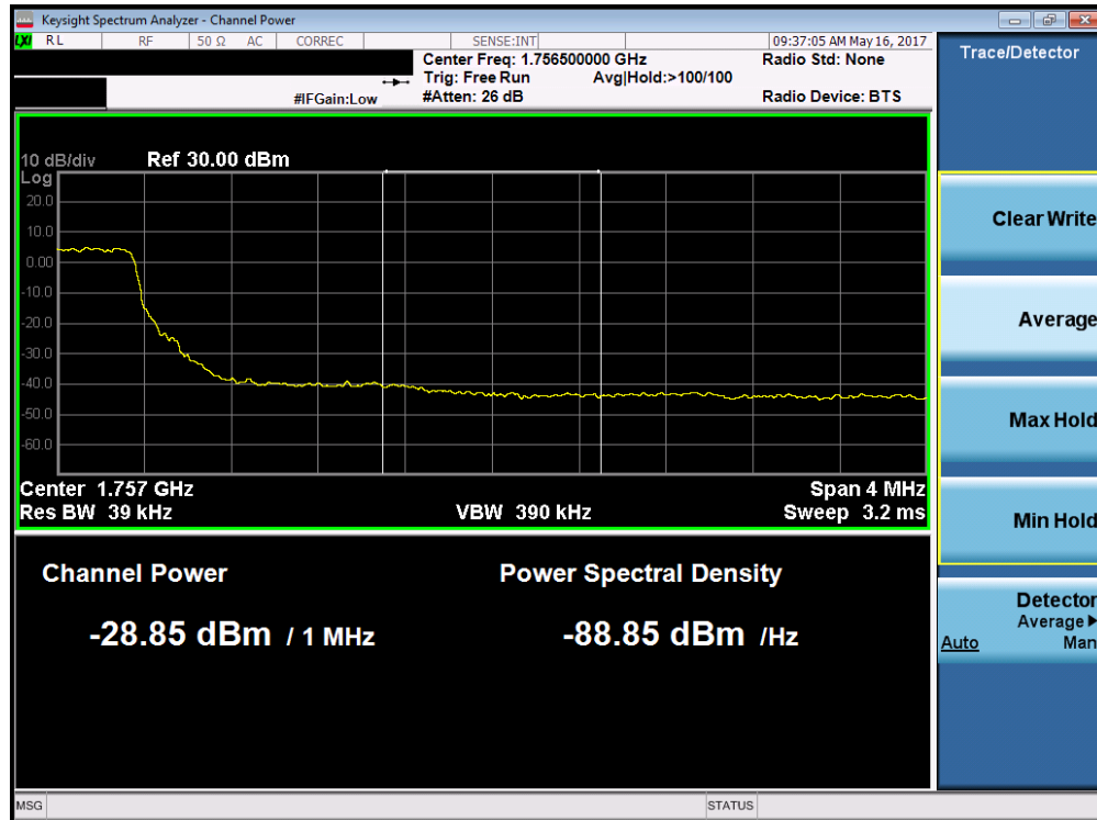
Plot 7-184. Upper Extended Band Edge Plot (Band 4 – 3.0MHz QPSK – RB Size 15)
