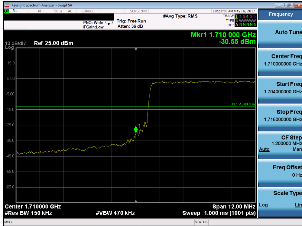
Plot 7-193. Lower Band Edge Plot (Band 4/66 – 15.0MHz QPSK – RB Size 75)
