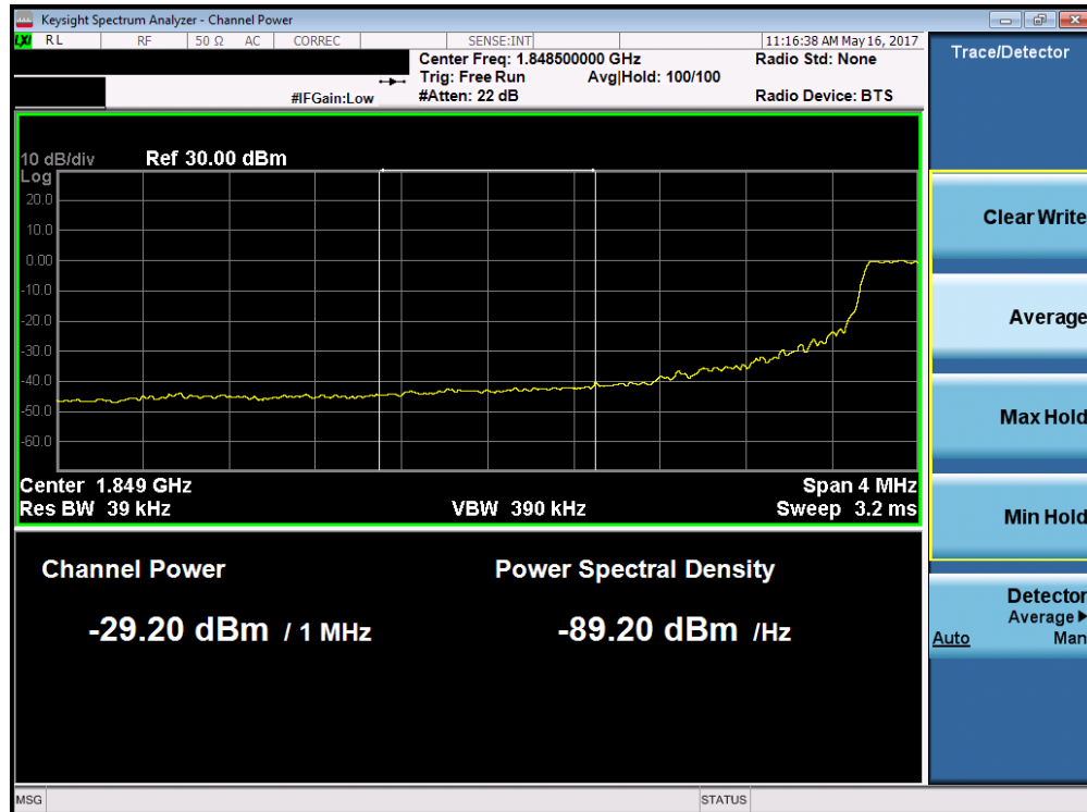
Plot 7-222. Lower Extended Band Edge Plot (Band 2/25 – 5.0MHz QPSK – RB Size 25)
