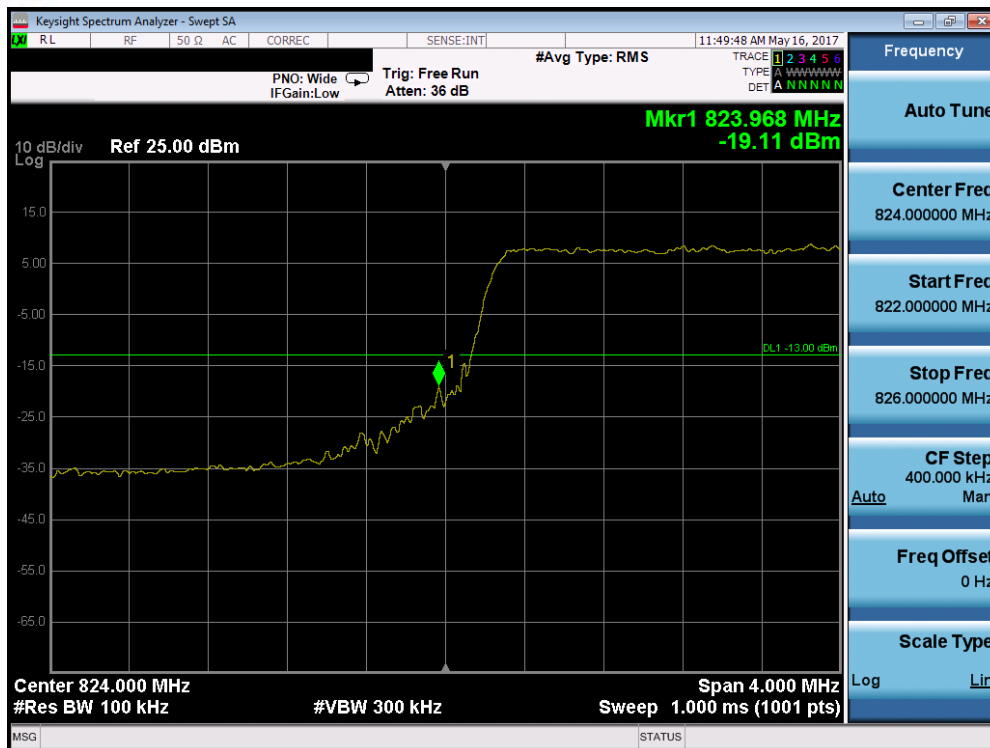
Plot 7-171. Lower Band Edge Plot (Band 5/26 – 5.0MHz QPSK – RB Size 25)
