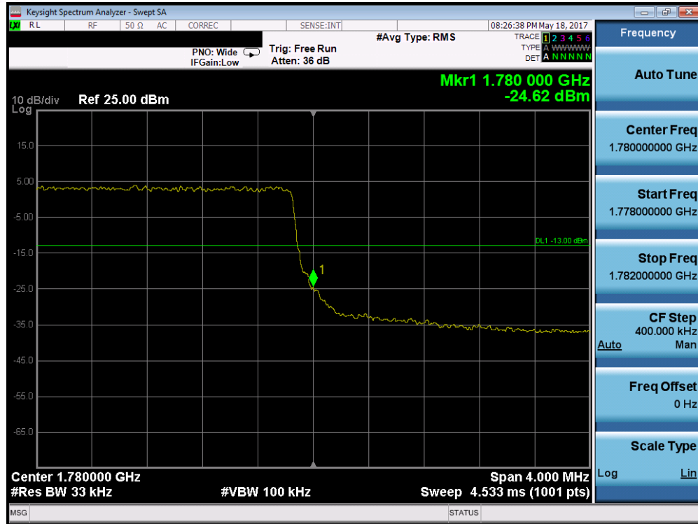
Plot 7-203. Upper Band Edge Plot (Band 66 – 3.0MHz QPSK – RB Size 15)
