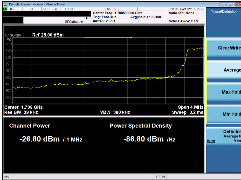
Plot 7-178. Lower Extended Band Edge Plot (Band 4/66 – 1.4MHz QPSK – RB Size 6)
