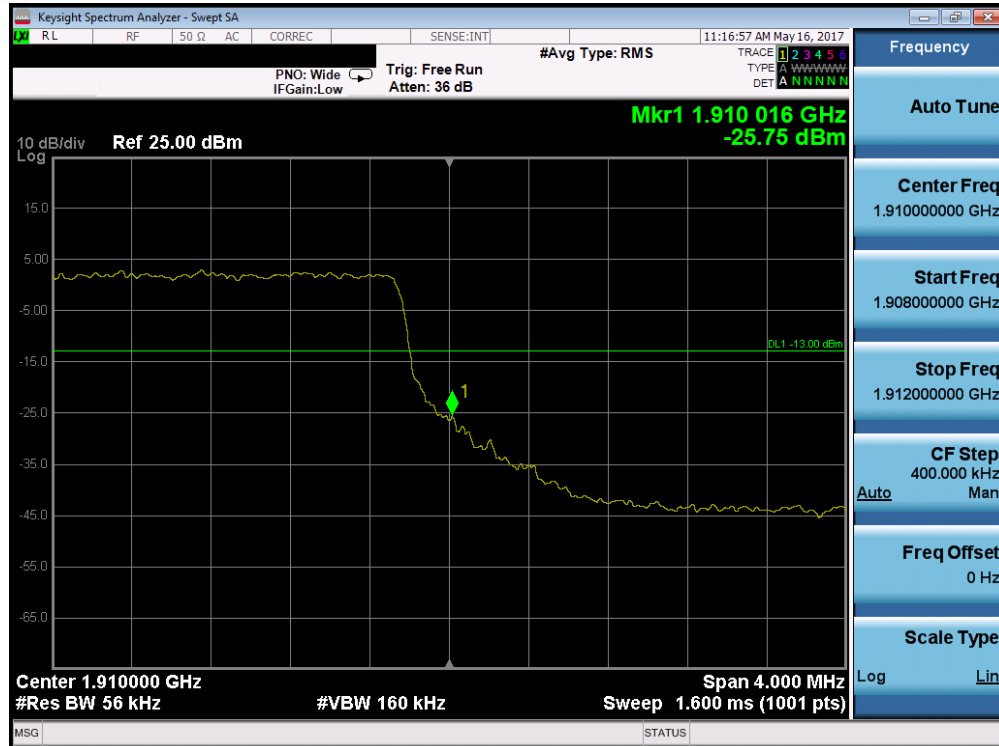
Plot 7-223. Upper Band Edge Plot (Band 2 – 5.0MHz QPSK – RB Size 25)
