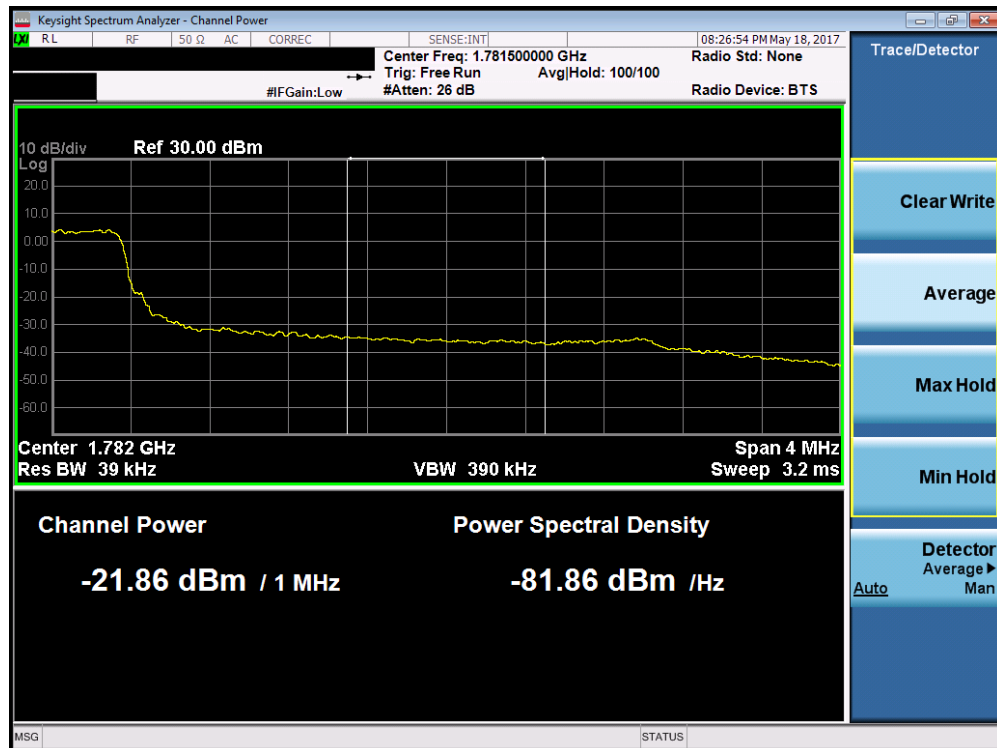
Plot 7-204. Upper Extended Band Edge Plot (Band 66 – 3.0MHz QPSK – RB Size 15)
