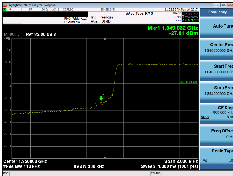
Plot 7-225. Lower Band Edge Plot (Band 2/25 – 10.0MHz QPSK – RB Size 50)
