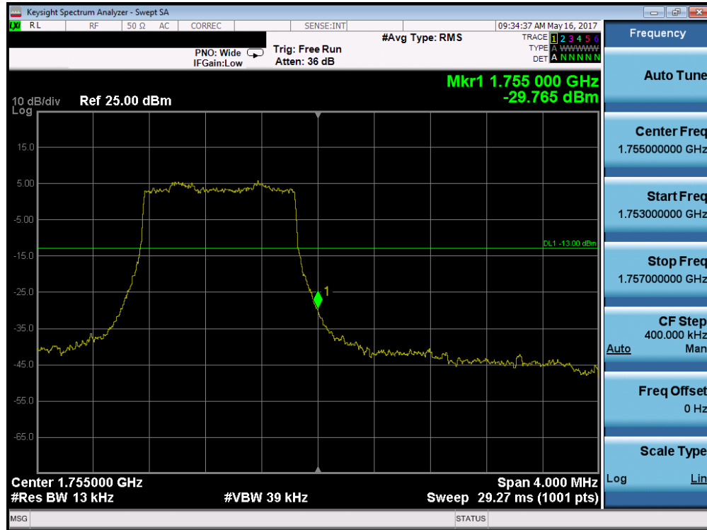
Plot 7-179. Upper Band Edge Plot (Band 4 – 1.4MHz QPSK – RB Size 6)
