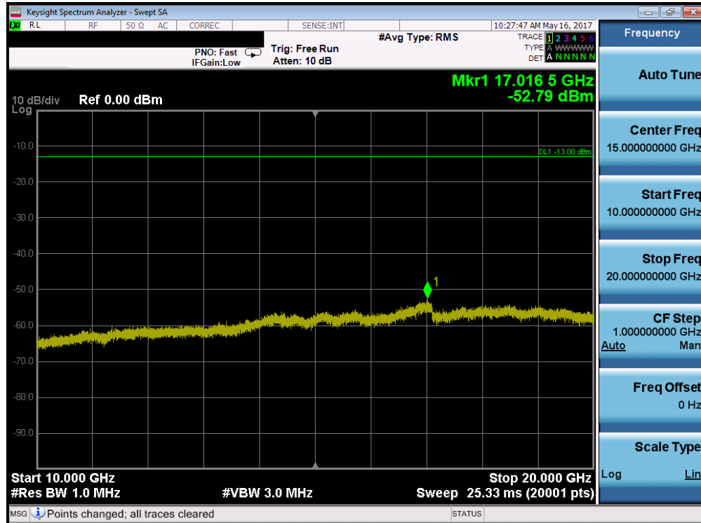
Plot 7-132. Conducted Spurious Plot (Band 2/25 – 20.0MHz QPSK – RB Size 1, RB Offset 0 – High Channel)
