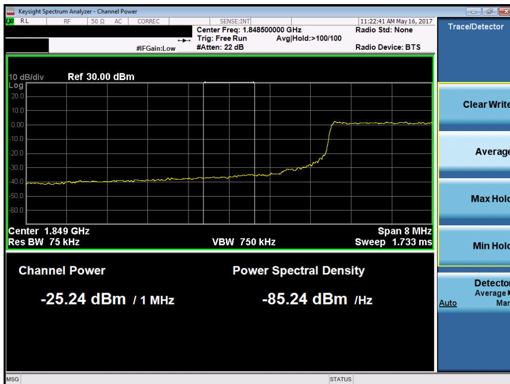
Plot 7-226. Lower Band Edge Plot (Band 2/25 – 10.0MHz QPSK – RB Size 50)
