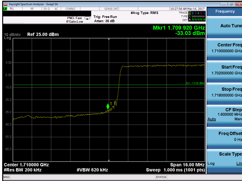
Plot 7-197. Lower Band Edge Plot (Band 4/66 – 20.0MHz QPSK – RB Size 100)
