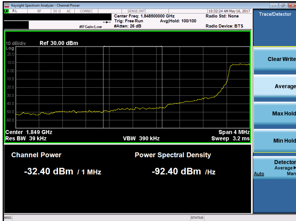
Plot 7-214. Lower Extended Band Edge Plot (Band 2/25 – 1.4MHz QPSK – RB Size 6)
