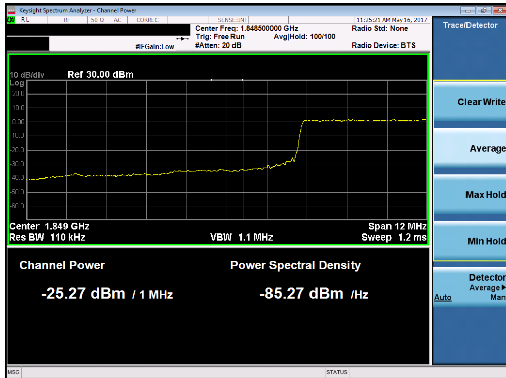
Plot 7-230. Lower Extended Band Edge Plot (Band 2/25 – 15.0MHz QPSK – RB Size 75)
