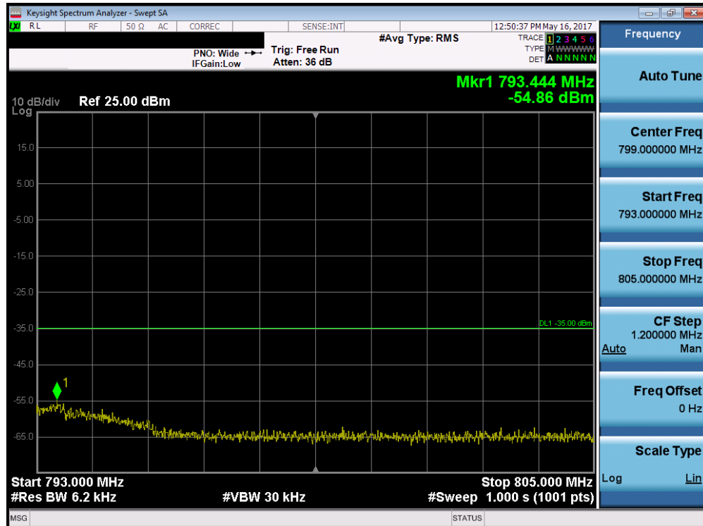
Plot 7-166. Upper Emission Mask Edge Plot (Band 13 – 10.0MHz QPSK – RB Size 50)
