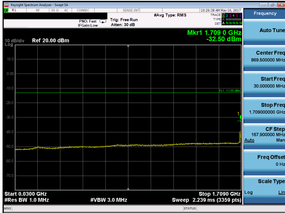
Plot 7-124. Conducted Spurious Plot (Band 2/25 – 20.0MHz QPSK – RB Size 1, RB Offset 0 – Low Channel)
