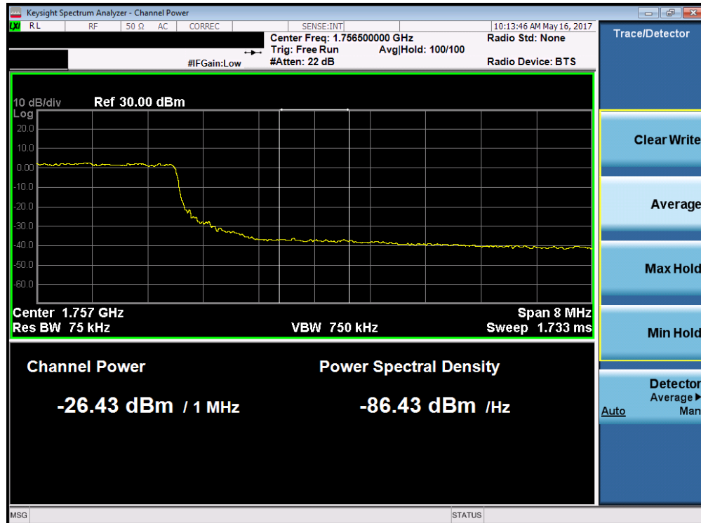
Plot 7-192. Upper Extended Band Edge Plot (Band 4 – 10.0MHz QPSK – RB Size 50)
