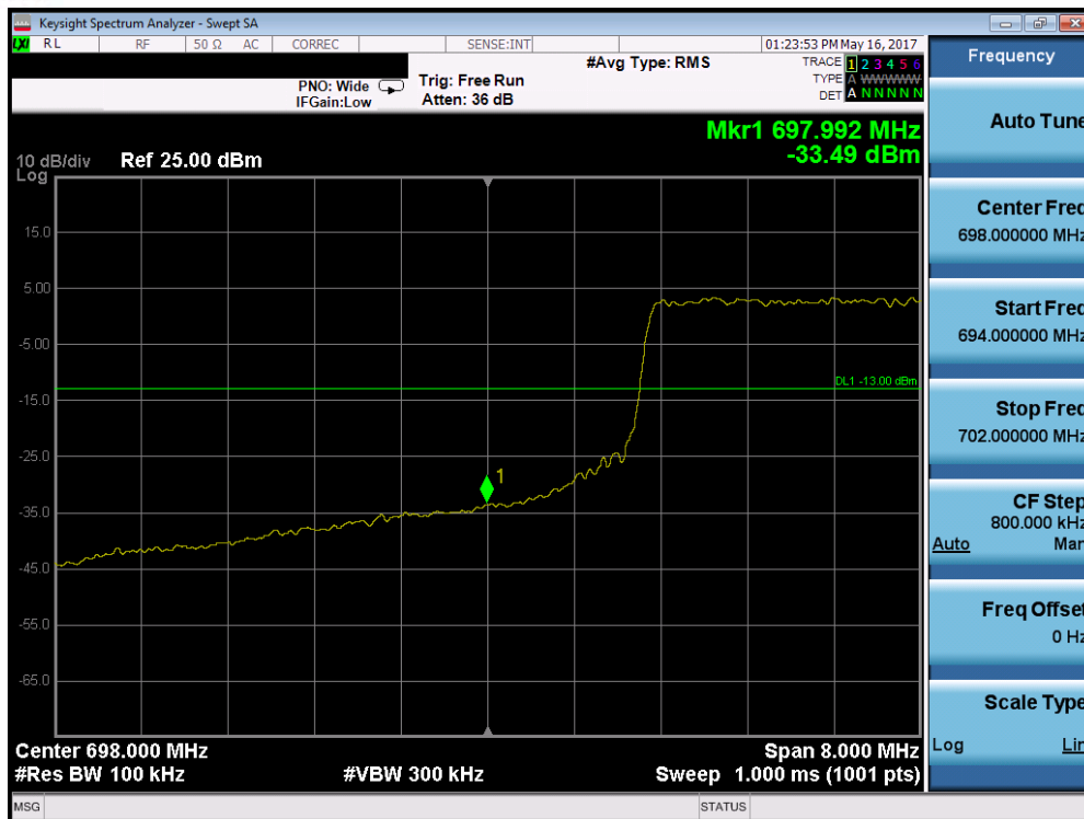
Plot 7-157. Lower Band Edge Plot (Band 12/17 - 10.0MHz QPSK - RB Size 50)
