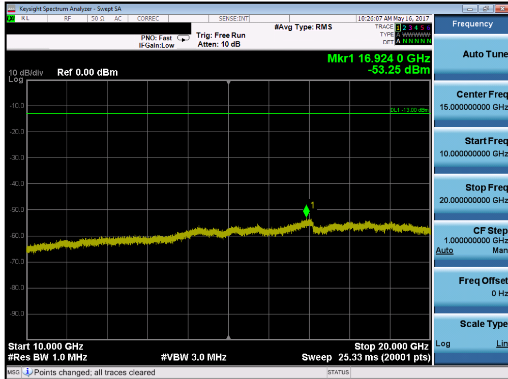
Plot 7-120. Conducted Spurious Plot (Band 4 – 20.0MHz QPSK – RB Size 1, RB Offset 0 – Mid Channel)
