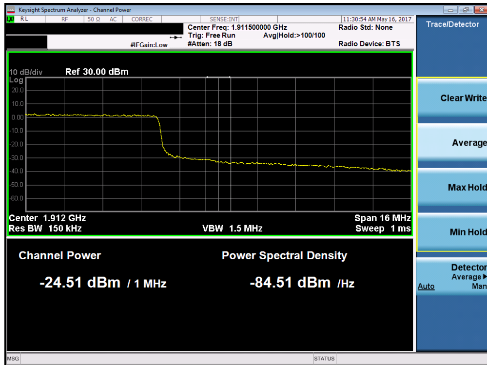
Plot 7-236. Upper Extended Band Edge Plot (Band 2 – 20.0MHz QPSK – RB Size 100)
