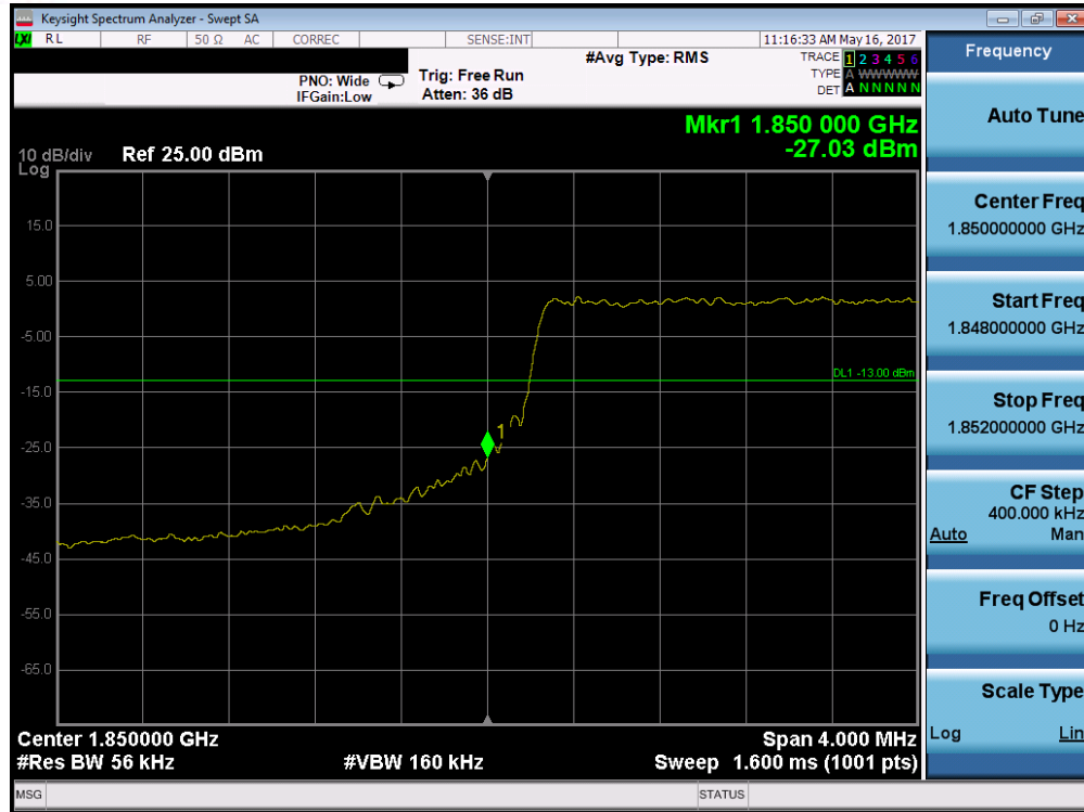
Plot 7-221. Lower Band Edge Plot (Band 2/25 – 5.0MHz QPSK – RB Size 25)
