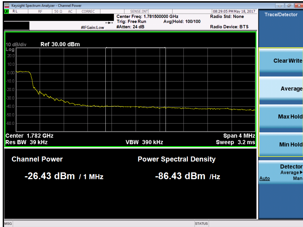
Plot 7-206. Upper Extended Band Edge Plot (Band 66 – 5.0MHz QPSK – RB Size 25)
