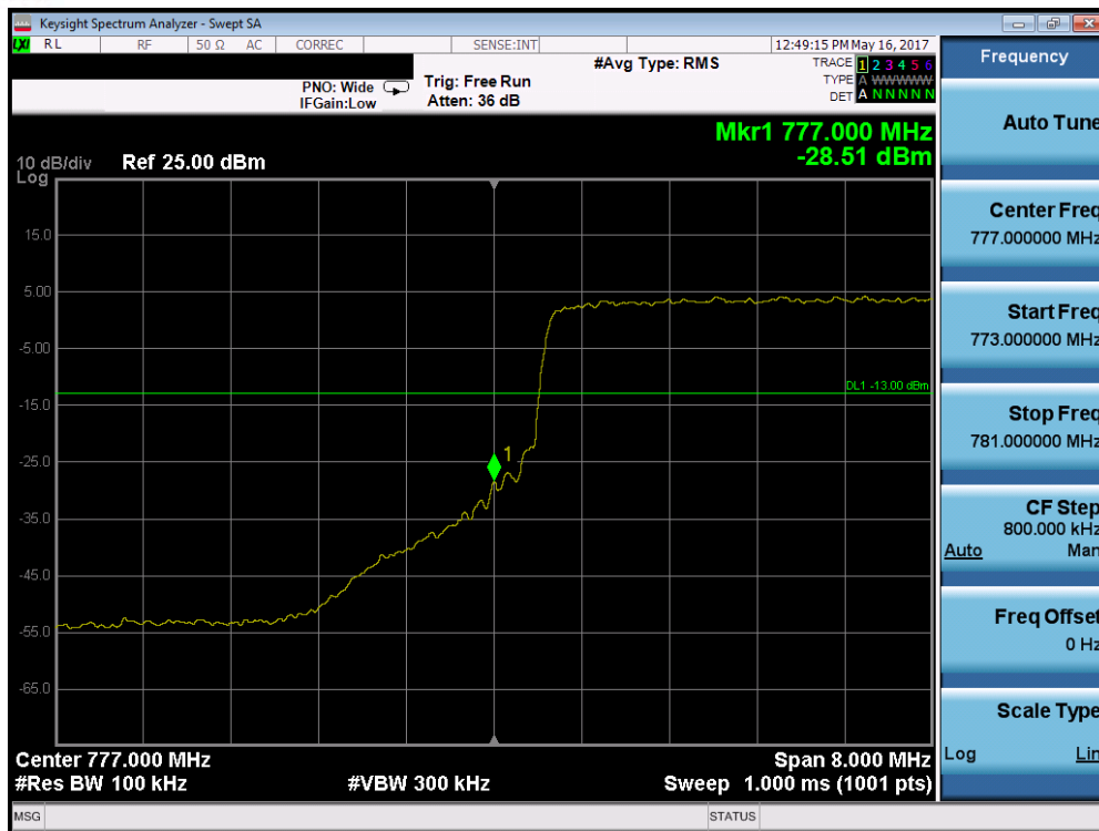
Plot 7-163. Lower Band Edge Plot (Band 13 – 10.0MHz QPSK – RB Size 50)
