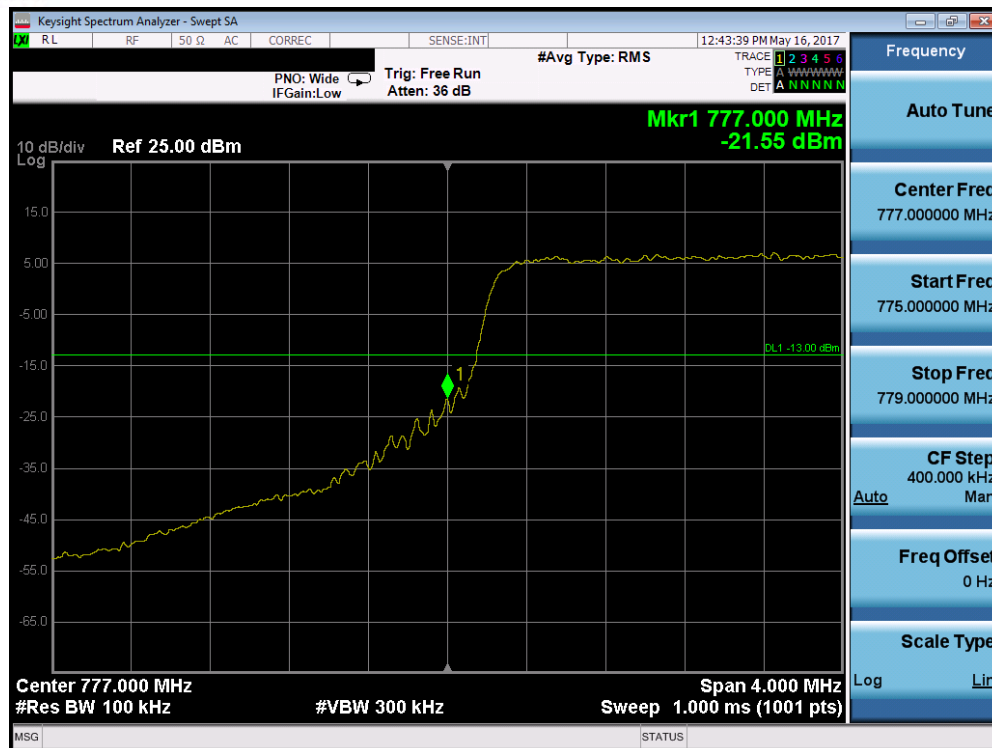
Plot 7-159. Lower Band Edge Plot (Band 13 – 5.0MHz QPSK – RB Size 25)
