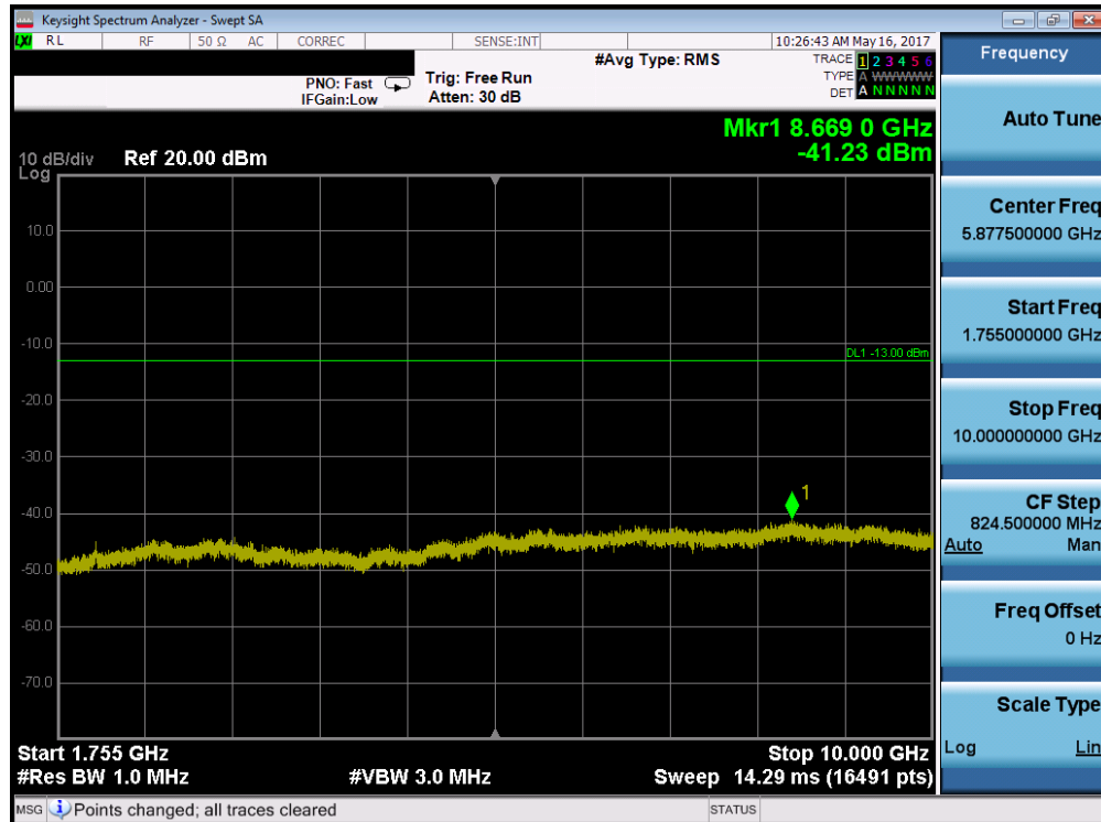
Plot 7-125. Conducted Spurious Plot (Band 2/25 – 20.0MHz QPSK – RB Size 1, RB Offset 0 – Low Channel)
