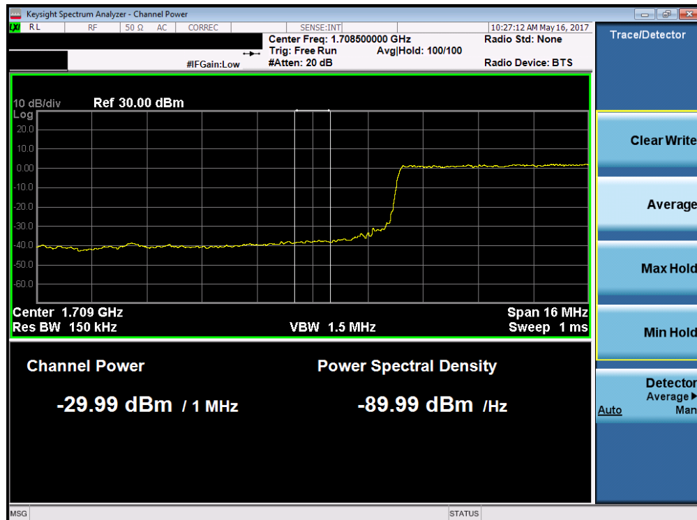
Plot 7-198. Lower Extended Band Edge Plot (Band 4/66 – 20.0MHz QPSK – RB Size 100)
