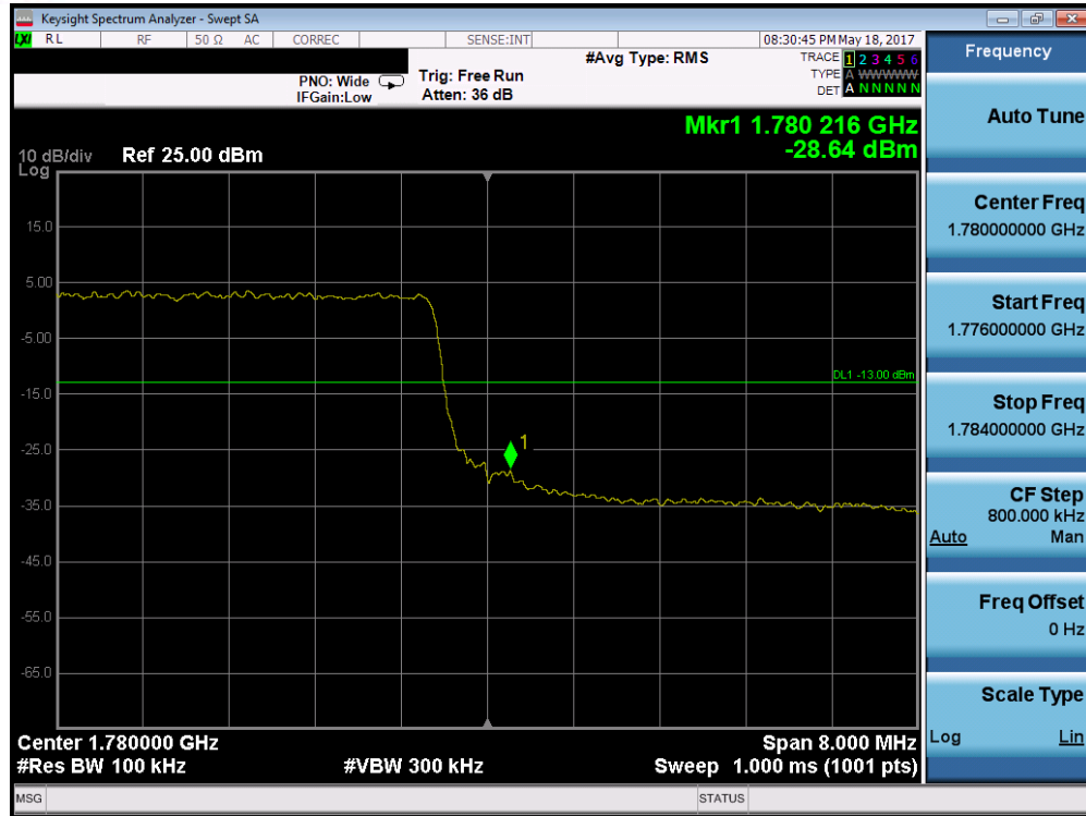
Plot 7-207. Upper Band Edge Plot (Band 66 – 10.0MHz QPSK – RB Size 50)
