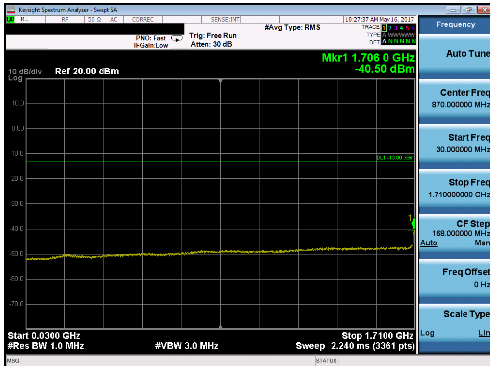
Plot 7-121. Conducted Spurious Plot (Band 4 – 20.0MHz QPSK – RB Size 1, RB Offset 0 – High Channel)
