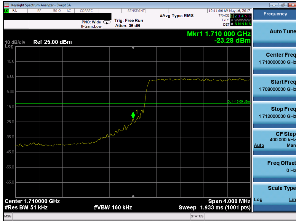
Plot 7-185. Lower Band Edge Plot (Band 4/66 – 5.0MHz QPSK – RB Size 25)
