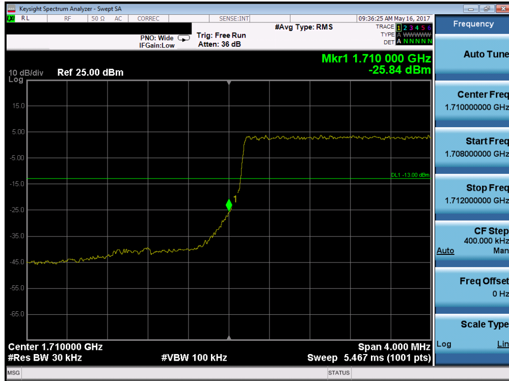
Plot 7-181. Lower Band Edge Plot (Band 4/66 – 3.0MHz QPSK – RB Size 15)
