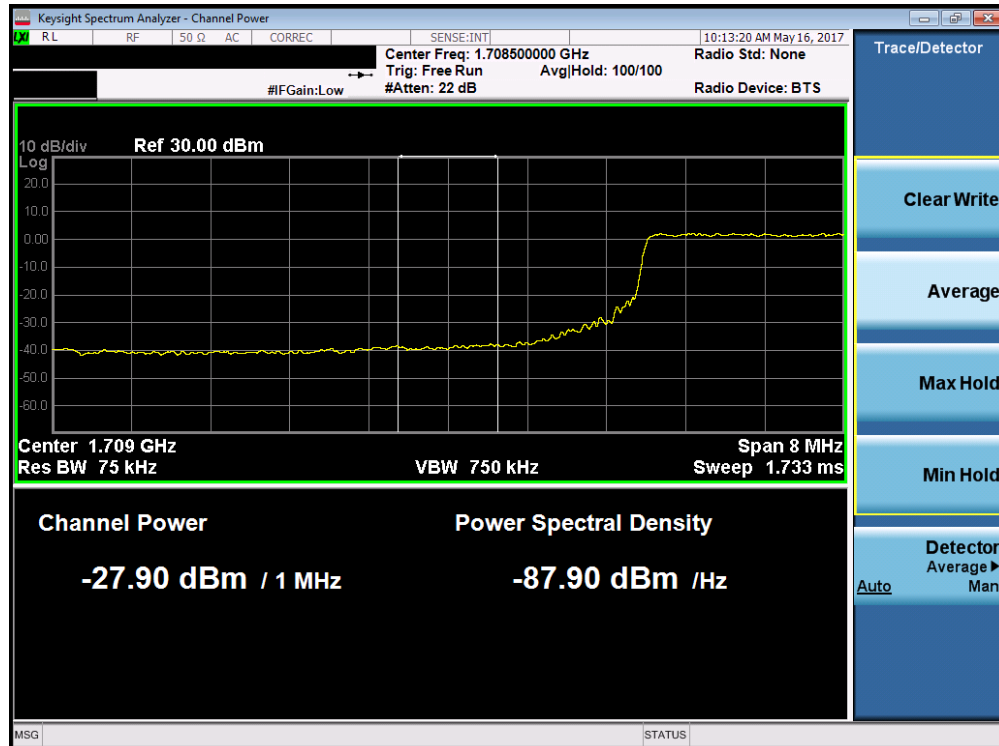
Plot 7-190. Lower Band Edge Plot (Band 4/66 – 10.0MHz QPSK – RB Size 50)
