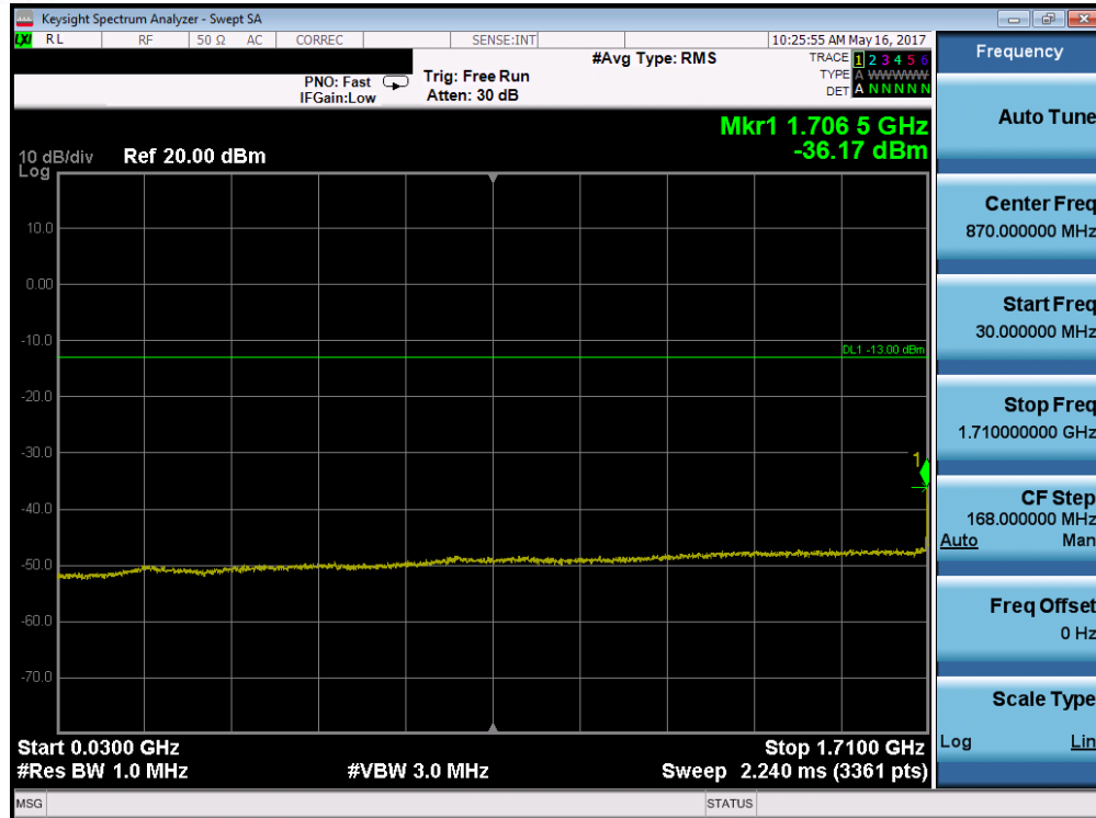
Plot 7-118. Conducted Spurious Plot (Band 4 – 20.0MHz QPSK – RB Size 1, RB Offset 0 – Mid Channel)
