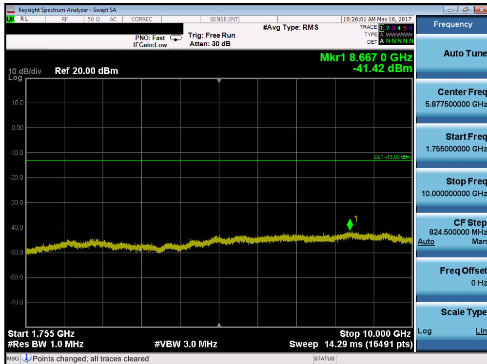
Plot 7-119. Conducted Spurious Plot (Band 4 – 20.0MHz QPSK – RB Size 1, RB Offset 0 – Mid Channel)
