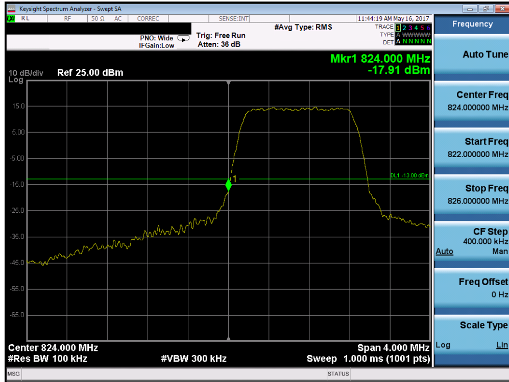
Plot 7-167. Lower Band Edge Plot (Band 5/26 – 1.4MHz QPSK – RB Size 6)
