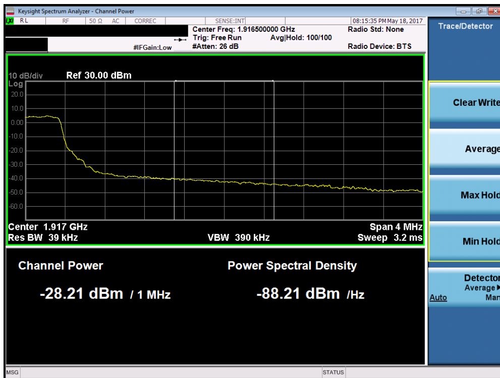
Plot 7-240. Upper Extended Band Edge Plot (Band 25 – 3.0MHz QPSK – RB Size 15)
