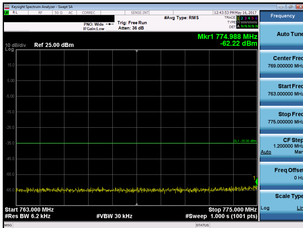
Plot 7-160. Lower Emission Mask Edge Plot (Band 13 – 5.0MHz QPSK – RB Size 25)
