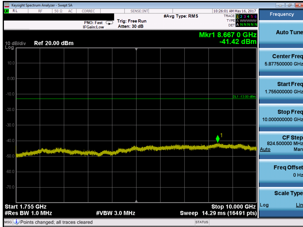
Plot 7-128. Conducted Spurious Plot (Band 2/25 – 20.0MHz QPSK – RB Size 1, RB Offset 0 – Mid Channel)
