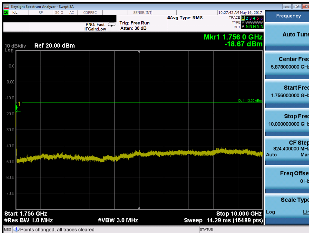
Plot 7-122. Conducted Spurious Plot (Band 4 – 20.0MHz QPSK – RB Size 1, RB Offset 0 – High Channel)
