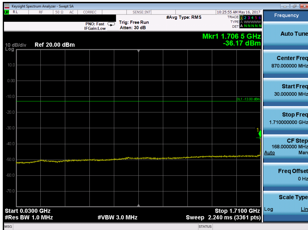
Plot 7-127. Conducted Spurious Plot (Band 2/25 – 20.0MHz QPSK – RB Size 1, RB Offset 0 – Mid Channel)
