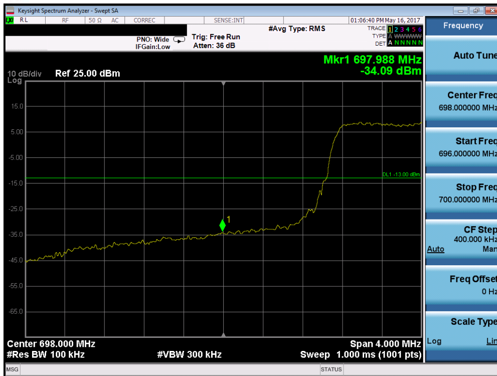
Plot 7-153. Lower Band Edge Plot (Band 12 – 3.0MHz QPSK – RB Size 15)
