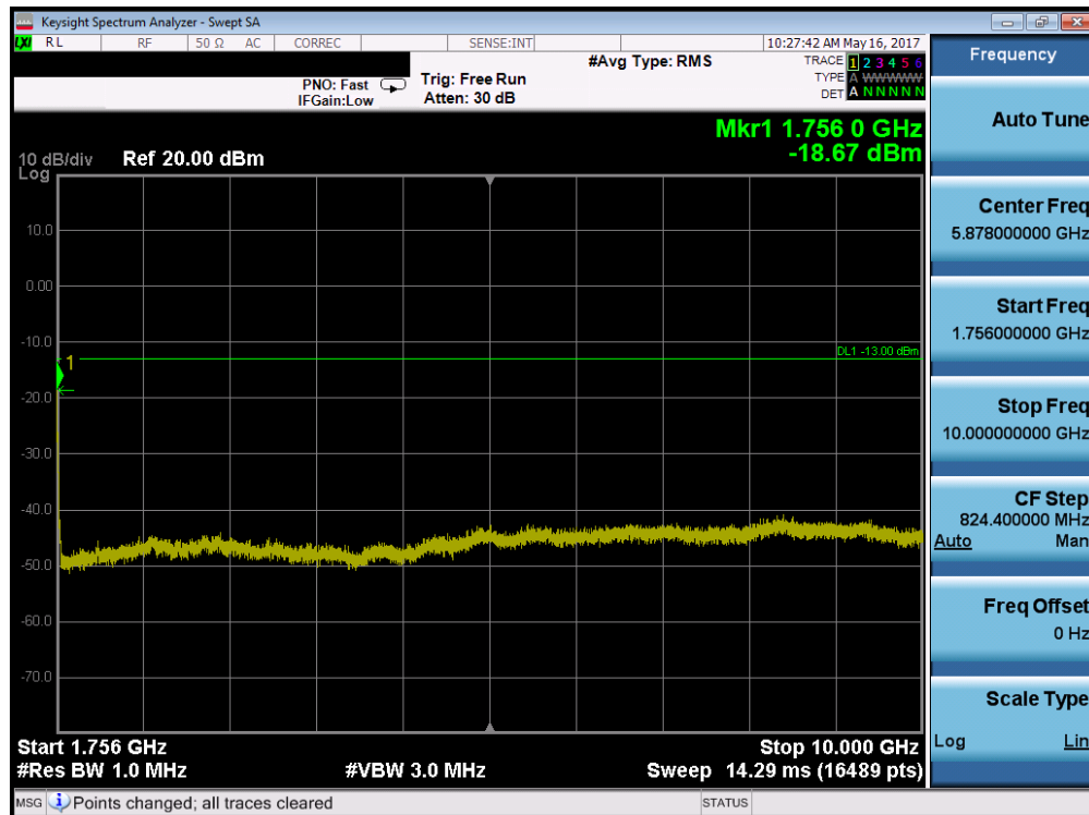
Plot 7-131. Conducted Spurious Plot (Band 2/25 – 20.0MHz QPSK – RB Size 1, RB Offset 0 – High Channel)
