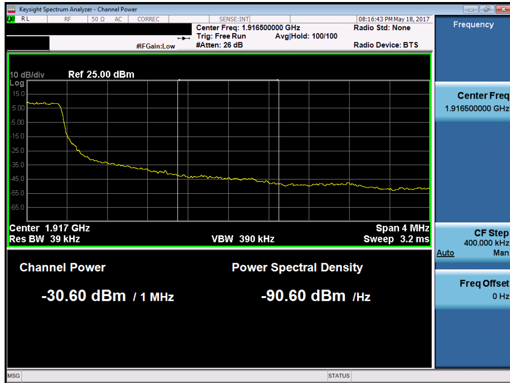
Plot 7-238. Upper Extended Band Edge Plot (Band 25 – 1.4MHz QPSK – RB Size 6)
