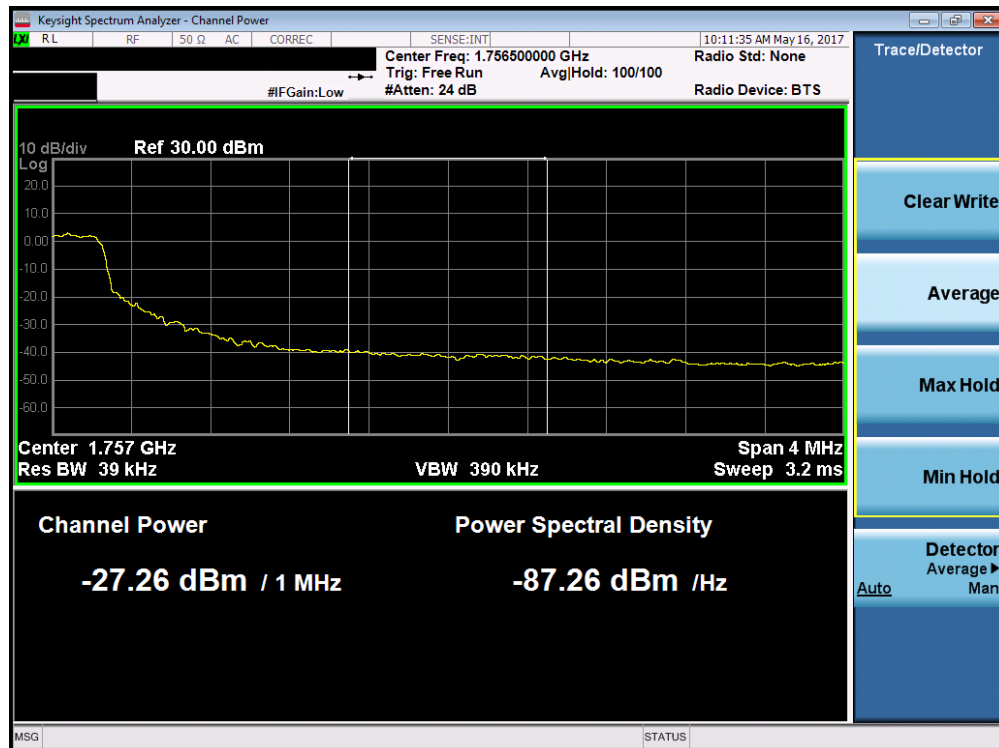
Plot 7-188. Upper Extended Band Edge Plot (Band 4 – 5.0MHz QPSK – RB Size 25)
