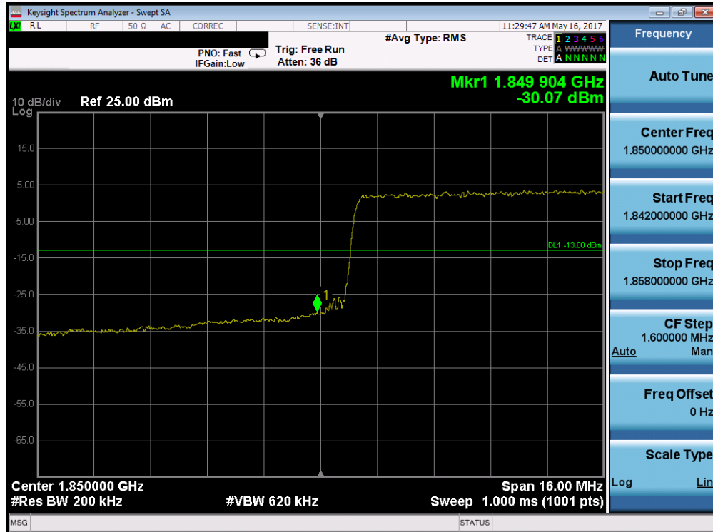
Plot 7-233. Lower Band Edge Plot (Band 2/25 – 20.0MHz QPSK – RB Size 100)
