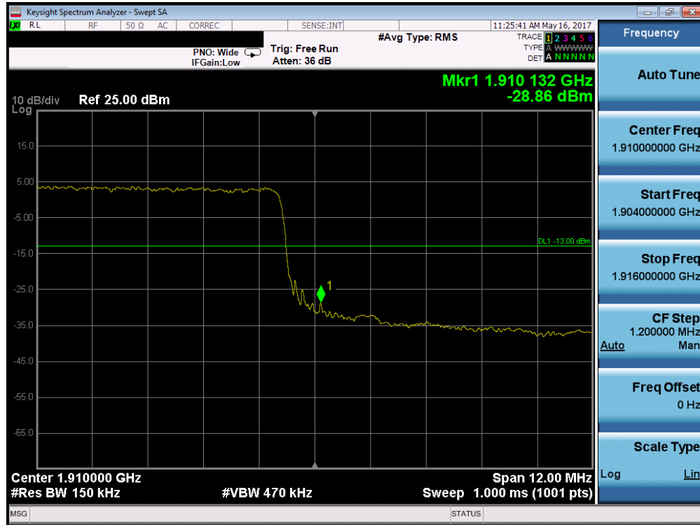
Plot 7-231. Upper Band Edge Plot (Band 2 – 15.0MHz QPSK – RB Size 75)
