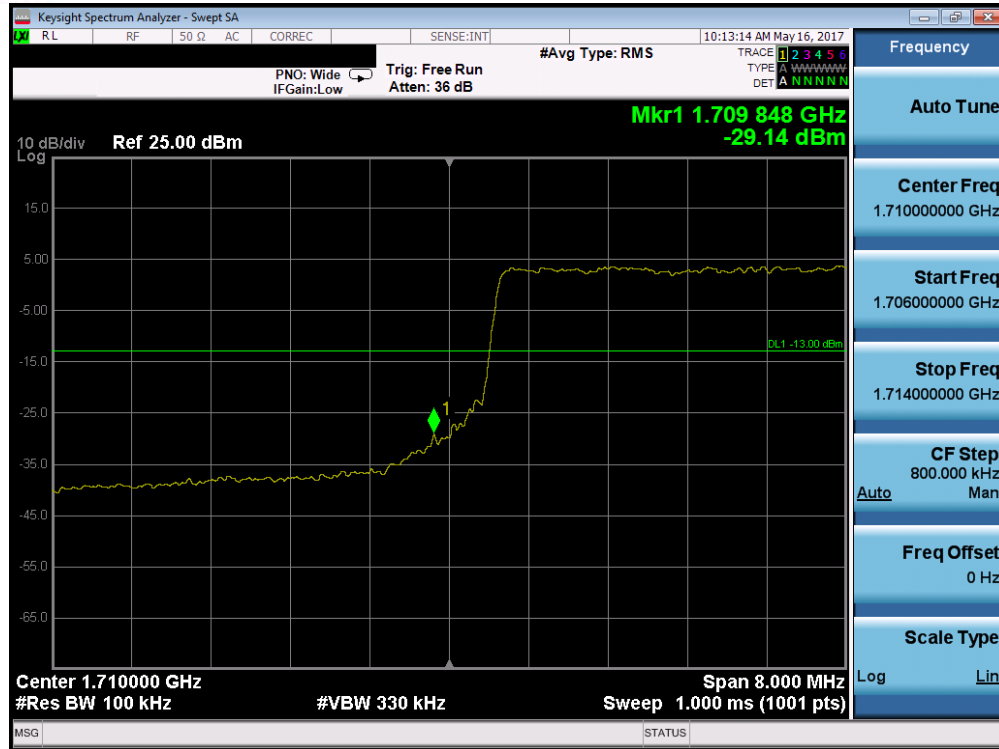
Plot 7-189. Lower Band Edge Plot (Band 4/66 – 10.0MHz QPSK – RB Size 50)
