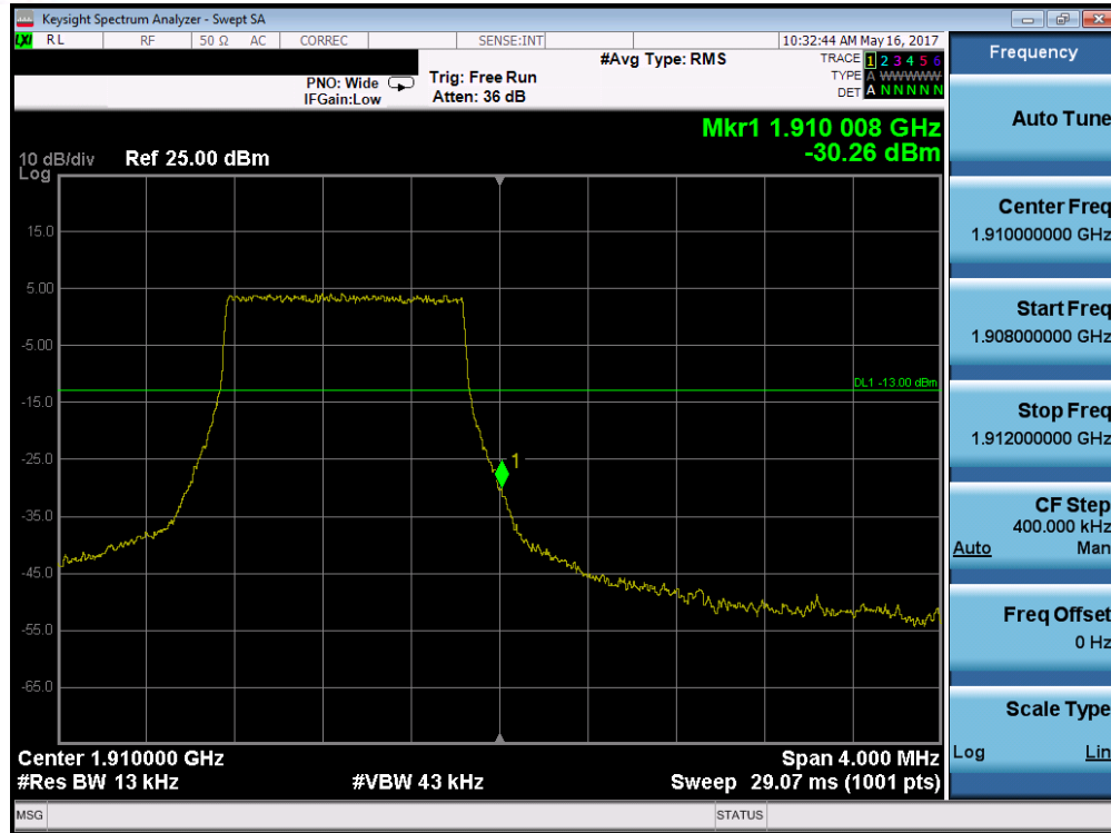
Plot 7-215. Upper Band Edge Plot (Band 2 – 1.4MHz QPSK – RB Size 6)
