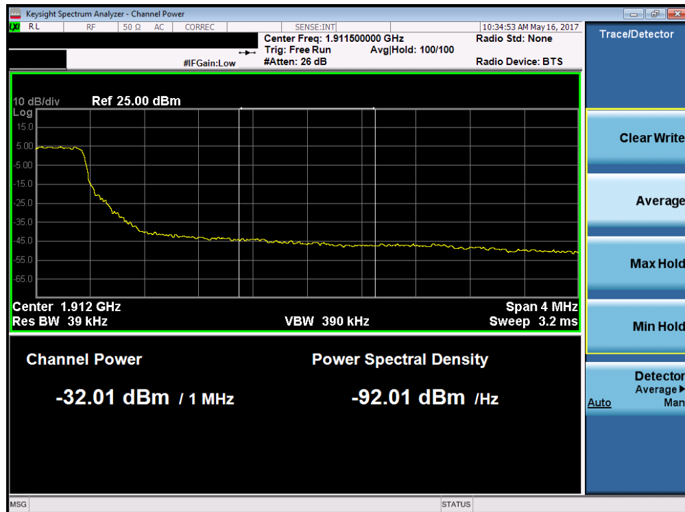
Plot 7-220. Upper Extended Band Edge Plot (Band 2 – 3.0MHz QPSK – RB Size 15)
