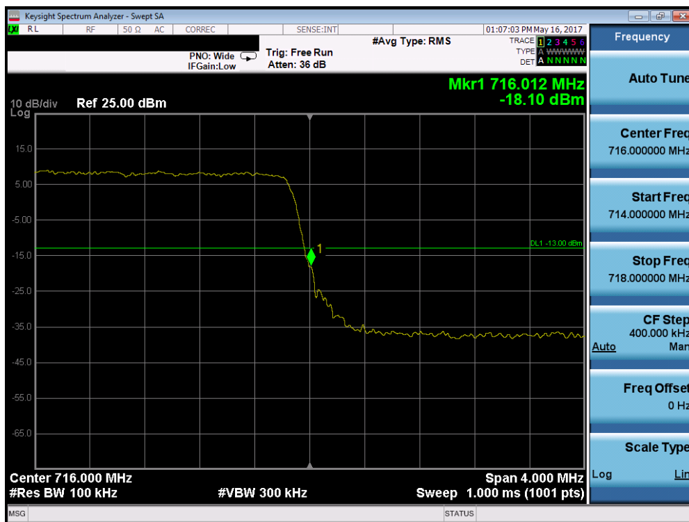
Plot 7-154. Upper Band Edge Plot (Band 12 – 3.0MHz QPSK – RB Size 15)
