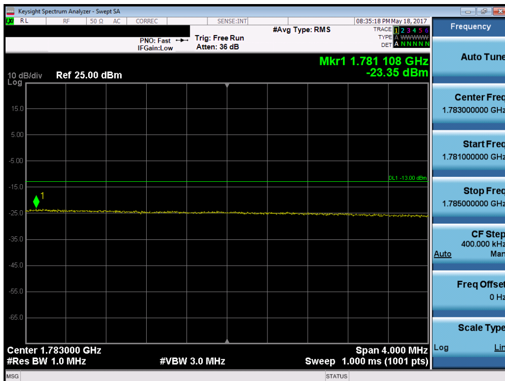
Plot 7-212. Upper Extended Band Edge Plot (Band 66 – 20.0MHz QPSK – RB Size 100)
