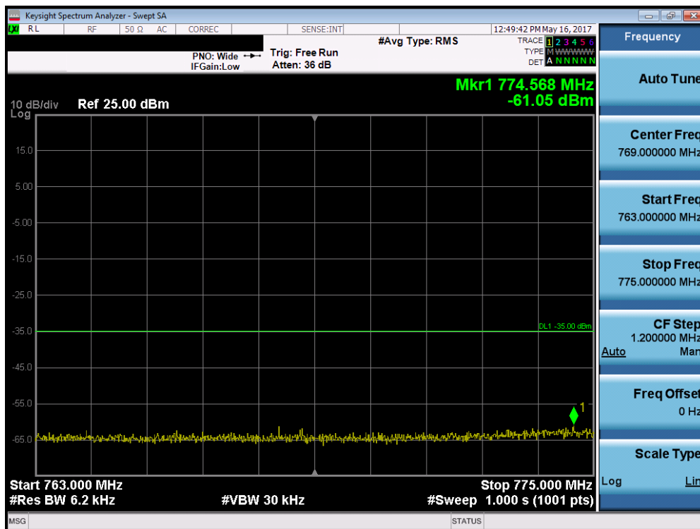
Plot 7-164. Lower Emission Mask Edge Plot (Band 13 – 10.0MHz QPSK – RB Size 50)
