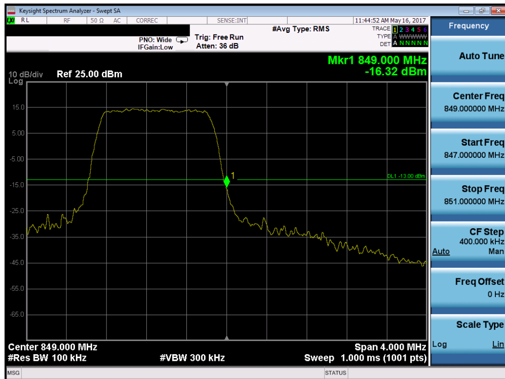
Plot 7-168. Upper Band Edge Plot (Band 5/26 – 1.4MHz QPSK – RB Size 6)
