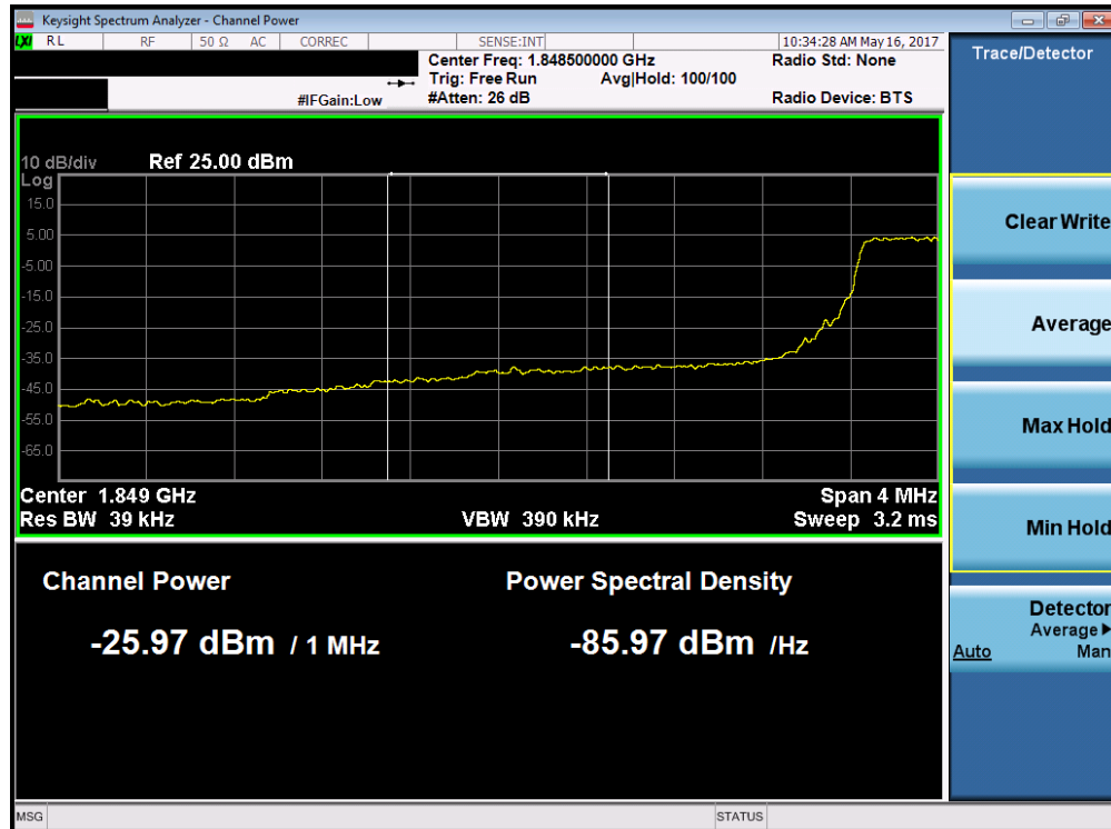
Plot 7-218. Lower Extended Band Edge Plot (Band 2/25 – 3.0MHz QPSK – RB Size 15)
