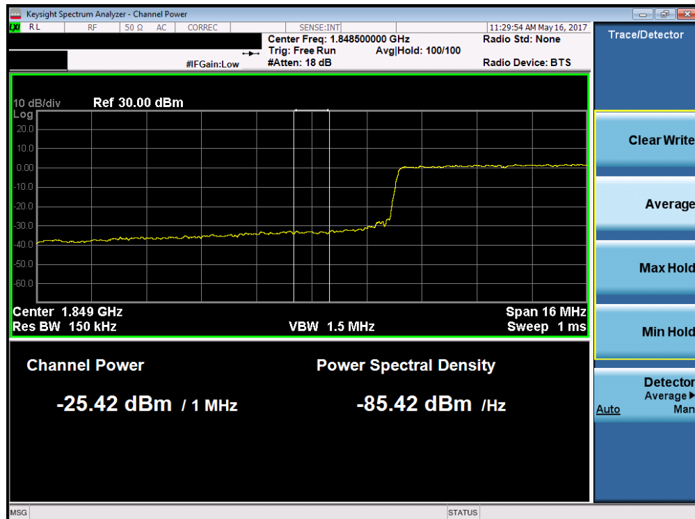
Plot 7-234. Lower Extended Band Edge Plot (Band 2/25 – 20.0MHz QPSK – RB Size 100)
