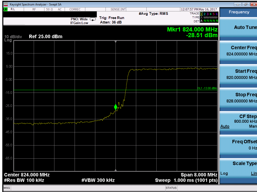
Plot 7-173. Lower Band Edge Plot (Band 5/26 – 10.0MHz QPSK – RB Size 50)
