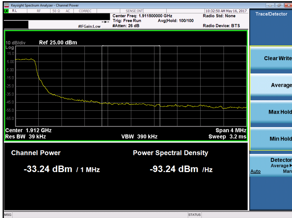
Plot 7-216. Upper Extended Band Edge Plot (Band 2 – 1.4MHz QPSK – RB Size 6)
