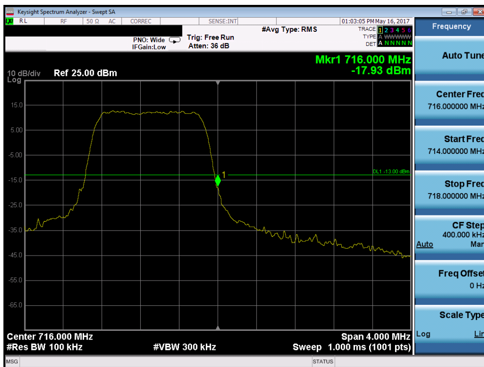
Plot 7-152. Upper Band Edge Plot (Band 12 - 1.4MHz QPSK - RB Size 6)
