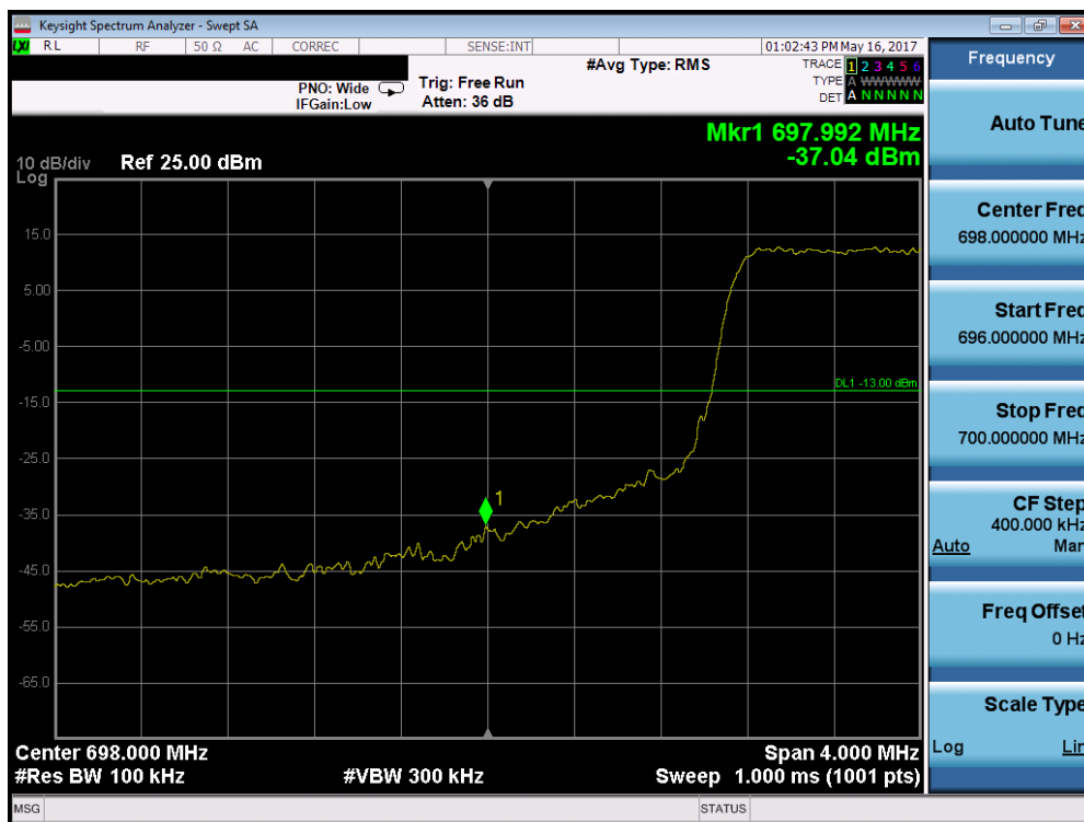
Plot 7-151. Lower Band Edge Plot (Band 12 - 1.4MHz QPSK - RB Size 6)
