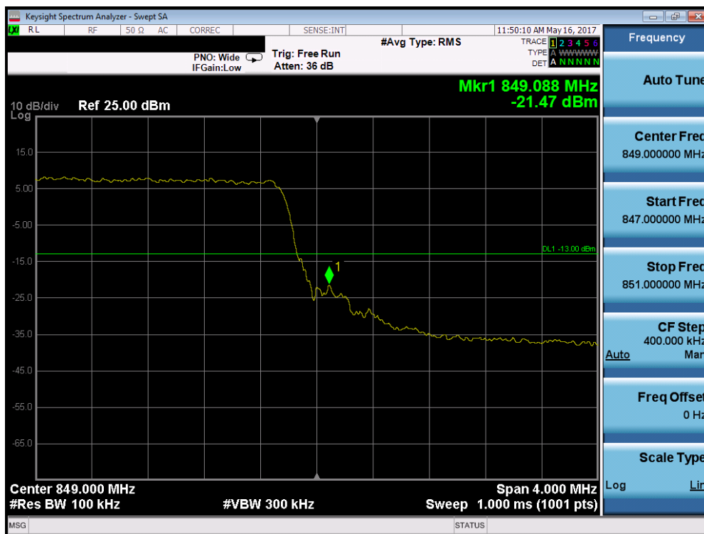
Plot 7-172. Upper Band Edge Plot (Band 5/26 – 5.0MHz QPSK – RB Size 25)
