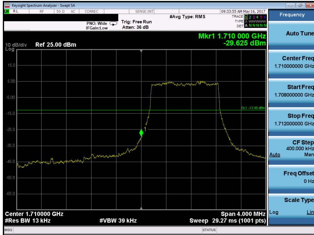
Plot 7-177. Lower Band Edge Plot (Band 4 /66– 1.4MHz QPSK – RB Size 6)
