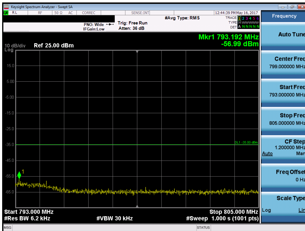
Plot 7-162. Upper Emission Mask Edge Plot (Band 13 – 5.0MHz QPSK – RB Size 25)
