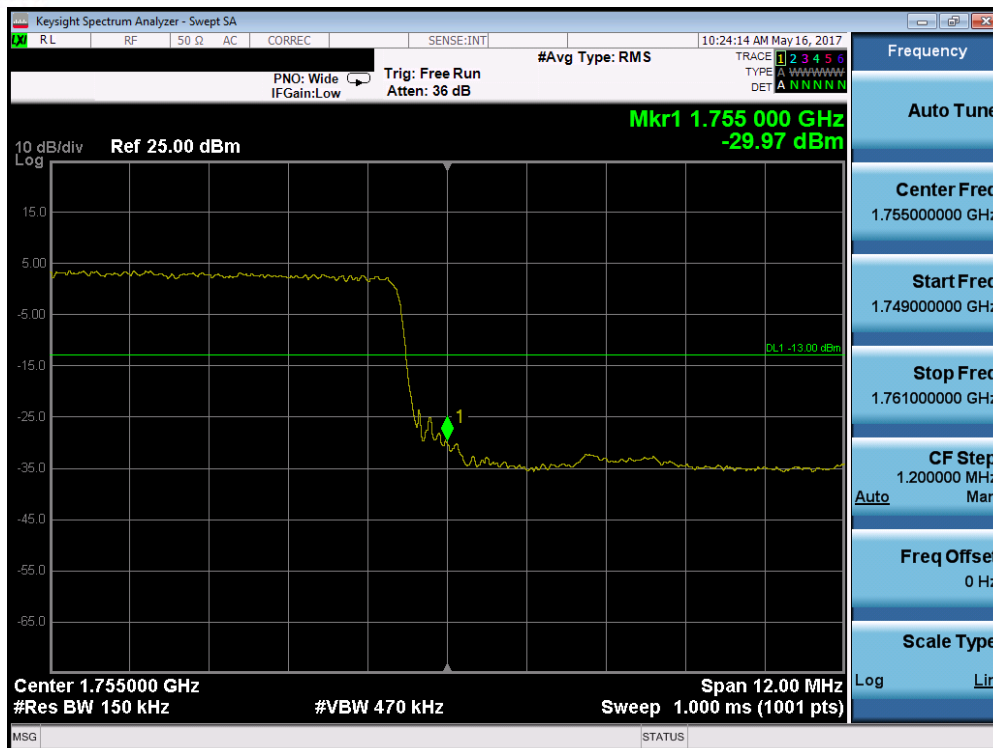
Plot 7-195. Upper Band Edge Plot (Band 4 – 15.0MHz QPSK – RB Size 75)
