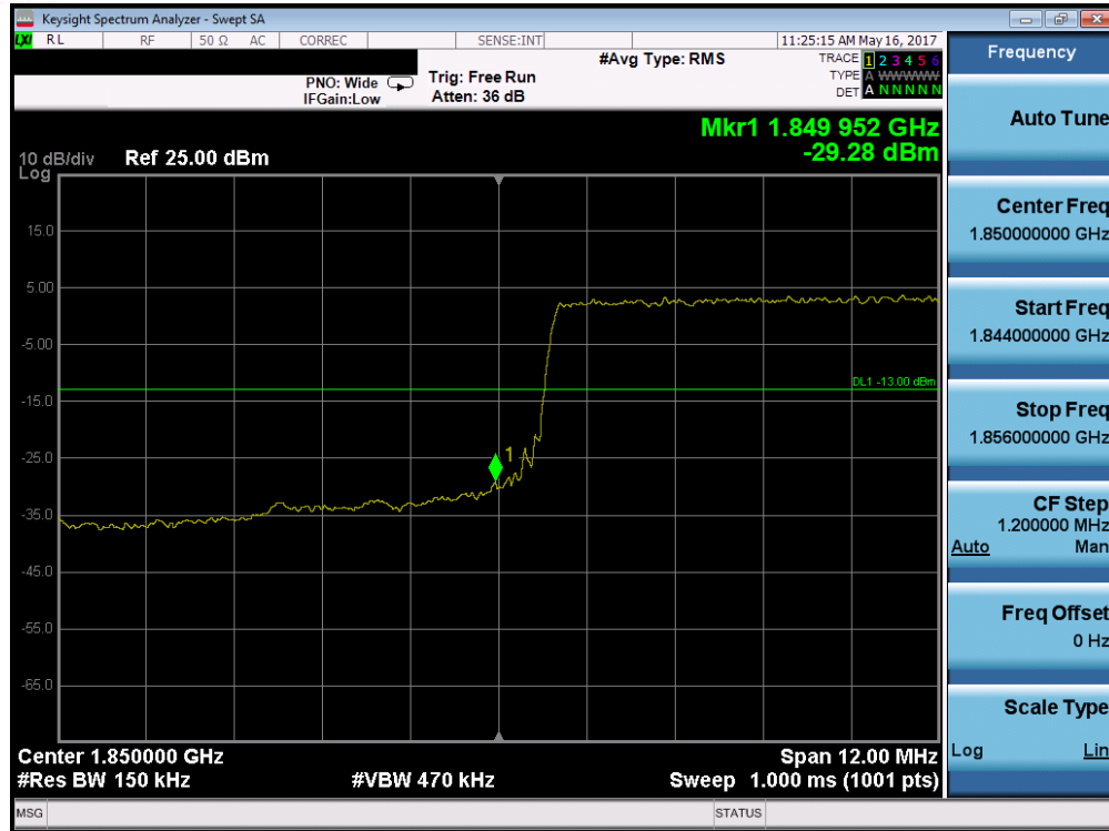
Plot 7-229. Lower Band Edge Plot (Band 2/25 – 15.0MHz QPSK – RB Size 75)
