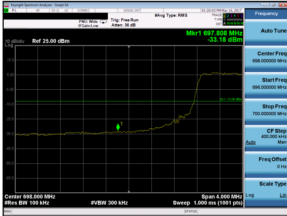
Plot 7-155. Lower Band Edge Plot (Band 12/17 – 5.0MHz QPSK – RB Size 25)
