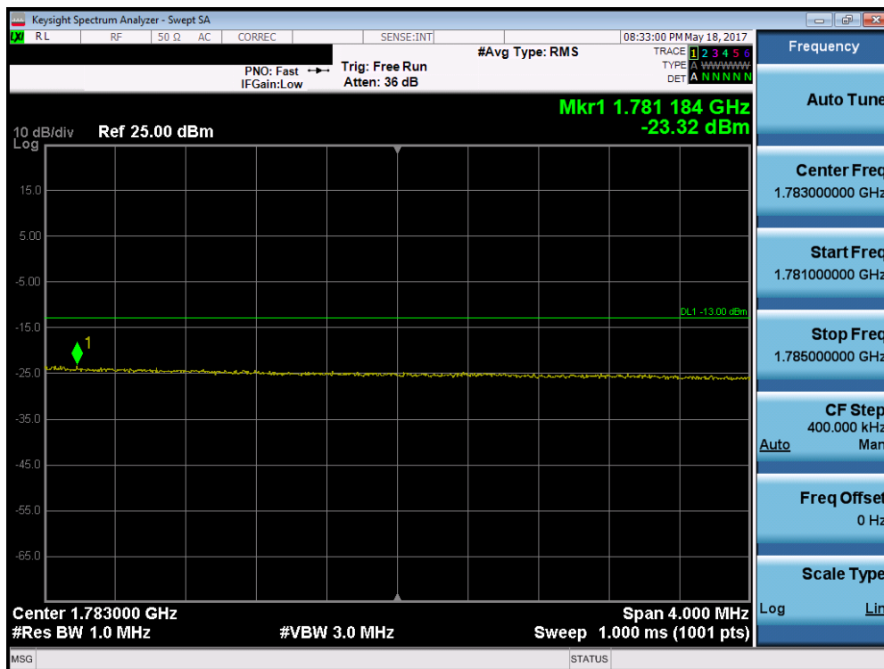
Plot 7-210. Upper Extended Band Edge Plot (Band 66 – 15.0MHz QPSK – RB Size 75)
