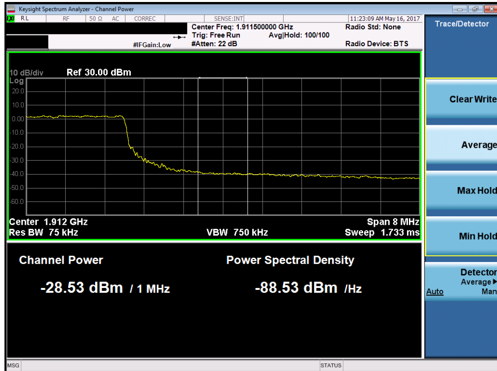
Plot 7-228. Upper Extended Band Edge Plot (Band 2 – 10.0MHz QPSK – RB Size 50)
