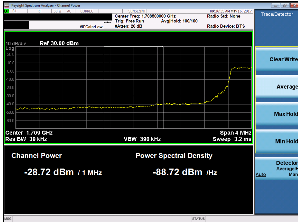
Plot 7-182. Lower Extended Band Edge Plot (Band 4/66 – 3.0MHz QPSK – RB Size 15)
