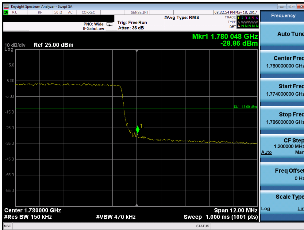
Plot 7-209. Upper Band Edge Plot (Band 66 – 15.0MHz QPSK – RB Size 75)
