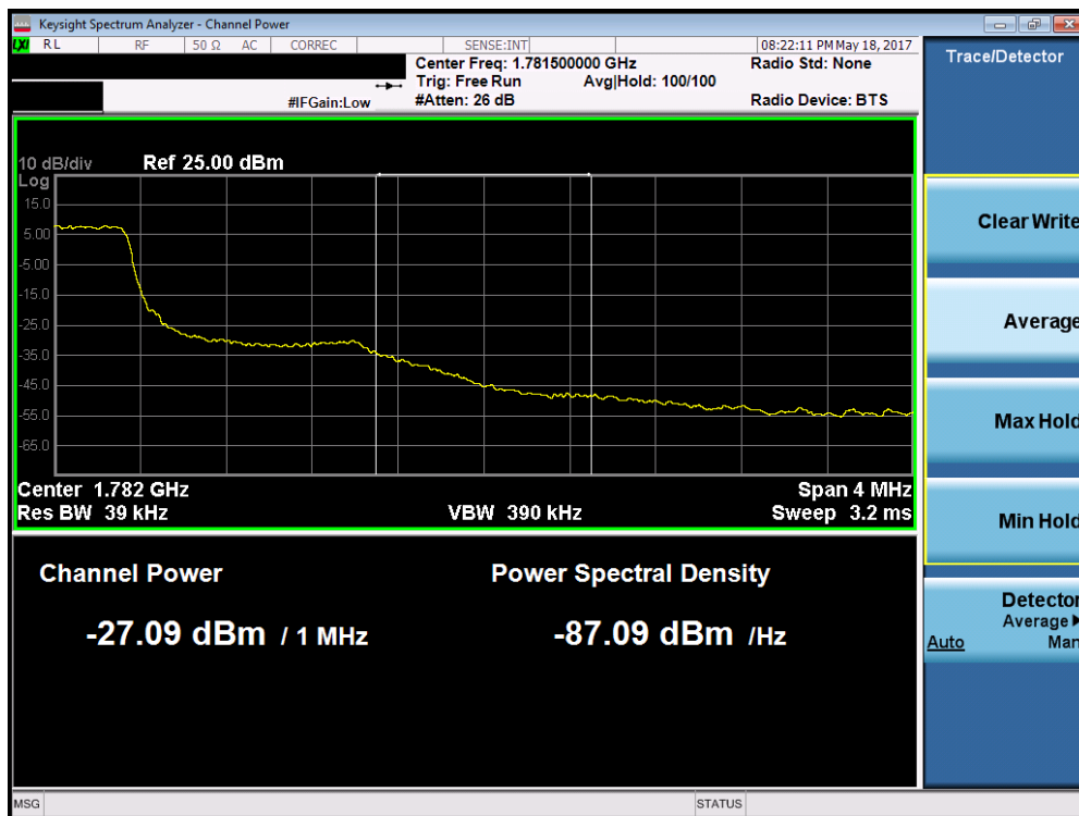
Plot 7-202. Upper Extended Band Edge Plot (Band 66 – 1.4MHz QPSK – RB Size 6)
