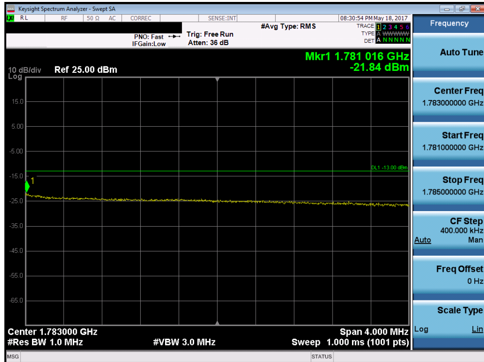
Plot 7-208. Upper Extended Band Edge Plot (Band 66 – 10.0MHz QPSK – RB Size 50)
