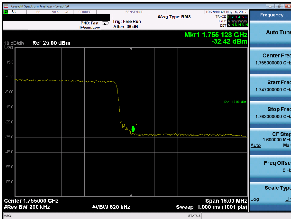
Plot 7-199. Upper Band Edge Plot (Band 4 – 20.0MHz QPSK – RB Size 100)
