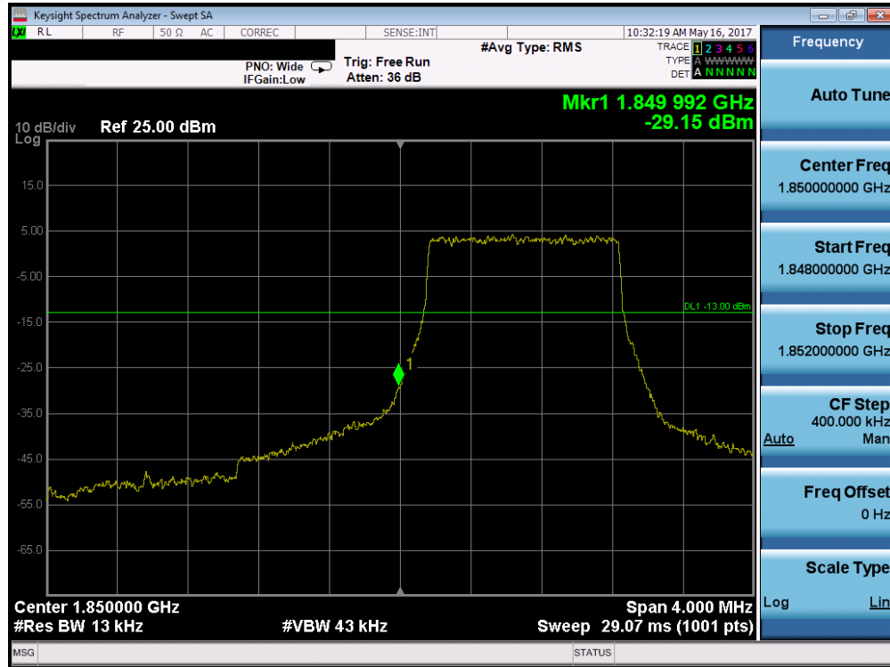
Plot 7-213. Lower Band Edge Plot (Band 2/25 – 1.4MHz QPSK – RB Size 6)
