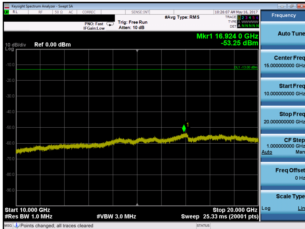
Plot 7-129. Conducted Spurious Plot (Band 2/25 – 20.0MHz QPSK – RB Size 1, RB Offset 0 – Mid Channel)
