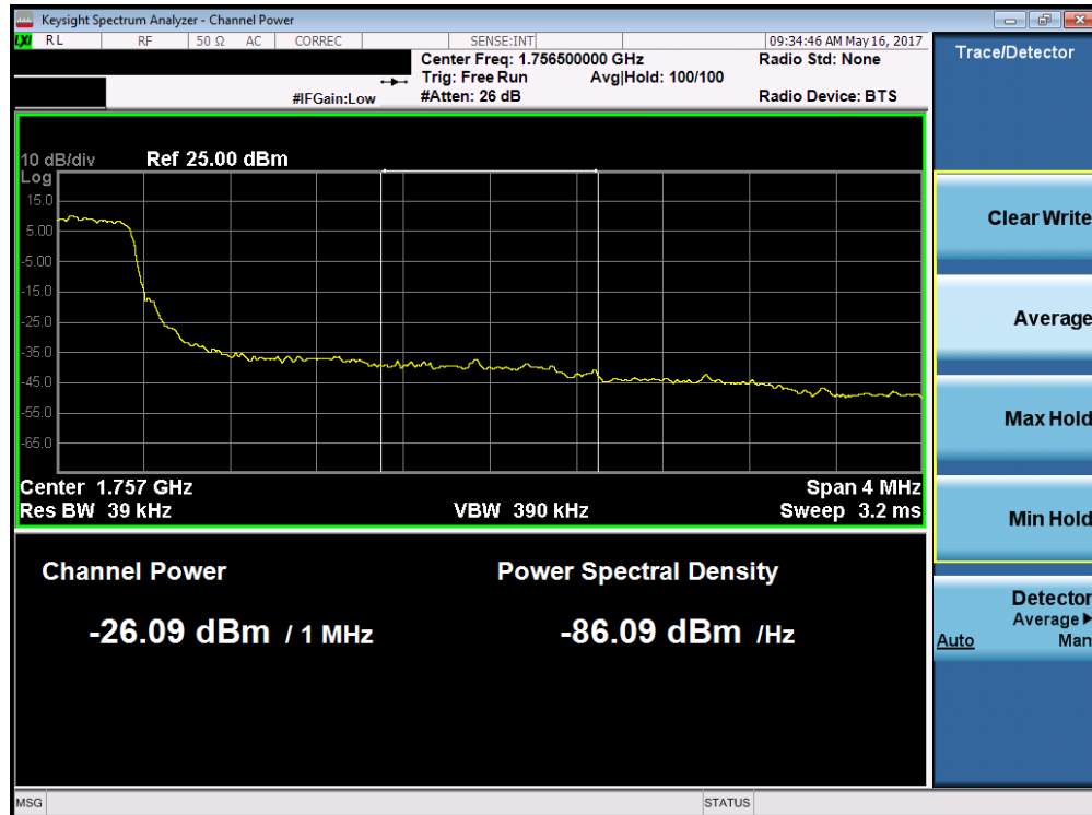
Plot 7-180. Upper Extended Band Edge Plot (Band 4 – 1.4MHz QPSK – RB Size 6)
