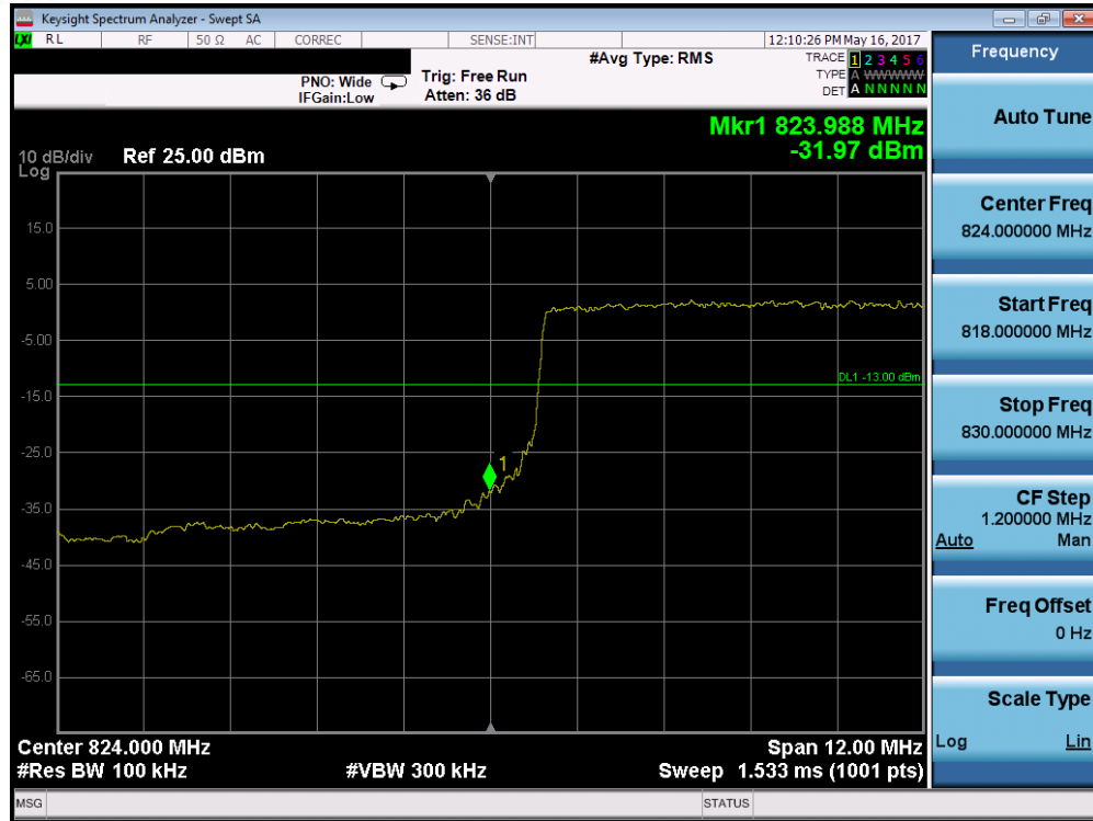
Plot 7-175. Lower Band Edge Plot (Band 26 – 15.0MHz QPSK – RB Size 75)
