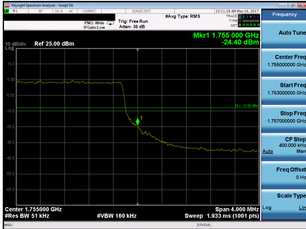
Plot 7-187. Upper Band Edge Plot (Band 4 – 5.0MHz QPSK – RB Size 25)
