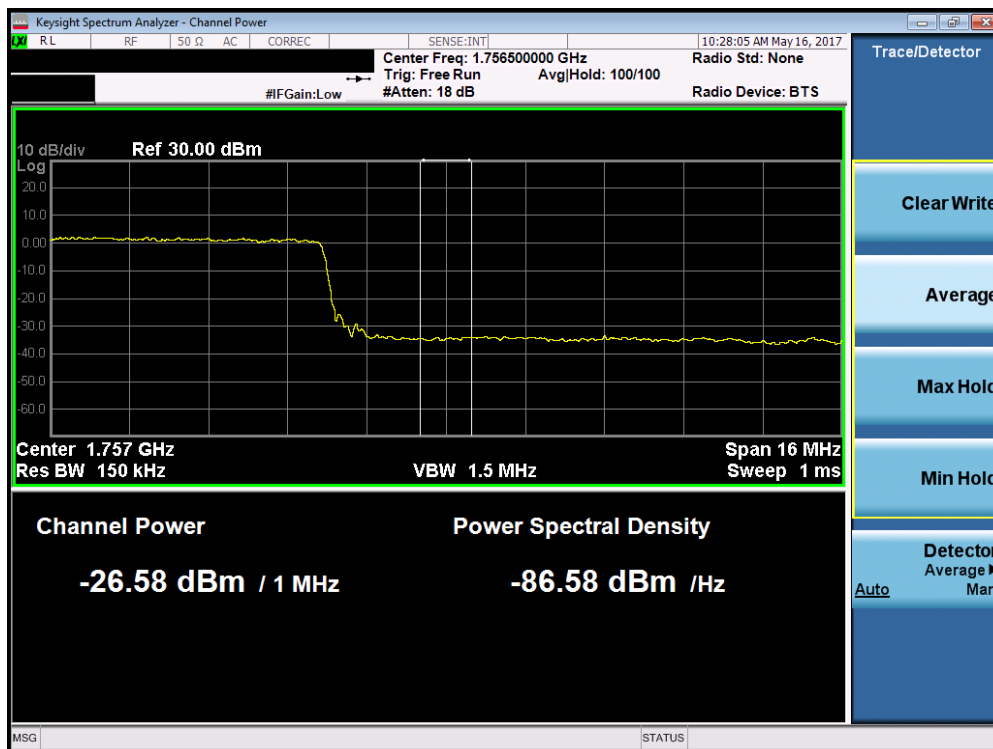
Plot 7-200. Upper Extended Band Edge Plot (Band 4 – 20.0MHz QPSK – RB Size 100)
