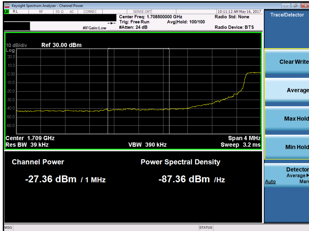
Plot 7-186. Lower Extended Band Edge Plot (Band 4/66 – 5.0MHz QPSK – RB Size 25)
