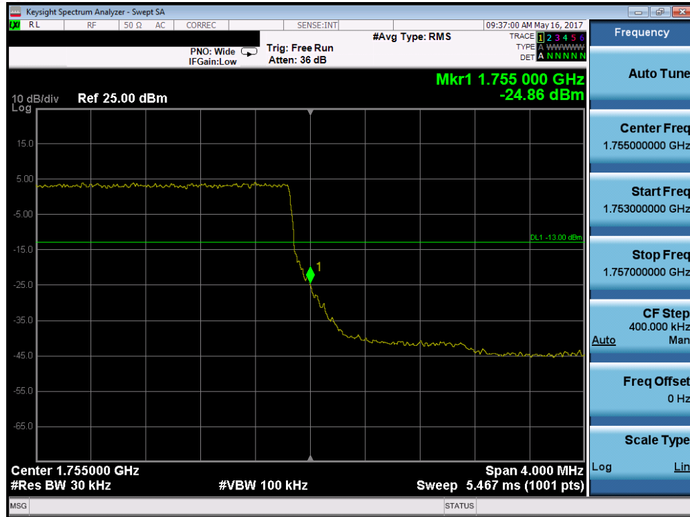
Plot 7-183. Upper Band Edge Plot (Band 4 – 3.0MHz QPSK – RB Size 15)
