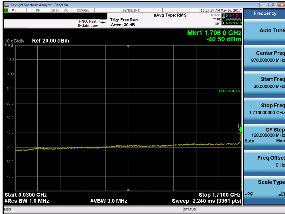
Plot 7-130. Conducted Spurious Plot (Band 2/25 – 20.0MHz QPSK – RB Size 1, RB Offset 0 – High Channel)
