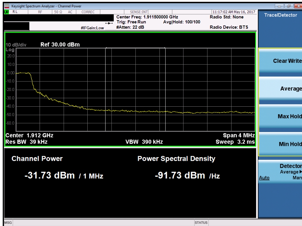
Plot 7-224. Upper Extended Band Edge Plot (Band 2 – 5.0MHz QPSK – RB Size 25)
