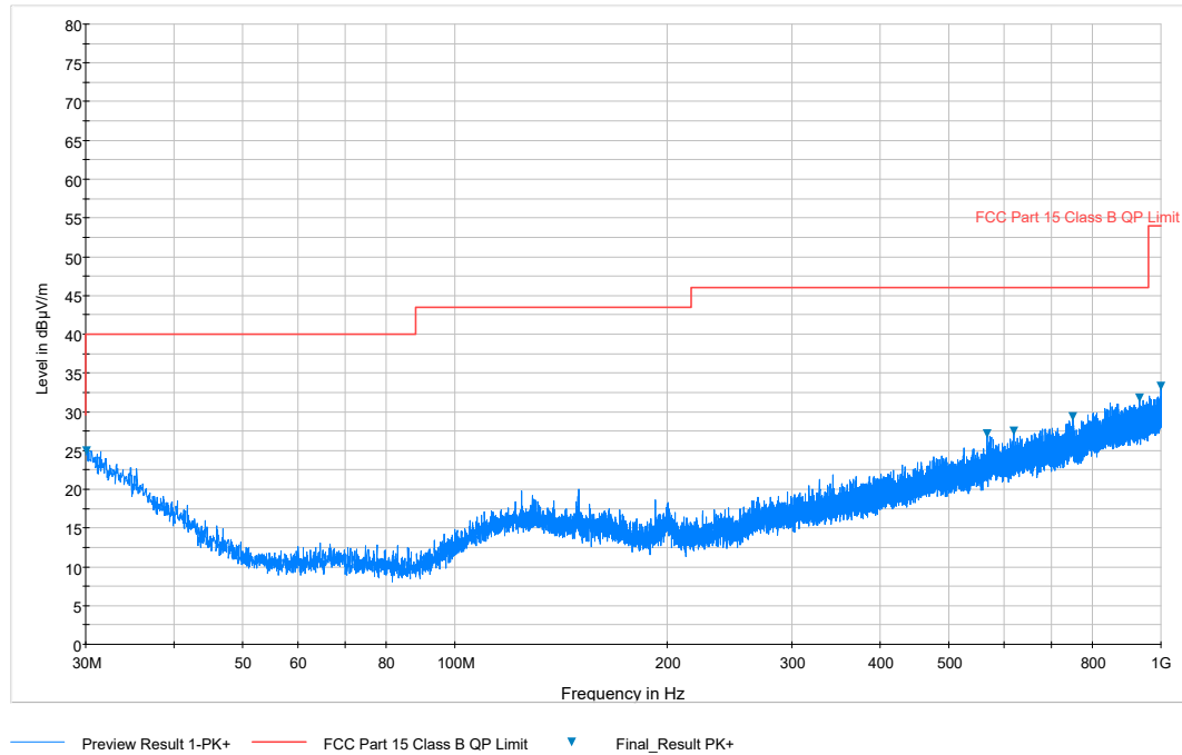
Plot 7-255. Radiated Spurious Plot below 1GHz (802.11a – U3 Ch. 157, Ant. Pol. H)
