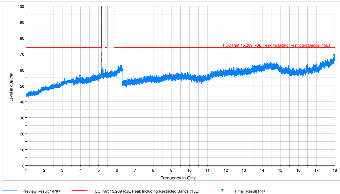
Plot 7-157. Radiated Spurious Plot above 1GHz (802.11a – U1 Ch. 40, Ant. Pol. H)
