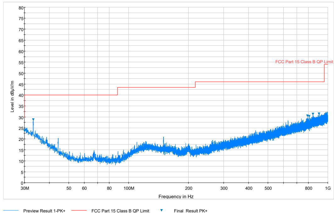
Plot 7-254. Radiated Spurious Plot below 1GHz (802.11a – U3 Ch. 157, Ant. Pol. V)
