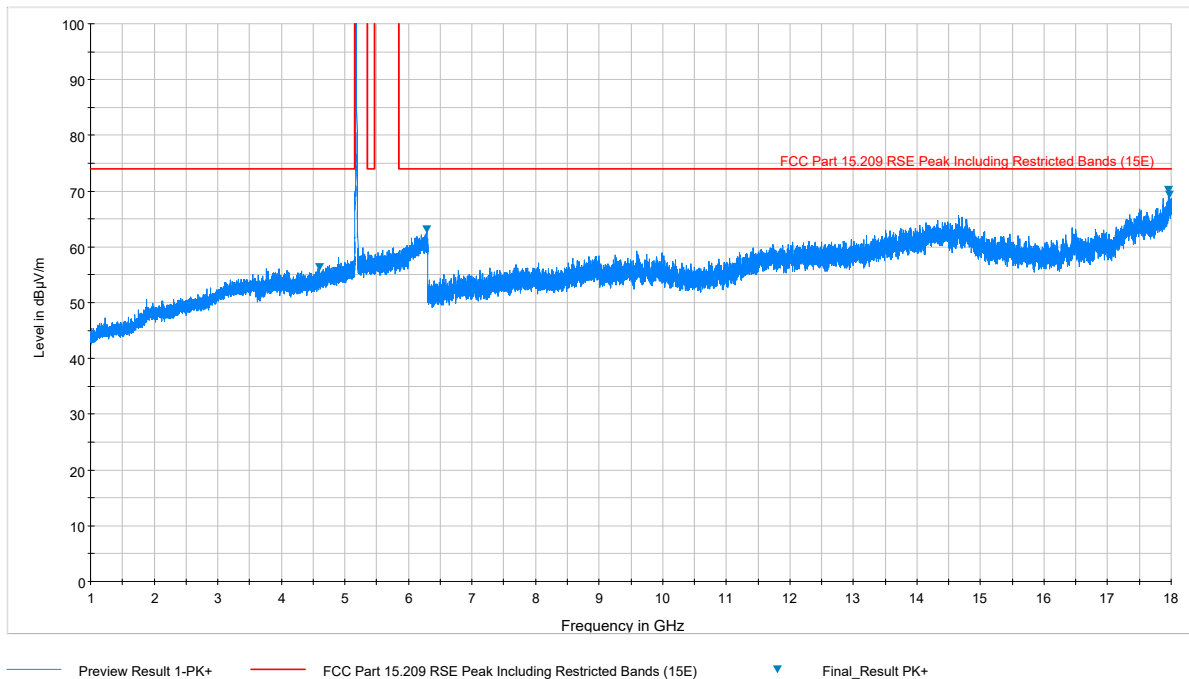
Plot 7-158. Radiated Spurious Plot above 1GHz (802.11a – U1 Ch. 40, Ant. Pol. V)
