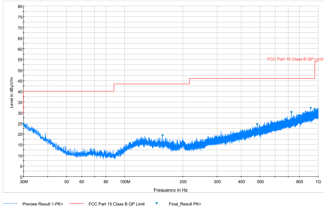
Plot 7-253. Radiated Spurious Plot below 1GHz (802.11a – U3 Ch. 157, Ant. Pol. H)
