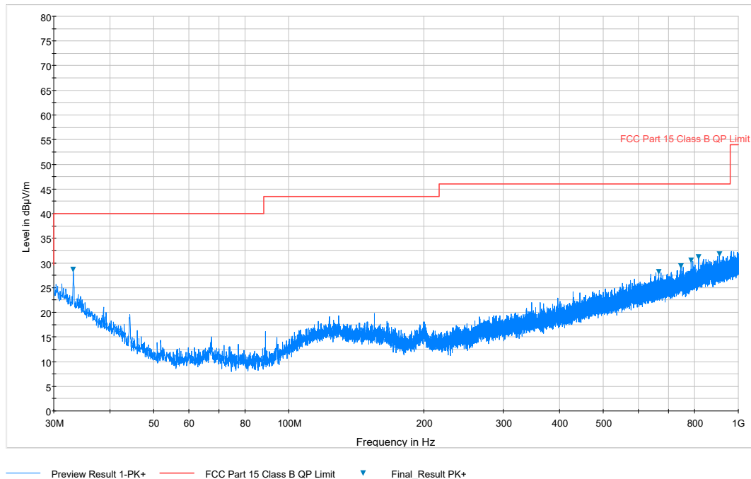
Plot 7-256. Radiated Spurious Plot below 1GHz (802.11a – U3 Ch. 157, Ant. Pol. V)
