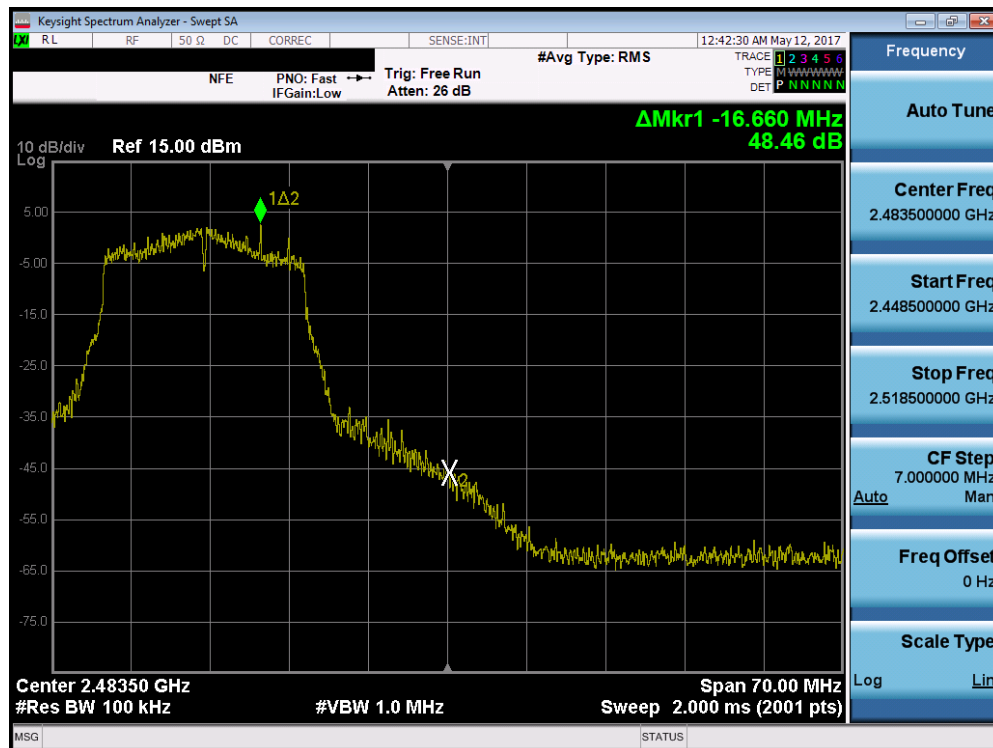
Plot 7-58. Band Edge Plot (802.11n (2.4GHz) – Ch. 11)
