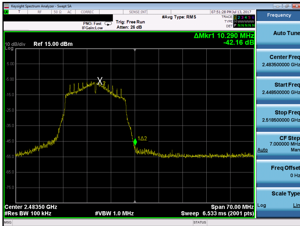
Plot 7-60. Band Edge Plot (802.11n (2.4GHz) – Ch. 13)
