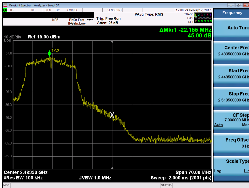
Plot 7-46. Band Edge Plot (802.11n (2.4GHz) – Ch. 11)
