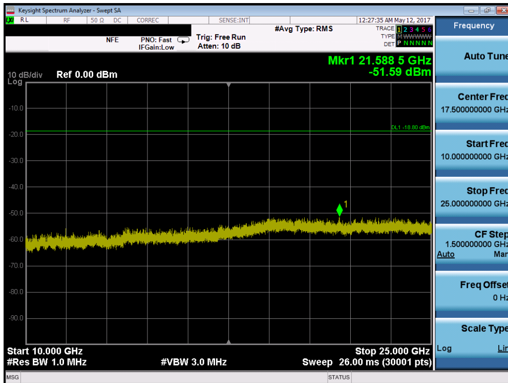
Plot 7-72. Conducted Spurious Plot (802.11b – Ch. 11)
