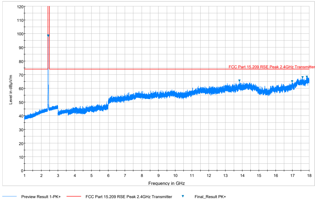
Plot 7-74. Radiated Spurious Plot above 1GHz (802.11b – Ch. 1, Ant. Pol. V)
