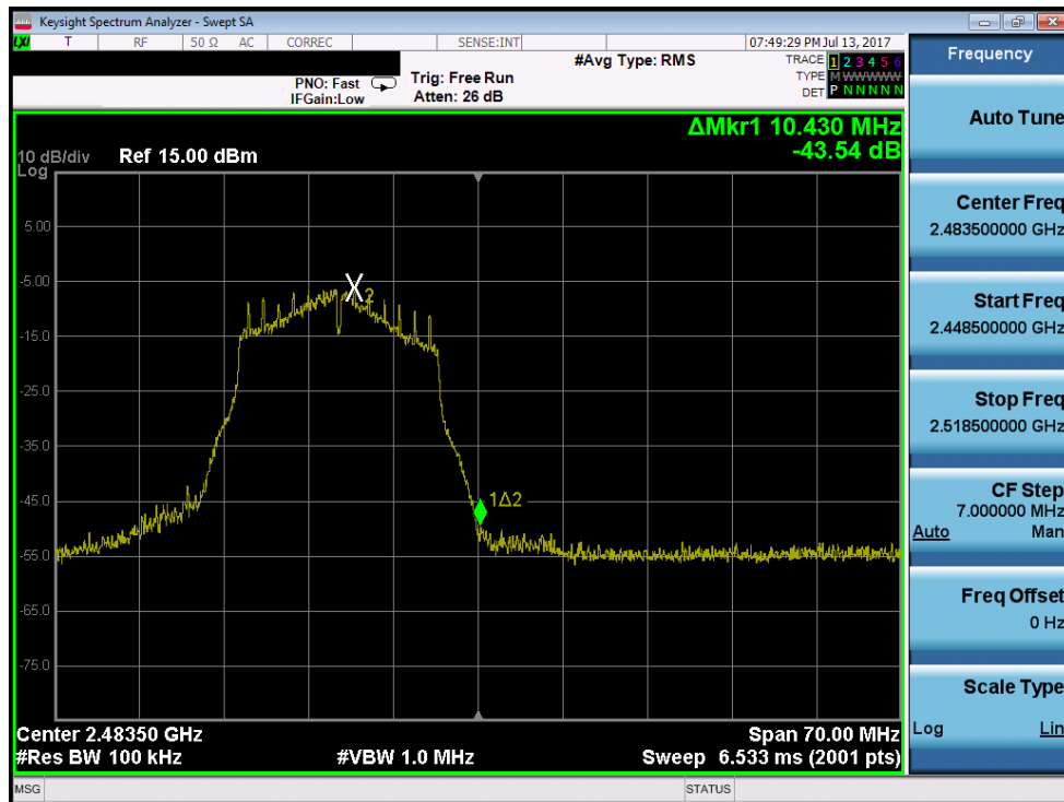
Plot 7-56. Band Edge Plot (802.11g – Ch. 13)
