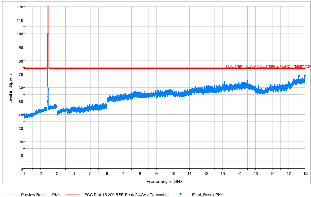
Plot 7-73. Radiated Spurious Plot above 1GHz (802.11b – Ch. 1, Ant. Pol. H)
