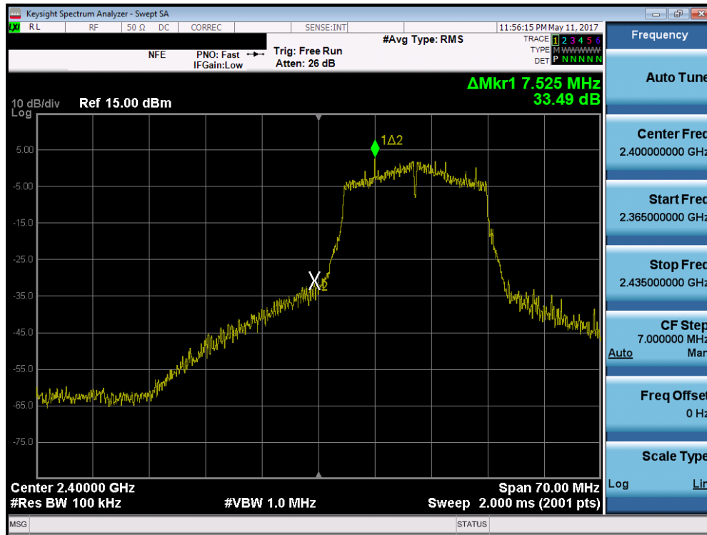
Plot 7-45. Band Edge Plot (802.11n (2.4GHz) – Ch. 1)
