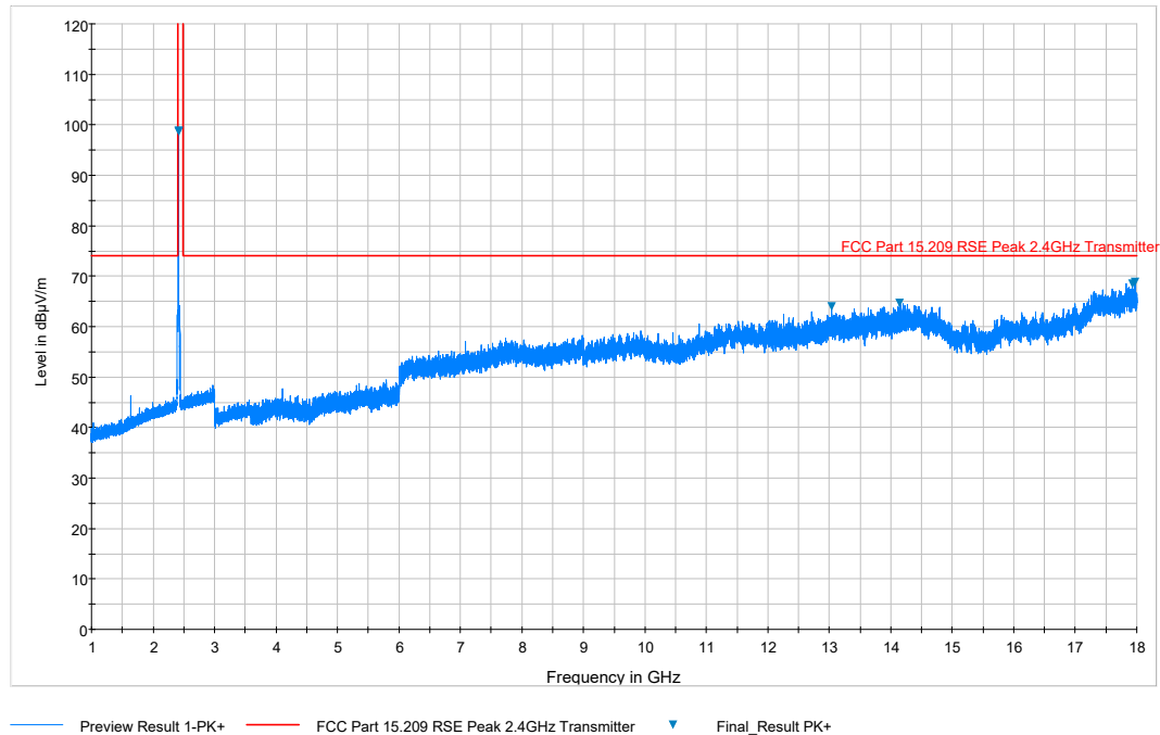
Plot 7-81. Radiated Spurious Plot above 1GHz (802.11b – Ch. 1, Ant. Pol. H)
