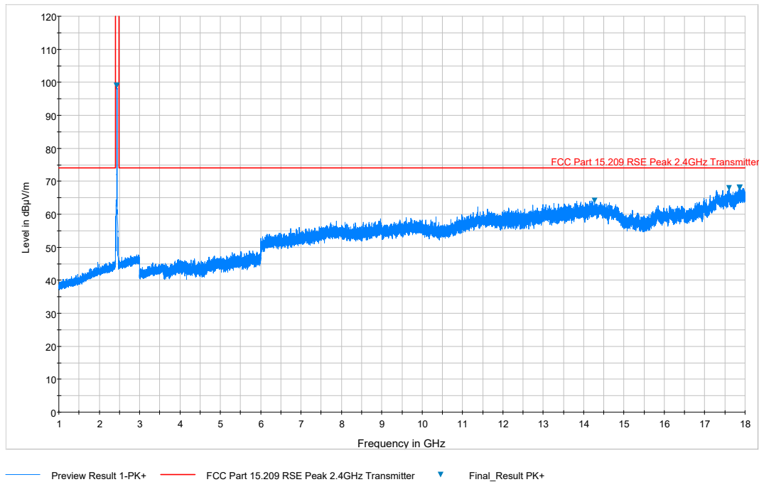
Plot 7-76. Radiated Spurious Plot above 1GHz (802.11b – Ch. 6, Ant. Pol. V)
