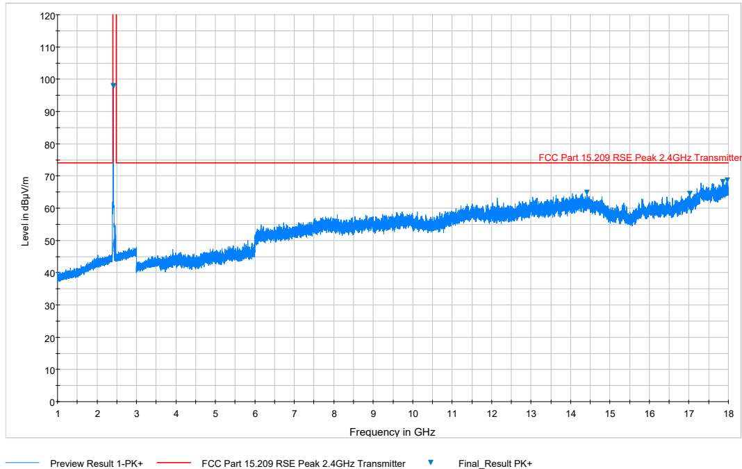
Plot 7-82. Radiated Spurious Plot above 1GHz (802.11b – Ch. 1, Ant. Pol. V)
