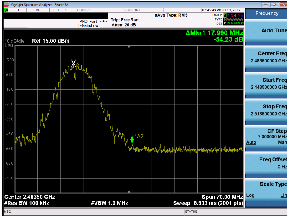
Plot 7-51. Band Edge Plot (802.11b – Ch. 12)
