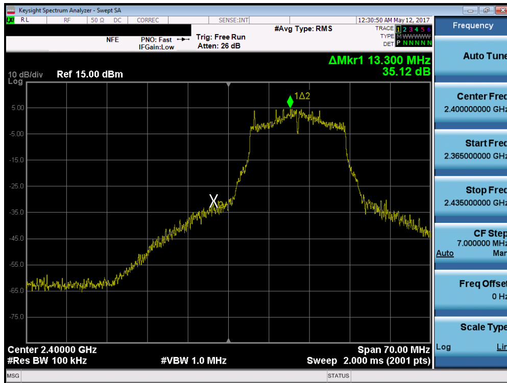
Plot 7-53. Band Edge Plot (802.11g– Ch. 1)
