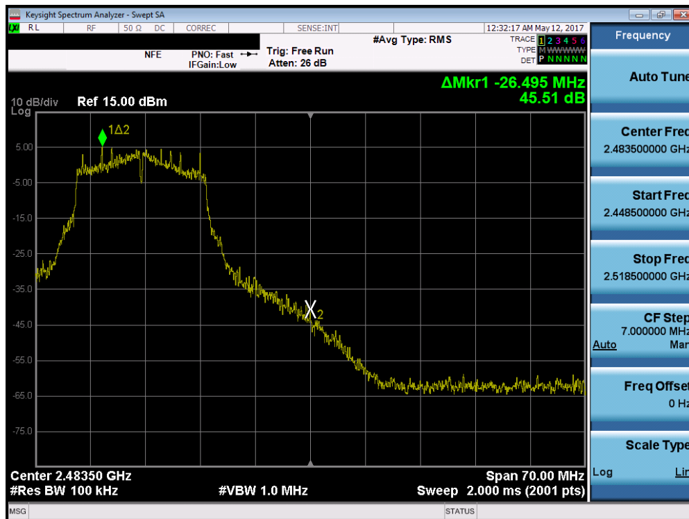
Plot 7-54. Band Edge Plot (802.11g – Ch. 11)
