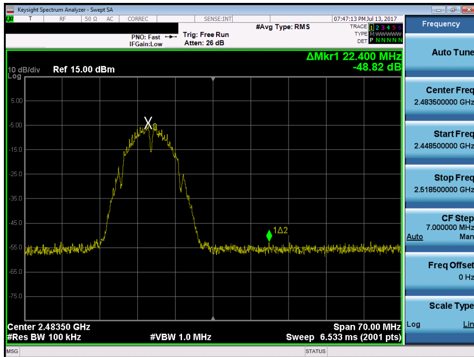
Plot 7-52. Band Edge Plot (802.11b – Ch. 13)
