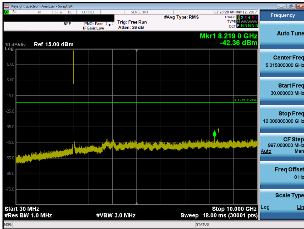
Plot 7-67. Conducted Spurious Plot (802.11b – Ch. 1)
