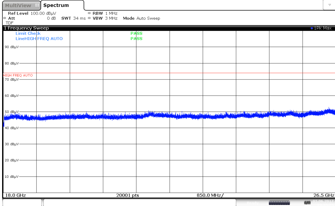
Plot 7-79. Radiated Spurious Plot above 18GHz (Pol. H)
