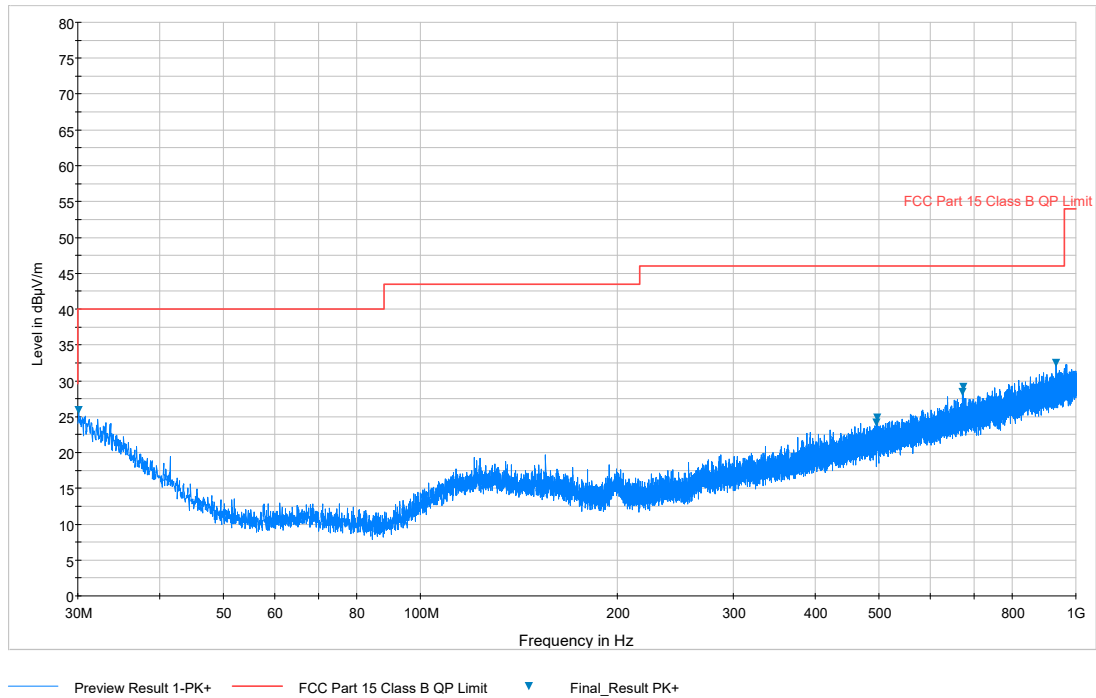
Plot 7-112. Radiated Spurious Plot below 1GHz (Pol. H)
