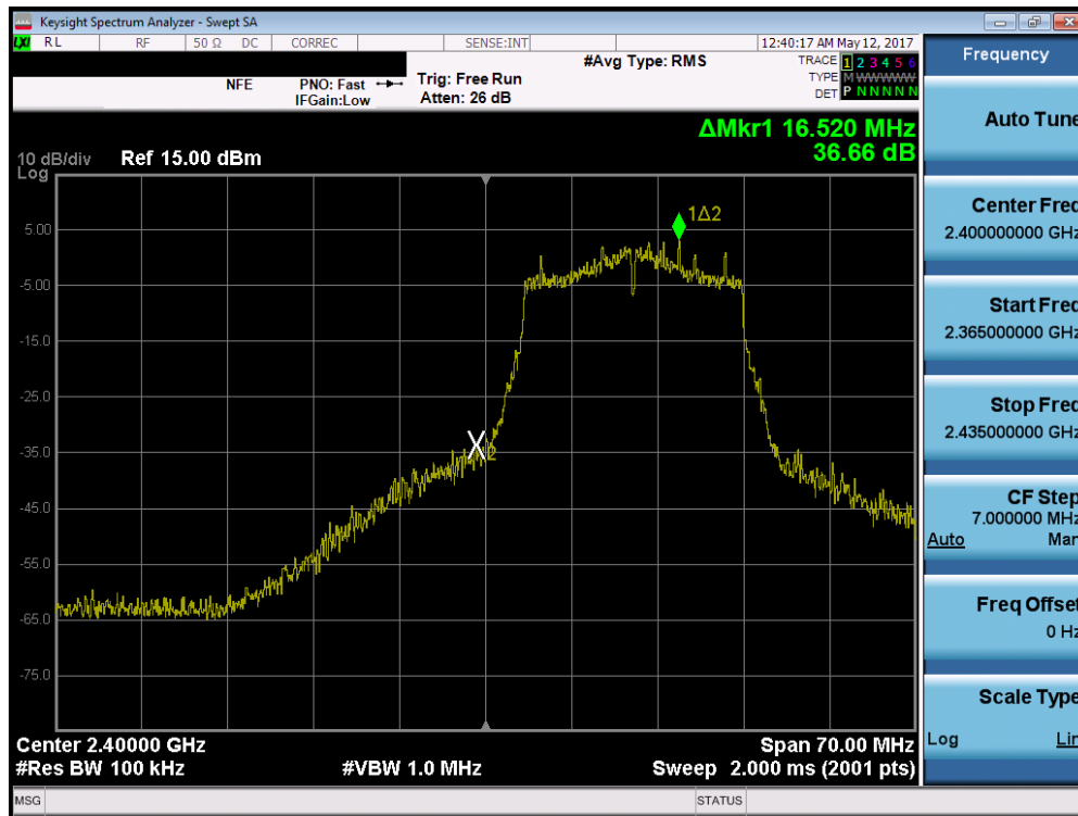
Plot 7-57. Band Edge Plot (802.11n (2.4GHz) – Ch. 1)
