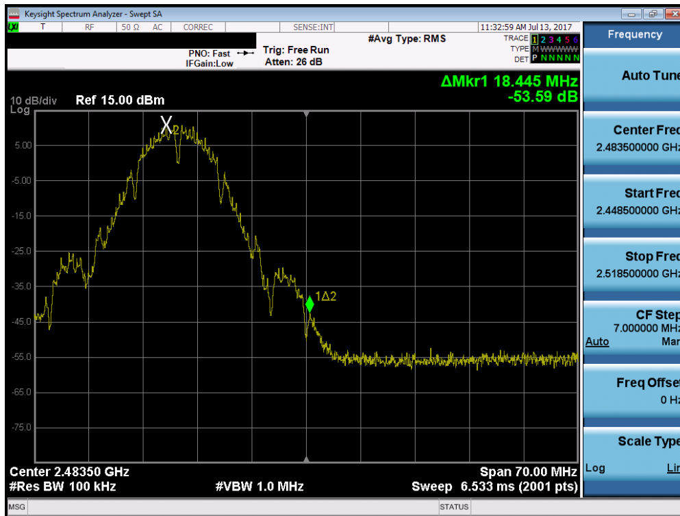
Plot 7-39. Band Edge Plot (802.11b – Ch. 12)
