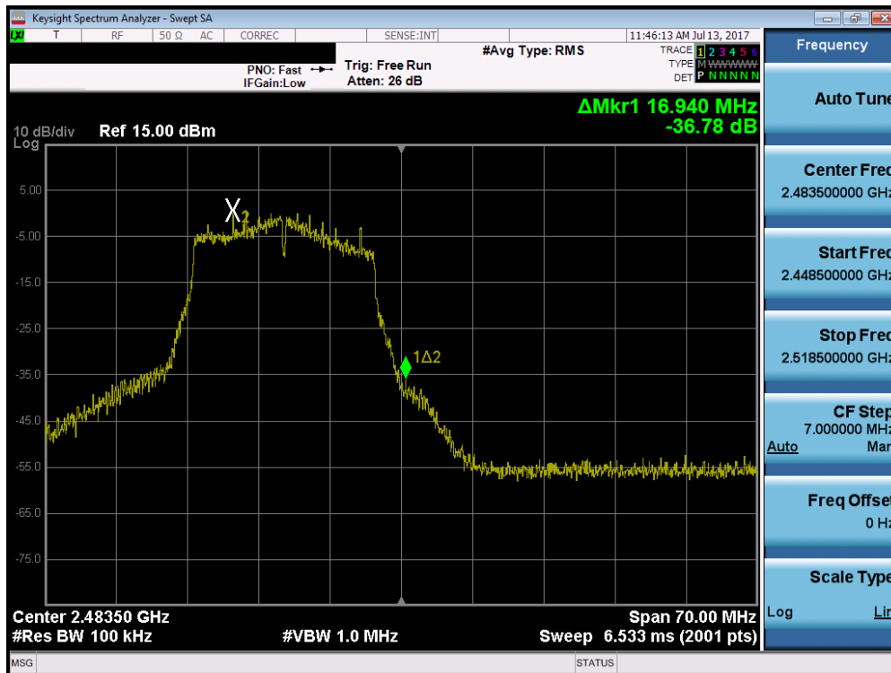
Plot 7-48. Band Edge Plot (802.11n (2.4GHz) – Ch. 13)
