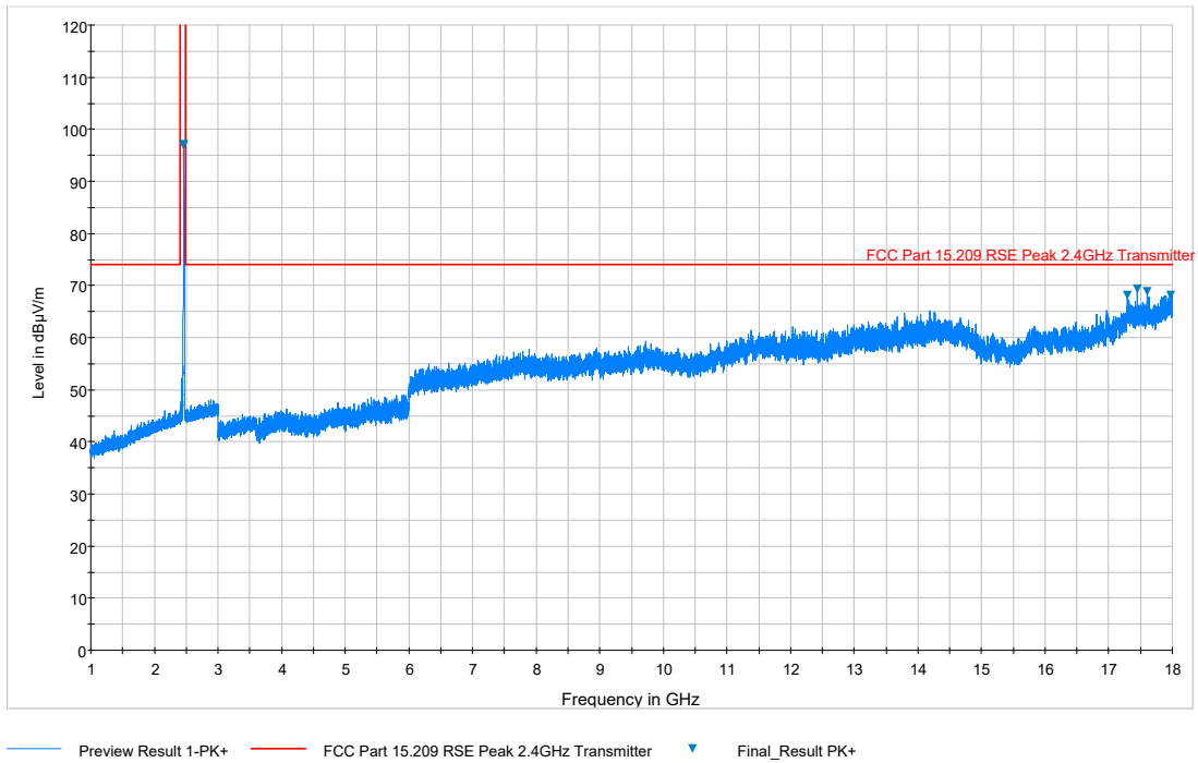
Plot 7-85. Radiated Spurious Plot above 1GHz (802.11b – Ch. 11, Ant. Pol. H)
