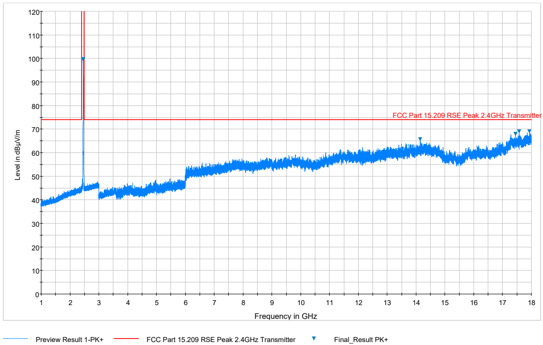
Plot 7-77. Radiated Spurious Plot above 1GHz (802.11b – Ch. 11, Ant. Pol. H)
