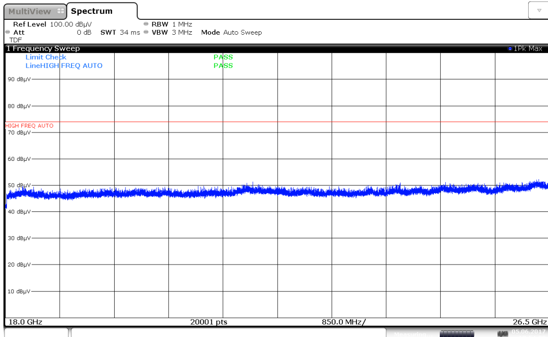
Plot 7-80. Radiated Spurious Plot above 18GHz (Pol. V)
