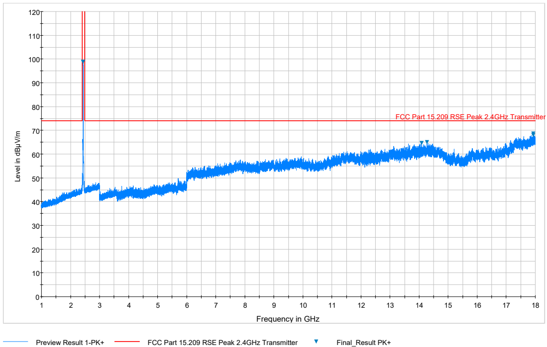
Plot 7-84. Radiated Spurious Plot above 1GHz (802.11b – Ch. 6, Ant. Pol. V)
