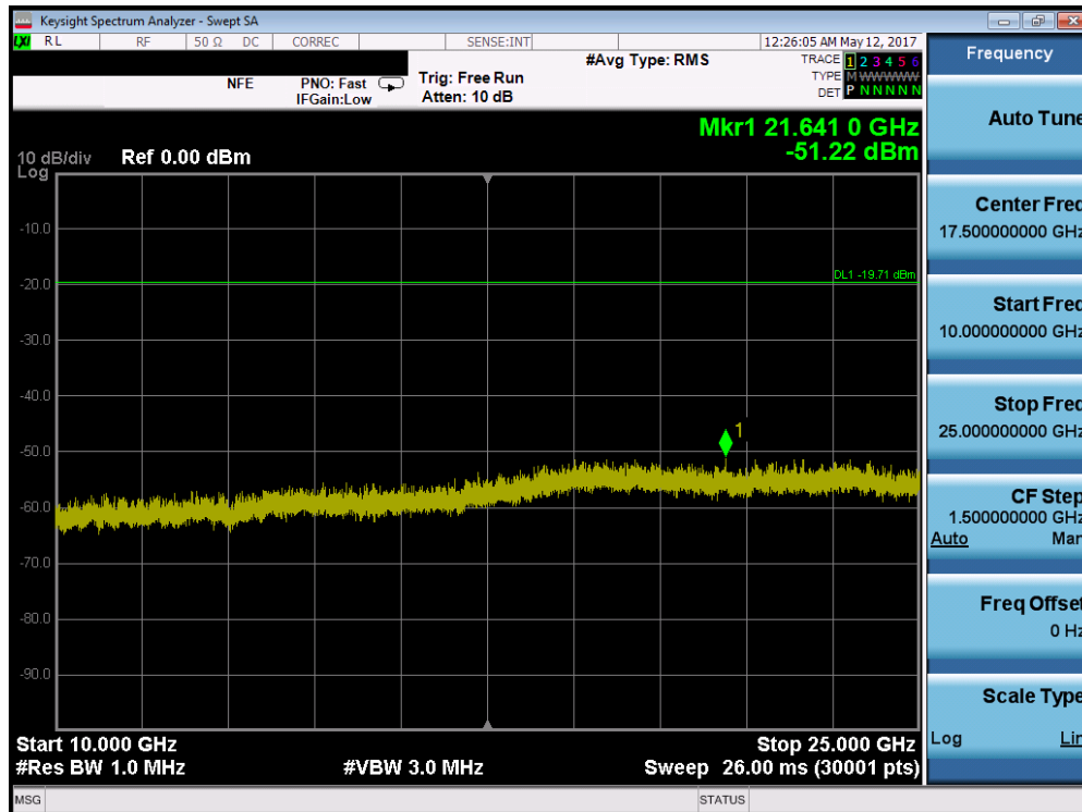
Plot 7-70. Conducted Spurious Plot (802.11b – Ch. 6)
