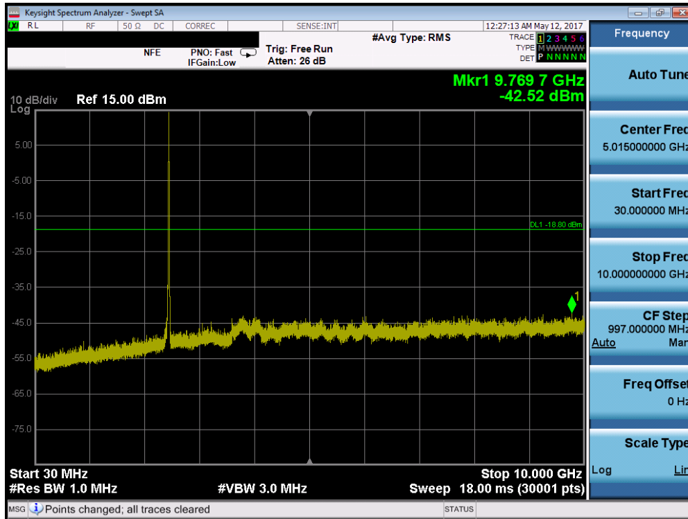
Plot 7-71. Conducted Spurious Plot (802.11b – Ch. 11)
