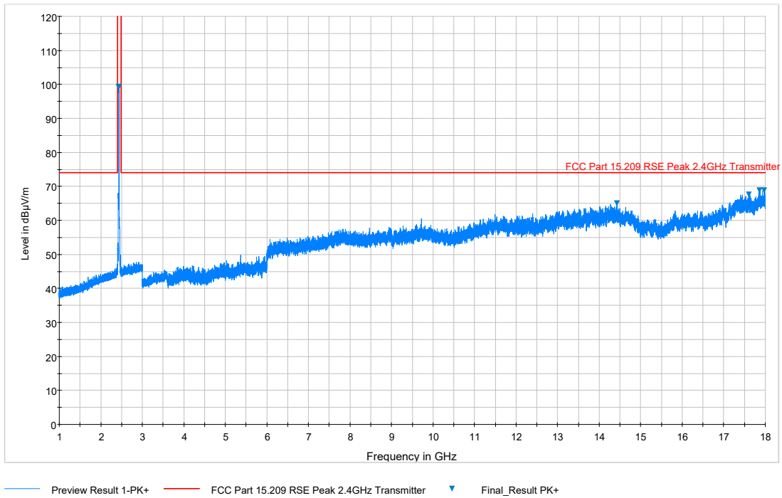
Plot 7-83. Radiated Spurious Plot above 1GHz (802.11b – Ch. 6, Ant. Pol. H)
