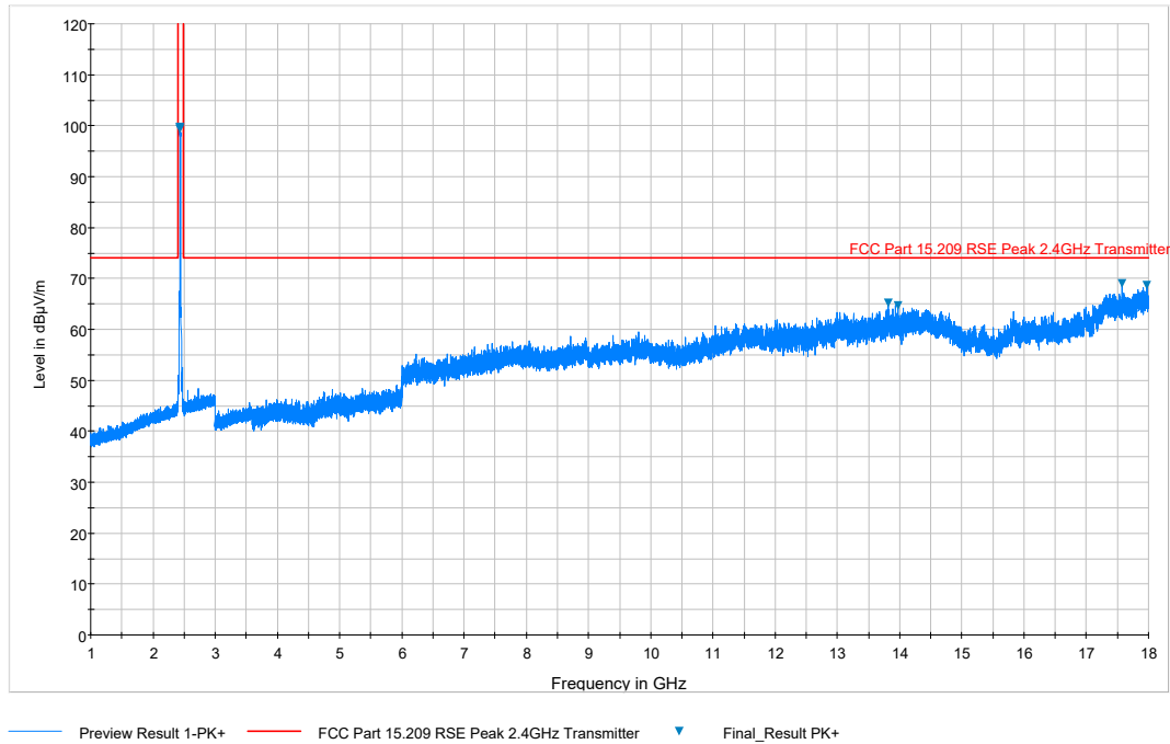
Plot 7-75. Radiated Spurious Plot above 1GHz (802.11b – Ch. 6, Ant. Pol. H)
