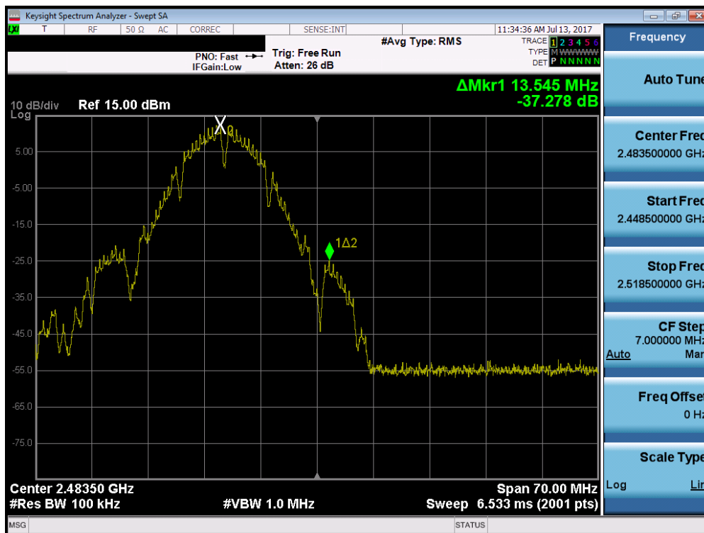
Plot 7-40. Band Edge Plot (802.11b – Ch. 13)
