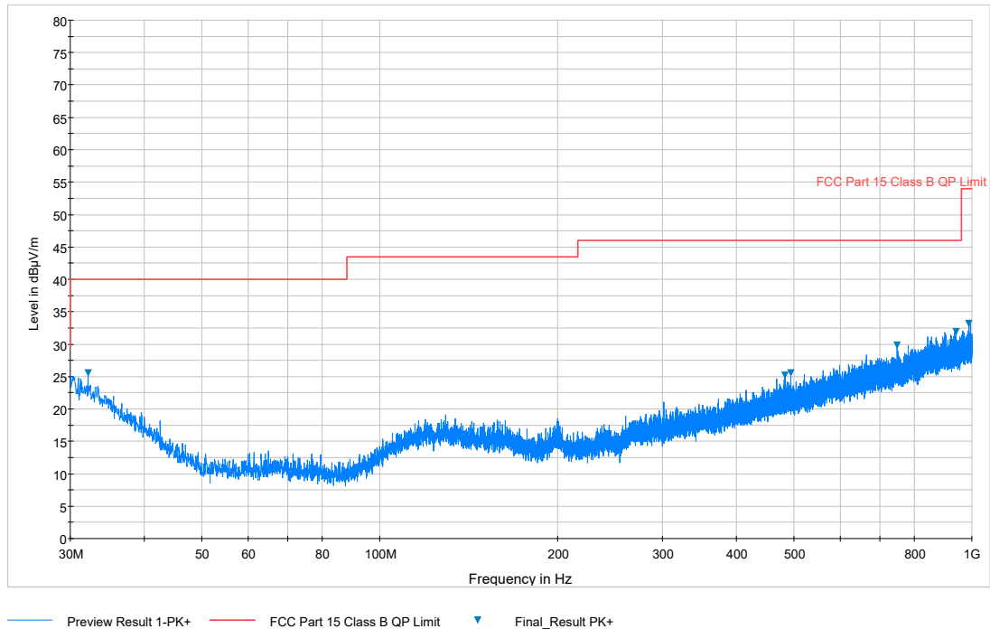
Plot 7-114. Radiated Spurious Plot below 1GHz (Pol. H)
