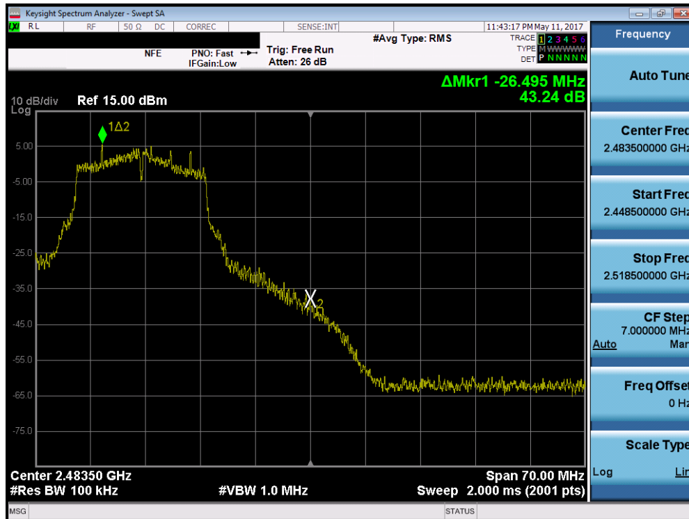
Plot 7-42. Band Edge Plot (802.11g – Ch. 11)
