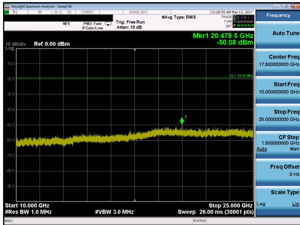
Plot 7-68. Conducted Spurious Plot (802.11b – Ch. 1)
