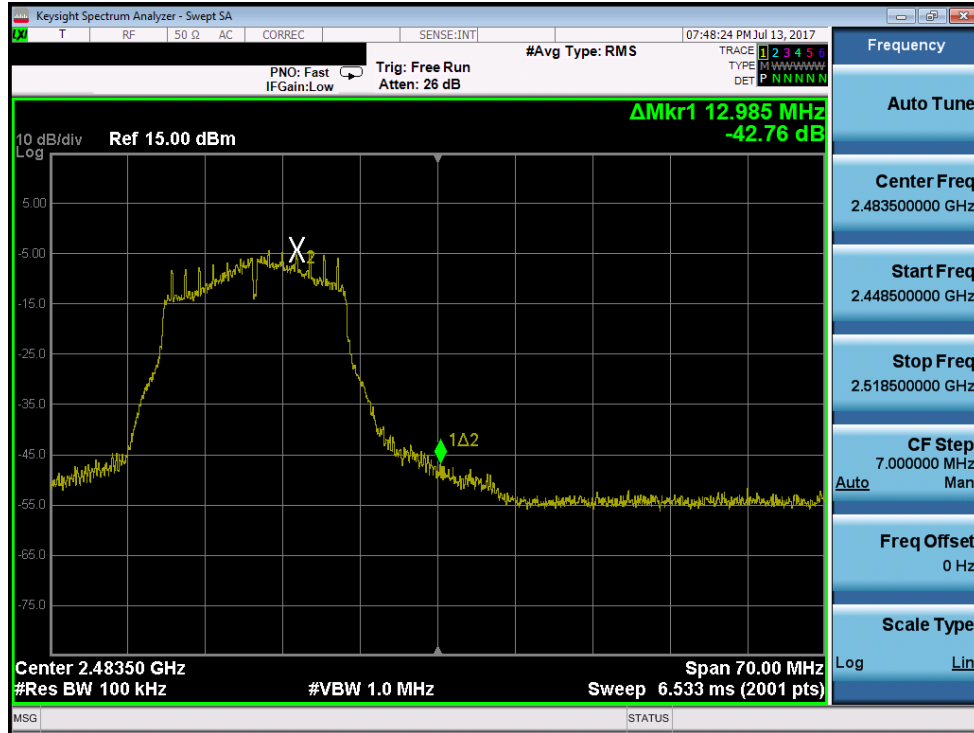
Plot 7-55. Band Edge Plot (802.11g – Ch. 12)
