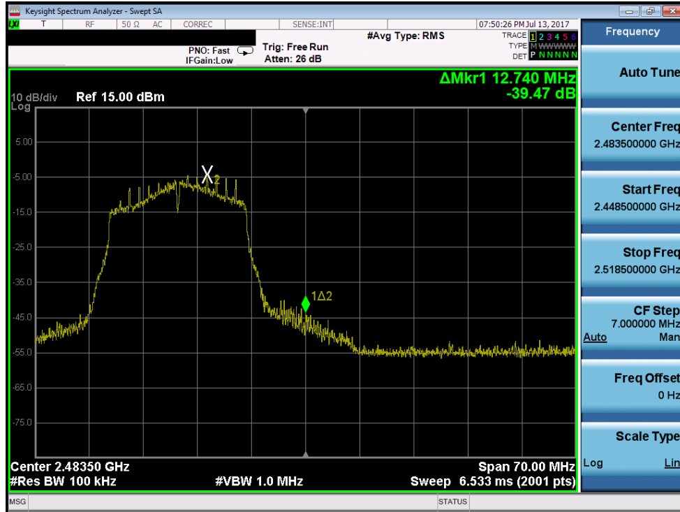
Plot 7-59. Band Edge Plot (802.11n (2.4GHz) – Ch. 12)
