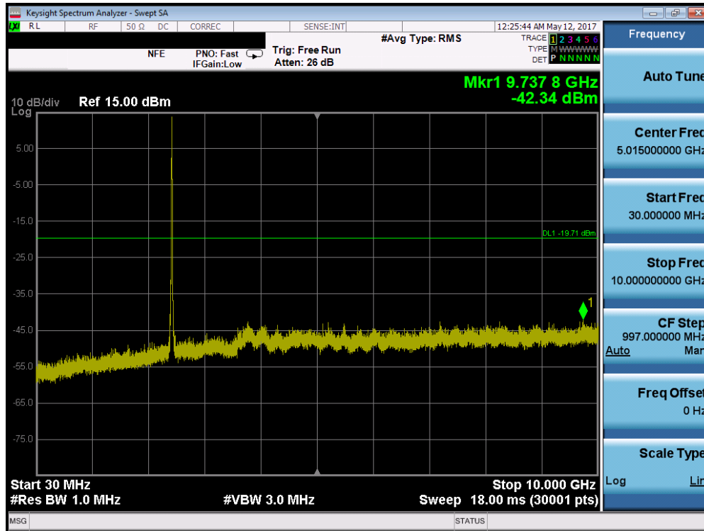
Plot 7-69. Conducted Spurious Plot (802.11b – Ch. 6)
