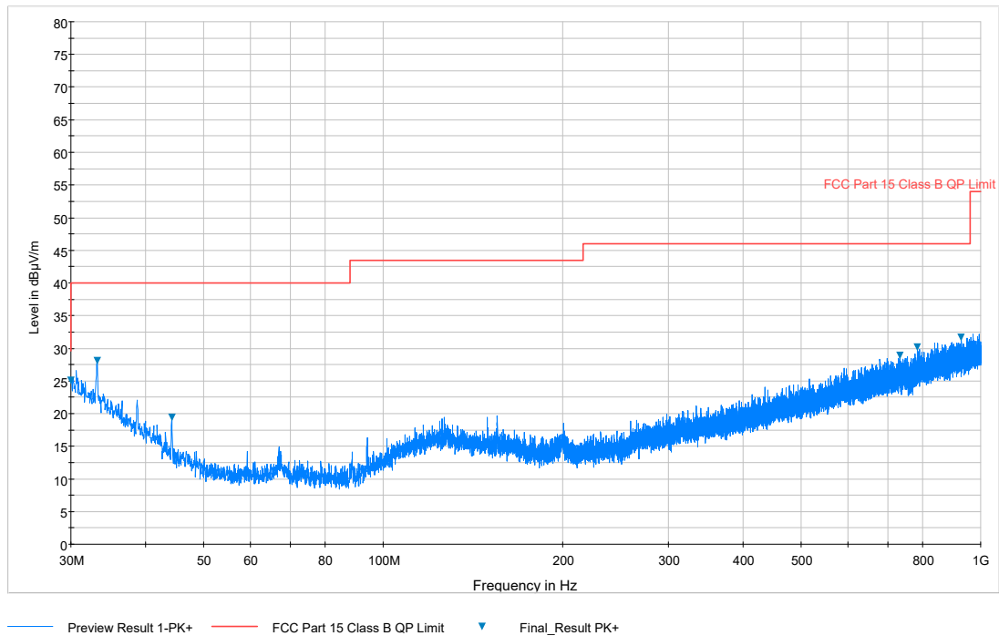
Plot 7-113. Radiated Spurious Plot below 1GHz (Pol. V)
