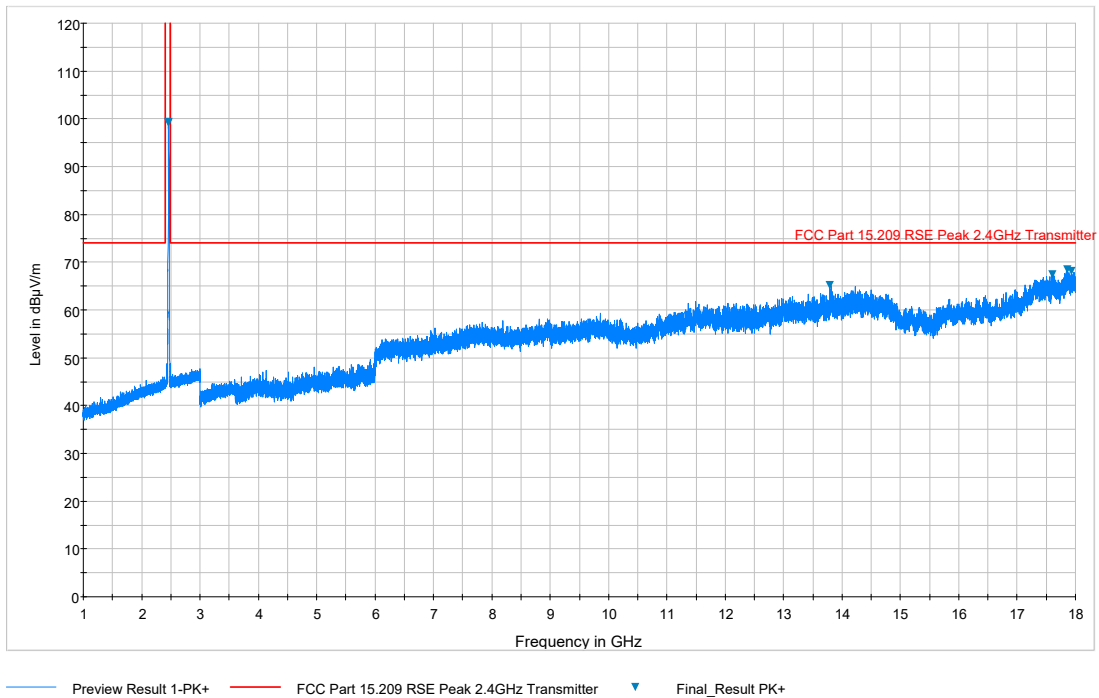
Plot 7-78. Radiated Spurious Plot above 1GHz (802.11b – Ch. 11, Ant. Pol. V)
