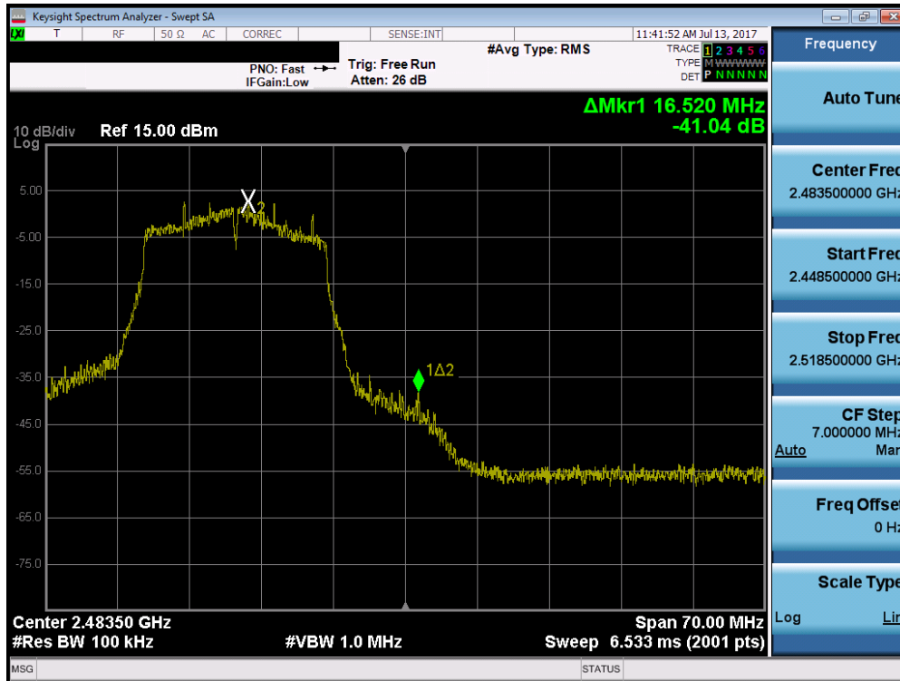
Plot 7-47. Band Edge Plot (802.11n (2.4GHz) – Ch. 12)
