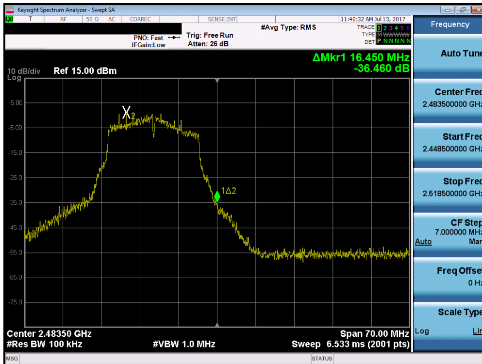
Plot 7-44. Band Edge Plot (802.11g - Ch. 13)
