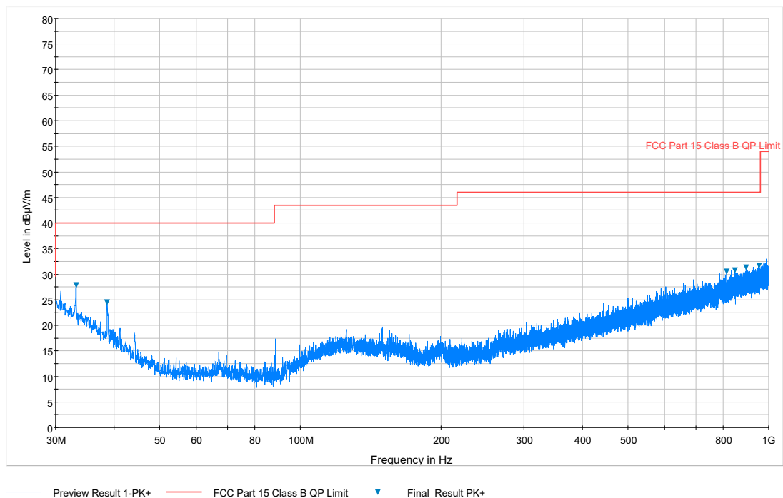
Plot 7-115. Radiated Spurious Plot below 1GHz (Pol. V)
