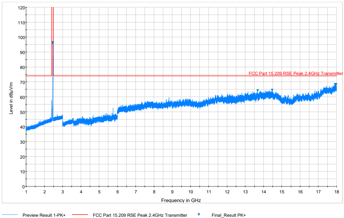
Plot 7-86. Radiated Spurious Plot above 1GHz (802.11b – Ch. 11, Ant. Pol. V)
