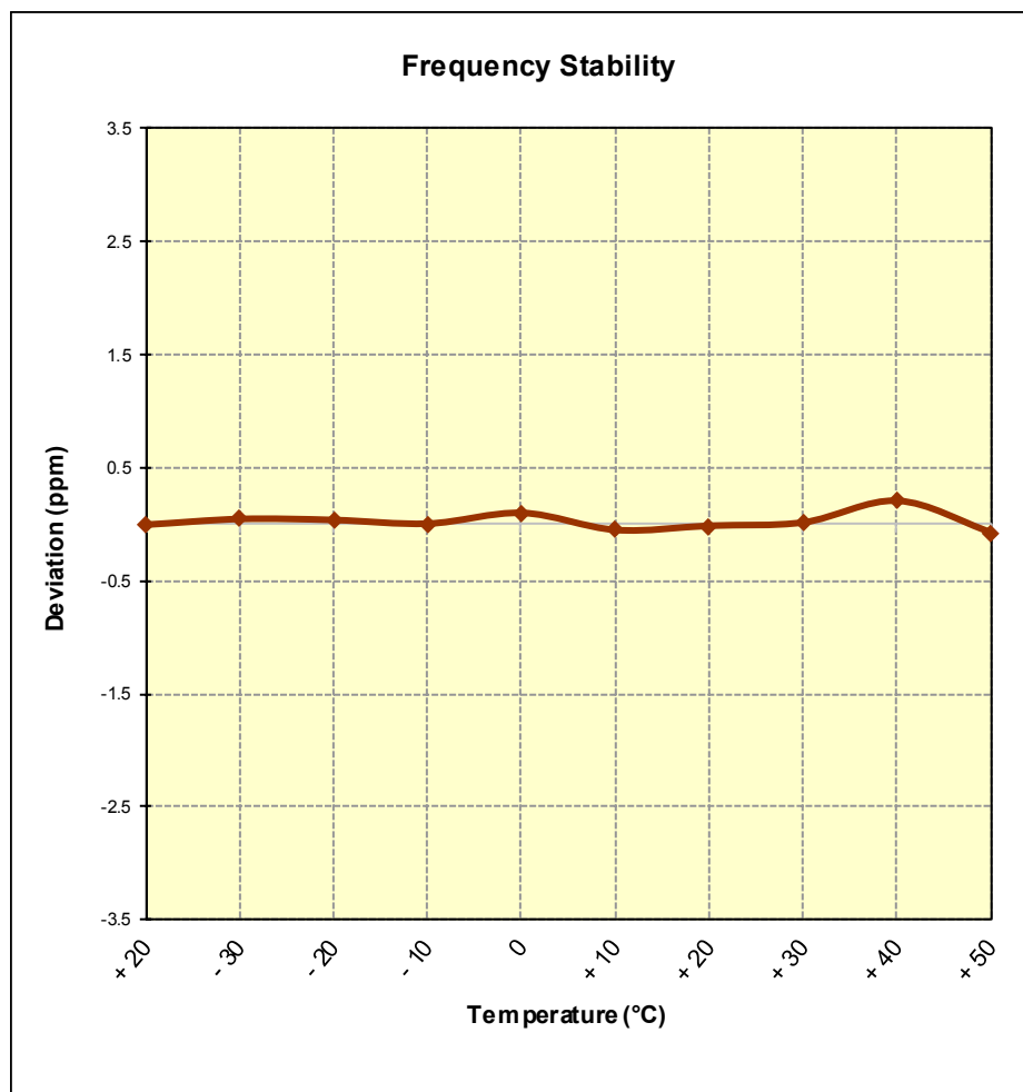
Figure 7-9. Frequency Stability Graph (PCS GPRS Mode – Ch. 661)
