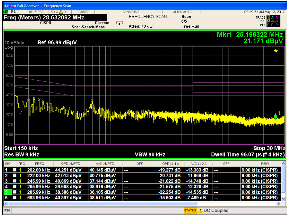
Plot 7-39. Line Conducted Plot with Bluetooth LE (L1)
