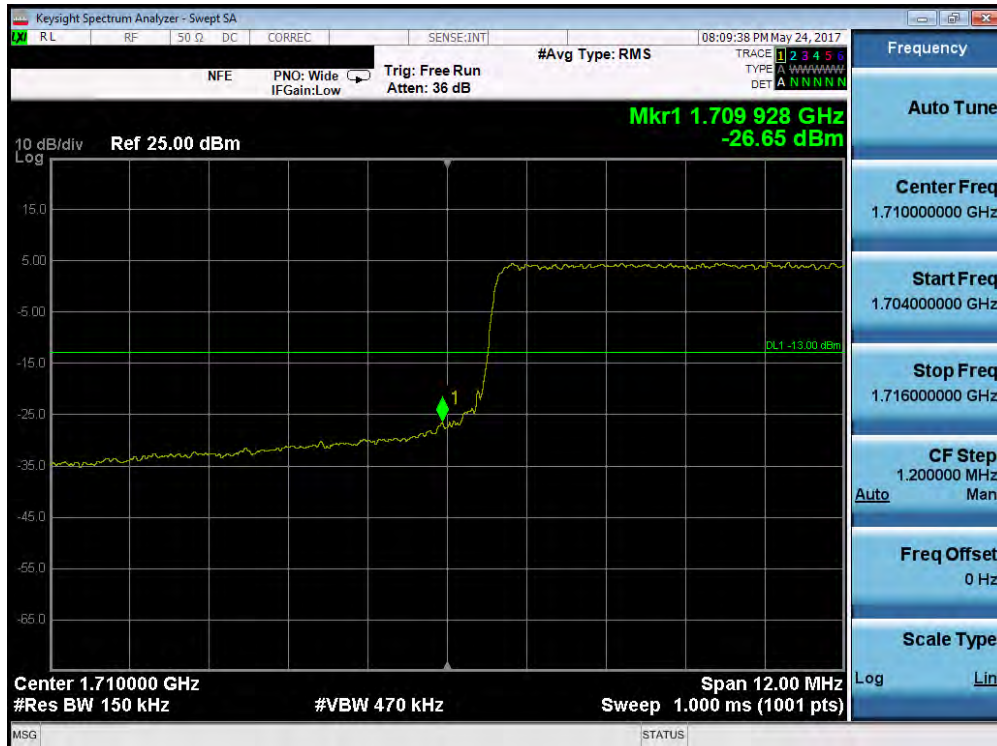
Plot 7-147. Lower Band Edge Plot (Band 4 – 15.0MHz QPSK – RB Size 75)
