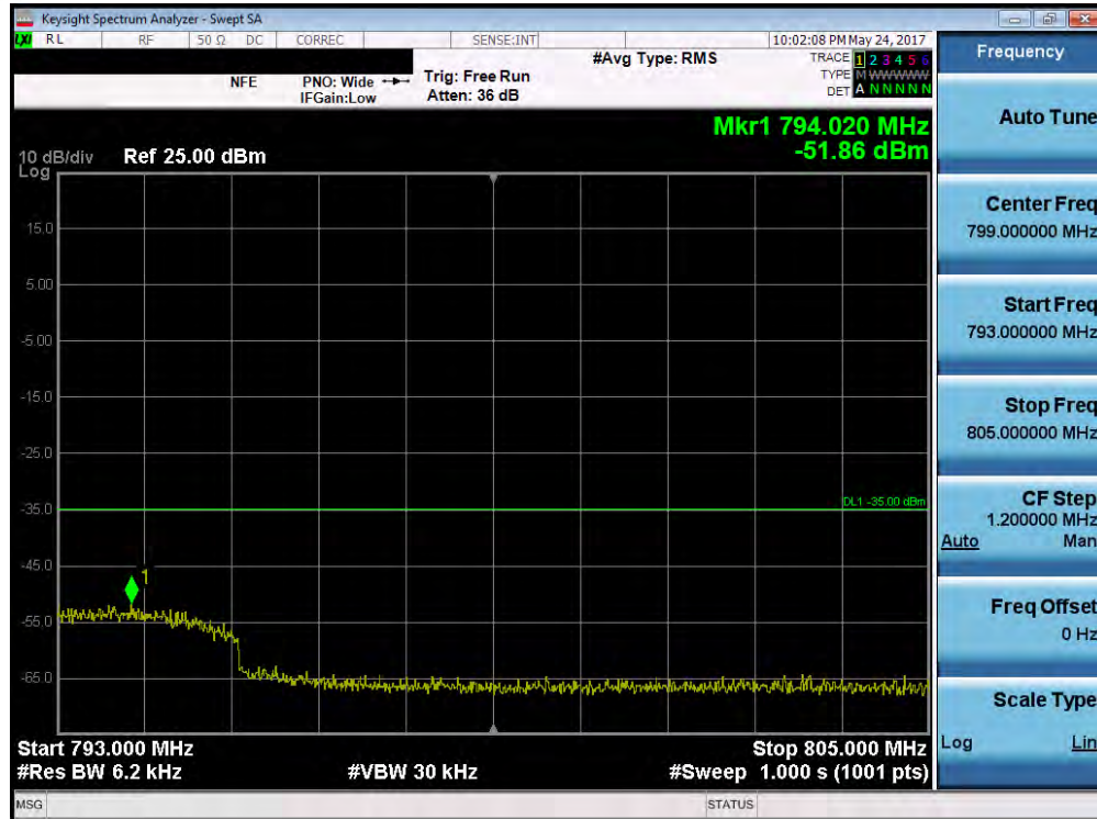
Plot 7-120. Upper Emission Mask Edge Plot (Band 13 – 10.0MHz QPSK – RB Size 50)
