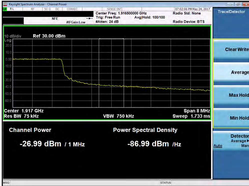
Plot 7-178. Upper Extended Band Edge Plot (Band 25 – 10.0MHz QPSK – RB Size 50)
