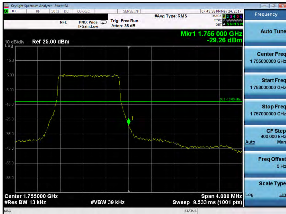
Plot 7-133. Upper Band Edge Plot (Band 4 – 1.4MHz QPSK – RB Size 6)
