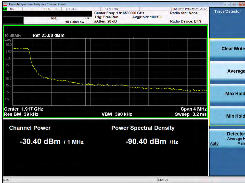
Plot 7-160. Upper Extended Band Edge Plot (Band 25 – 1.4MHz QPSK – RB Size 6)
