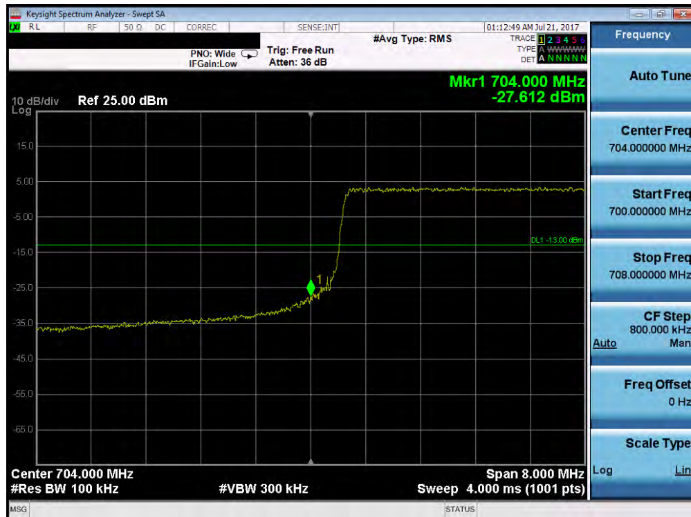
Plot 7-111. Lower Band Edge Plot (Band 17 – 10.0MHz QPSK – RB Size 50)
