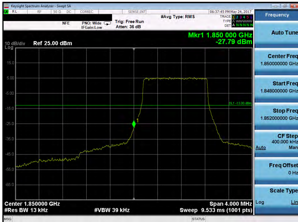
Plot 7-155. Lower Band Edge Plot (Band 2/25 – 1.4MHz QPSK – RB Size 6)
