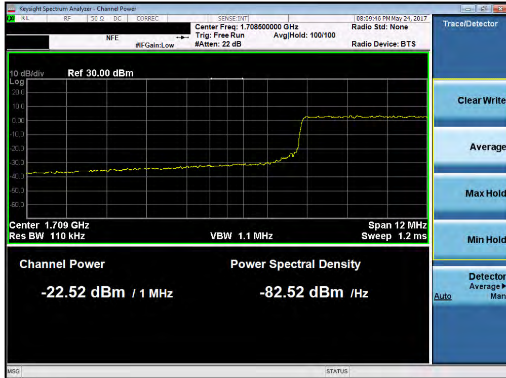
Plot 7-148. Lower Extended Band Edge Plot (Band 4 – 15.0MHz QPSK – RB Size 75)
