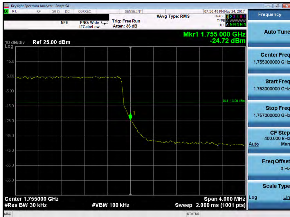
Plot 7-137. Upper Band Edge Plot (Band 4 – 3.0MHz QPSK – RB Size 15)
