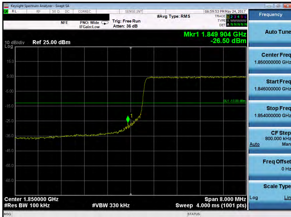
Plot 7-173. Lower Band Edge Plot (Band 2/25 – 10.0MHz QPSK – RB Size 50)
