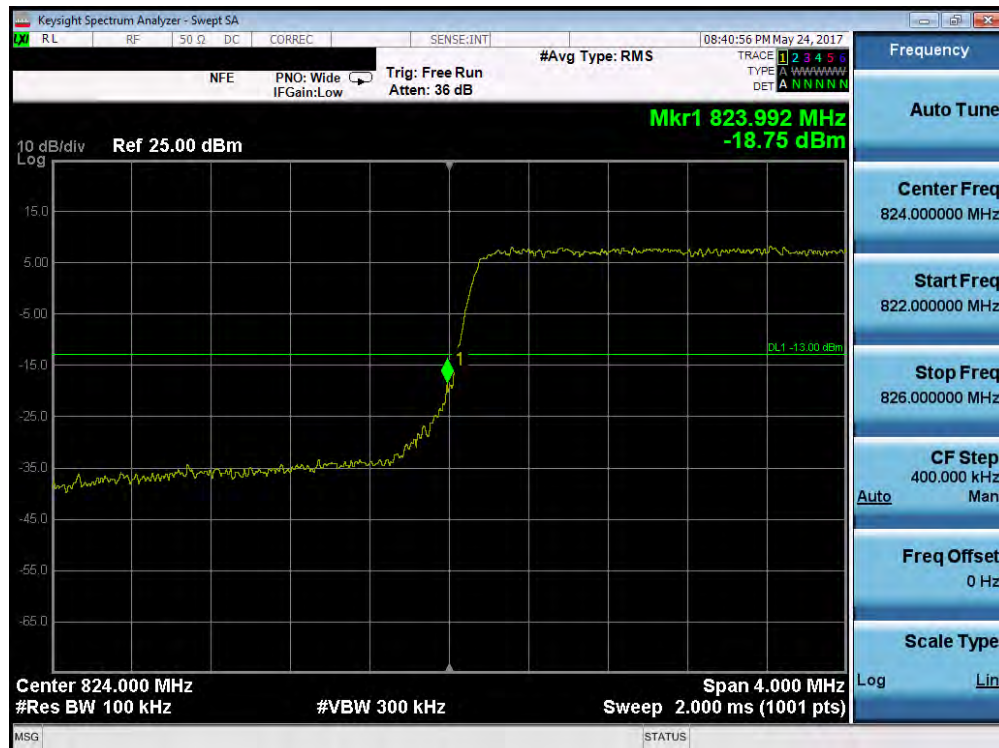
Plot 7-123. Lower Band Edge Plot (Band 5/26 – 3.0MHz QPSK – RB Size 15)
