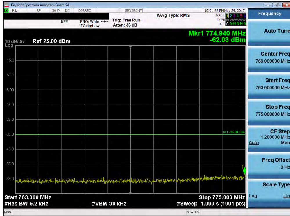
Plot 7-118. Lower Emission Mask Edge Plot (Band 13 – 10.0MHz QPSK – RB Size 50)
