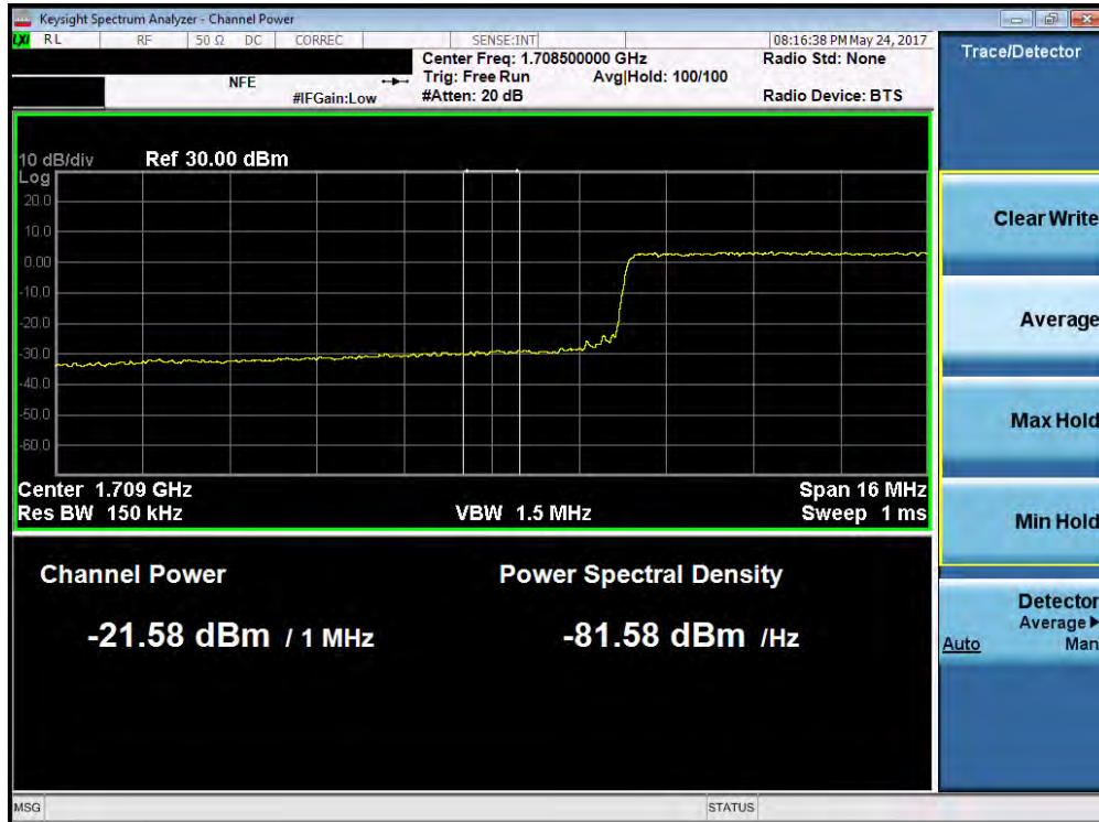
Plot 7-152. Lower Extended Band Edge Plot (Band 4 – 20.0MHz QPSK – RB Size 100)
