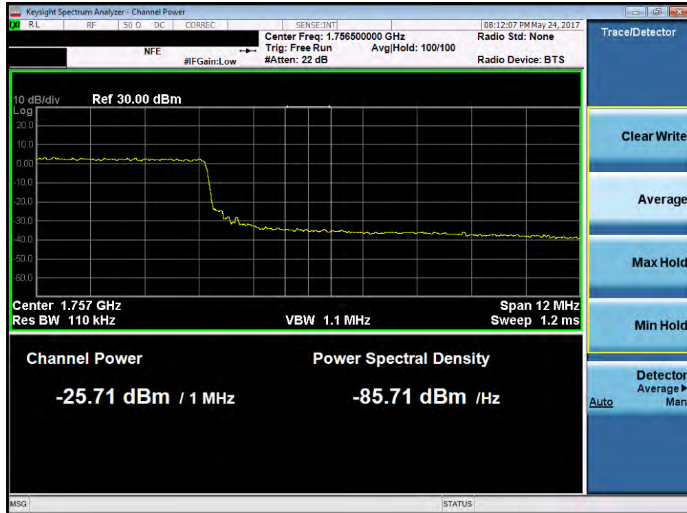
Plot 7-150. Upper Extended Band Edge Plot (Band 4 – 15.0MHz QPSK – RB Size 75)
