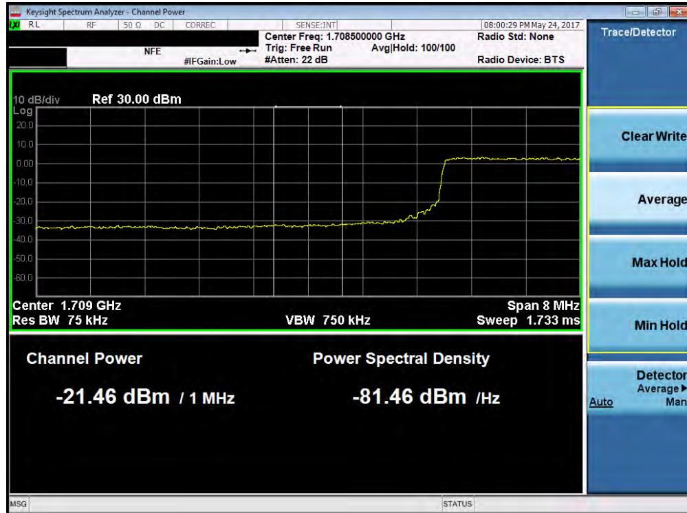
Plot 7-144. Lower Extended Band Edge Plot (Band 4 – 10.0MHz QPSK – RB Size 50)
