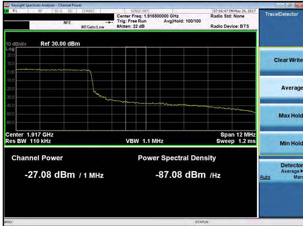
Plot 7-184. Upper Extended Band Edge Plot (Band 25 – 15.0MHz QPSK – RB Size 75)
