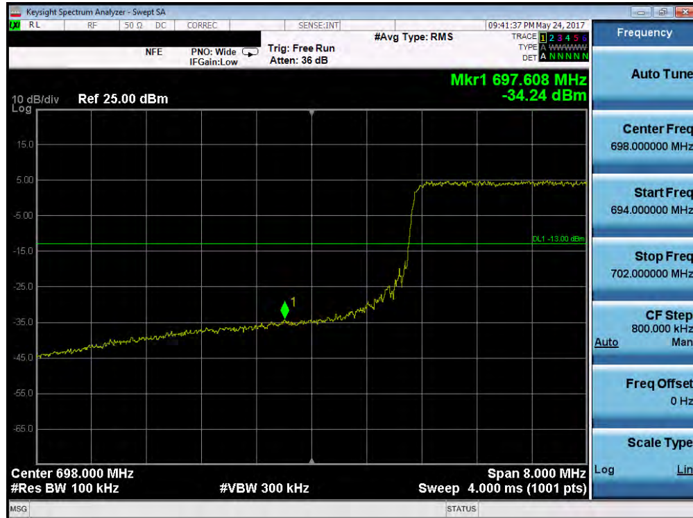
Plot 7-110. Lower Band Edge Plot (Band 12 – 10.0MHz QPSK – RB Size 50)
