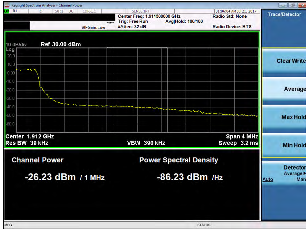
Plot 7-164. Upper Extended Band Edge Plot (Band 2 – 3.0MHz QPSK – RB Size 15)
