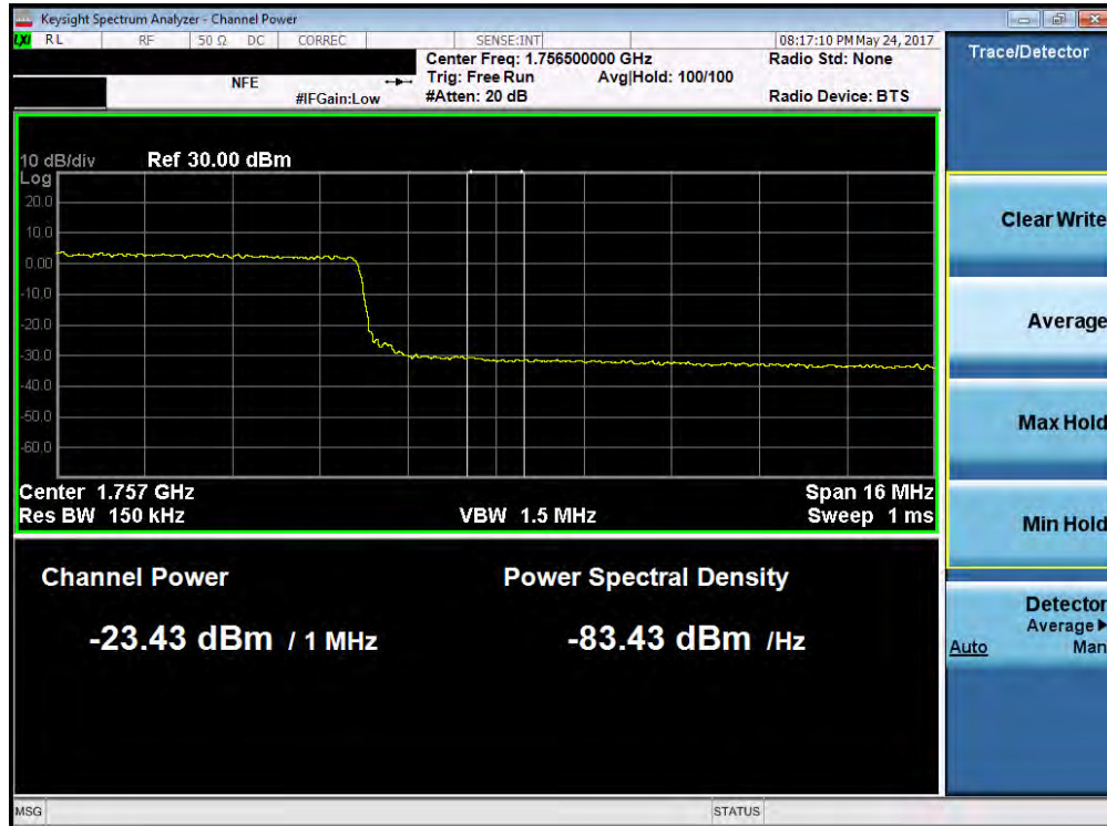
Plot 7-154. Upper Extended Band Edge Plot (Band 4 – 20.0MHz QPSK – RB Size 100)
