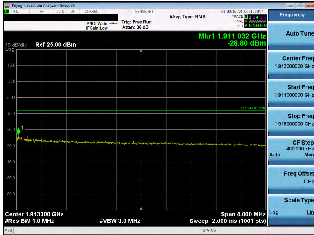
Plot 7-182. Upper Extended Band Edge Plot (Band 2 – 15.0MHz QPSK – RB Size 75)
