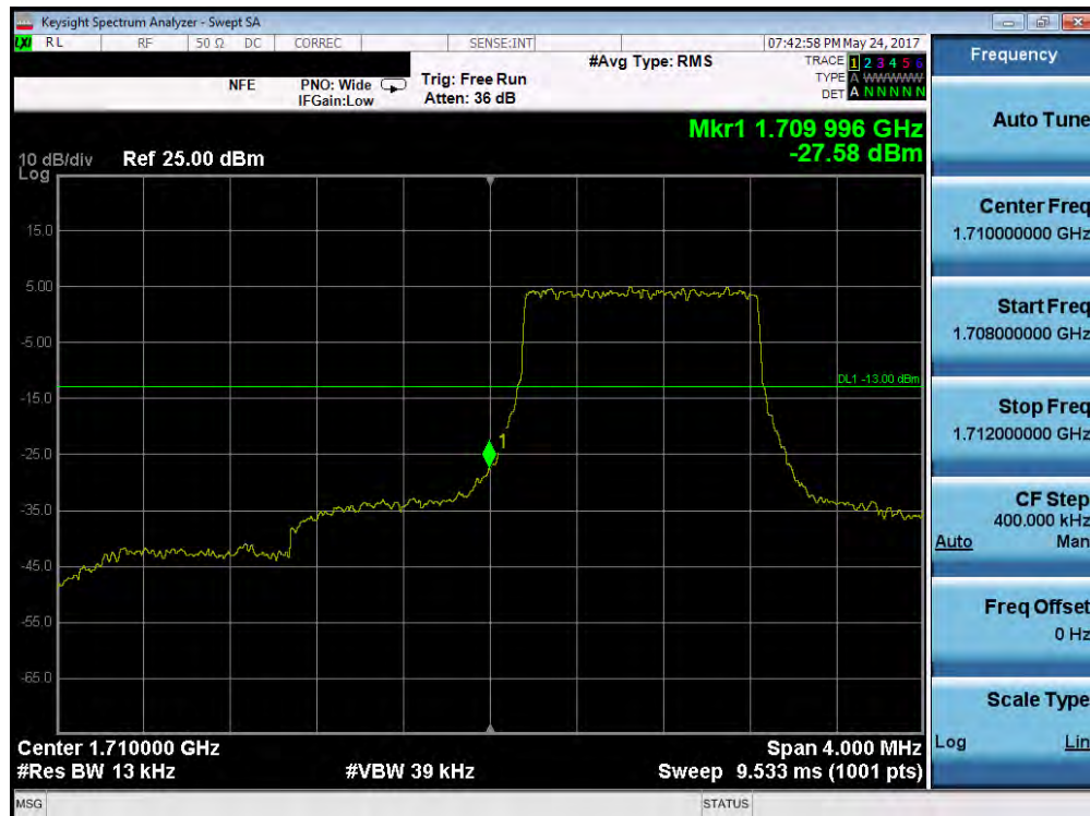
Plot 7-131. Lower Band Edge Plot (Band 4 – 1.4MHz QPSK – RB Size 6)
