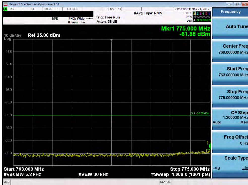
Plot 7-114. Lower Emission Mask Edge Plot (Band 13 - 5.0MHz QPSK - RB Size 25)
