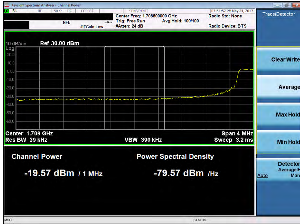
Plot 7-140. Lower Extended Band Edge Plot (Band 4 – 5.0MHz QPSK – RB Size 25)
