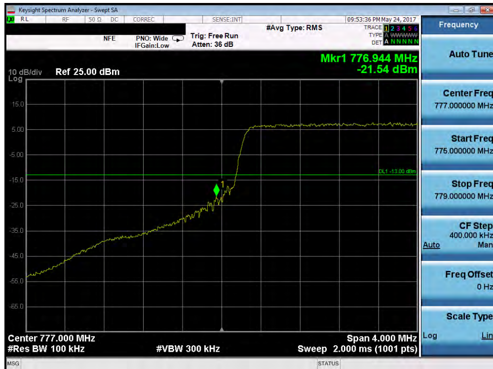
Plot 7-113. Lower Band Edge Plot (Band 13 - 5.0MHz QPSK - RB Size 25)
