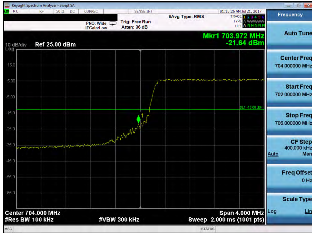
Plot 7-108. Lower Band Edge Plot (Band 17 – 5.0MHz QPSK – RB Size 25)
