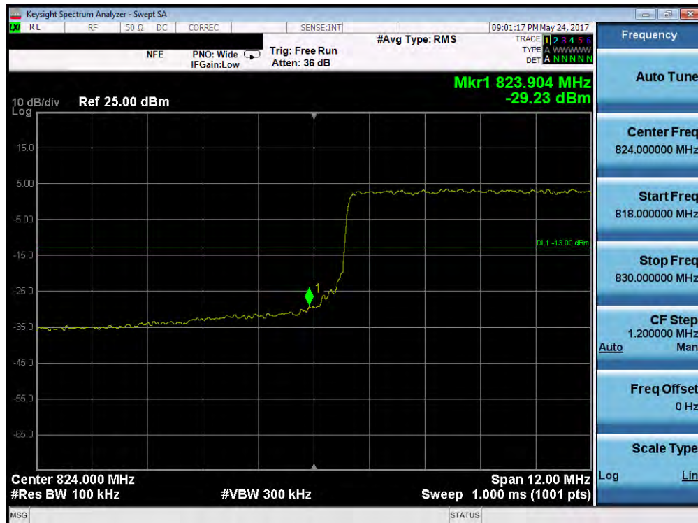
Plot 7-129. Lower Band Edge Plot (Band 26 - 15.0MHz QPSK - RB Size 75)
