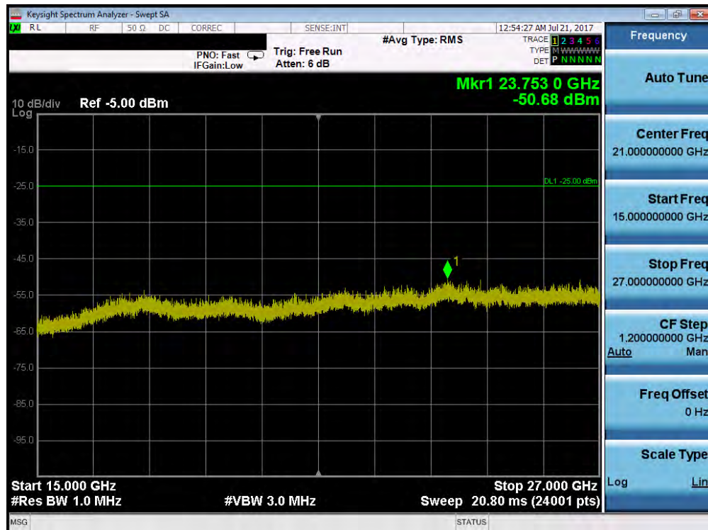
Plot 7-102. Conducted Spurious Plot (Band 41 – 5.0MHz QPSK – RB Size 1, RB Offset 0 – High Channel)
