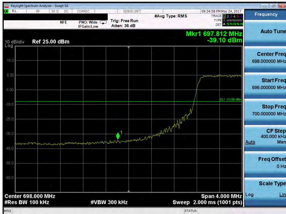
Plot 7-107. Lower Band Edge Plot (Band 12 - 5.0MHz QPSK - RB Size 25)
