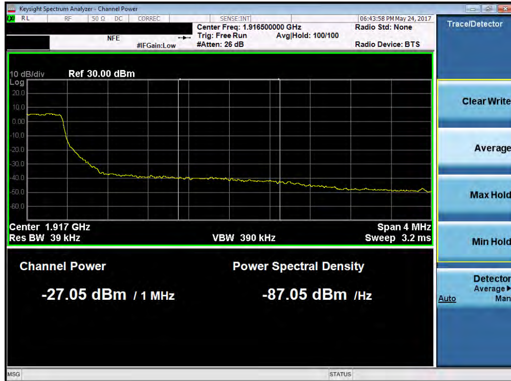
Plot 7-166. Upper Extended Band Edge Plot (Band 25 – 3.0MHz QPSK – RB Size 15)
