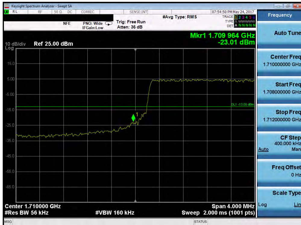
Plot 7-139. Lower Band Edge Plot (Band 4 – 5.0MHz QPSK – RB Size 25)
