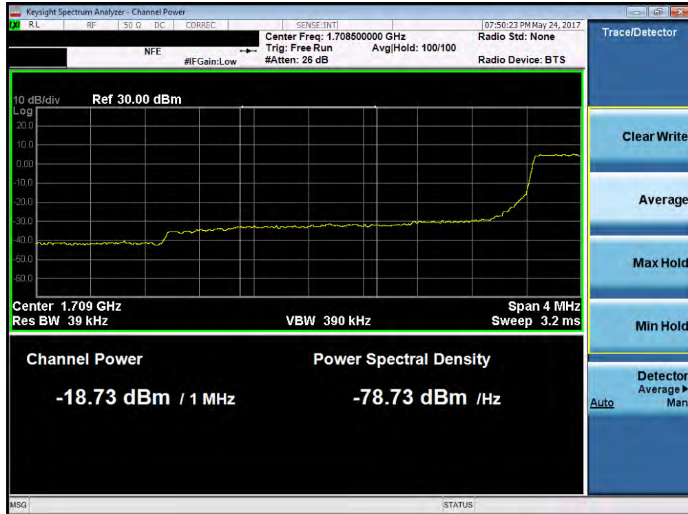
Plot 7-136. Lower Extended Band Edge Plot (Band 4 – 3.0MHz QPSK – RB Size 15)
