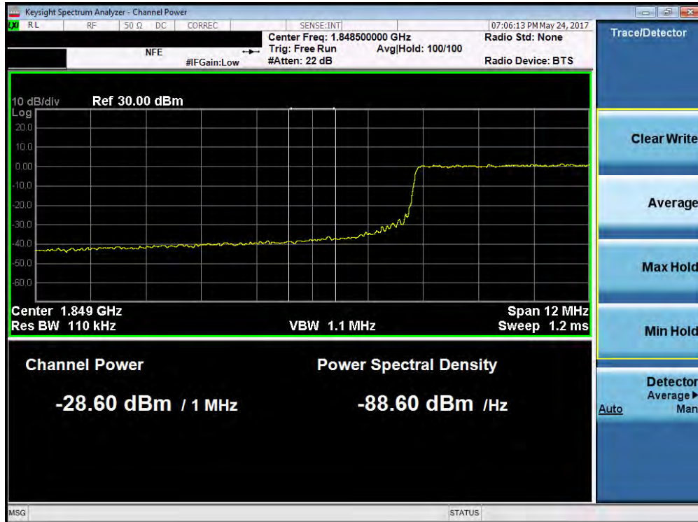
Plot 7-180. Lower Extended Band Edge Plot (Band 2/25 – 15.0MHz QPSK – RB Size 75)
