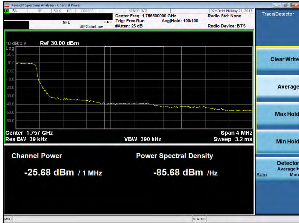
Plot 7-134. Upper Extended Band Edge Plot (Band 4 – 1.4MHz QPSK – RB Size 6)
