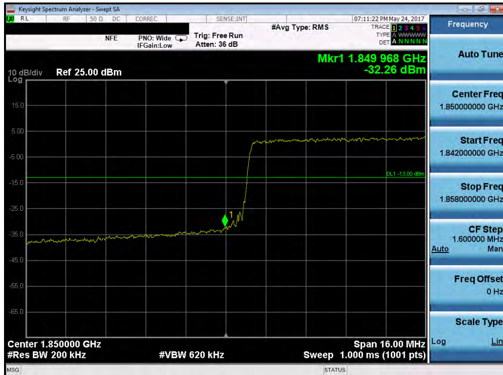
Plot 7-185. Lower Band Edge Plot (Band 2/25 – 20.0MHz QPSK – RB Size 100)
