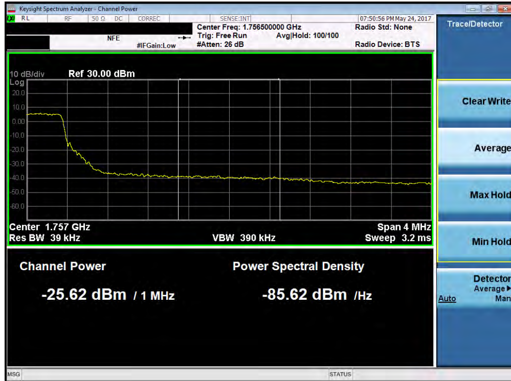
Plot 7-138. Upper Extended Band Edge Plot (Band 4 – 3.0MHz QPSK – RB Size 15)
