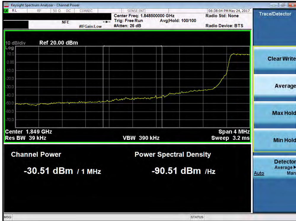
Plot 7-156. Lower Extended Band Edge Plot (Band 2/25 – 1.4MHz QPSK – RB Size 6)
