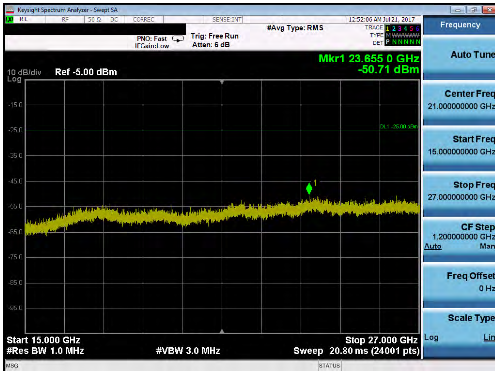
Plot 7-96. Conducted Spurious Plot (Band 41 – 5.0MHz QPSK – RB Size 1, RB Offset 0 – Low Channel)
