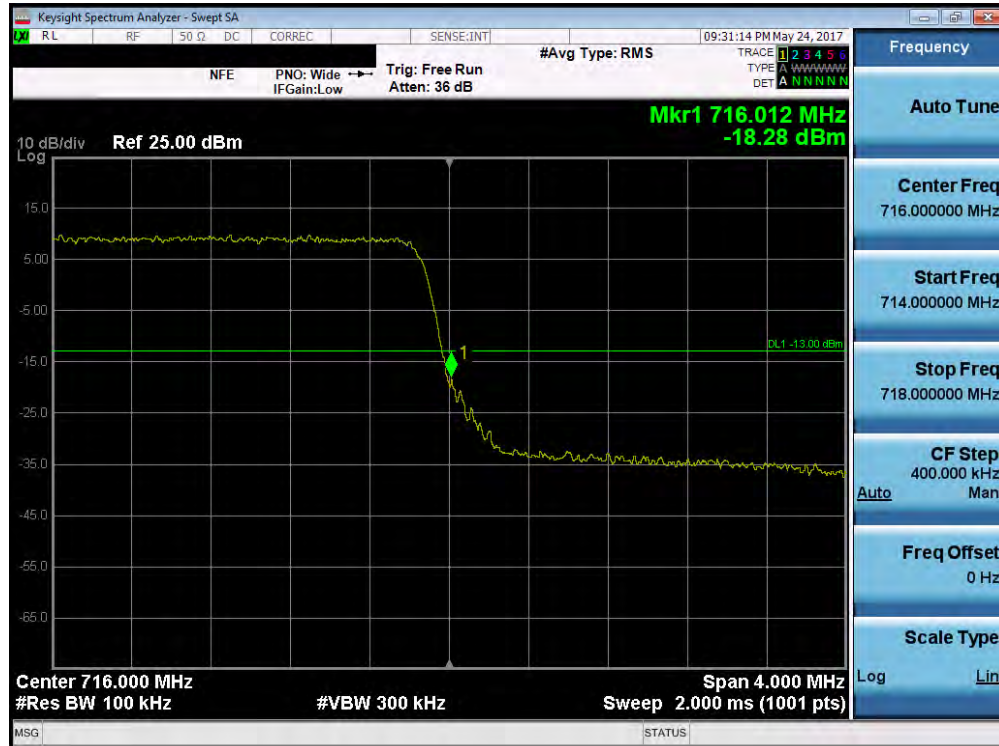
Plot 7-106. Upper Band Edge Plot (Band 12 - 3.0MHz QPSK - RB Size 15)
