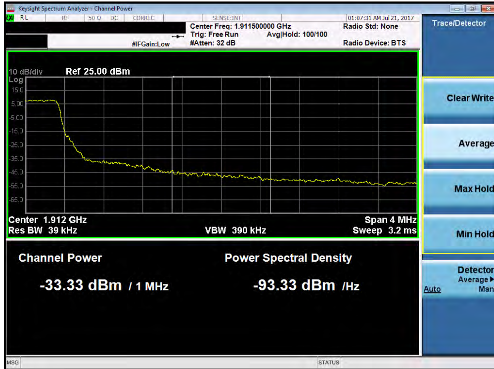
Plot 7-158. Upper Extended Band Edge Plot (Band 2 – 1.4MHz QPSK – RB Size 6)
