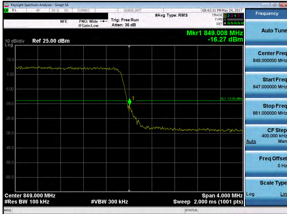
Plot 7-124. Upper Band Edge Plot (Band 5/26 – 3.0MHz QPSK – RB Size 15)
