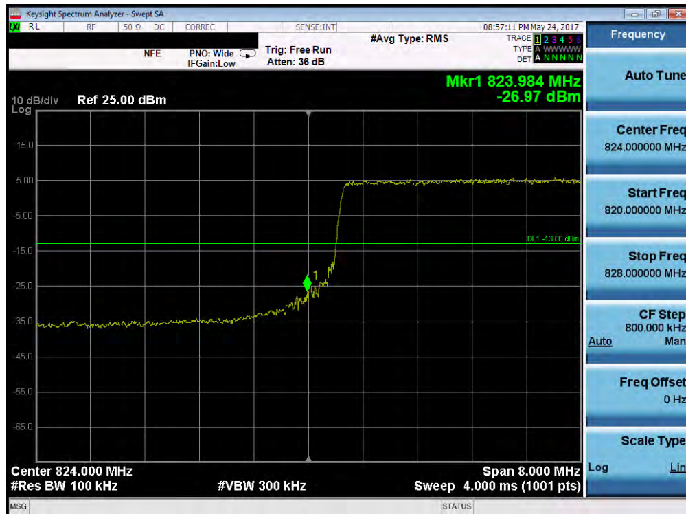
Plot 7-127. Lower Band Edge Plot (Band 5/26 - 10.0MHz QPSK - RB Size 50)
