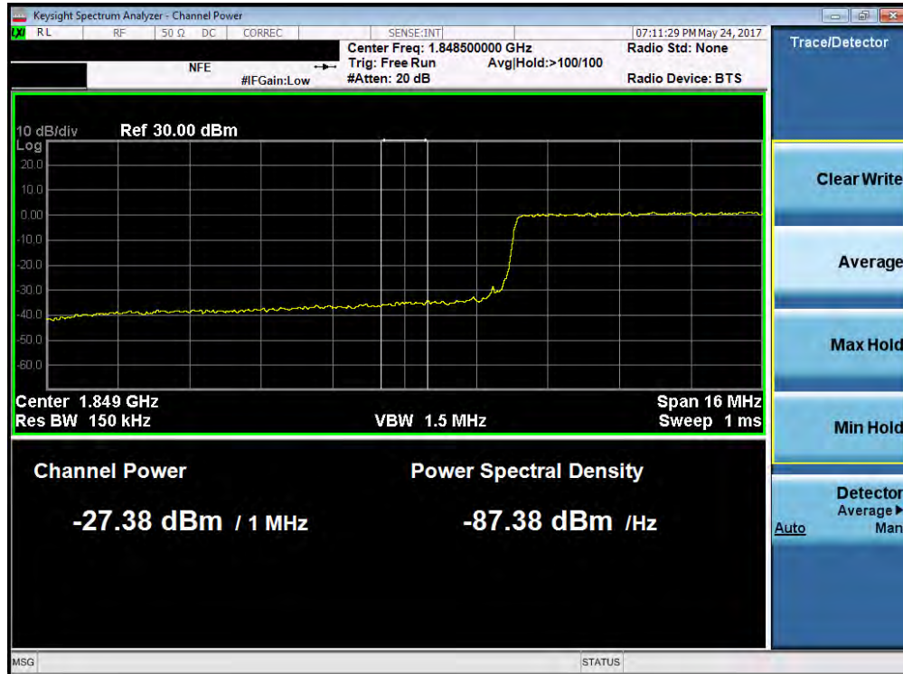
Plot 7-186. Lower Extended Band Edge Plot (Band 2/25 – 20.0MHz QPSK – RB Size 100)
