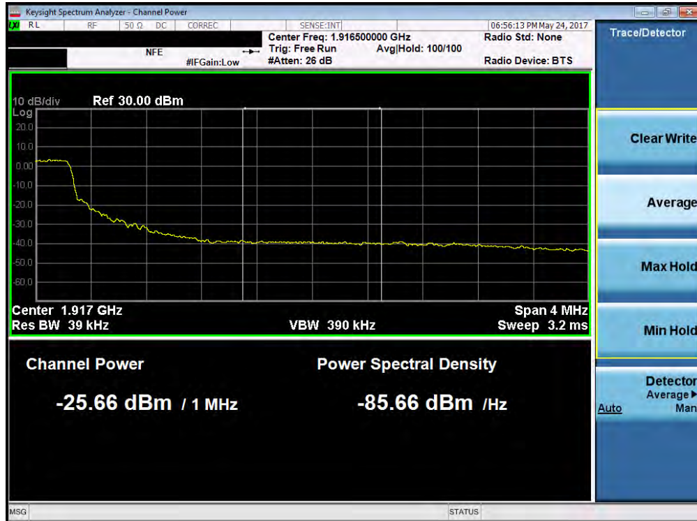
Plot 7-172. Upper Extended Band Edge Plot (Band 25 – 5.0MHz QPSK – RB Size 25)
