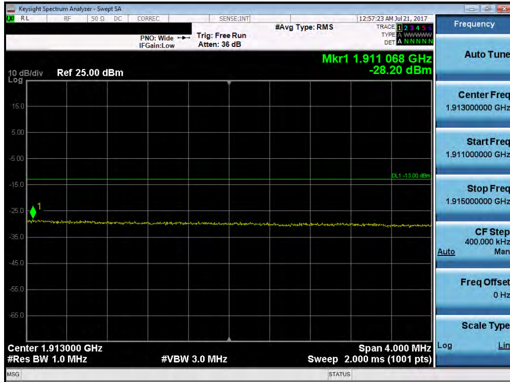
Plot 7-188. Upper Extended Band Edge Plot (Band 2 – 20.0MHz QPSK – RB Size 100)
