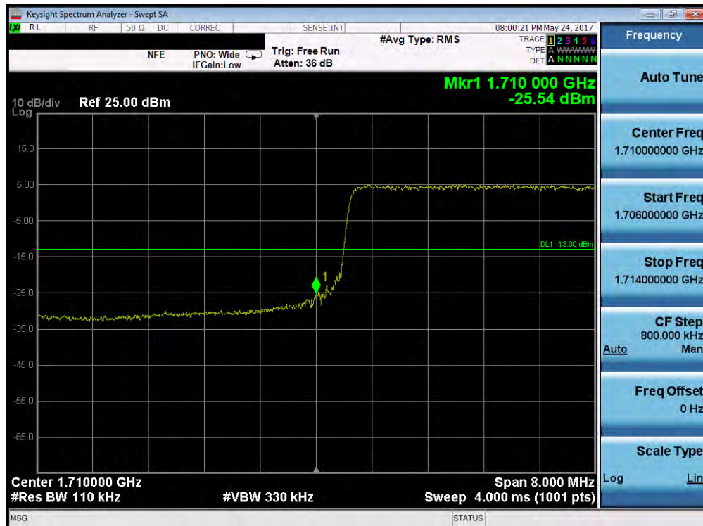
Plot 7-143. Lower Band Edge Plot (Band 4 – 10.0MHz QPSK – RB Size 50)
