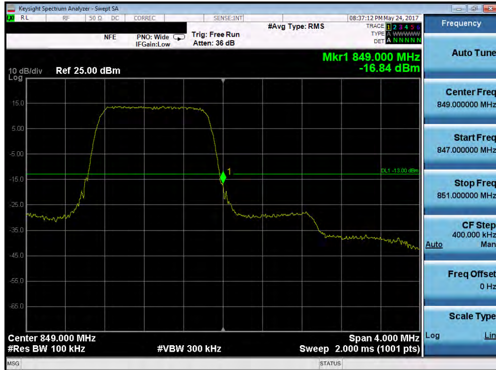
Plot 7-122. Upper Band Edge Plot (Band 5/26 – 1.4MHz QPSK – RB Size 6)
