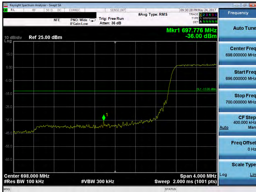
Plot 7-105. Lower Band Edge Plot (Band 12 - 3.0MHz QPSK - RB Size 15)
