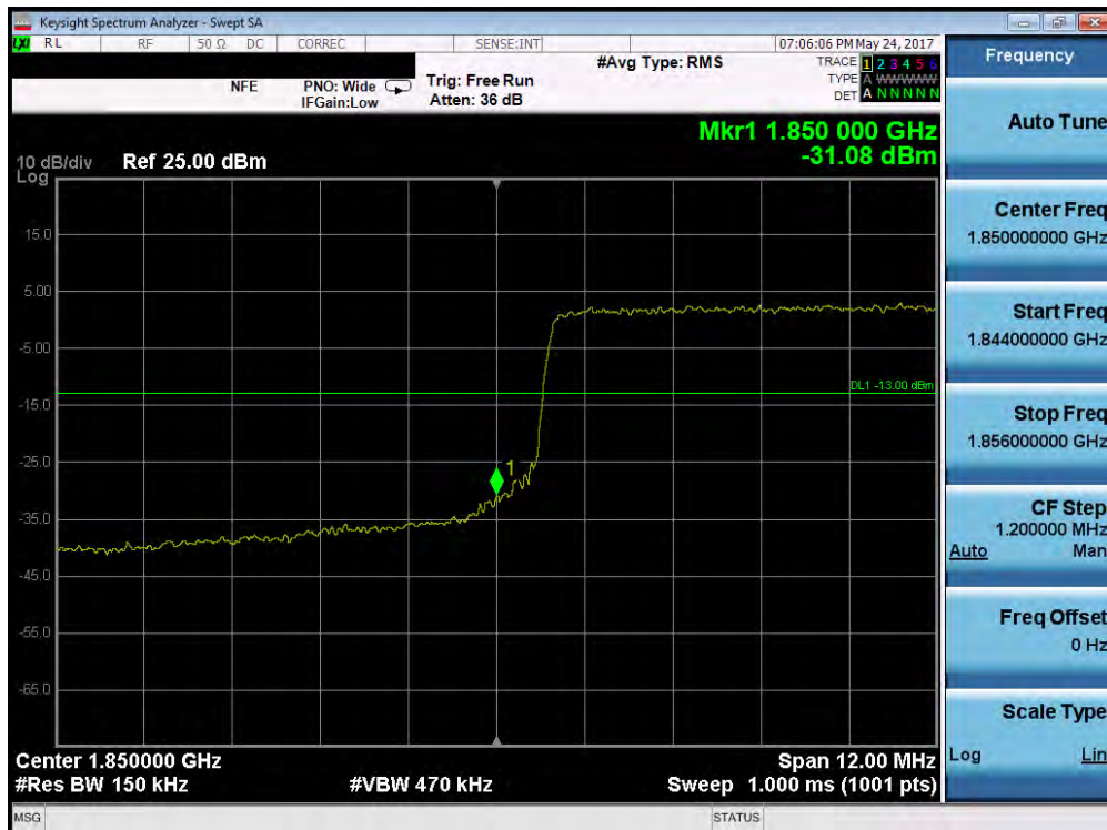
Plot 7-179. Lower Band Edge Plot (Band 2/25 – 15.0MHz QPSK – RB Size 75)
