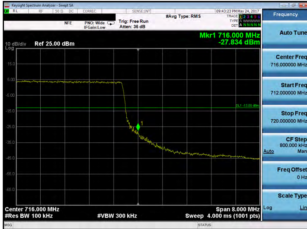
Plot 7-112. Upper Band Edge Plot (Band 12/17 - 10.0MHz QPSK - RB Size 50)
