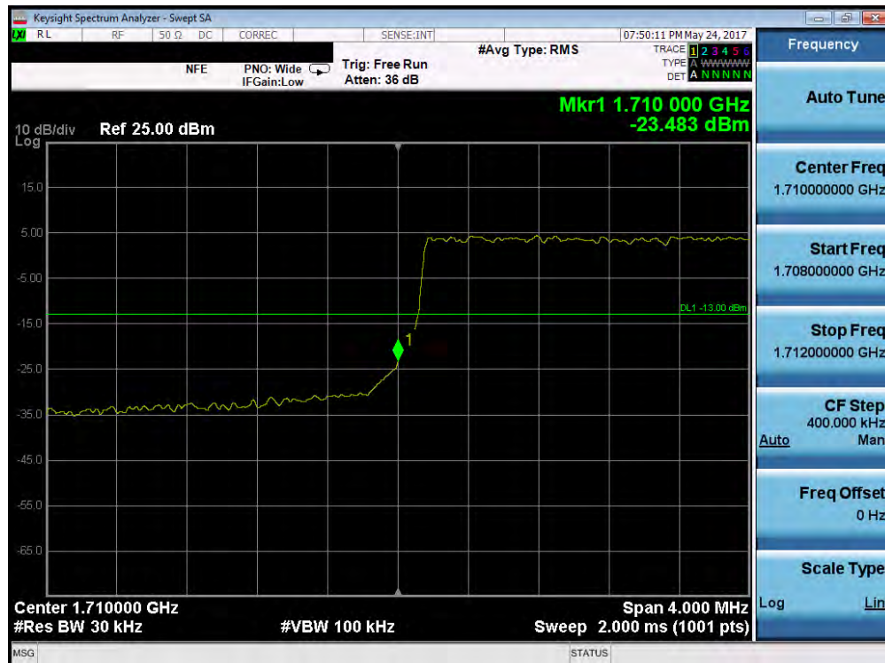
Plot 7-135. Lower Band Edge Plot (Band 4 – 3.0MHz QPSK – RB Size 15)
