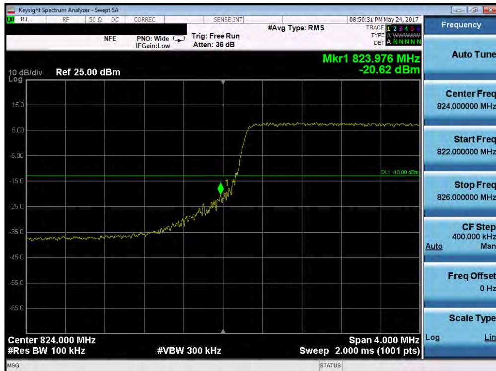
Plot 7-125. Lower Band Edge Plot (Band 5/26 – 5.0MHz QPSK – RB Size 25)
