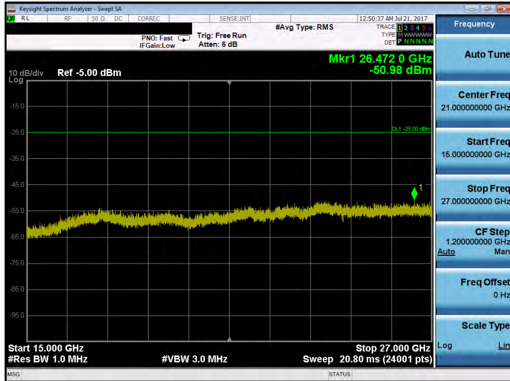
Plot 7-99. Conducted Spurious Plot (Band 41 – 5.0MHz QPSK – RB Size 1, RB Offset 0 – Mid Channel)
