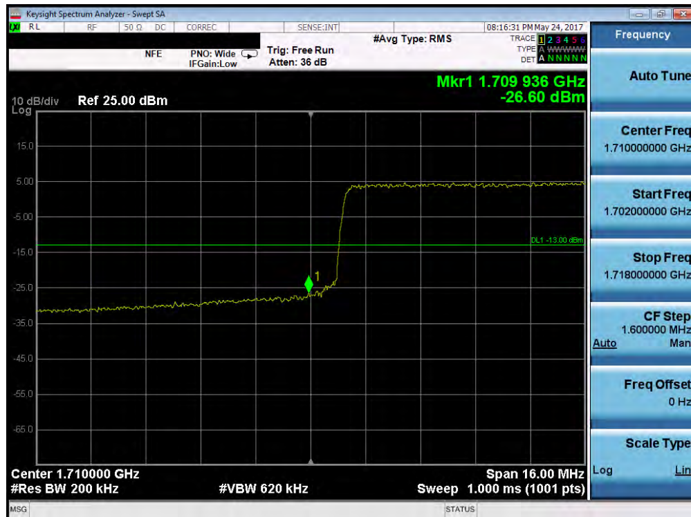
Plot 7-151. Lower Band Edge Plot (Band 4 – 20.0MHz QPSK – RB Size 100)
