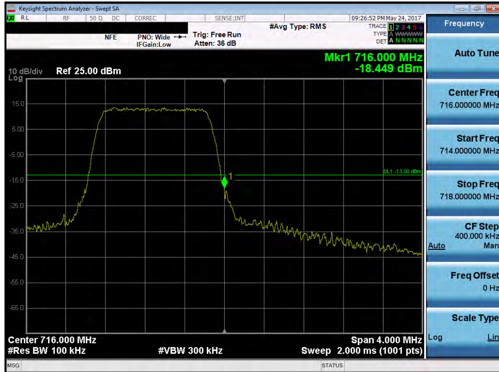
Plot 7-104. Upper Band Edge Plot (Band 12 - 1.4MHz QPSK - RB Size 6)
