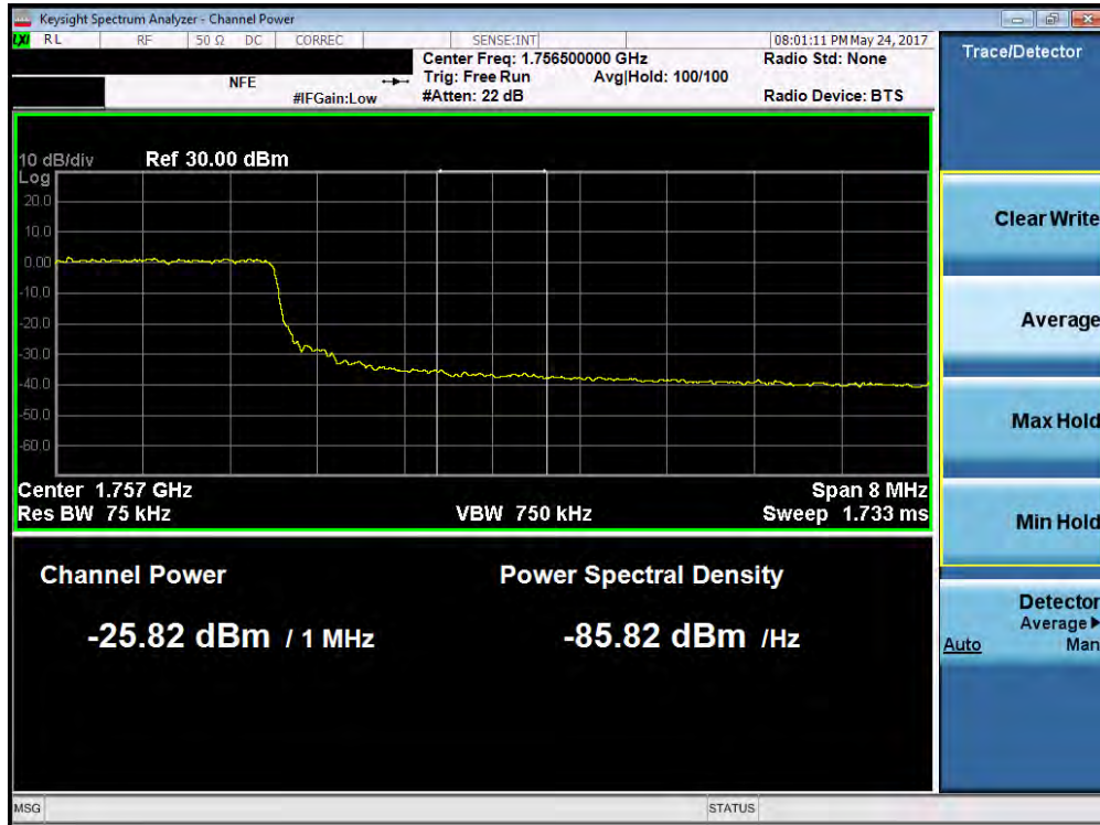
Plot 7-146. Upper Extended Band Edge Plot (Band 4 – 10.0MHz QPSK – RB Size 50)
