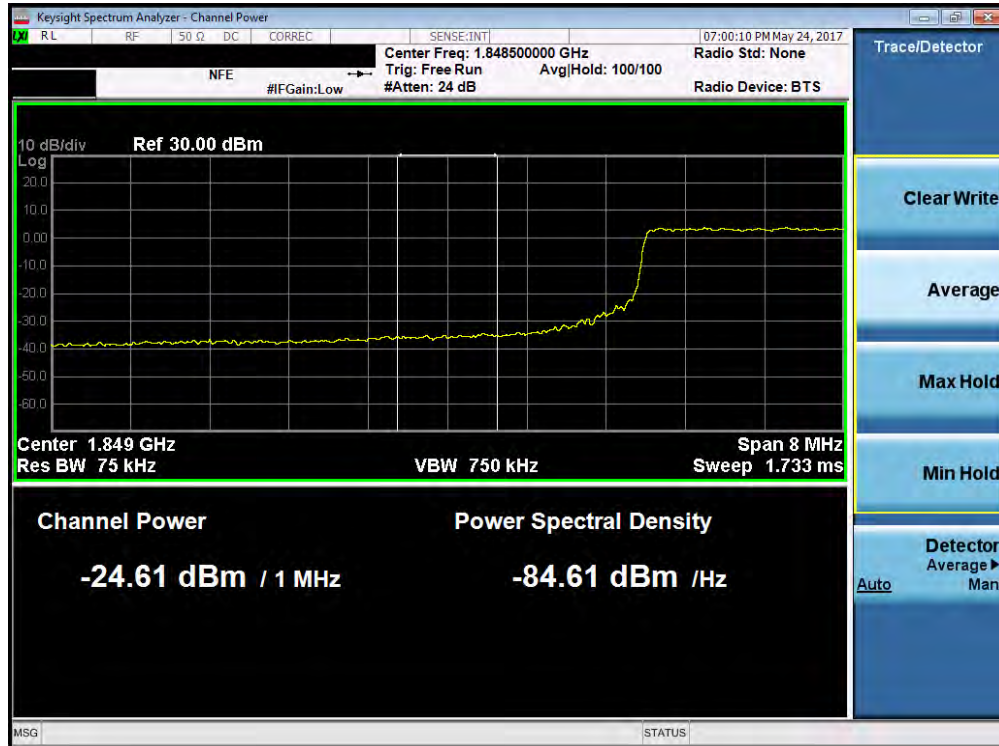
Plot 7-174. Lower Extended Band Edge Plot (Band 2/25 – 10.0MHz QPSK – RB Size 50)
