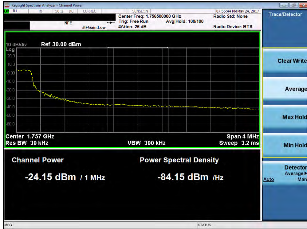
Plot 7-142. Upper Extended Band Edge Plot (Band 4 – 5.0MHz QPSK – RB Size 25)
