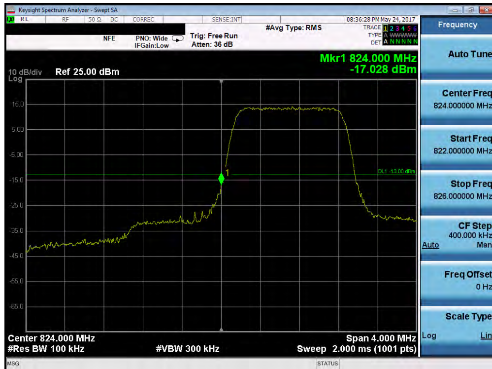
Plot 7-121. Lower Band Edge Plot (Band 5/26 – 1.4MHz QPSK – RB Size 6)
