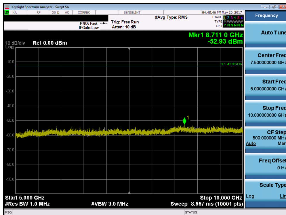
Plot 7-14. Conducted Spurious Plot (1.4 MHz QPSK – RB Size 1, RB Offset 0 – High Channel)
