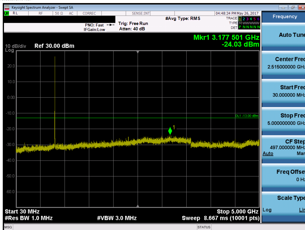
Plot 7-13. Conducted Spurious Plot (1.4 MHz QPSK – RB Size 1, RB Offset 0 – High Channel)
