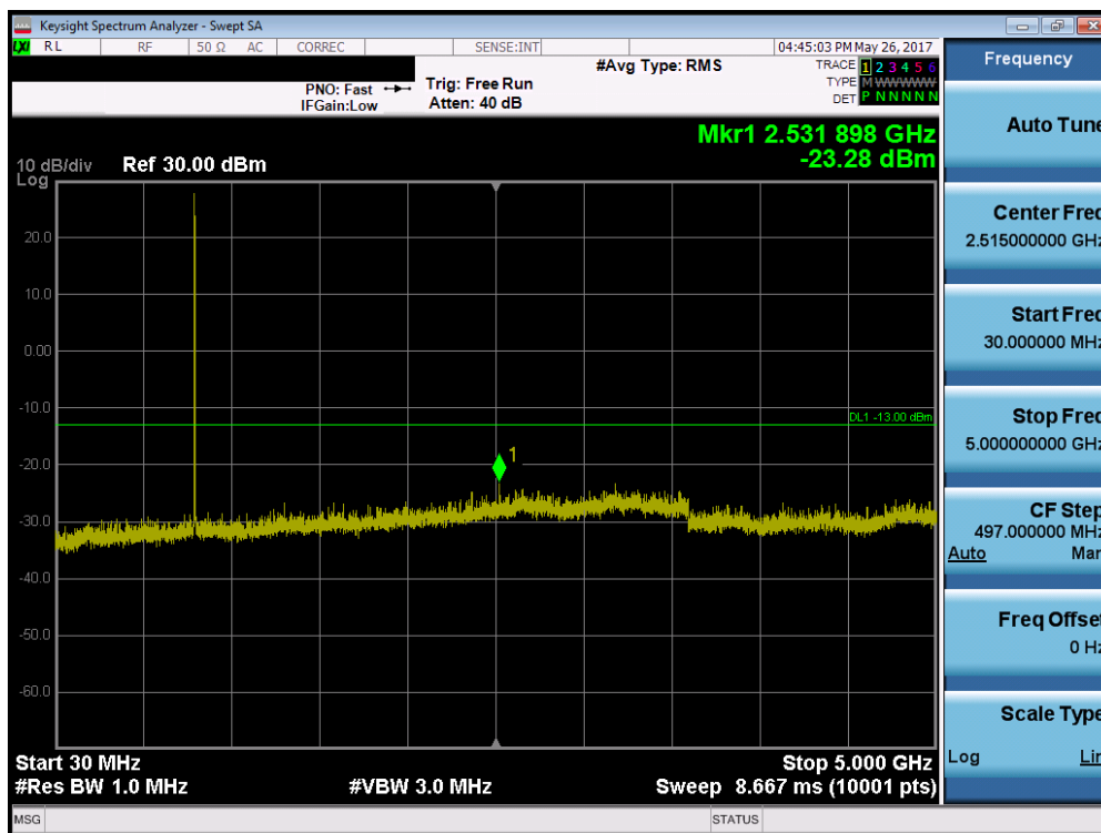
Plot 7-11. Conducted Spurious Plot (1.4 MHz QPSK – RB Size 1, RB Offset 0 – Low Channel)
