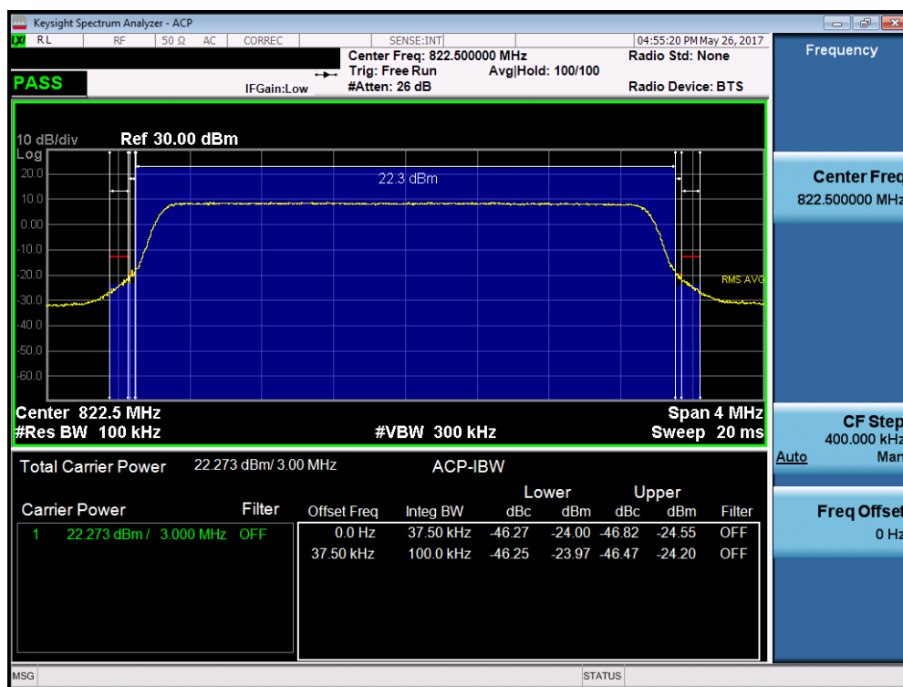
Plot 7-18. Channel Edge Plot (3MHz QPSK – RB Size 15 – High Channel)
