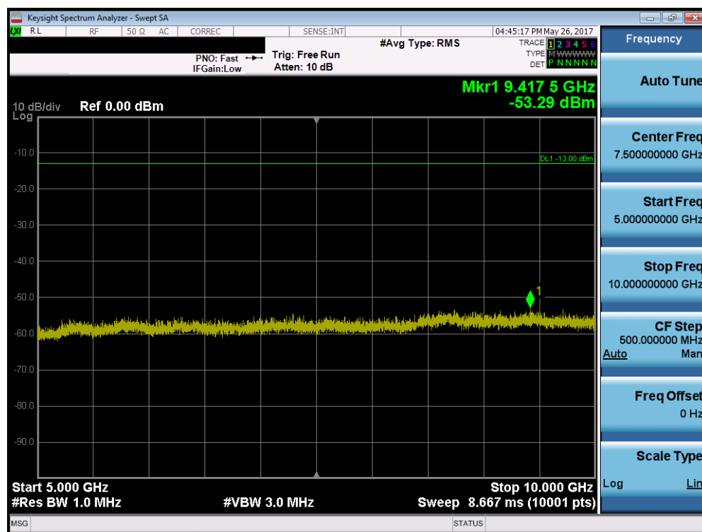
Plot 7-12. Conducted Spurious Plot (1.4 MHz QPSK – RB Size 1, RB Offset 0 – Low Channel)
