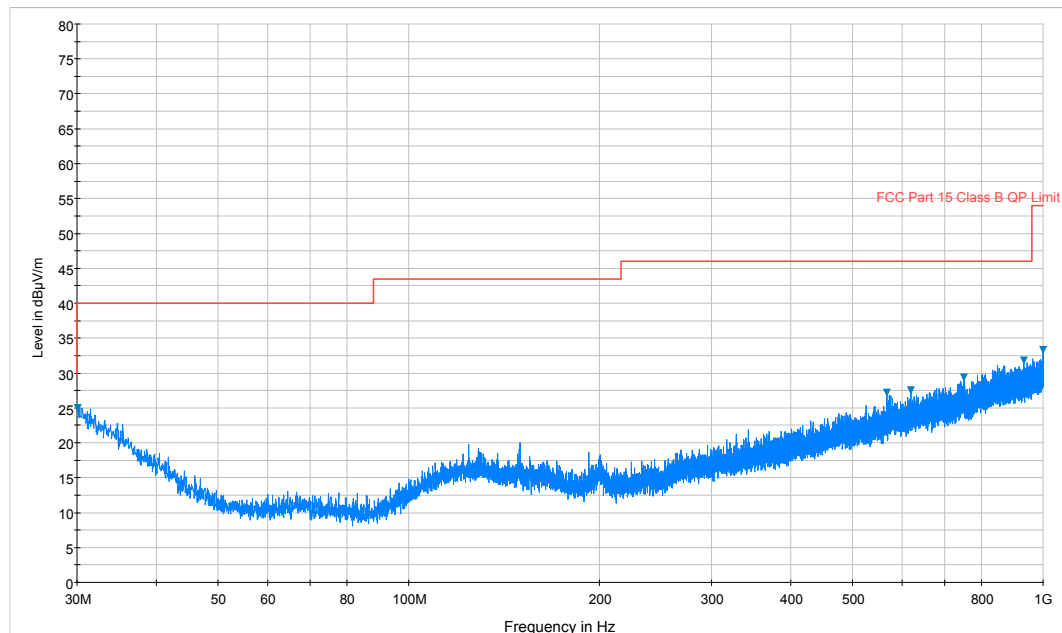
Plot 7-255. Radiated Spurious Plot below 1GHz (802.11a – U3 Ch. 157, Ant. Pol. H)
