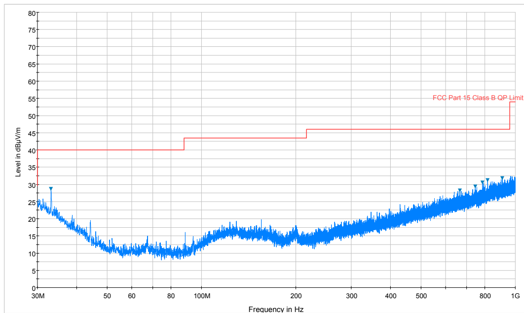
Plot 7-256. Radiated Spurious Plot below 1GHz (802.11a – U3 Ch. 157, Ant. Pol. V)
