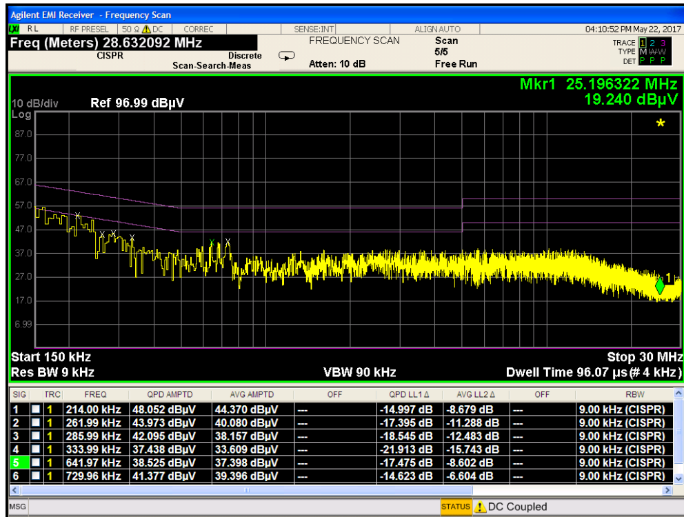
Plot 7-96. Line Conducted Plot with 802.11b (L1)
