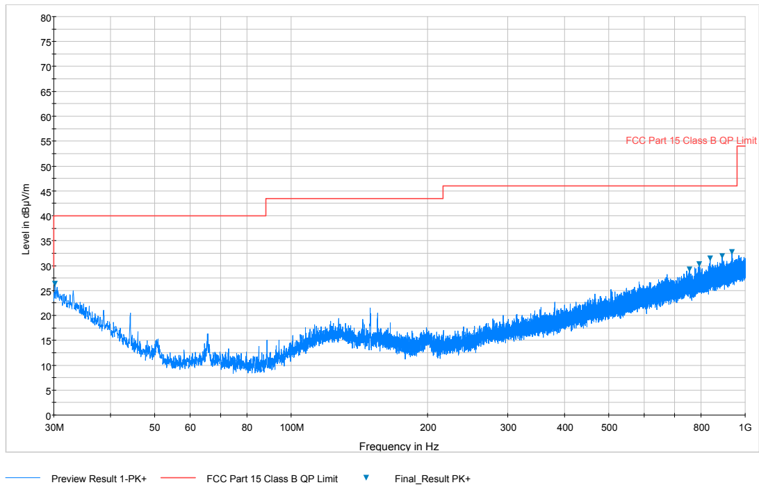
Plot 7-95. Radiated Spurious Plot below 1GHz (Pol. V)
