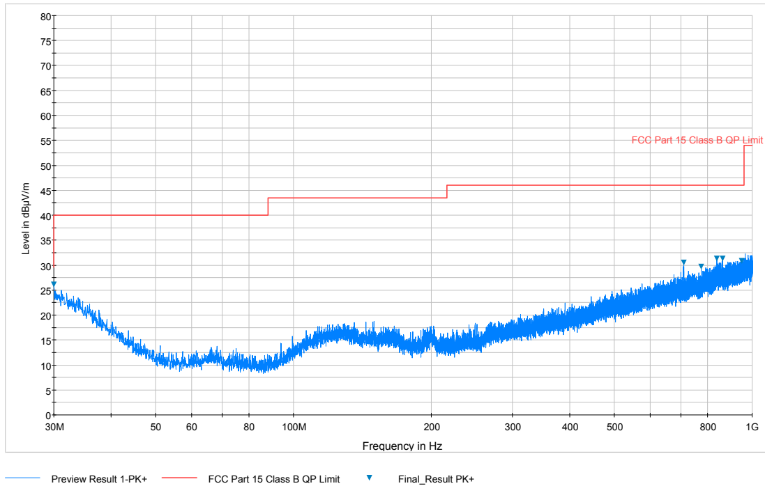
Plot 7-94. Radiated Spurious Plot below 1GHz (Pol. H)
