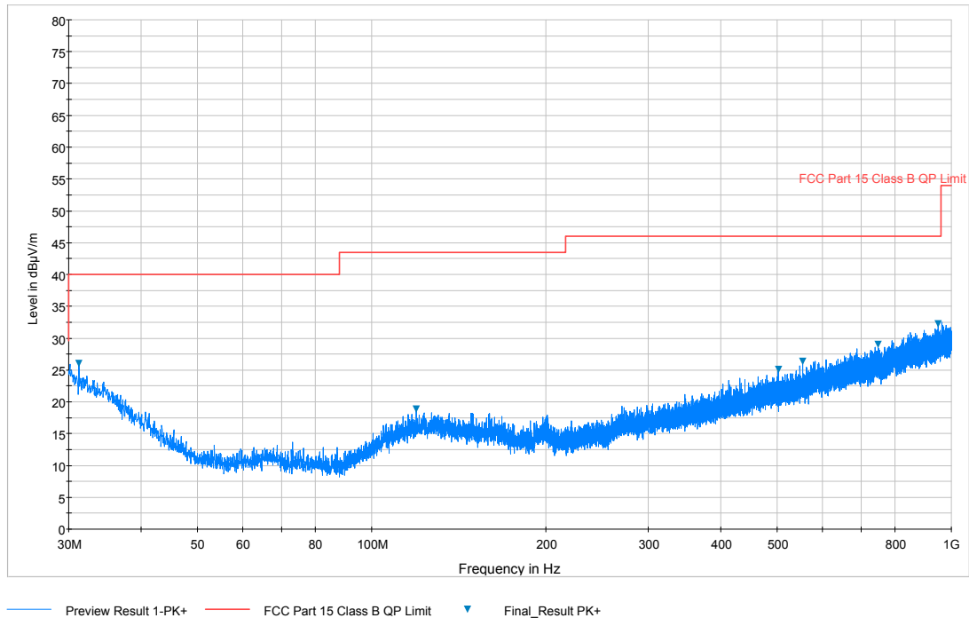
Plot 7-92. Radiated Spurious Plot below 1GHz (Pol. H)
