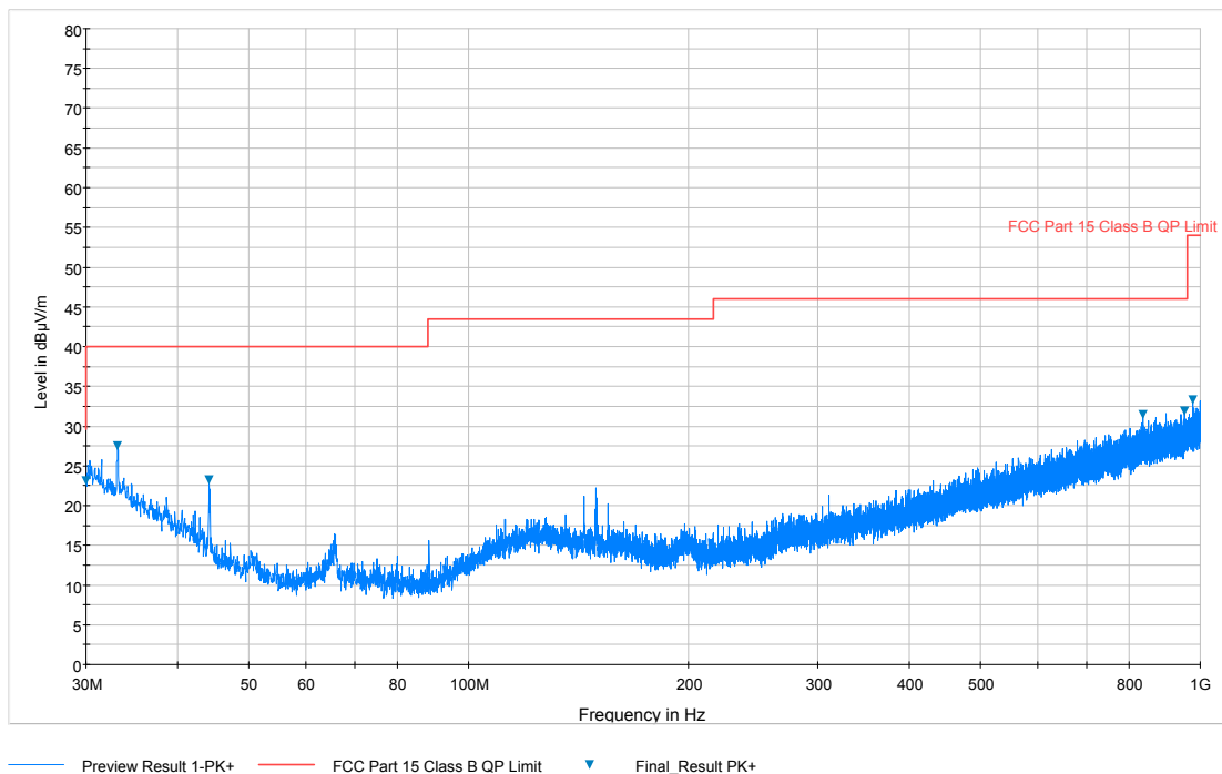
Plot 7-93. Radiated Spurious Plot below 1GHz (Pol. V)
