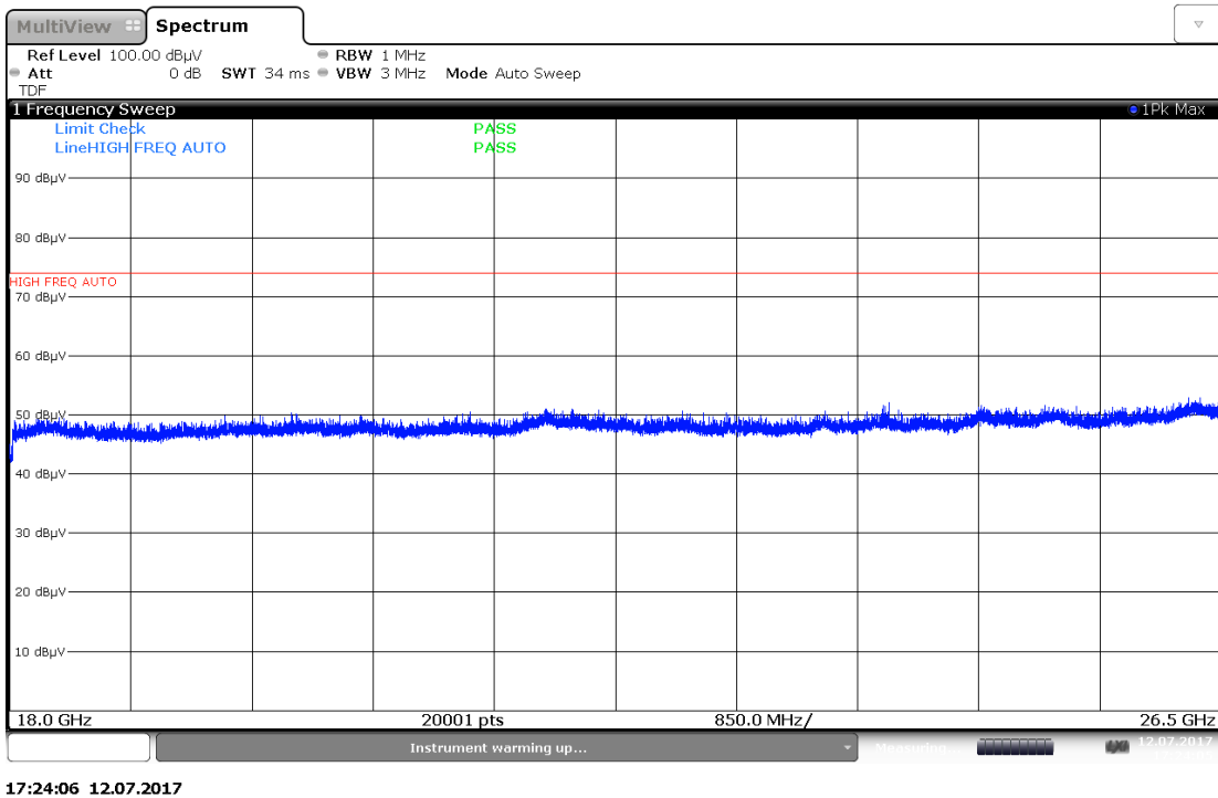
Plot 7-68. Radiated Spurious Plot above 18GHz (Pol. V)
