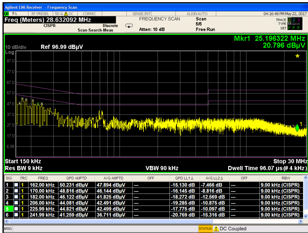
Plot 7-97. Line Conducted Plot with 802.11b (N)
