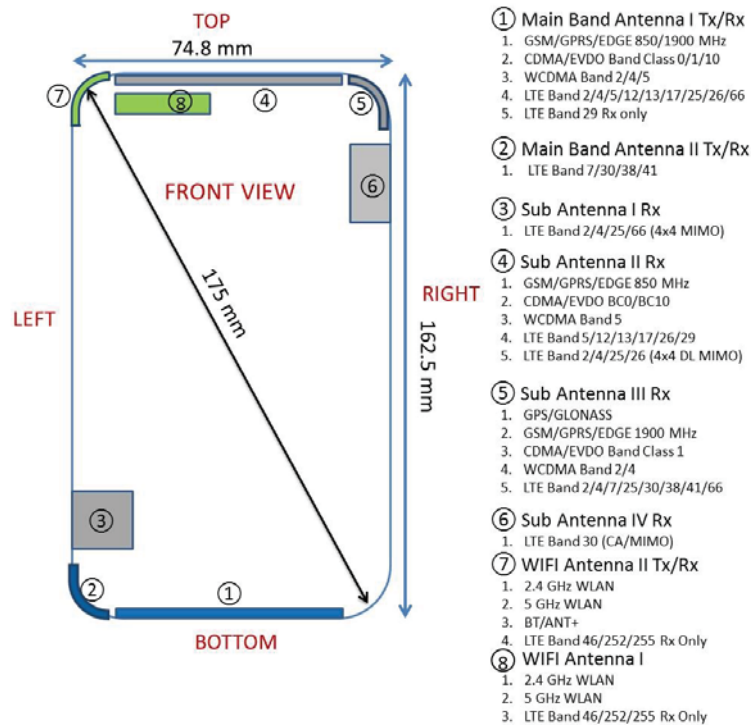
Figure F-1 DUT Antenna Locations
