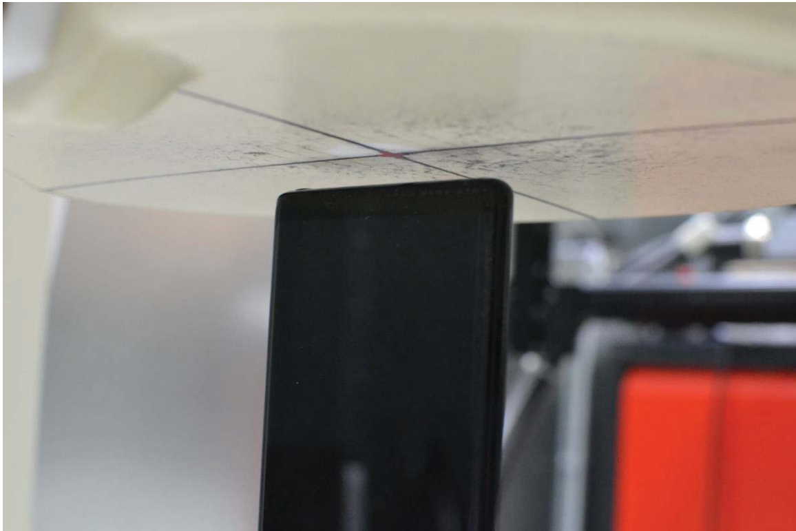
SAR Test Setup Photo 15 – Bottom Edge at 8 mm
