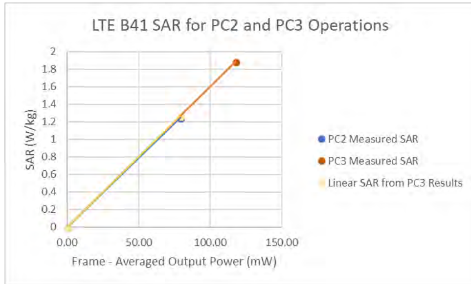
Figure 14-4 LTE Band 41 Phablet Linearity
