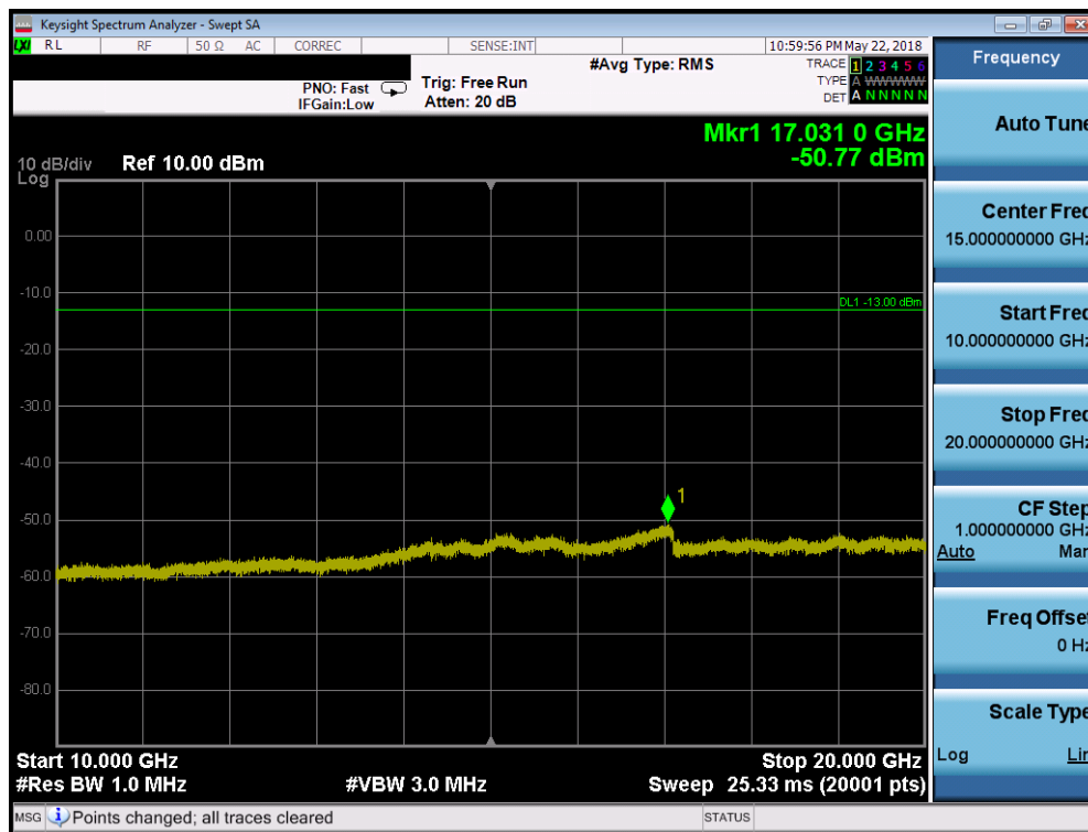
Plot 7-62. Conducted Spurious Plot (PCS WCDMA Mode - High Channel)
