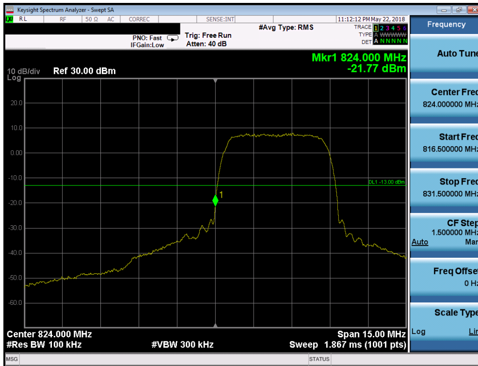
Plot 7-73. Band Edge Plot (Cellular WCDMA Mode - Low Channel)
