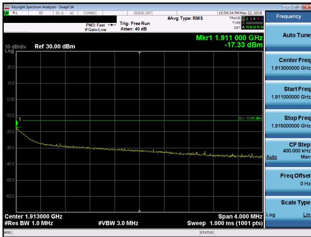
Plot 7-82. 4MHz Span Plot (PCS WCDMA Mode - High Channel)
