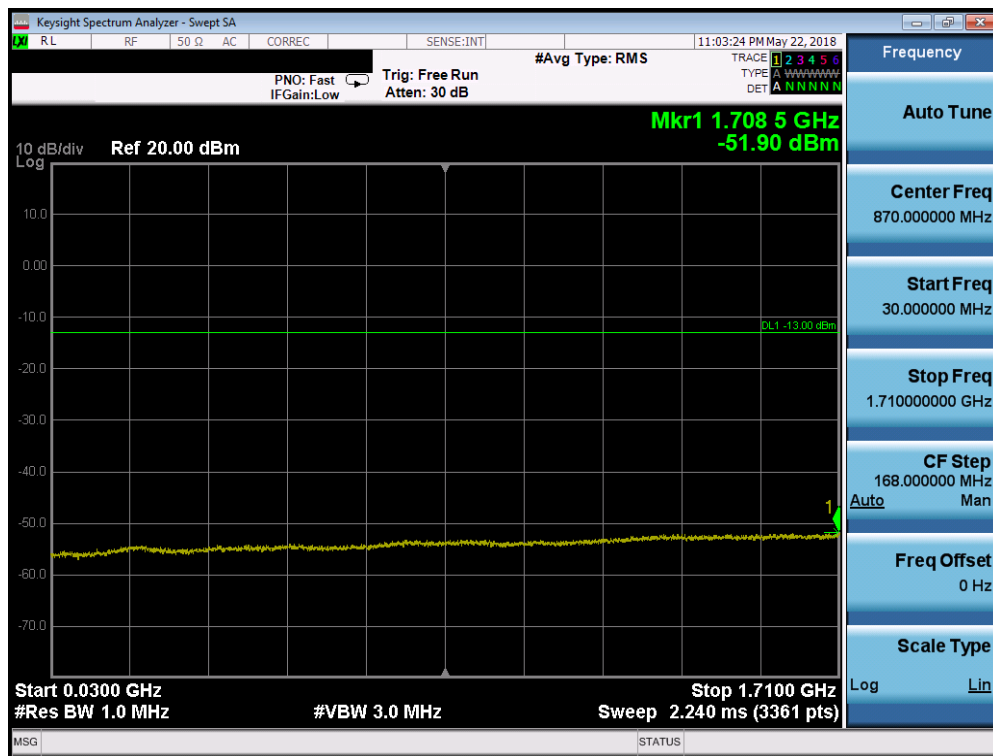
Plot 7-48. Conducted Spurious Plot (AWS WCDMA Mode - Mid Channel)
