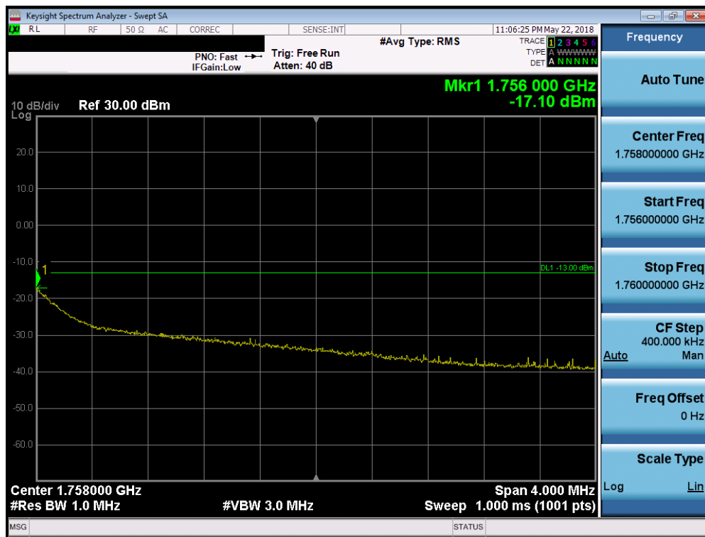
Plot 7-78. 4MHz Span Plot (AWS WCDMA Mode - High Channel)
