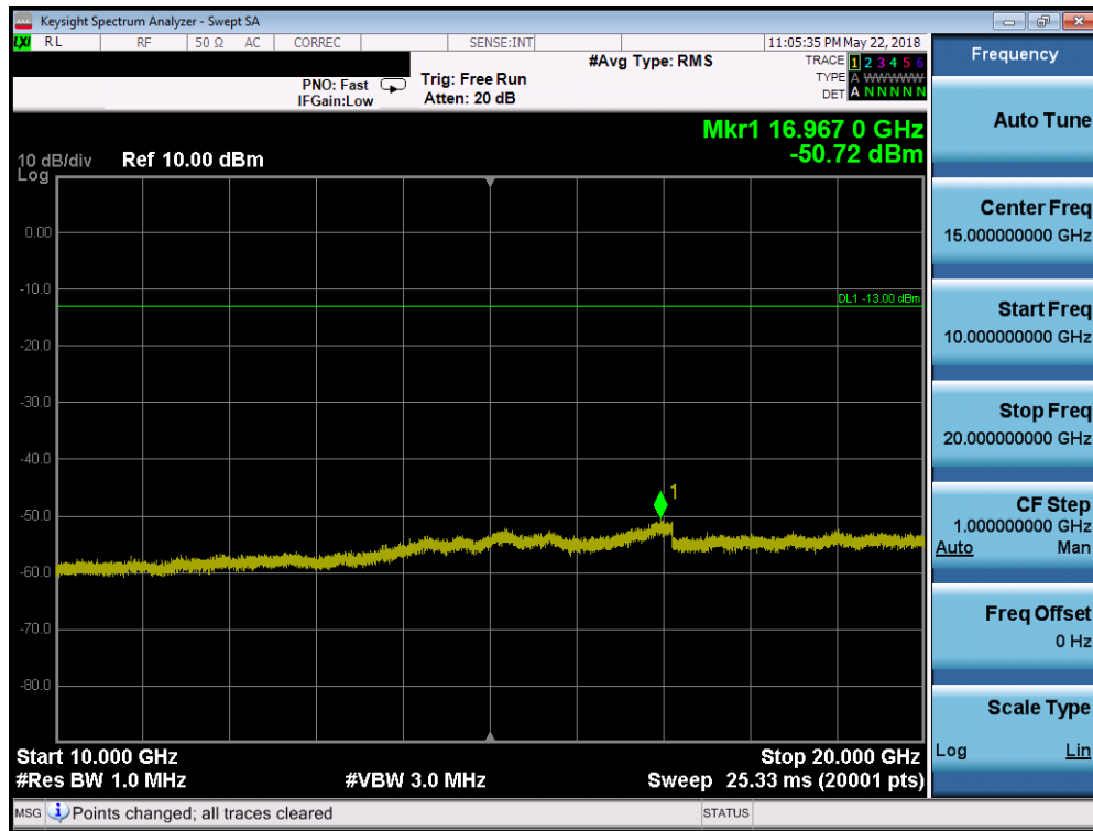
Plot 7-47. Conducted Spurious Plot (AWS WCDMA Mode - Low Channel)
