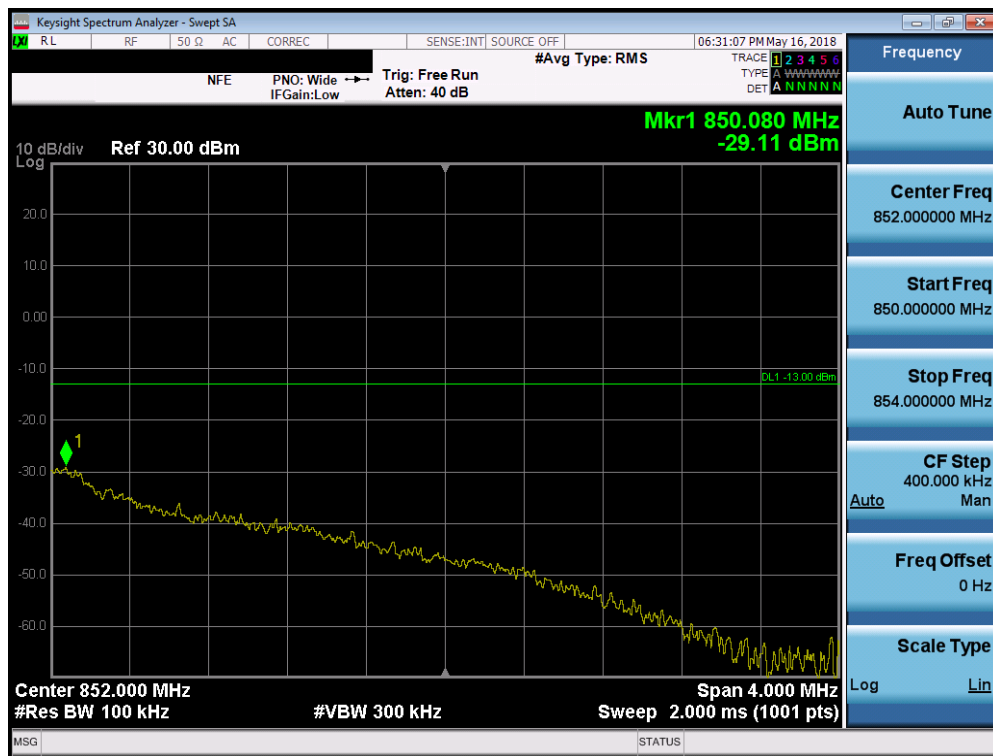
Plot 7-72. 4MHz Span Plot (Cellular CDMA Mode - High Channel)
