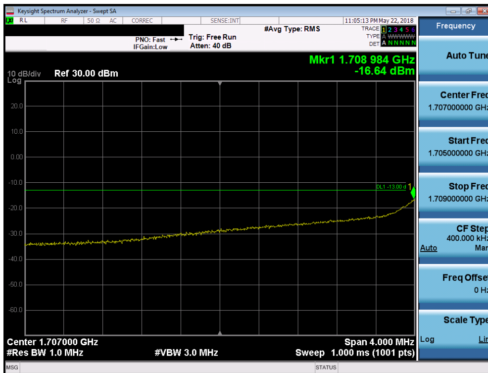
Plot 7-76. 4MHz Span Plot (AWS WCDMA Mode - Low Channel)
