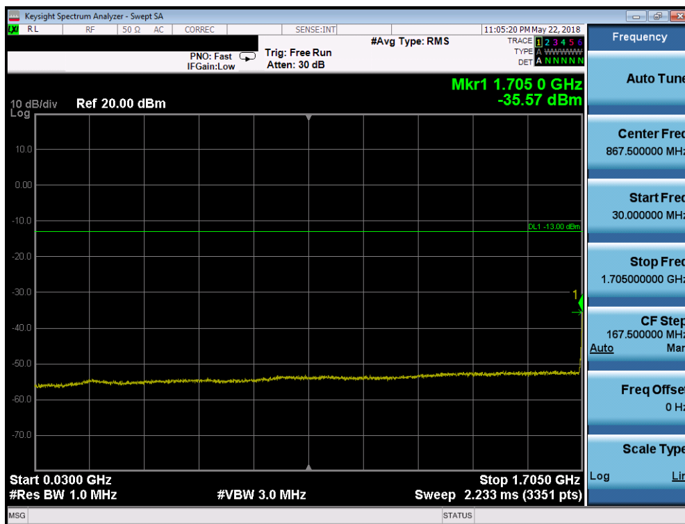
Plot 7-45. Conducted Spurious Plot (AWS WCDMA Mode - Low Channel)
