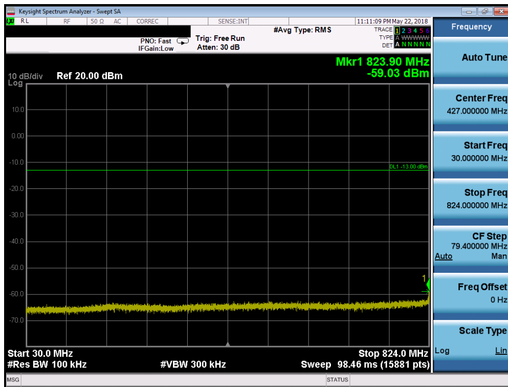
Plot 7-39. Conducted Spurious Plot (Cellular WCDMA Mode - Mid Channel)
