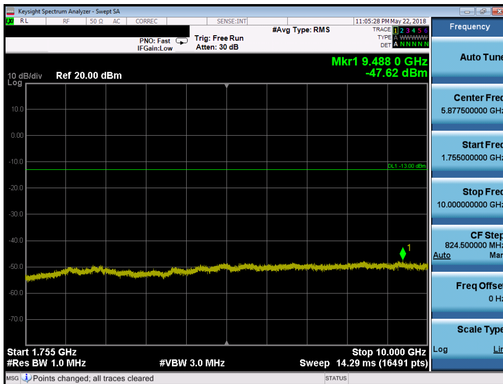
Plot 7-46. Conducted Spurious Plot (AWS WCDMA Mode - Low Channel)
