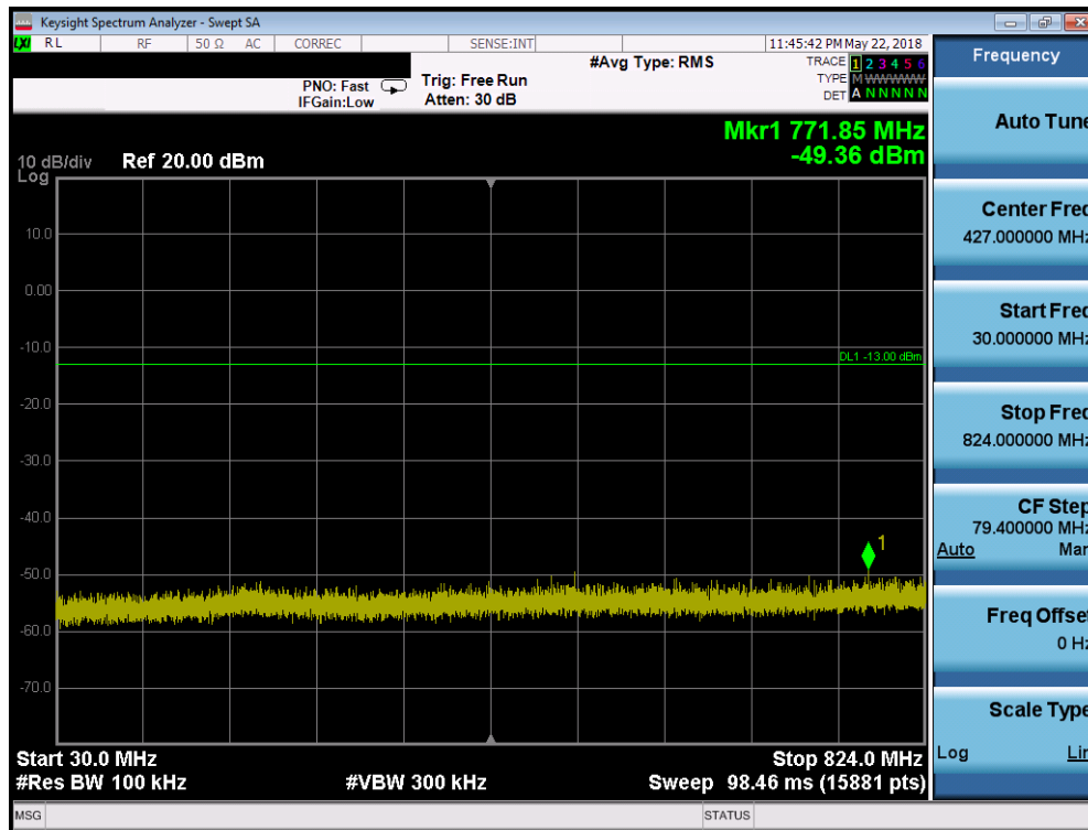
Plot 7-15. Conducted Spurious Plot (Cellular GPRS Mode - High Channel)
