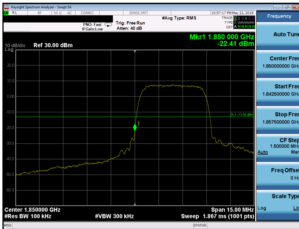
Plot 7-79. Band Edge Plot (PCS WCDMA Mode - Low Channel)
