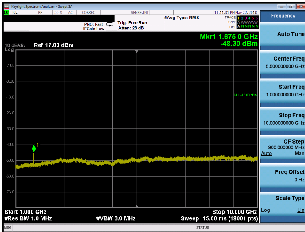
Plot 7-41. Conducted Spurious Plot (Cellular WCDMA Mode - Mid Channel)
