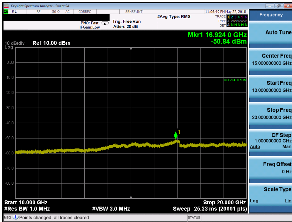
Plot 7-53. Conducted Spurious Plot (AWS WCDMA Mode - High Channel)
