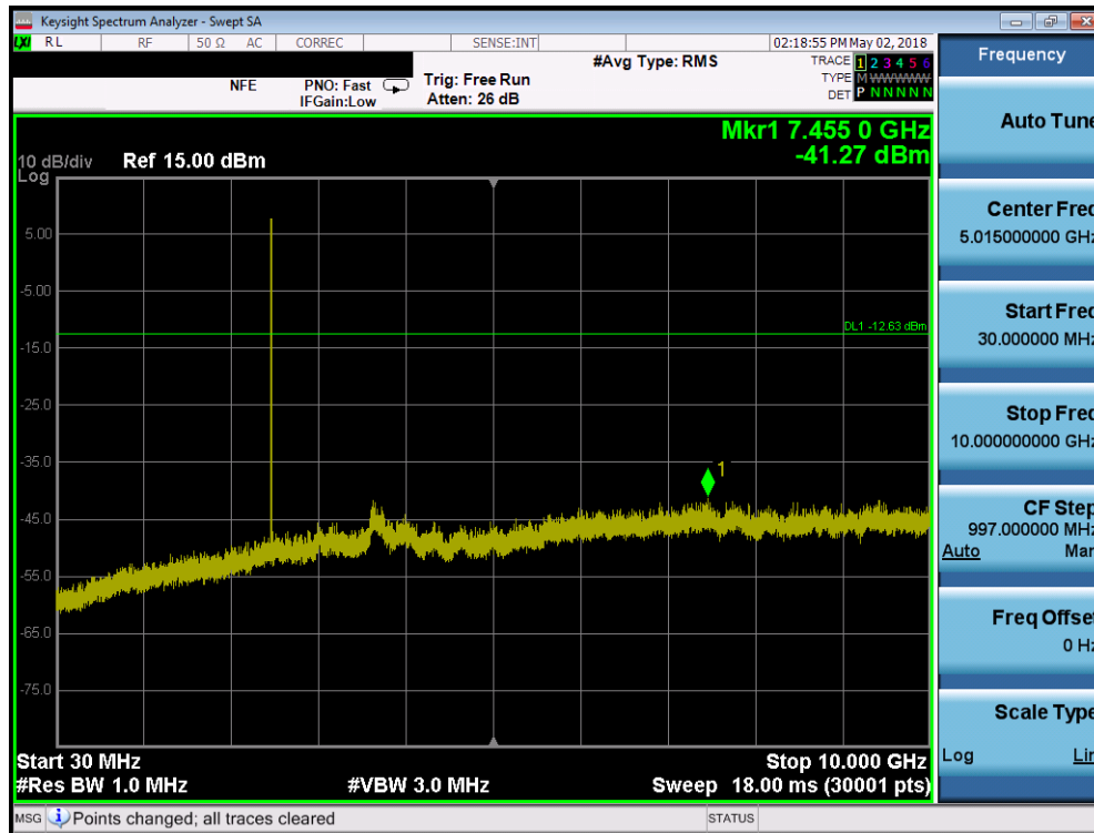
Plot 7-33. Conducted Spurious Plot (Bluetooth (LE), 2Mbps – Ch. 39)
