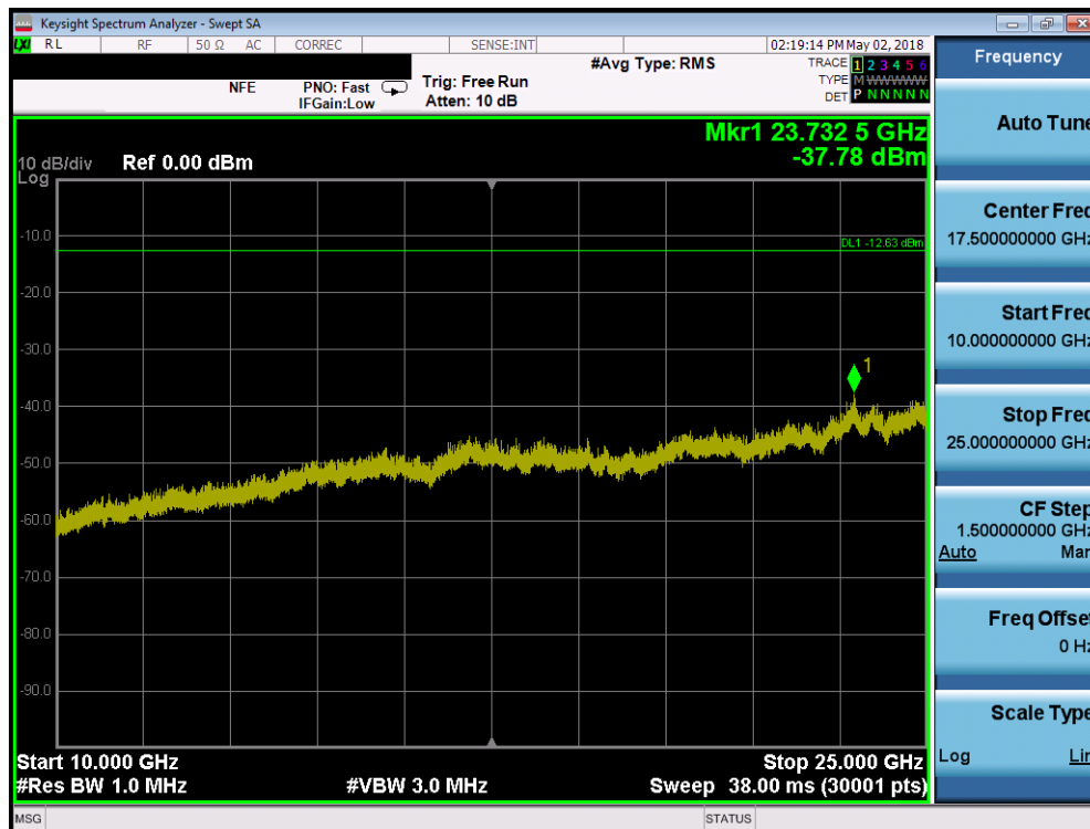
Plot 7-34. Conducted Spurious Plot (Bluetooth (LE), 2Mbps – Ch. 39)
