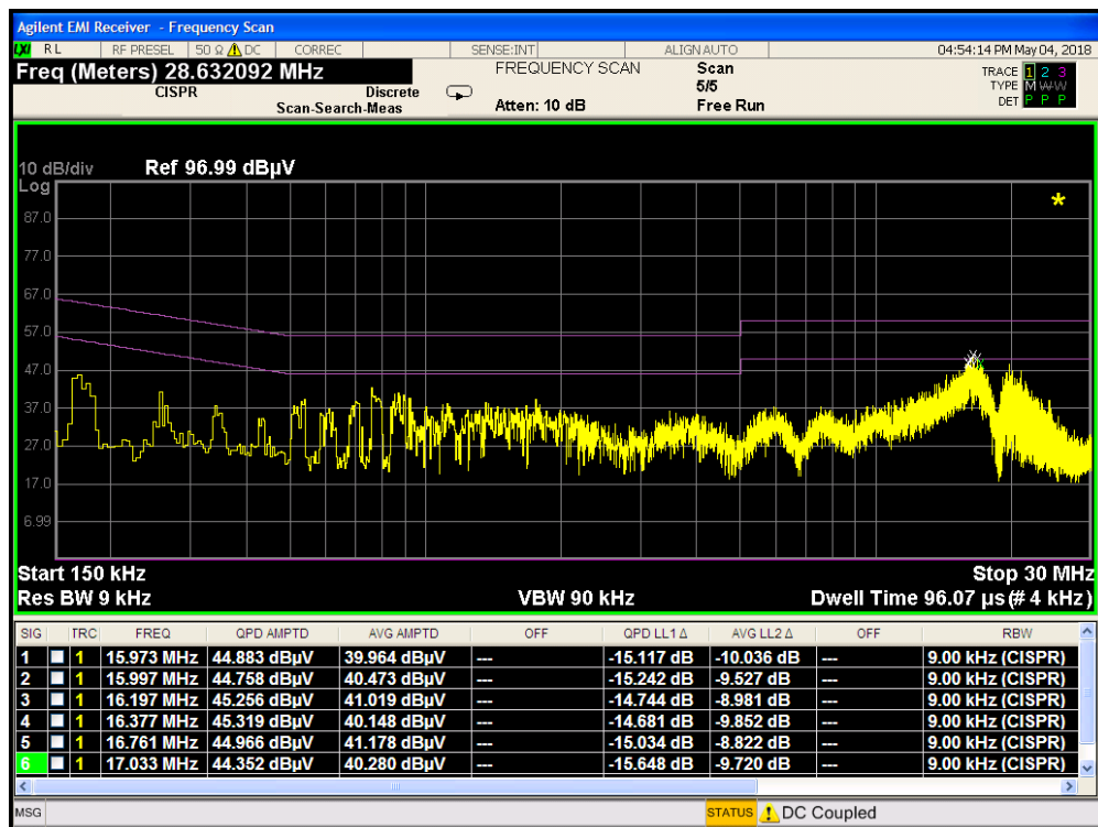
Plot 7-52. Line-Conducted Test Plot (N) with Travel Adapter
