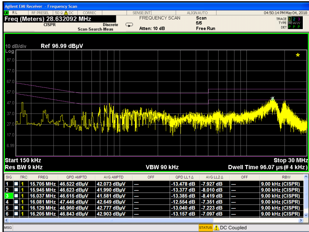
Plot 7-51. Line-Conducted Test Plot (L1) with Travel Adapter
