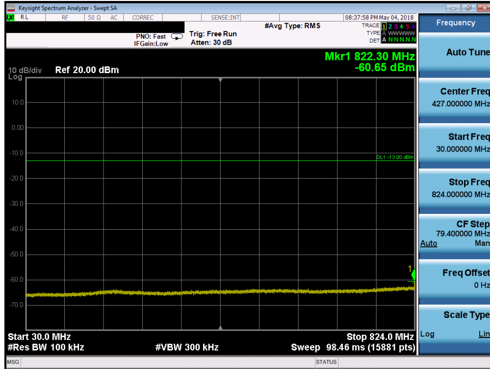
Plot 7-118. Conducted Spurious Plot (Band 26/5 - 5.0MHz QPSK - RB Size 1, RB Offset 0 - High Channel)
