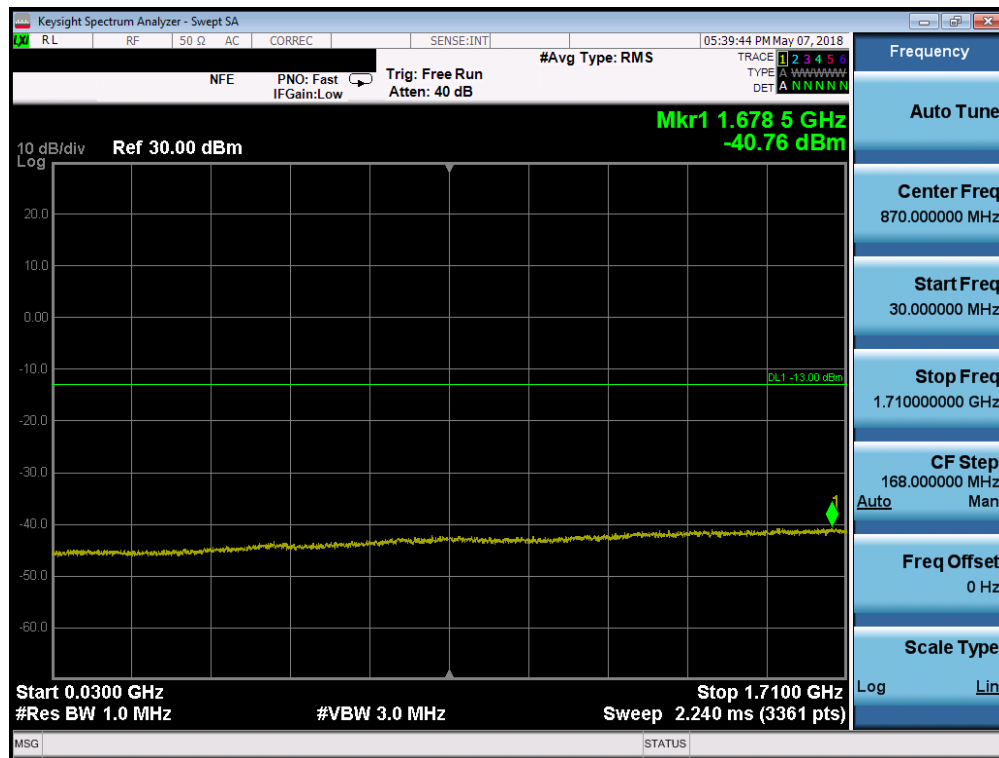
Plot 7-124. Conducted Spurious Plot (Band 66/4 - 5.0MHz QPSK - RB Size 1, RB Offset 0 - Mid Channel)
