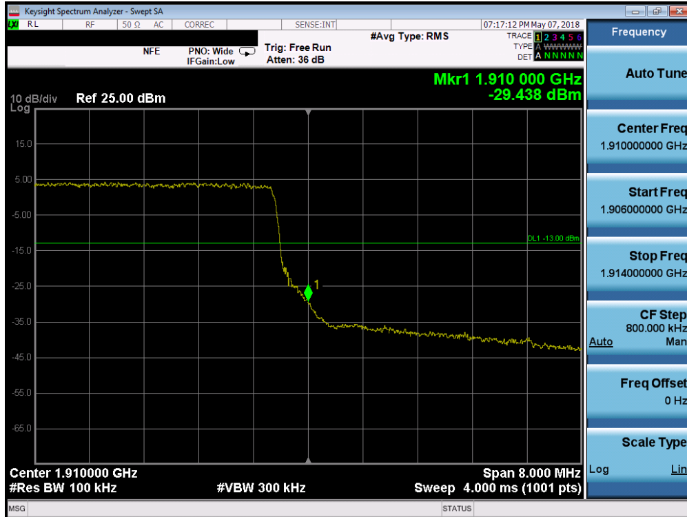
Plot 7-232. Upper Band Edge Plot (Band 2 - 10.0MHz QPSK - Full RB Configuration)
