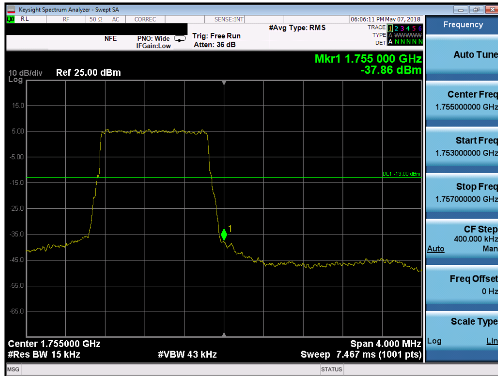
Plot 7-178. Upper Band Edge Plot (Band 4 - 1.4MHz QPSK - Full RB Configuration)
