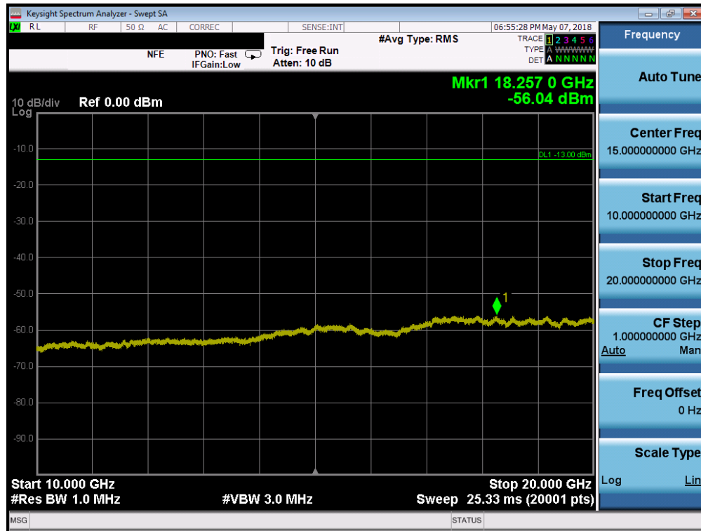
Plot 7-132. Conducted Spurious Plot (Band 25/2 - 5.0MHz QPSK - RB Size 1, RB Offset 0 - Low Channel)
