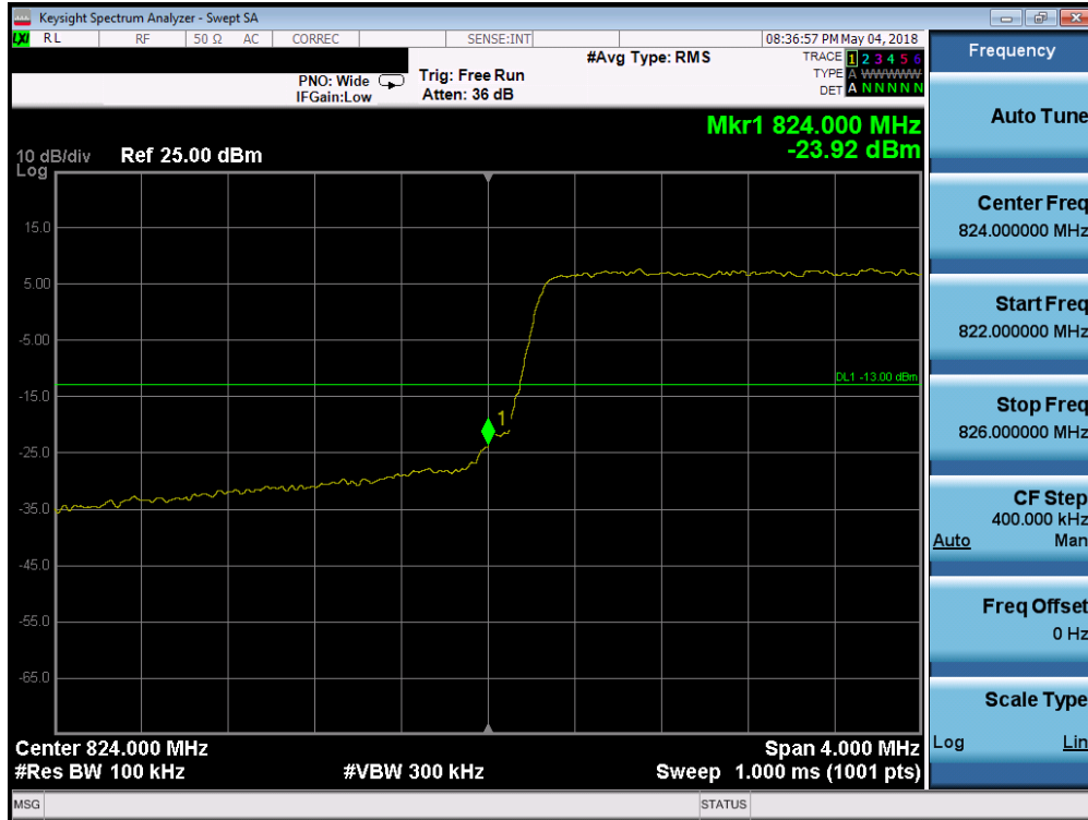
Plot 7-170. Lower Band Edge Plot (Band 26/5 - 5.0MHz QPSK - Full RB Configuration)
