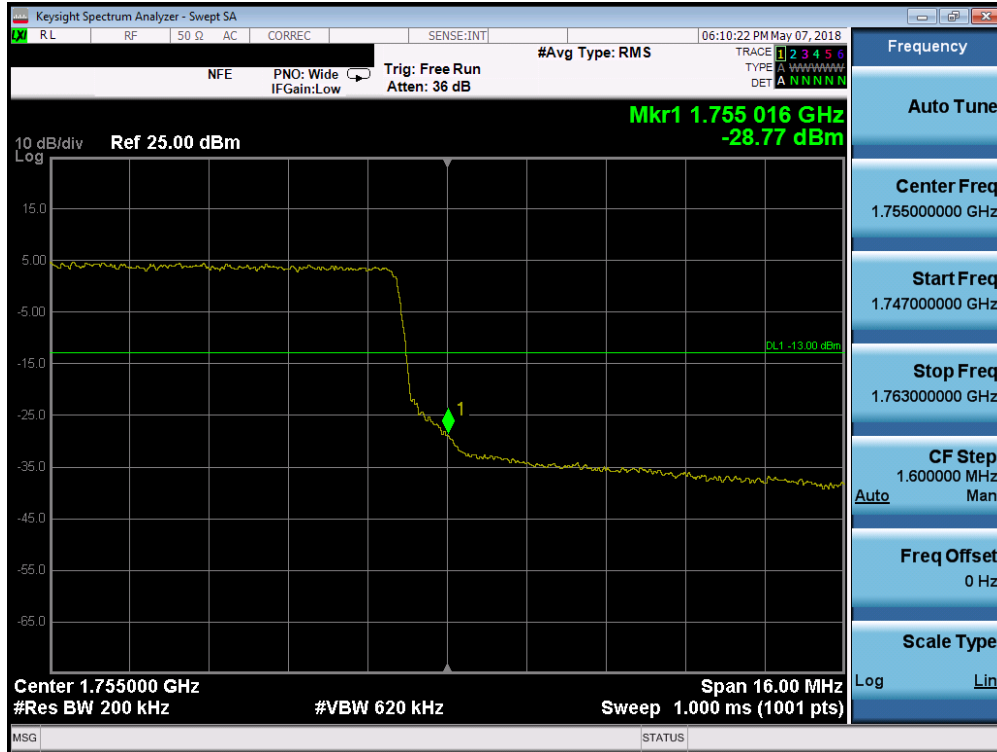
Plot 7-208. Upper Band Edge Plot (Band 4 - 20.0MHz QPSK - Full RB Configuration)
