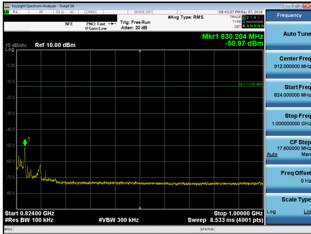
Plot 7-20. Conducted Spurious Plot (LTE B26 – 5.0MHz QPSK – RB Size 1, RB Offset 0 – High Channel)
