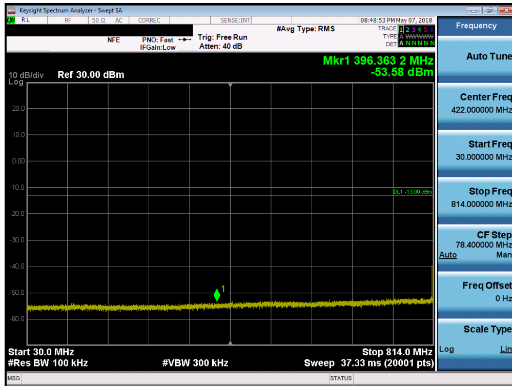
Plot 7-16. Conducted Spurious Plot (LTE B26 – 5.0MHz QPSK – RB Size 1, RB Offset 0 – Low Channel)
