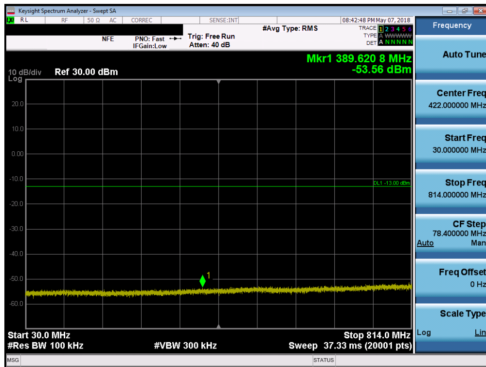
Plot 7-19. Conducted Spurious Plot (LTE B26 – 5.0MHz QPSK – RB Size 1, RB Offset 0 – High Channel)
