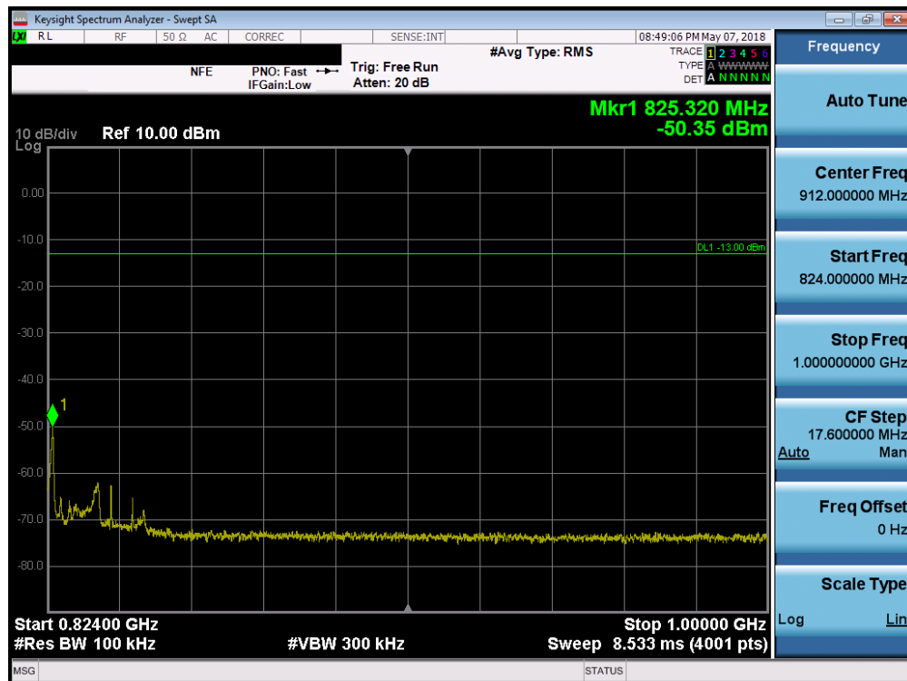
Plot 7-17. Conducted Spurious Plot (LTE B26 – 5.0MHz QPSK – RB Size 1, RB Offset 0 – Low Channel)
