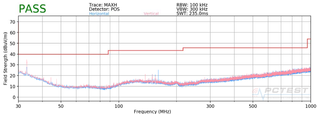
Plot 7-4. Radiated Spurious Plot 30MHz – 1GHz
