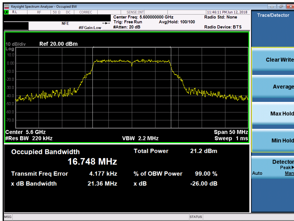
Plot 7-49. 26dB Bandwidth Plot (802.11a (UNII Band 2C) – Ch. 120)
