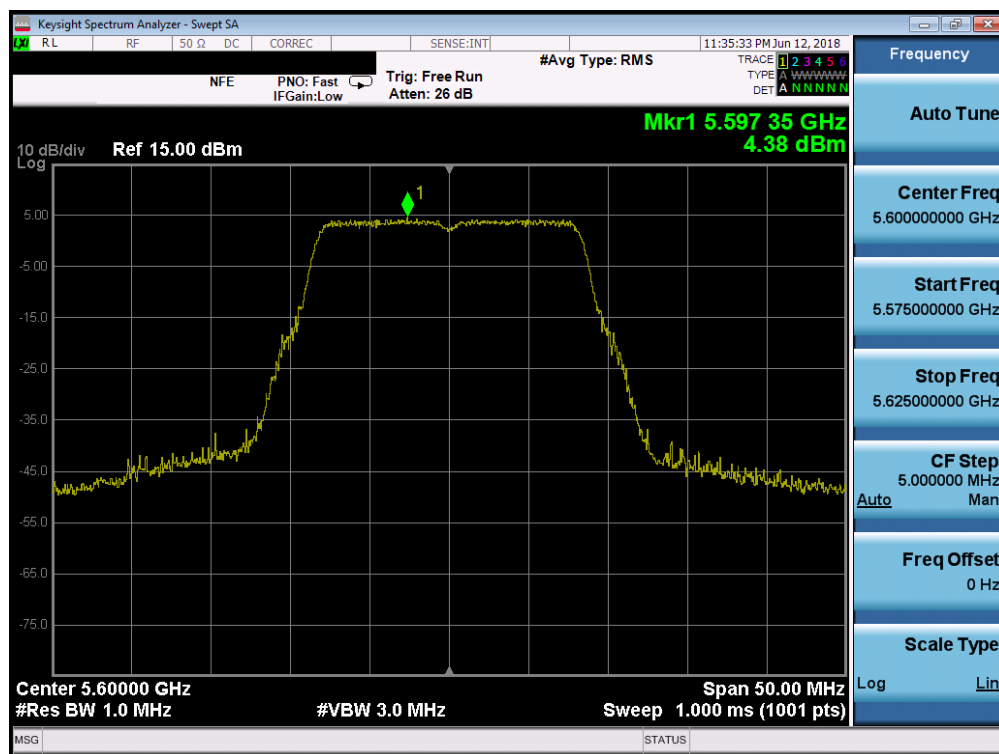
Plot 7-96. Power Spectral Density Plot (802.11a (UNII Band 2C) – Ch. 120)
