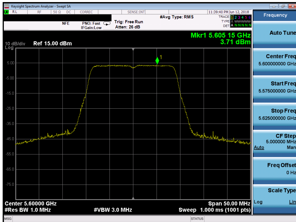
Plot 7-99. Power Spectral Density Plot (20MHz BW 802.11n (UNII Band 2C) – Ch. 120)
