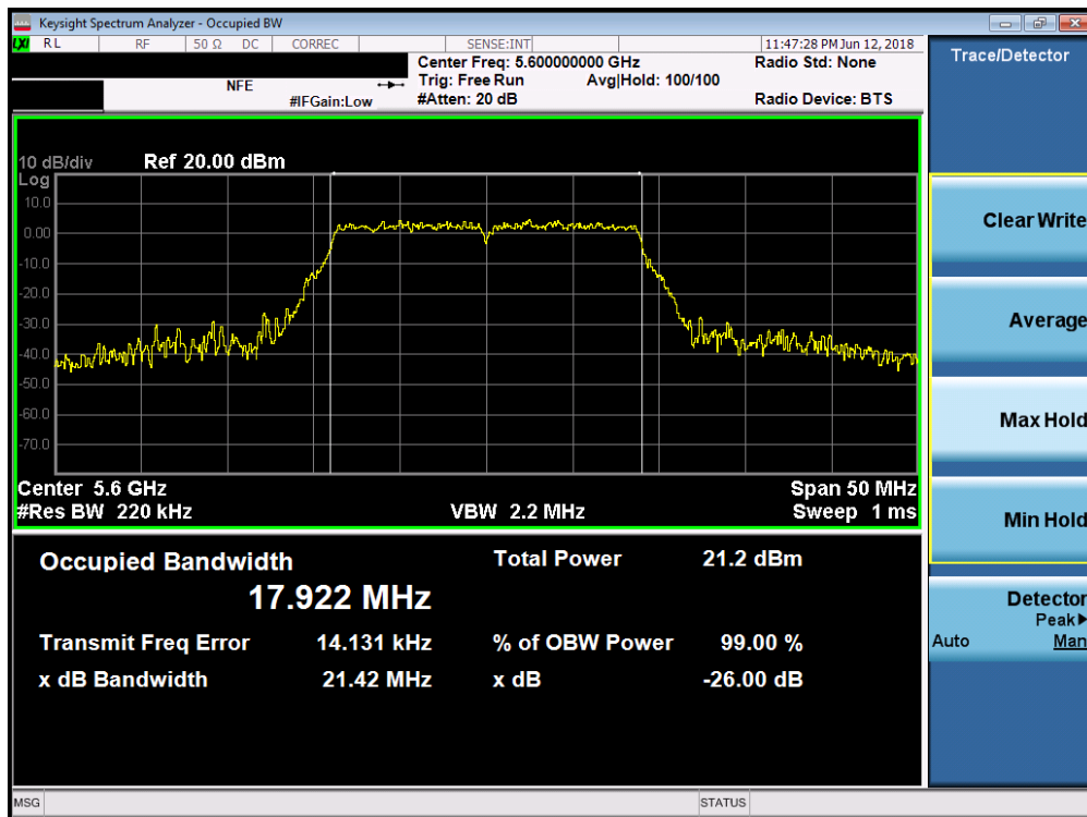
Plot 7-52. 26dB Bandwidth Plot (20MHz BW 802.11n (UNII Band 2C) – Ch. 120)
