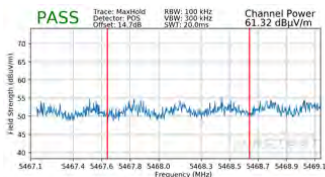
Plot 7-206. Radiated Lower Band Edge Plot (Peak – UNII Band 2C)
