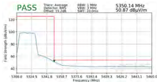
Plot 7-176. Radiated Upper Band Edge Plot (Average – UNII Band 2A)
