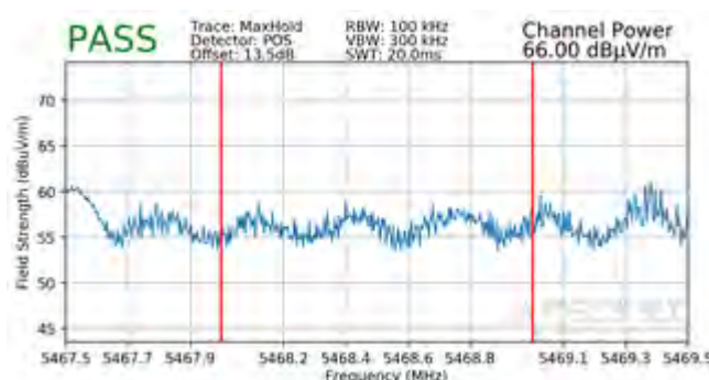
Plot 7-251. Radiated Lower Band Edge Plot (Peak – UNII Band 2C)
