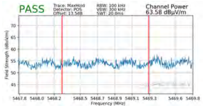
Plot 7-254. Radiated Band Edge Plot (Peak – WCP)
