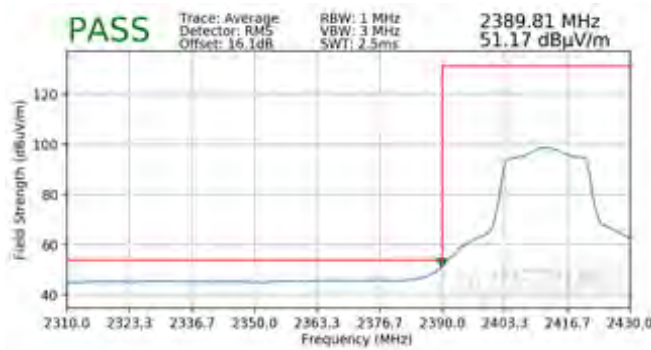
Plot 7-119. Radiated Restricted Band Edge Measurement MIMO with WCP (Average)
