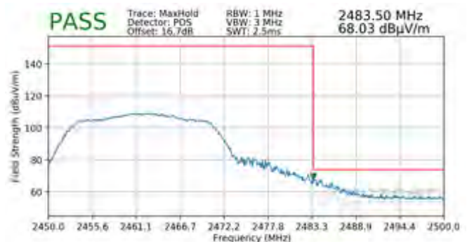
Plot 7-114. Radiated Restricted Upper Band Edge Measurement MIMO (Peak)
