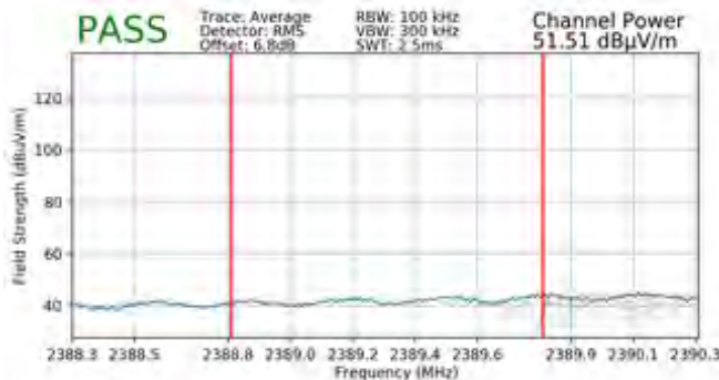
Plot 7-91. Radiated Restricted Lower Band Edge Measurement SISO ANT2 (Average)
