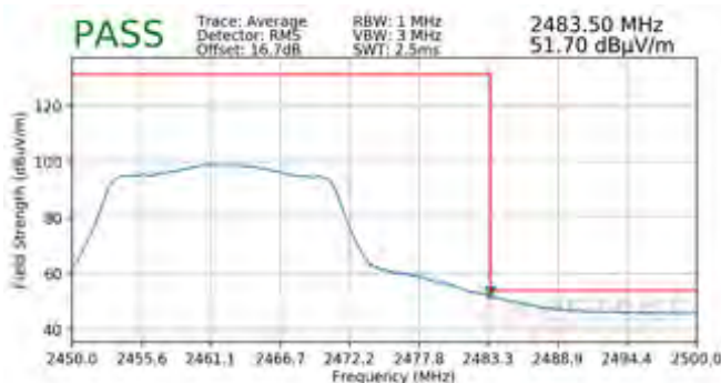
Plot 7-113. Radiated Restricted Upper Band Edge Measurement MIMO (Average)
