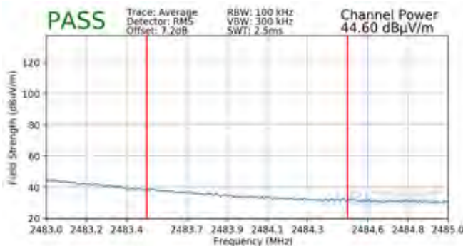
Plot 7-107. Radiated Restricted Upper Band Edge Measurement CDD (Average)
