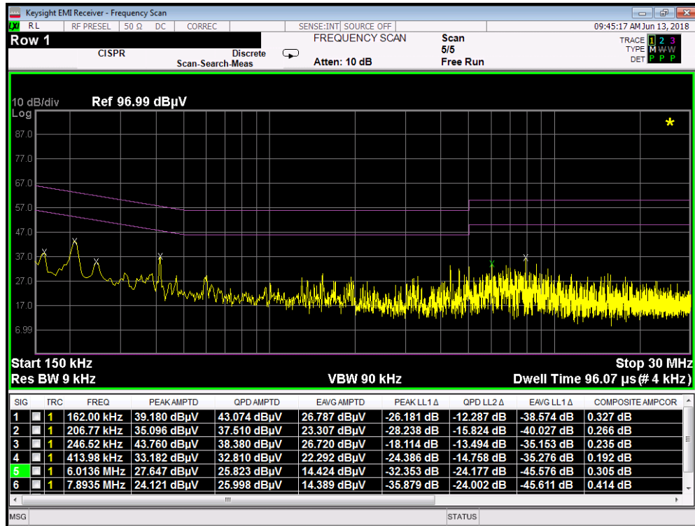
Plot 7-125. Line Conducted Plot with 802.11b (L1) with Wireless Charging Pad
