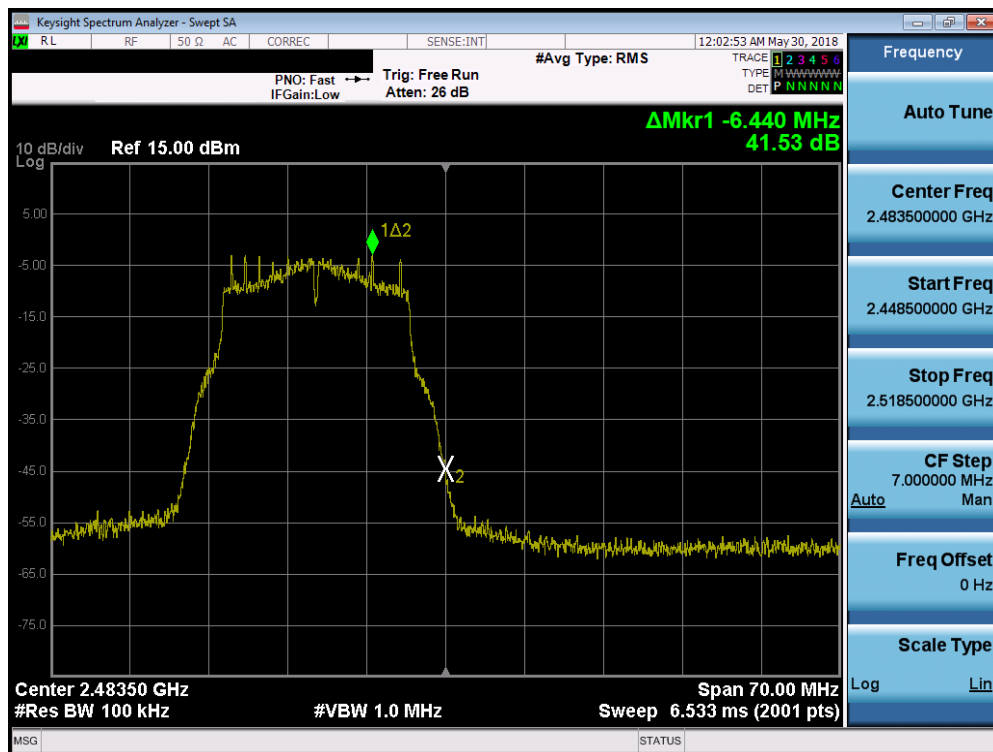
Plot 7-44. Band Edge Plot SISO ANT1 (802.11g - Ch. 13)
