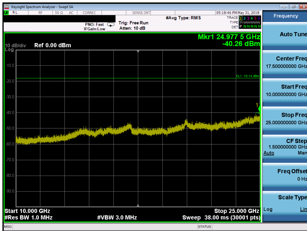
Plot 7-70. Conducted Spurious Plot SISO ANT2 (802.11b – Ch. 6)
