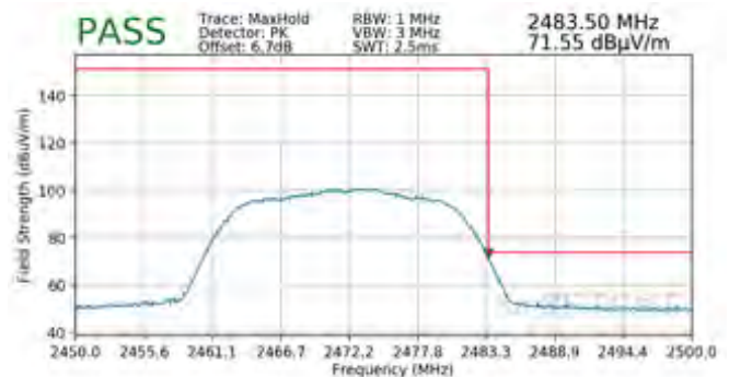
Plot 7-118. Radiated Restricted Upper Band Edge Measurement MIMO (Peak)
