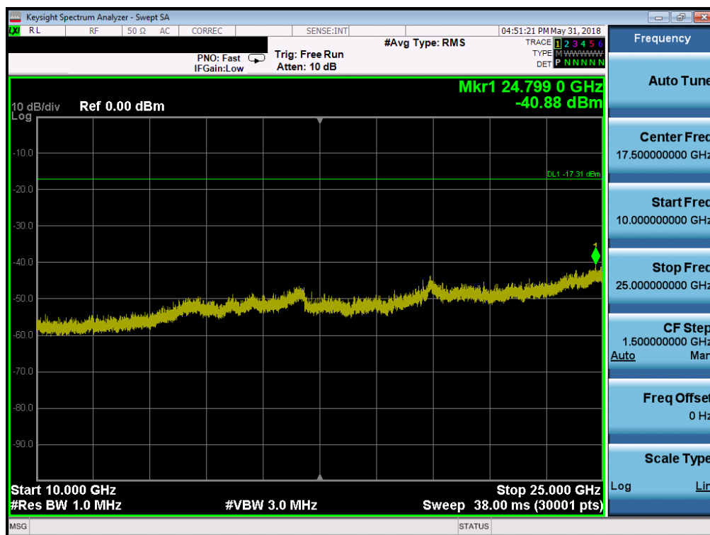
Plot 7-64. Conducted Spurious Plot SISO ANT1 (802.11b – Ch. 6)
