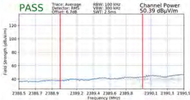
Plot 7-101. Radiated Restricted Lower Band Edge Measurement CDD (Average)
