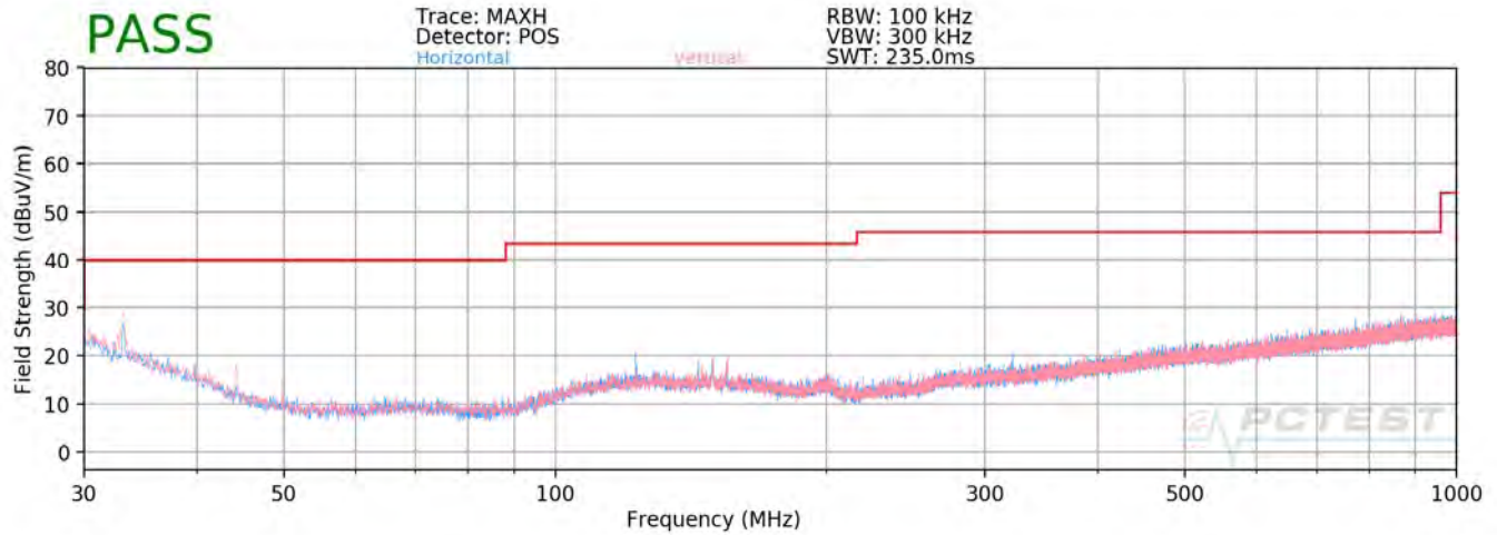
Plot 7-122. Radiated Spurious Plot below 1GHz SISO ANT2
