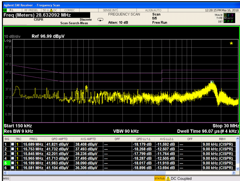
Plot 7-126. Line Conducted Plot with 802.11b (N) with Wireless Charging Pad
