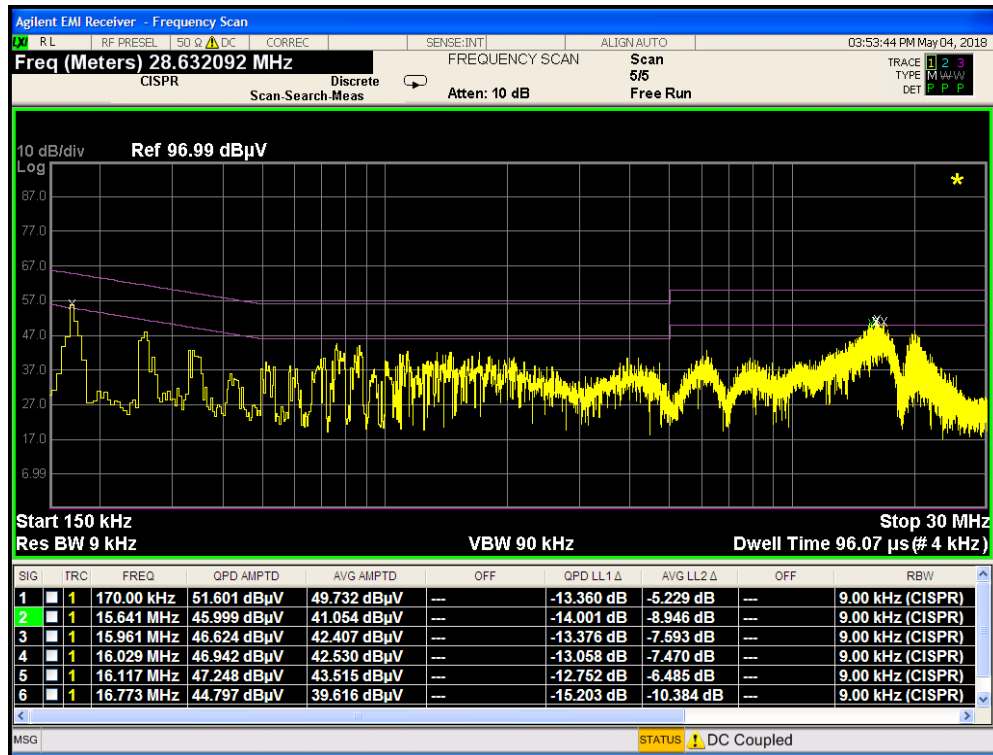
Plot 7-123. Line Conducted Plot with 802.11b (L1) with Travel Adapter
