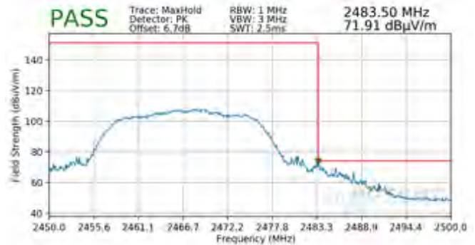
Plot 7-116. Radiated Restricted Upper Band Edge Measurement MIMO (Peak)
