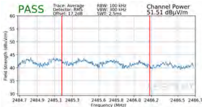
Plot 7-103. Radiated Restricted Upper Band Edge Measurement CDD (Average)
