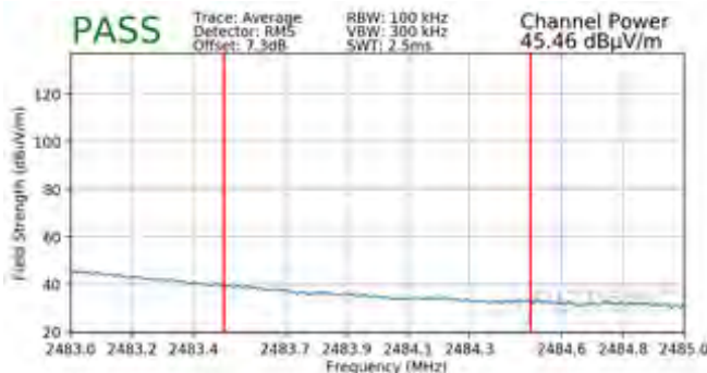
Plot 7-87. Radiated Restricted Band Edge Measurement SISO ANT1 (Average)
