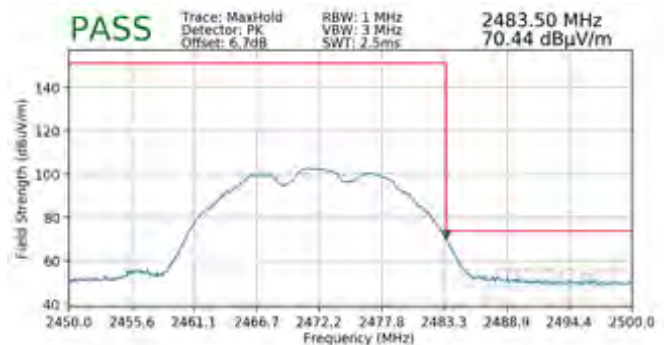
Plot 7-108. Radiated Restricted Upper Band Edge Measurement CDD (Peak)
