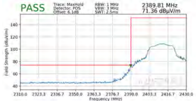
Plot 7-82. Radiated Restricted Lower Band Edge Measurement SISO ANT1 (Peak)
