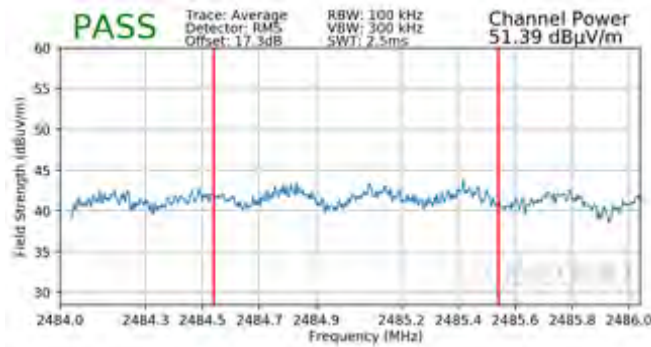
Plot 7-109. Radiated Restricted Band Edge Measurement CDD with WCP (Average)
