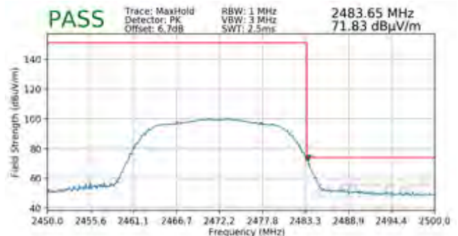
Plot 7-88. Radiated Restricted Band Edge Measurement SISO ANT1 (Peak)
