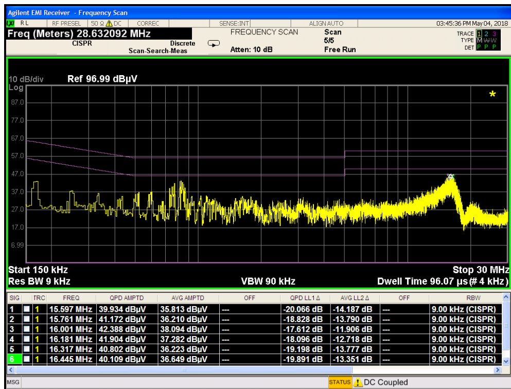
Plot 7-124. Line Conducted Plot with 802.11b (N) with Travel Adapter
