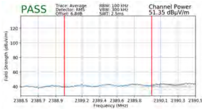
Plot 7-99. Radiated Restricted Band Edge Measurement SISO ANT2 with WCP (Average)
