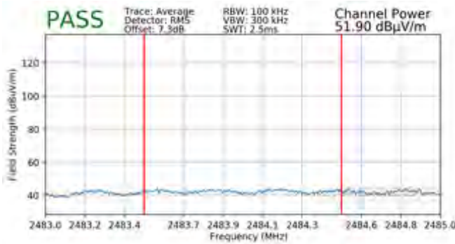
Plot 7-105. Radiated Restricted Upper Band Edge Measurement CDD (Average)
