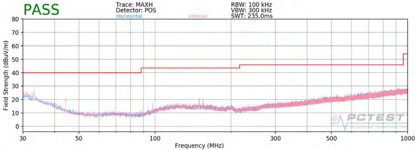
Plot 7-121. Radiated Spurious Plot below 1GHz SISO ANT1
