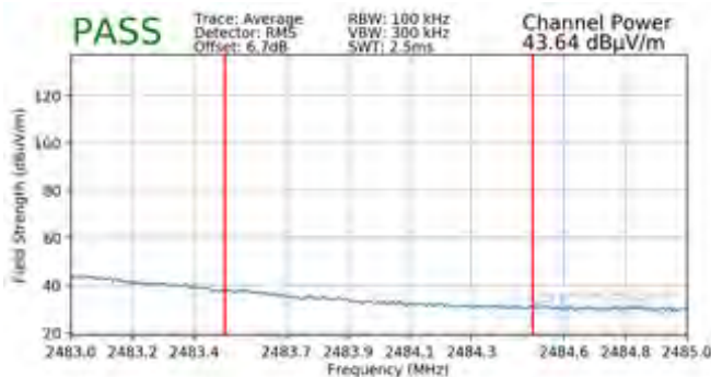
Plot 7-117. Radiated Restricted Upper Band Edge Measurement MIMO (Average)
