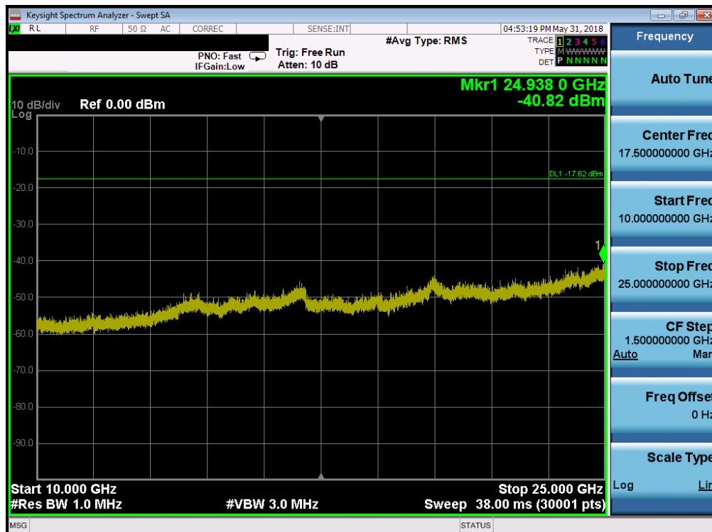
Plot 7-66. Conducted Spurious Plot SISO ANT1 (802.11b – Ch. 11)
