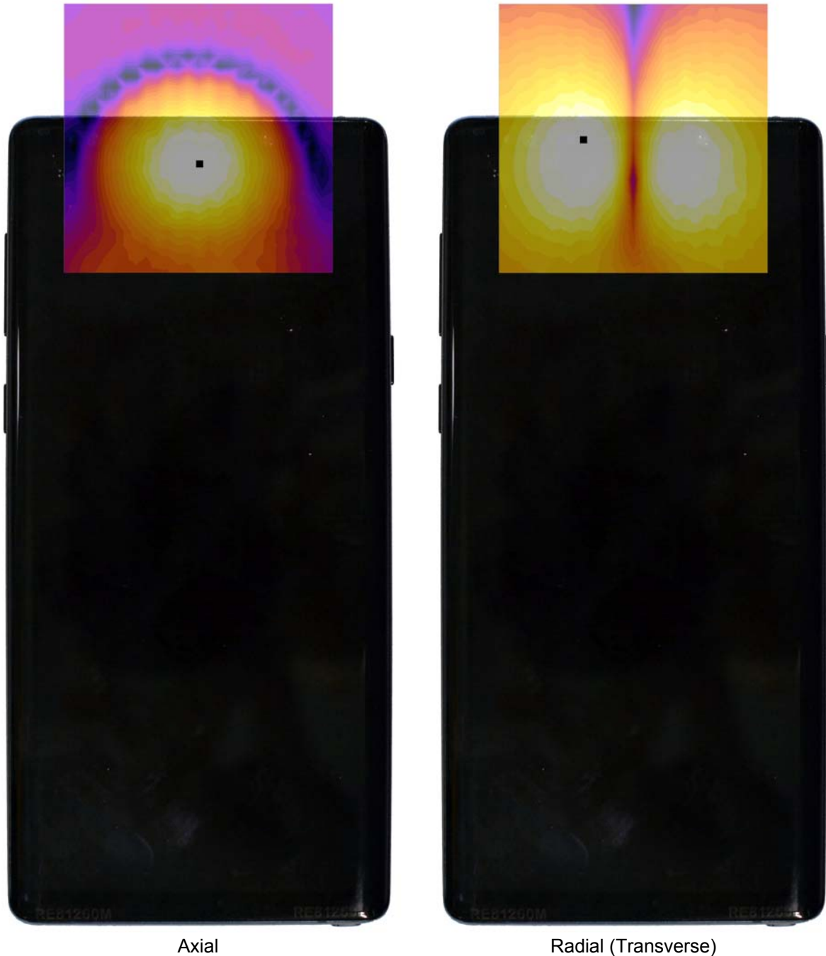
Figure 14-3 T-Coil Scan Overlay Magnetic Field Distributions
