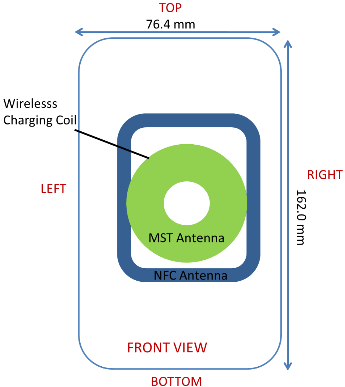
Figure F-2 NFC Antenna Locations
