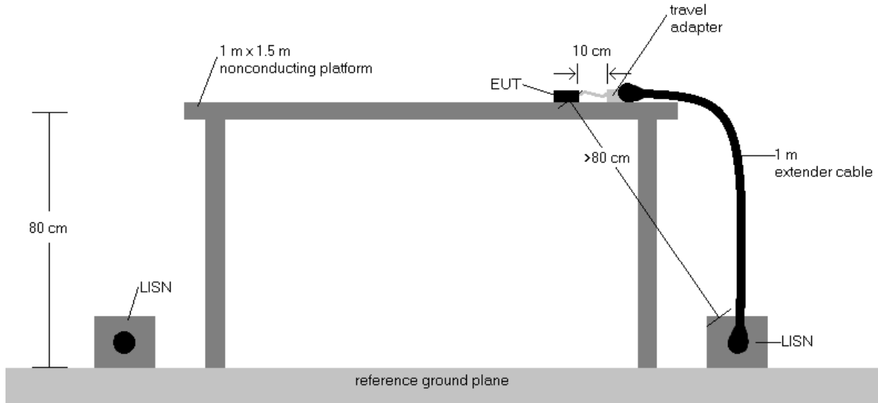
Figure 7-3. Test Instrument & Measurement Setup
