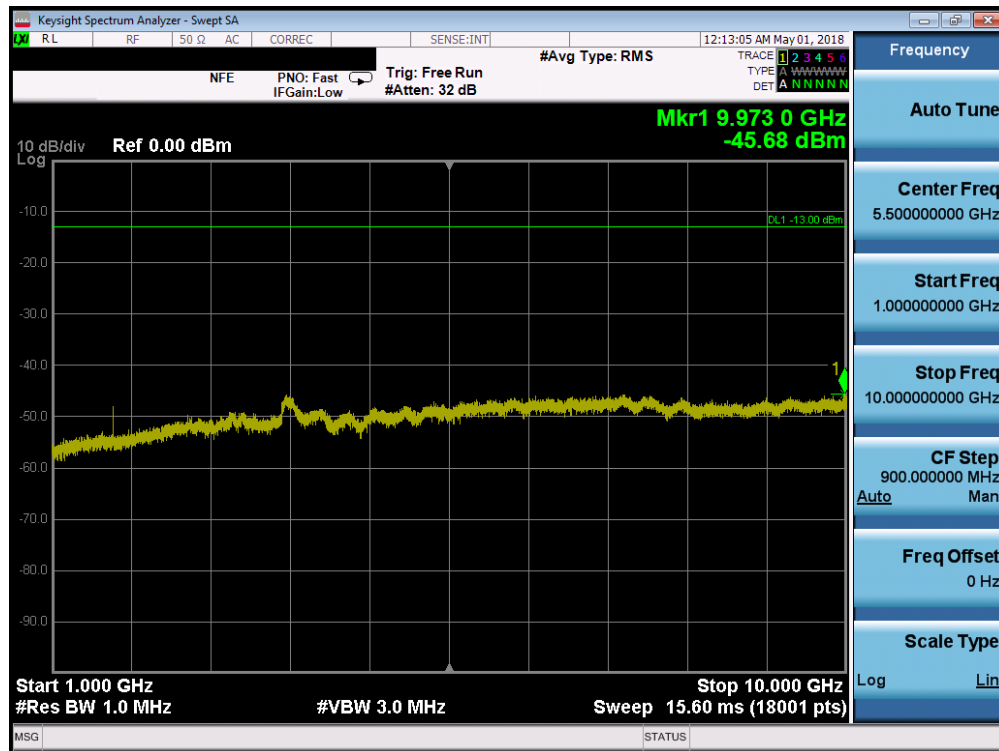
Plot 7-120. Conducted Spurious Plot (Band 26/5 - 3.0MHz QPSK - RB Size 1, RB Offset 0 - High Channel)
