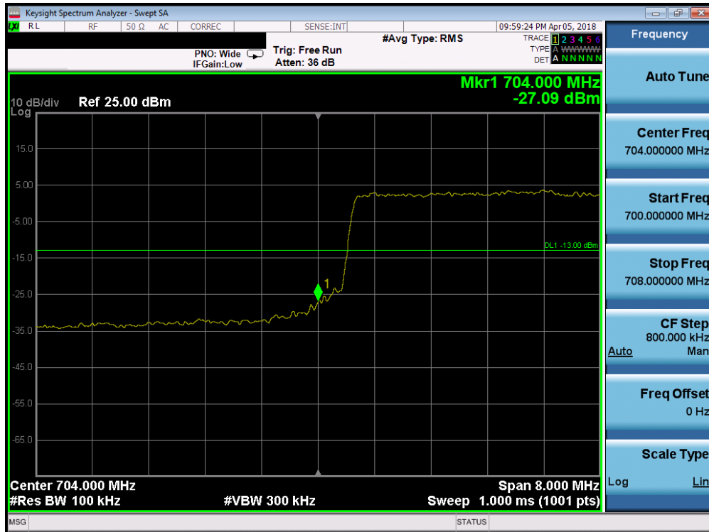
Plot 7-165. Lower Band Edge Plot (Band 17 - 10.0MHz QPSK - Full RB Configuration)
