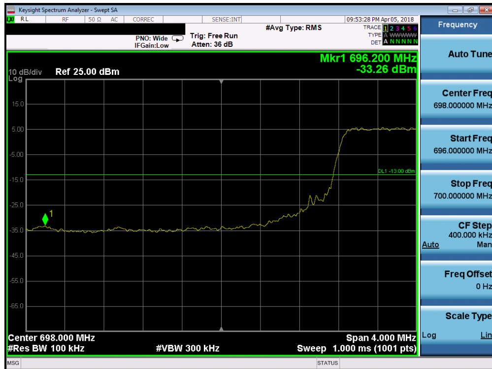
Plot 7-161. Lower Band Edge Plot (Band 12 - 5.0MHz QPSK - Full RB Configuration)
