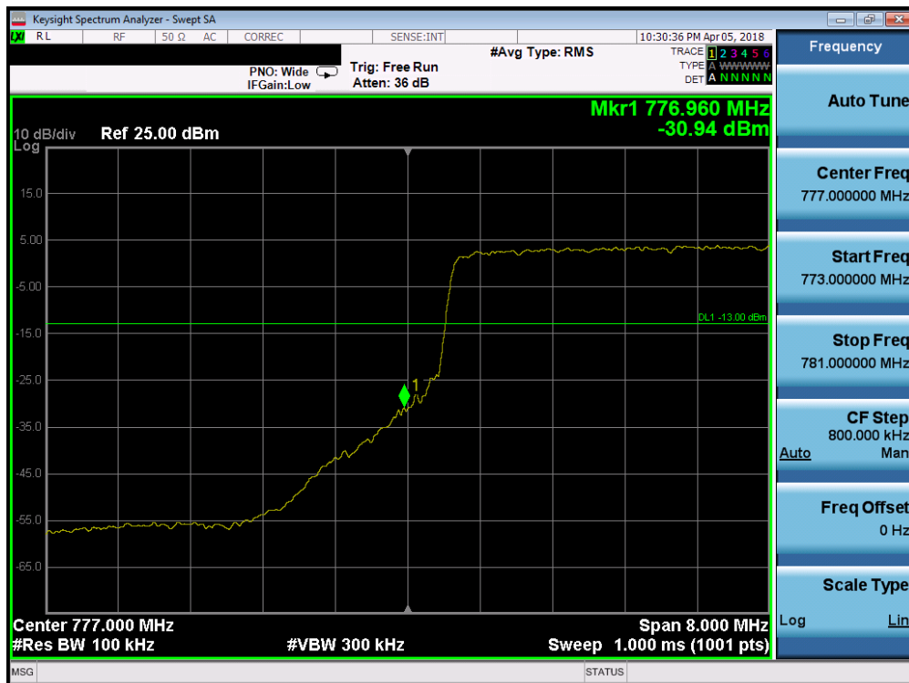
Plot 7-169. Lower Band Edge Plot (Band 13 - 10.0MHz QPSK - Full RB Configuration)
