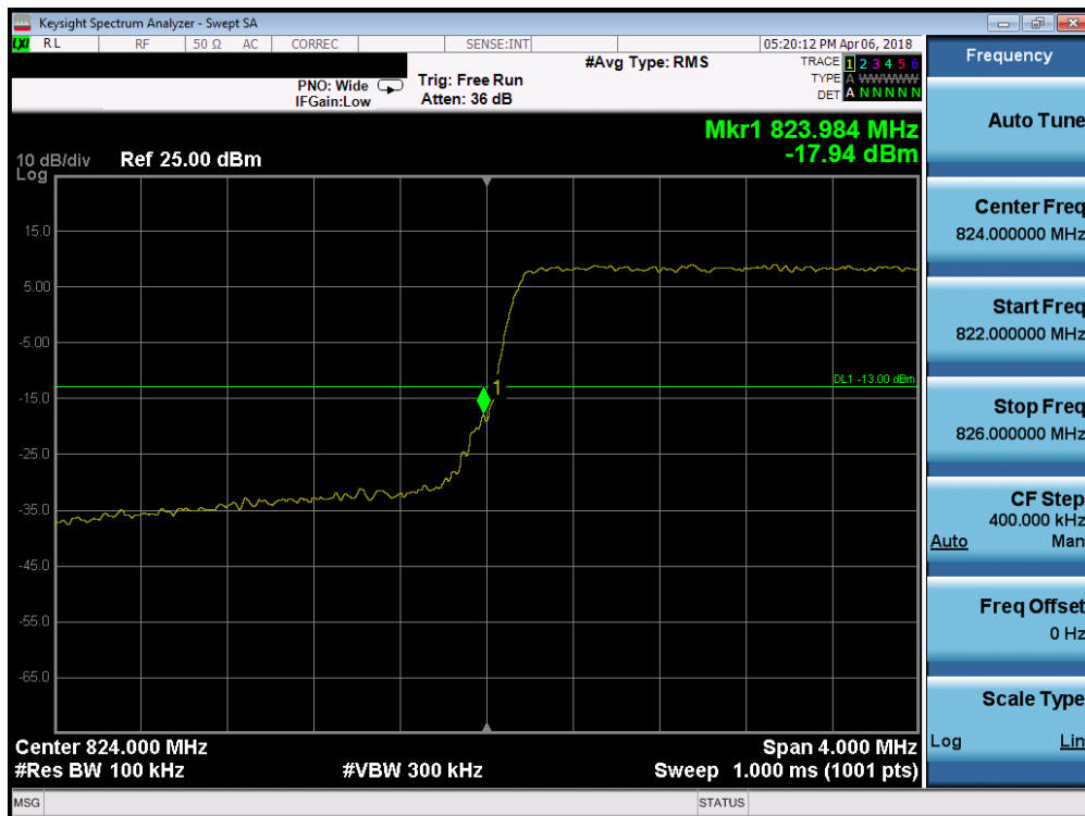
Plot 7-173. Lower Band Edge Plot (Band 26/5 - 3.0MHz QPSK - Full RB Configuration)
