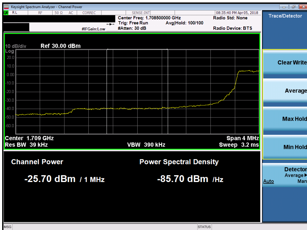
Plot 7-188. Lower Extended Band Edge Plot (Band 66/4 - 3.0MHz QPSK - Full RB Configuration)
