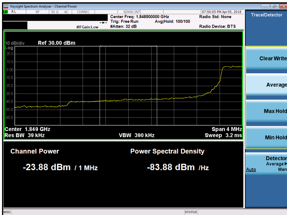
Plot 7-224. Lower Extended Band Edge Plot (Band 25/2 - 3.0MHz QPSK - Full RB Configuration)
