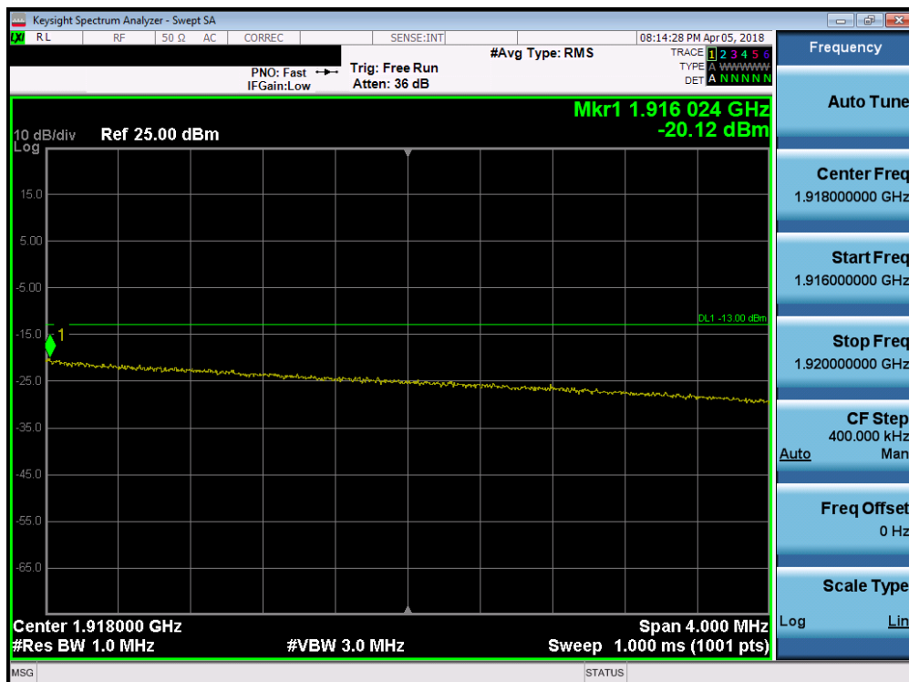
Plot 7-240. Upper Extended Band Edge Plot (Band 25 - 10.0MHz QPSK - Full RB Configuration)
