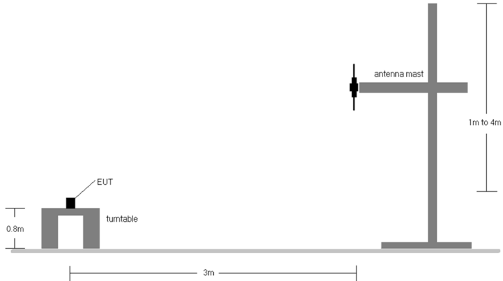
Figure 1-1. Radiated Test Setup <1GHz
