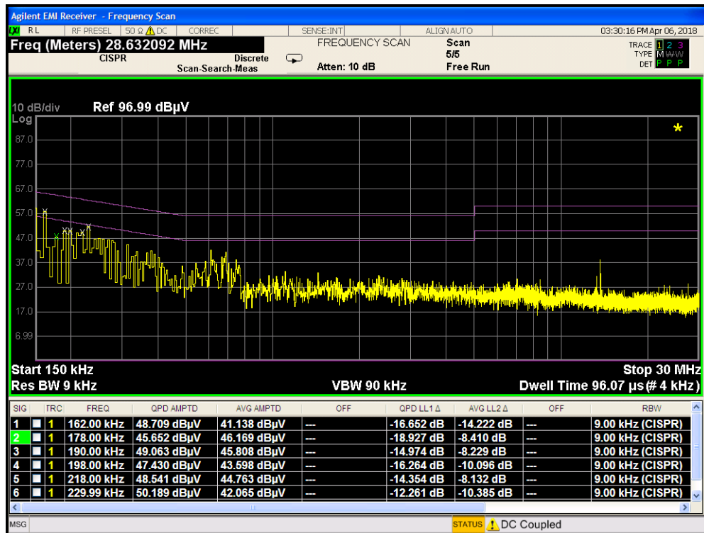
Plot 7-6. Line-Conducted Test Plot with Travel Adapter (N)
