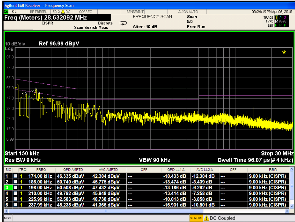
Plot 7-5. Line-Conducted Test Plot with Travel Adapter (L1)
