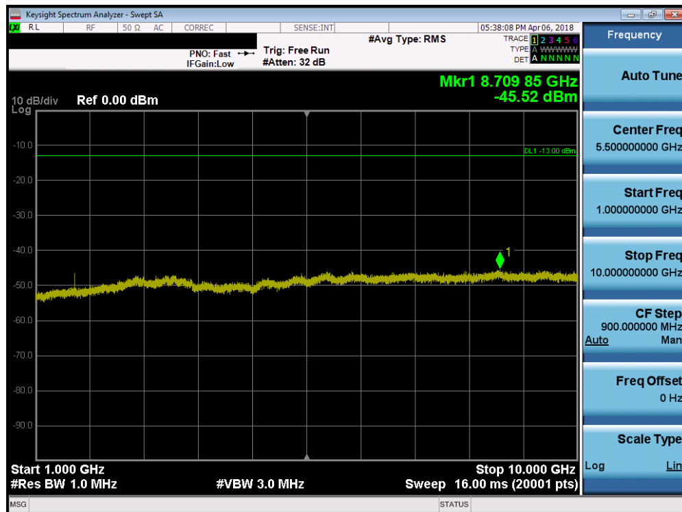
Plot 7-21. Conducted Spurious Plot (LTE B26 – 1.4MHz QPSK – RB Size 1, RB Offset 0 – High Channel)
