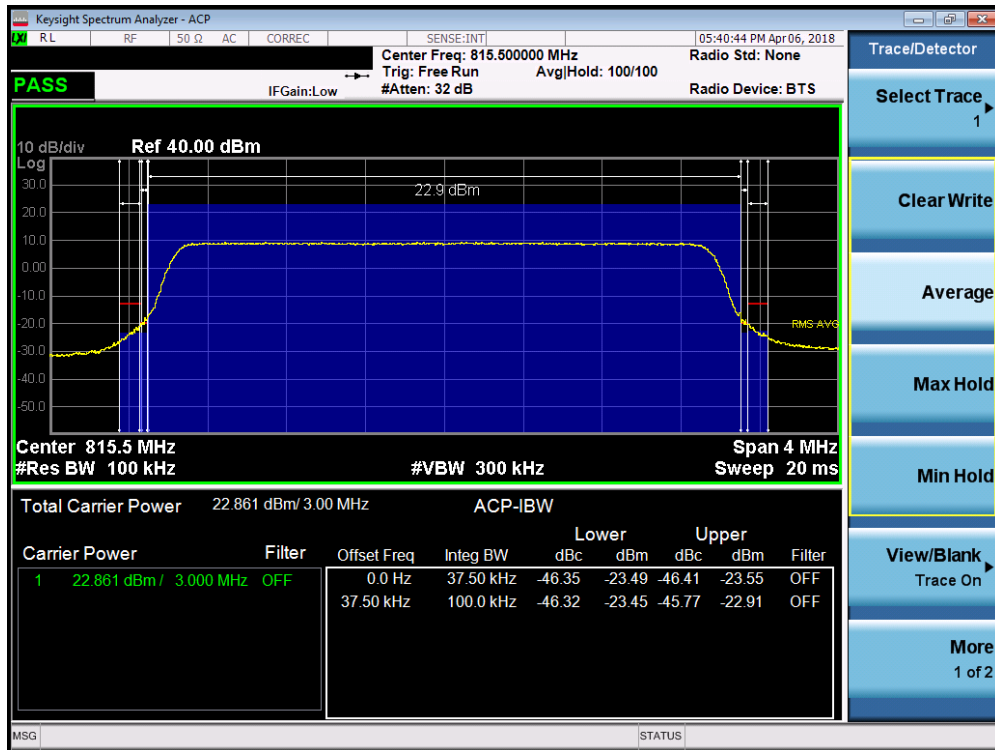
Plot 7-24. Channel Edge Plot (LTE B26 – 3MHz QPSK – RB Size 15– Low Channel)
