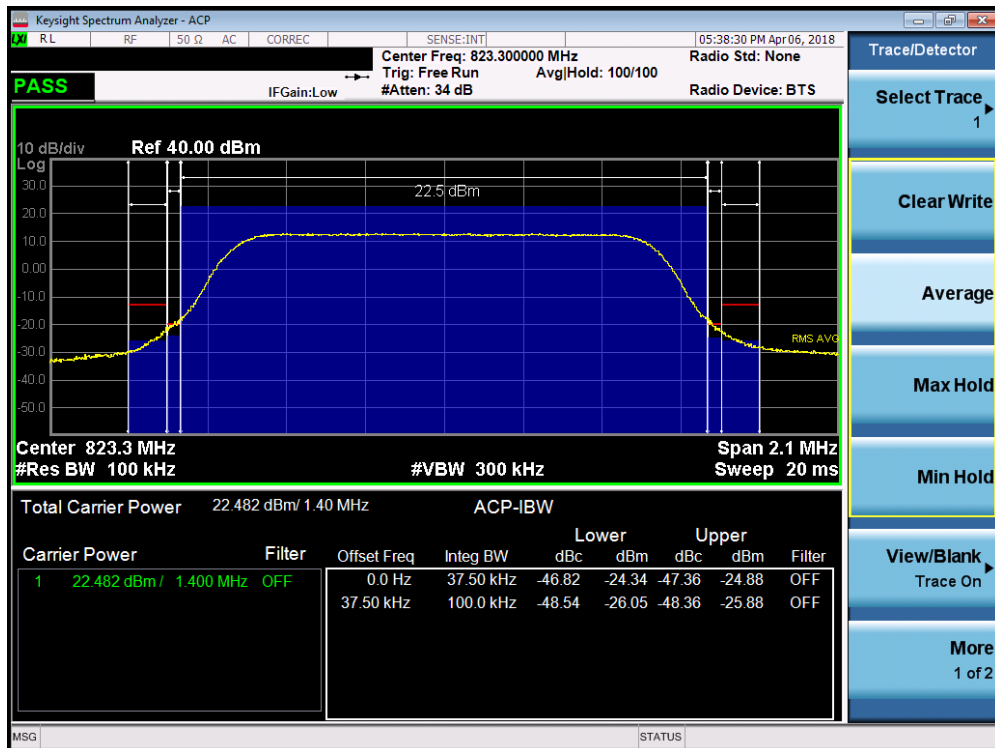
Plot 7-23. Channel Edge Plot (LTE B26 – 1.4MHz QPSK – RB Size 6 – High Channel)
