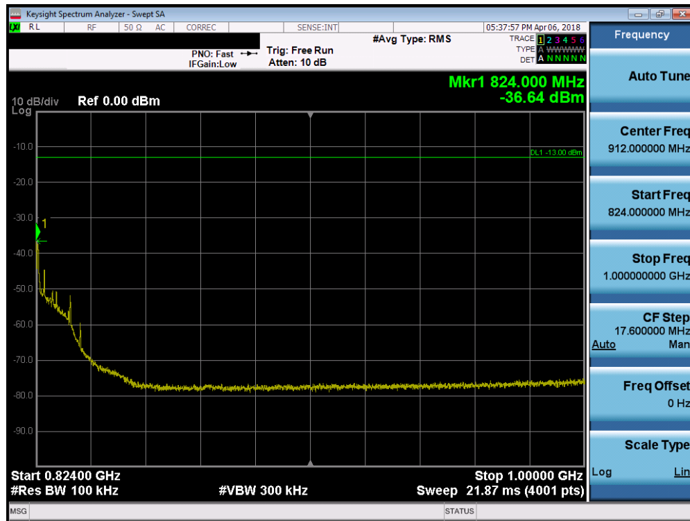
Plot 7-20. Conducted Spurious Plot (LTE B26 – 1.4MHz QPSK – RB Size 1, RB Offset 0 – High Channel)
