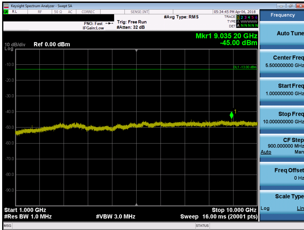
Plot 7-18. Conducted Spurious Plot (LTE B26 – 1.4MHz QPSK – RB Size 1, RB Offset 0 – Low Channel)
