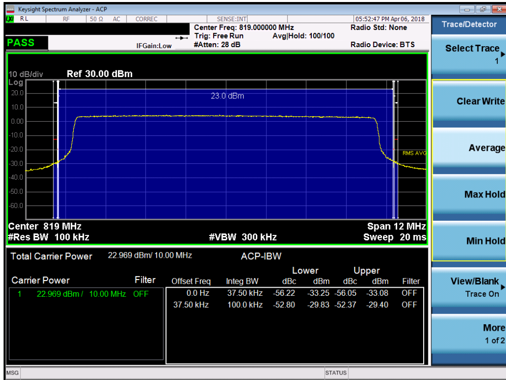
Plot 7-28. Channel Edge Plot (LTE B26 – 10MHz QPSK – RB Size 50)
