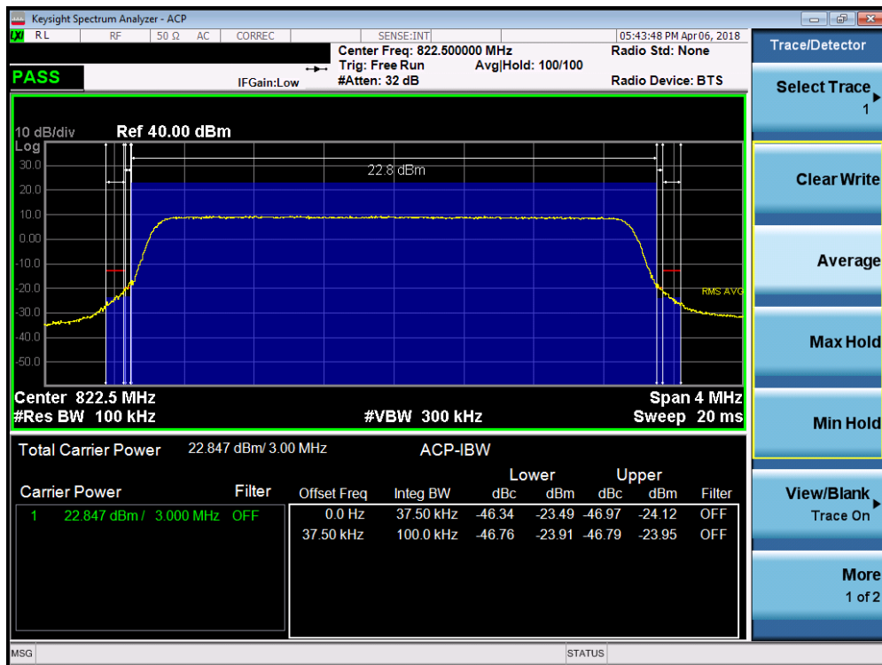
Plot 7-25. Channel Edge Plot (LTE B26 – 3MHz QPSK – RB Size 15 – High Channel)
