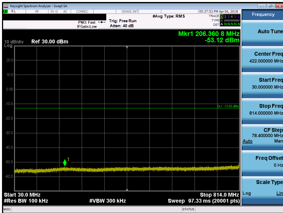
Plot 7-19. Conducted Spurious Plot (LTE B26 – 1.4MHz QPSK – RB Size 1, RB Offset 0 – High Channel)
