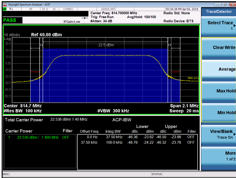
Plot 7-22. Channel Edge Plot (LTE B26 – 1.4MHz QPSK – RB Size 6– Low Channel)
