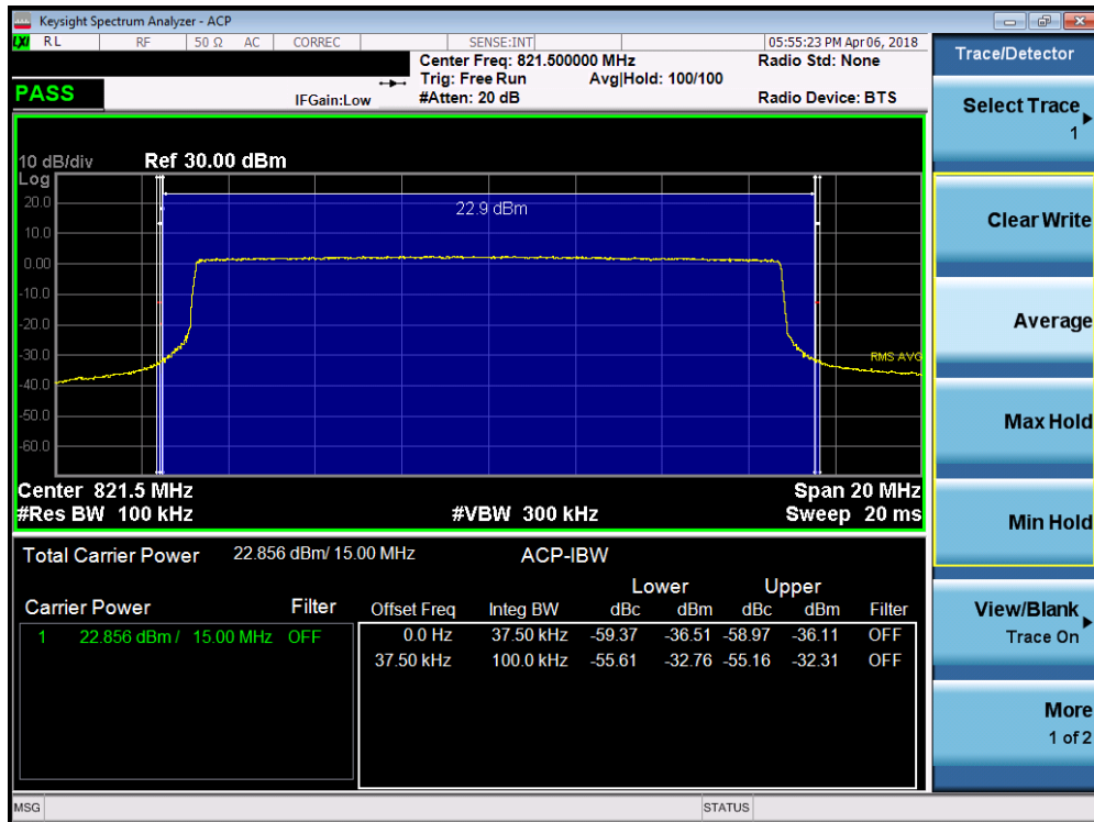
Plot 7-29. Channel Edge Plot (LTE B26 – 15MHz QPSK – RB Size 75)
