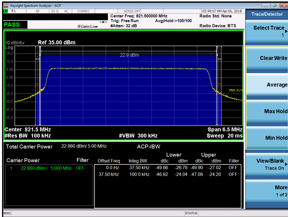
Plot 7-27. Channel Edge Plot (LTE B26 – 5MHz QPSK – RB Size 25 – High Channel)
