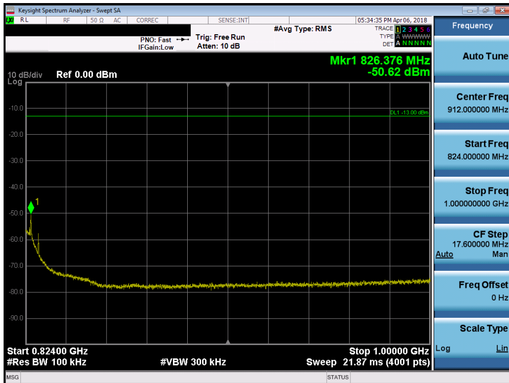
Plot 7-17. Conducted Spurious Plot (LTE B26 – 1.4MHz QPSK – RB Size 1, RB Offset 0 – Low Channel)
