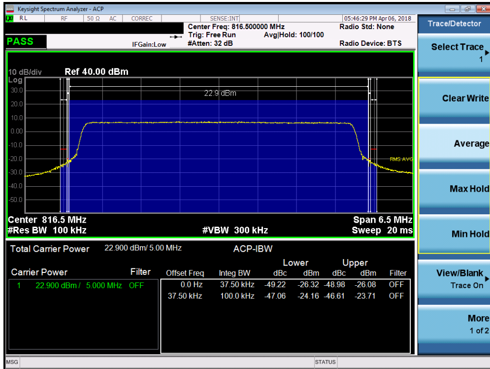
Plot 7-26. Channel Edge Plot (LTE B26 – 5MHz QPSK – RB Size 25– Low Channel)
