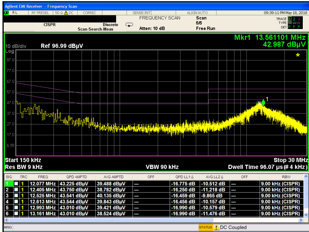
Plot 7-51. Line-Conducted Test Plot with Travel Adapter (L1)
