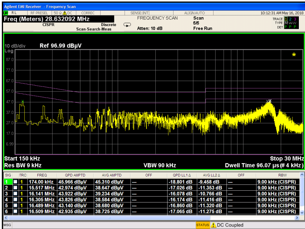
Plot 7-53. Line-Conducted Test Plot with Wireless Charging Pad (L1)
