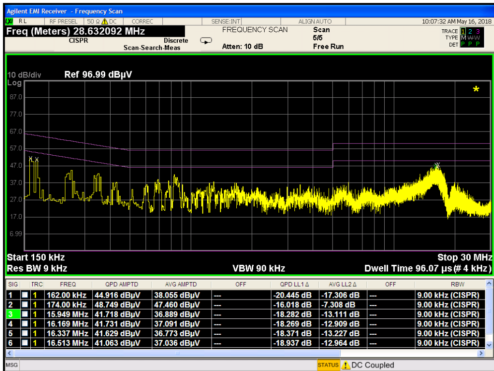
Plot 7-54. Line-Conducted Test Plot with Wireless Charging Pad (N)
