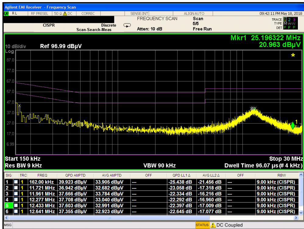
Plot 7-52. Line-Conducted Test Plot with Travel Adapter (N)
