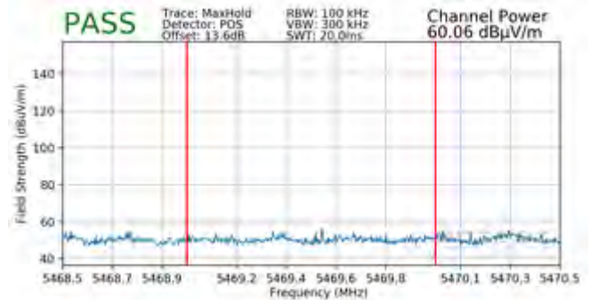
Plot 7-192. Radiated Lower Band Edge Plot (Peak – UNII Band 2C)
