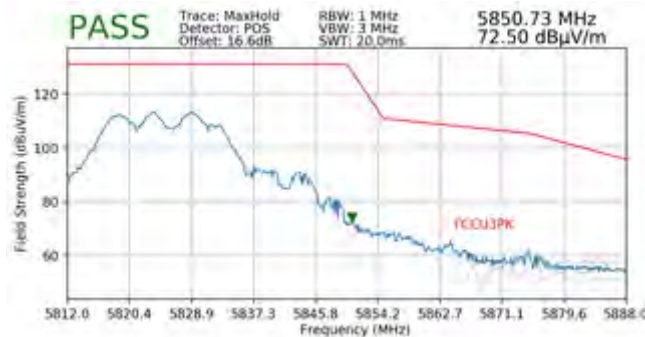
Plot 7-265. Radiated Upper Band Edge Plot (Peak – UNII Band 3)
