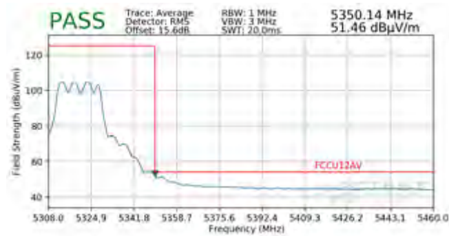
Plot 7-266. Radiated Band Edge Plot (Average – WCP)
