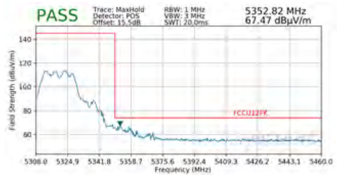
Plot 7-267. Radiated Band Edge Plot (Peak – WCP)
