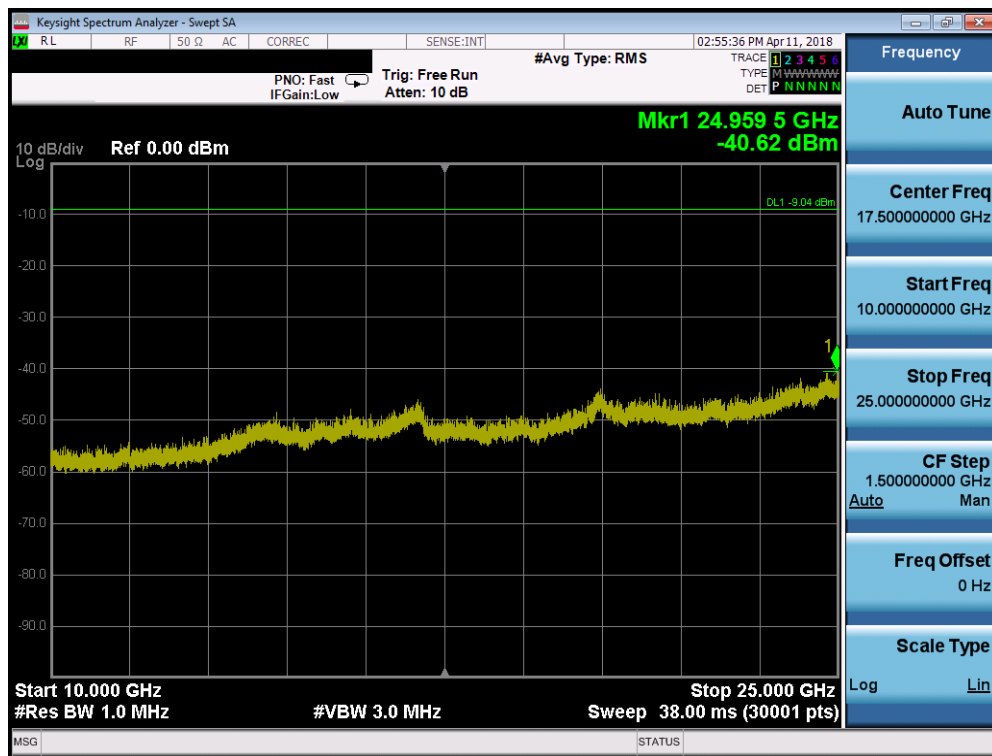
Plot 7-64. Conducted Spurious Plot SISO ANT1 (802.11b – Ch. 6)
