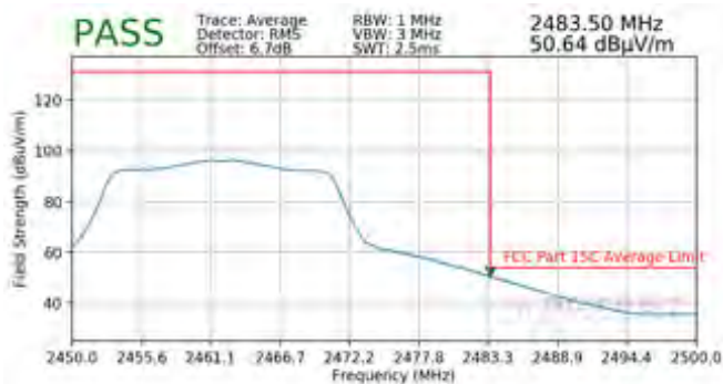
Plot 7-93. Radiated Restricted Upper Band Edge Measurement SISO ANT2 (Average)
