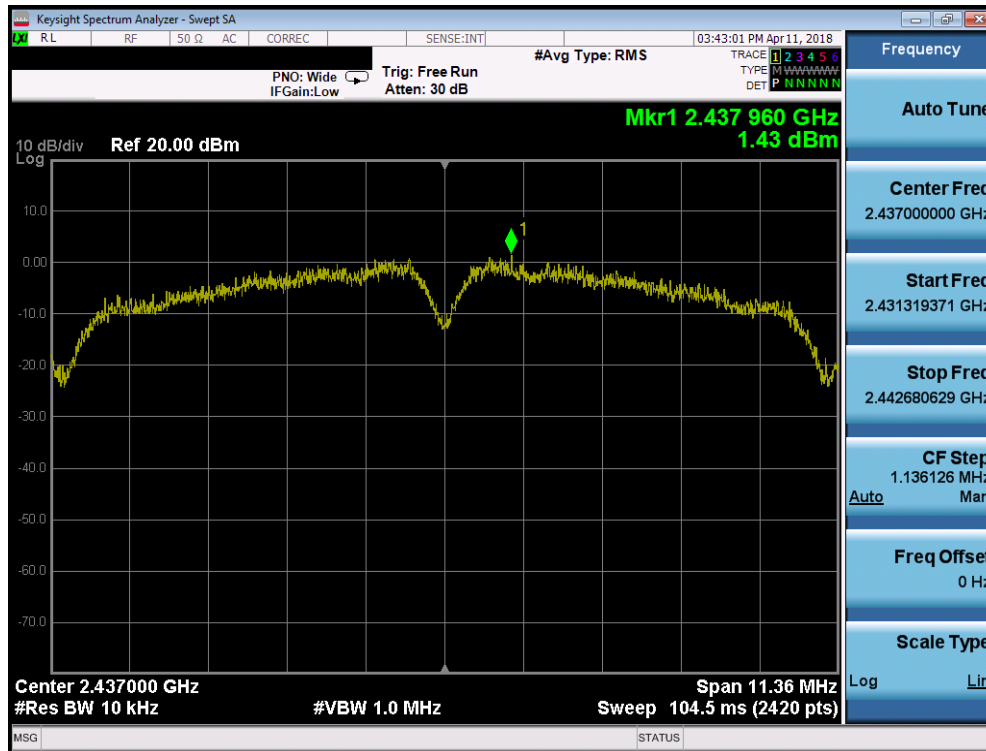
Plot 7-29. Power Spectral Density Plot SISO ANT2 (802.11b – Ch. 6)
