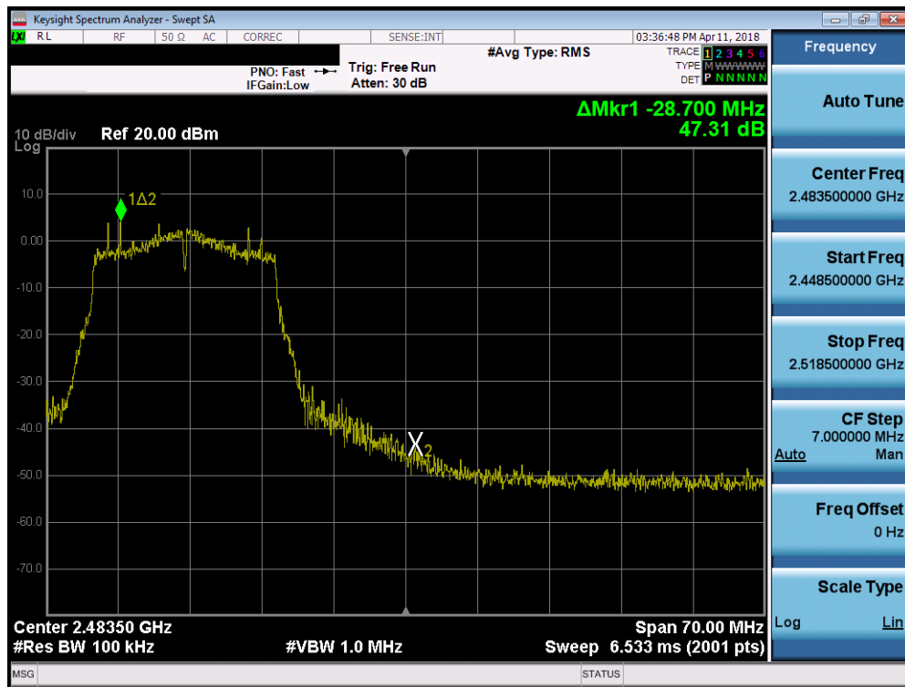
Plot 7-46. Band Edge Plot SISO ANT1 (802.11n (2.4GHz) – Ch. 11)
