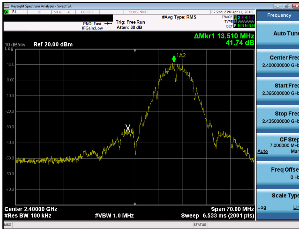
Plot 7-37. Band Edge Plot SISO ANT1 (802.11b – Ch. 1)
