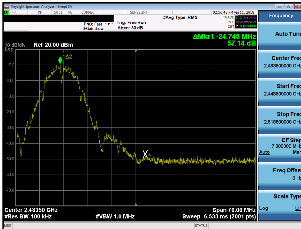
Plot 7-38. Band Edge Plot SISO ANT1 (802.11b – Ch. 11)
