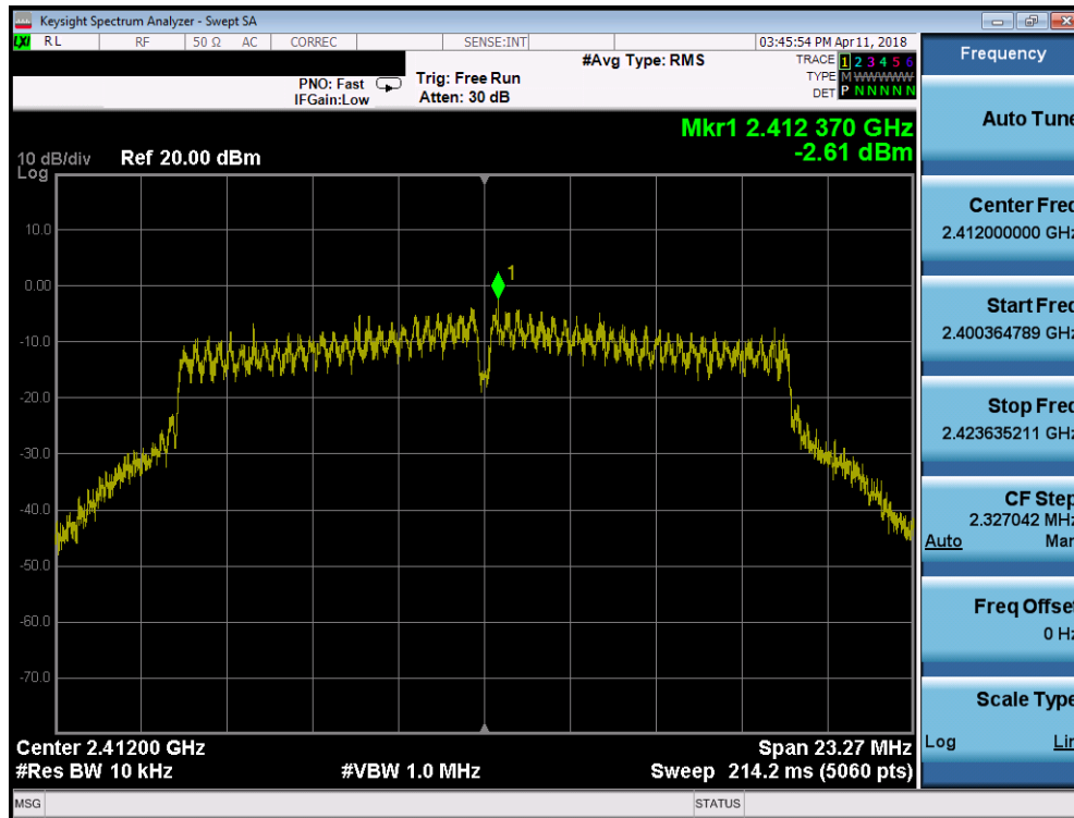
Plot 7-31. Power Spectral Density Plot SISO ANT2 (802.11g – Ch. 1)
