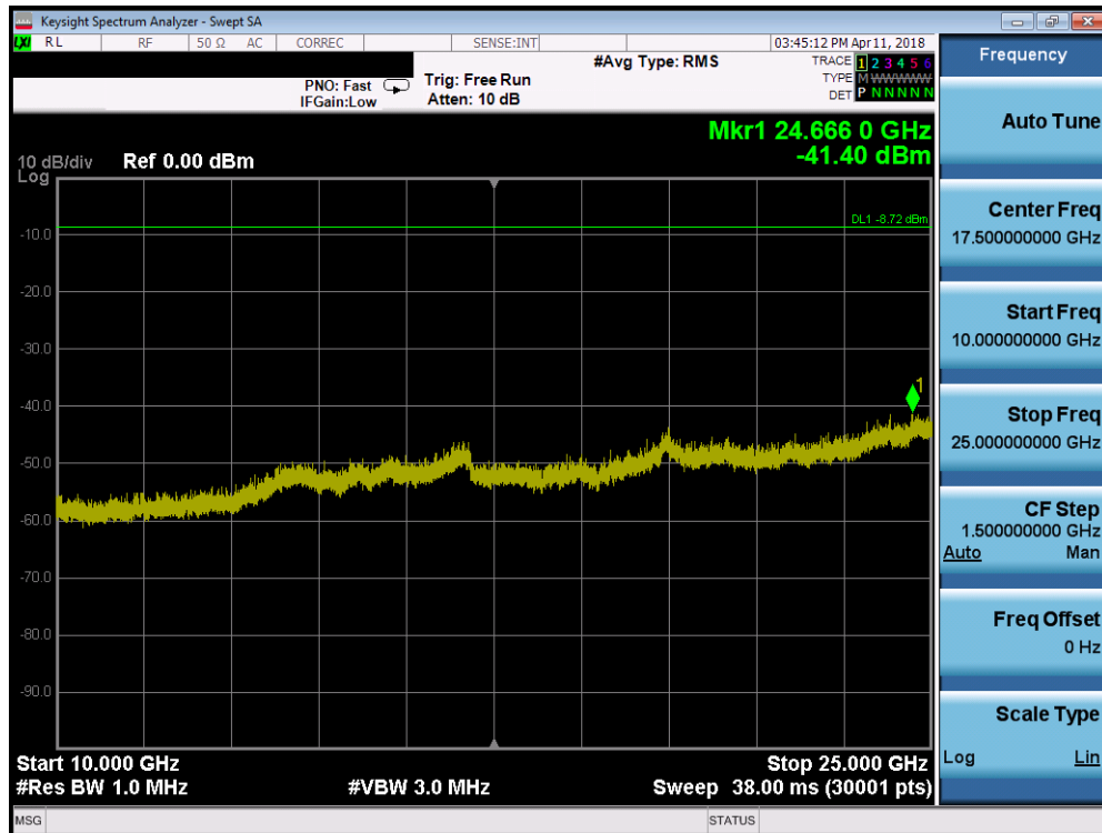
Plot 7-72. Conducted Spurious Plot SISO ANT2 (802.11b – Ch. 11)
