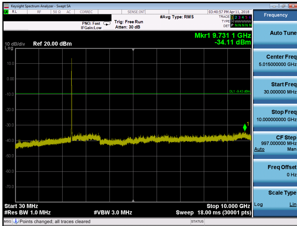
Plot 7-67. Conducted Spurious Plot SISO ANT2 (802.11b – Ch. 1)
