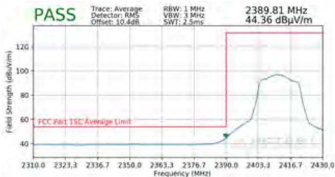
Plot 7-81. Radiated Restricted Lower Band Edge Measurement SISO ANT1 (Average)
