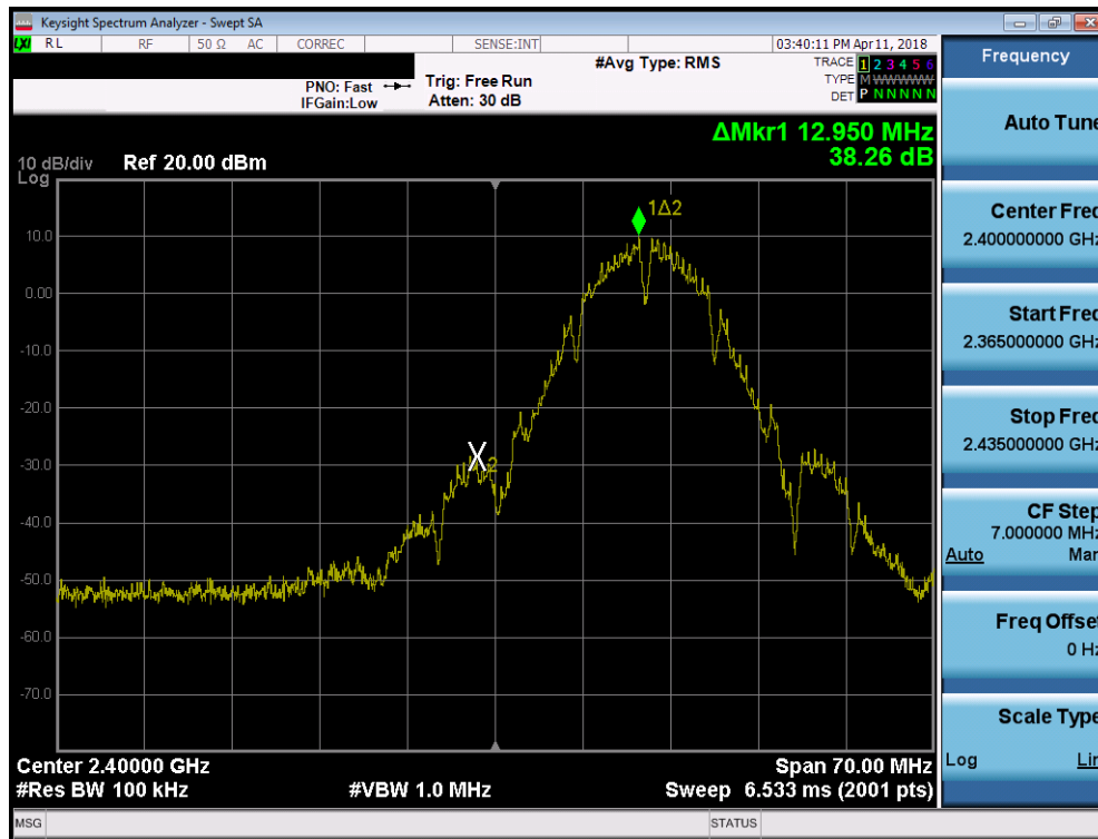
Plot 7-49. Band Edge Plot SISO ANT2 (802.11b – Ch. 1)
