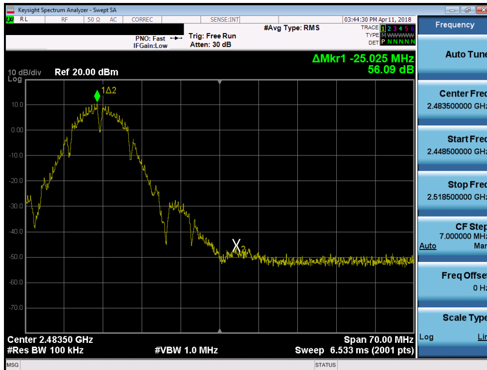
Plot 7-50. Band Edge Plot SISO ANT2 (802.11b – Ch. 11)
