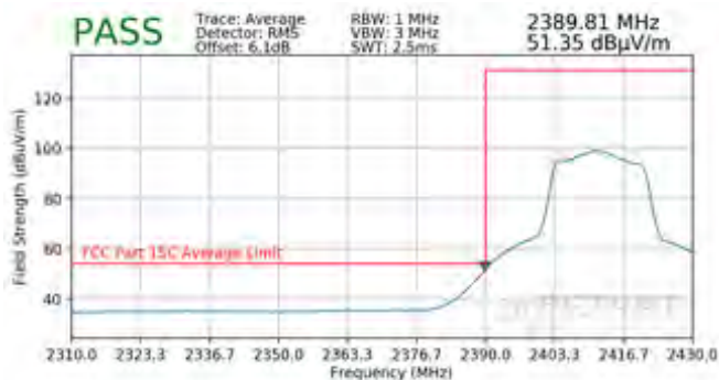
Plot 7-101. Radiated Restricted Lower Band Edge Measurement MIMO (Average)
