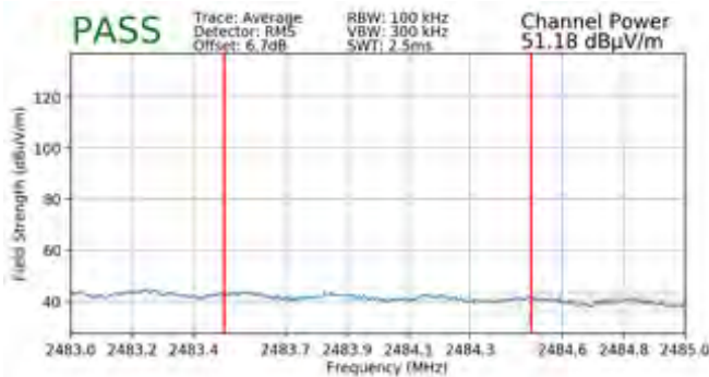
Plot 7-109. Radiated Restricted Band Edge Measurement MIMO with WCP (Average)
