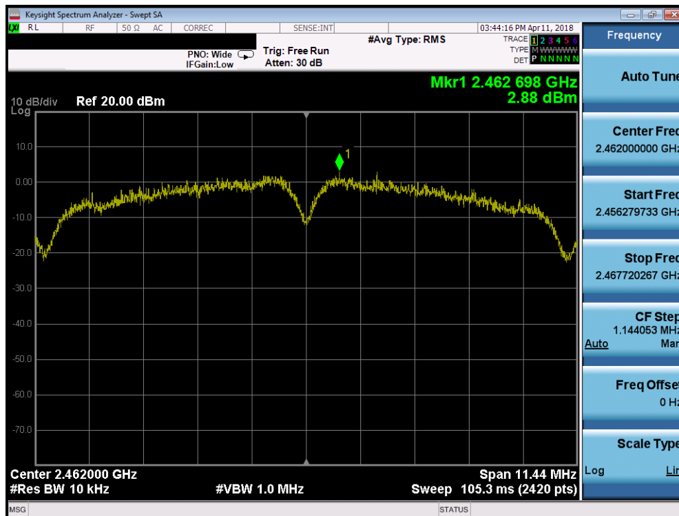
Plot 7-30. Power Spectral Density Plot SISO ANT2 (802.11b – Ch. 11)
