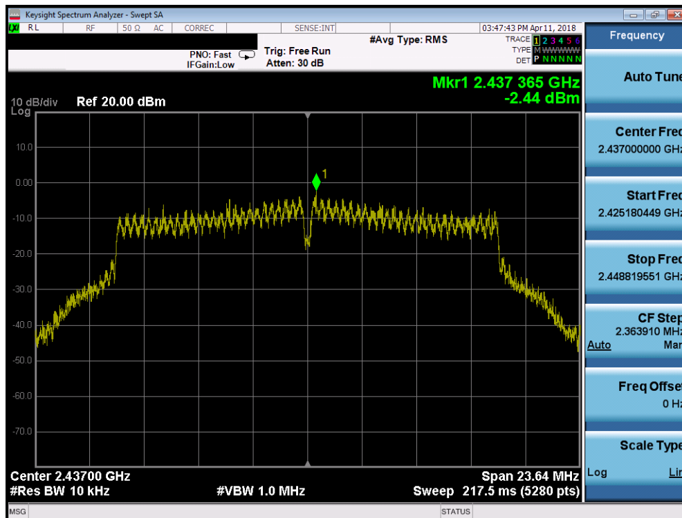
Plot 7-32. Power Spectral Density Plot SISO ANT2 (802.11g – Ch. 6)
