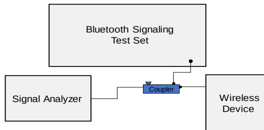
Figure 9-5 Power Measurement Setup
